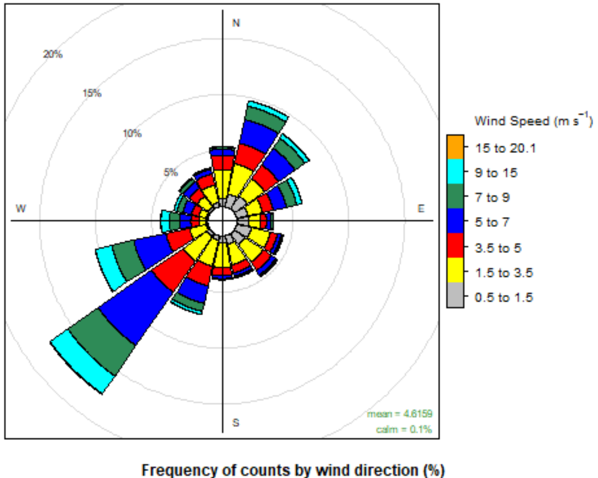
Figure 3-2: Distribution wind speeds and wind directions (wind from) observed at Auckland Airport (2019 - 2023)
