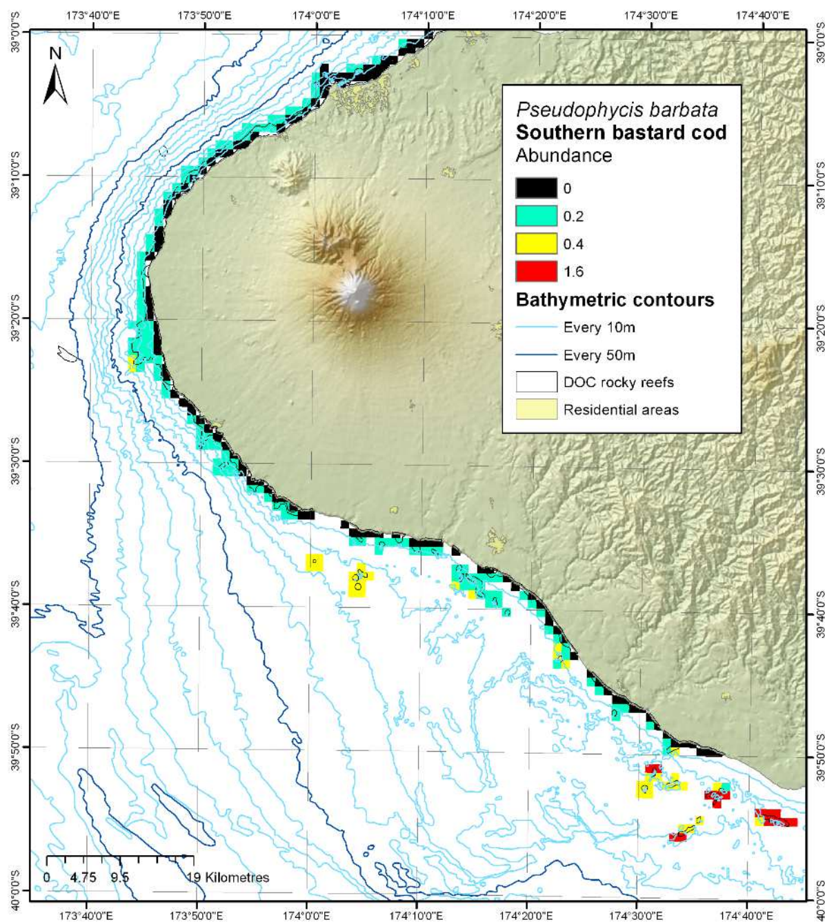
Figure 10-16: Modelled distribution and abundance of southern bastard cod on Taranaki subtidal reefs.
