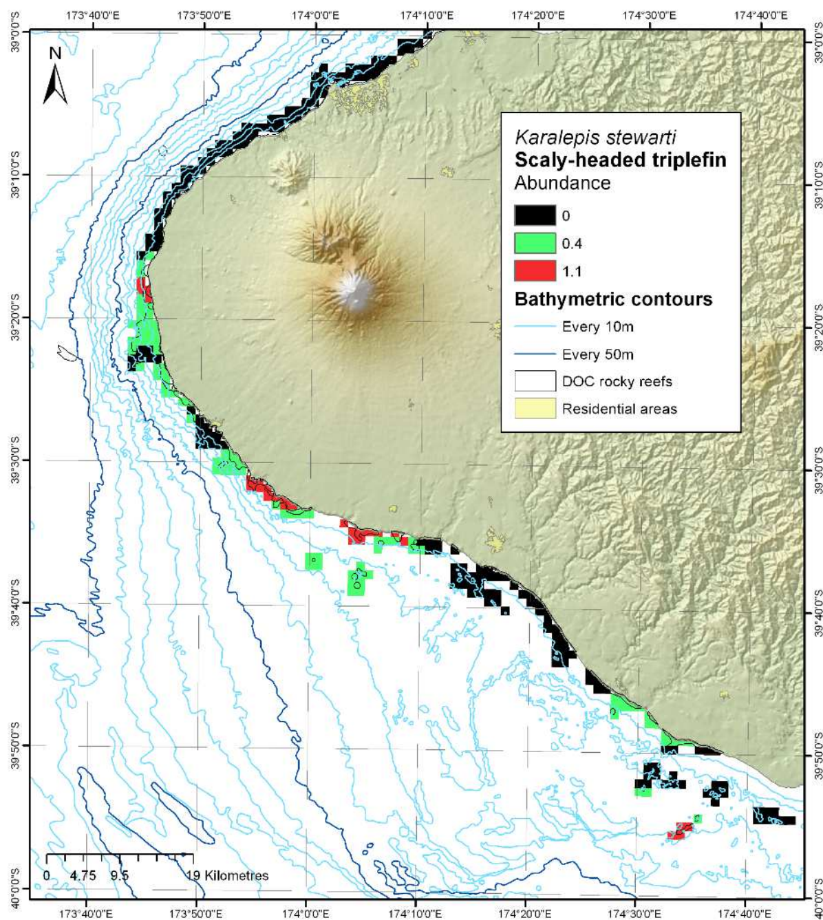
Figure 10-12: Modelled distribution and abundance of scaly-headed triplefin on Taranaki subtidal reefs.
