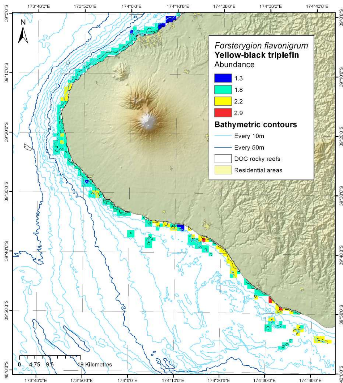
Figure 10-36: Modelled distribution and abundance of yellow-black triplefin on Taranaki subtidal reefs.
