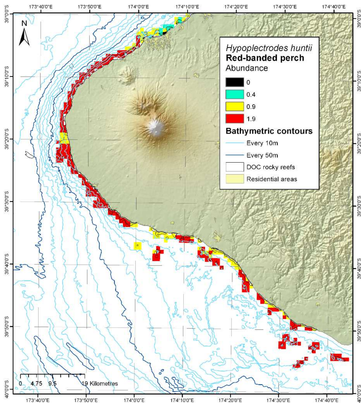
Figure 10-21: Modelled distribution and abundance of red-banded perch on Taranaki subtidal reefs.
