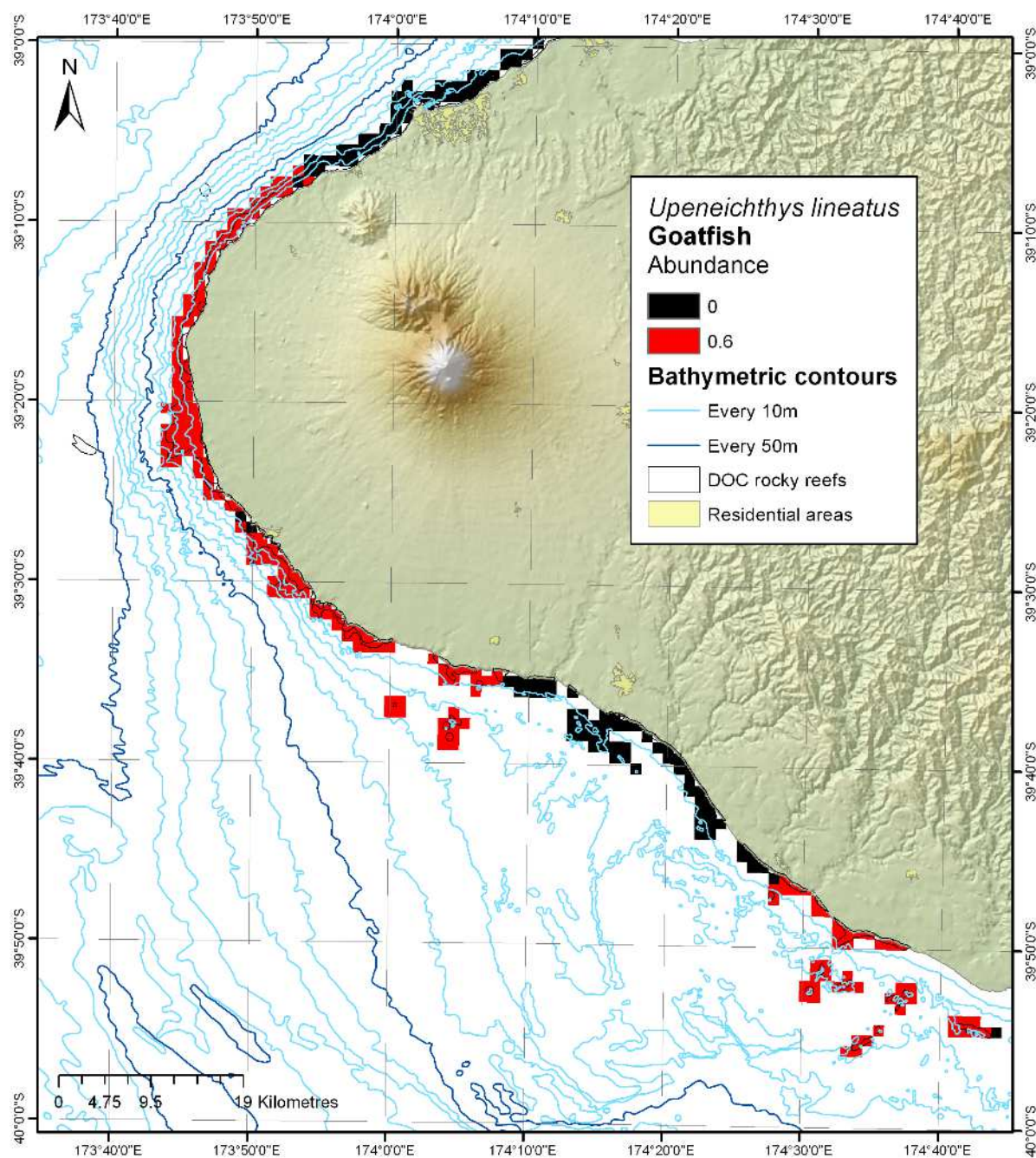
Figure 10-6: Modelled distribution and abundance of goatfish on Taranaki subtidal reefs.
