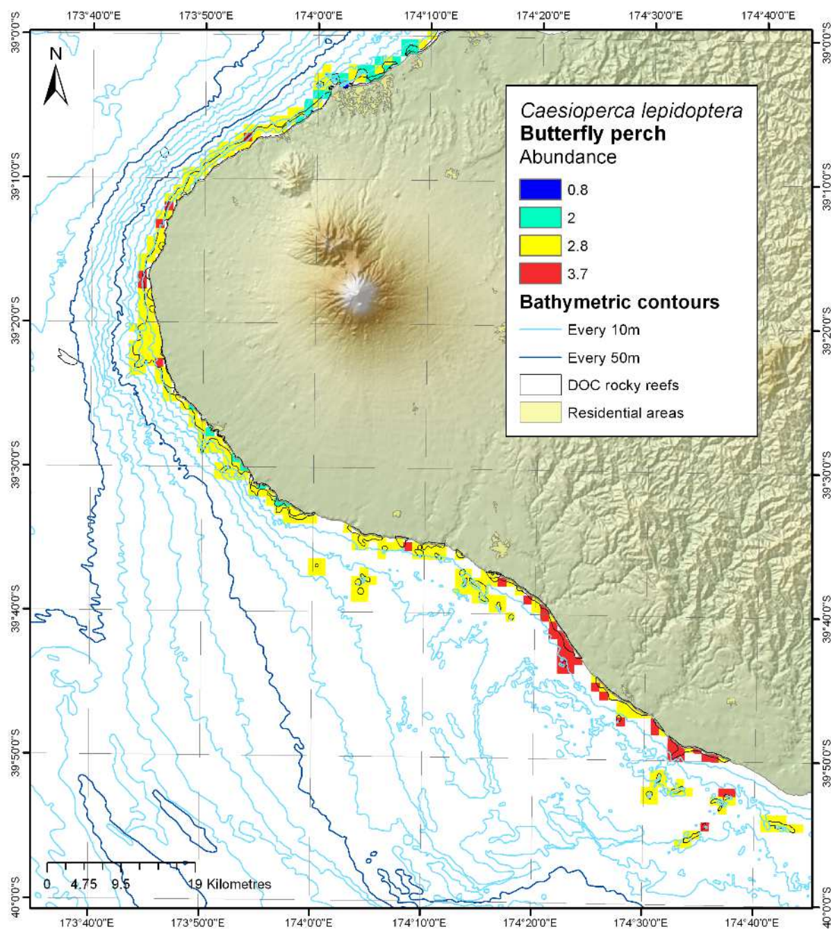
Figure 10-37: Modelled distribution and abundance of butterfly perch on Taranaki subtidal reefs.
