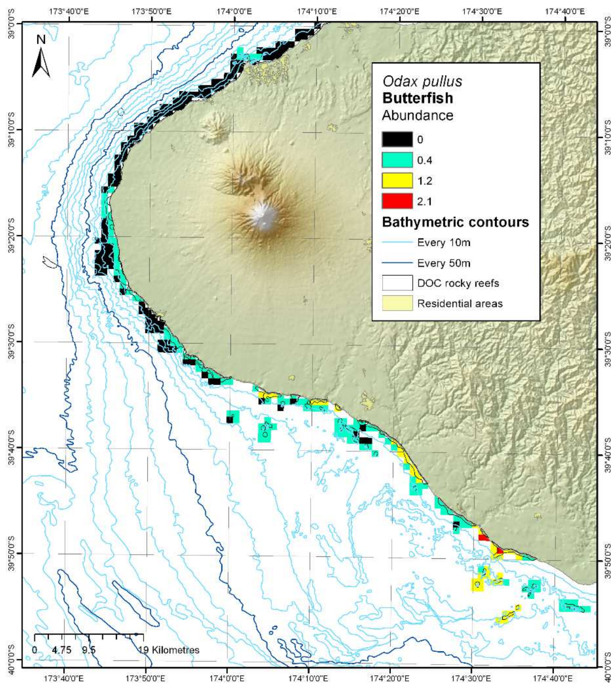
Figure 10-27: Modelled distribution and abundance of butterfish on Taranaki subtidal reefs.
