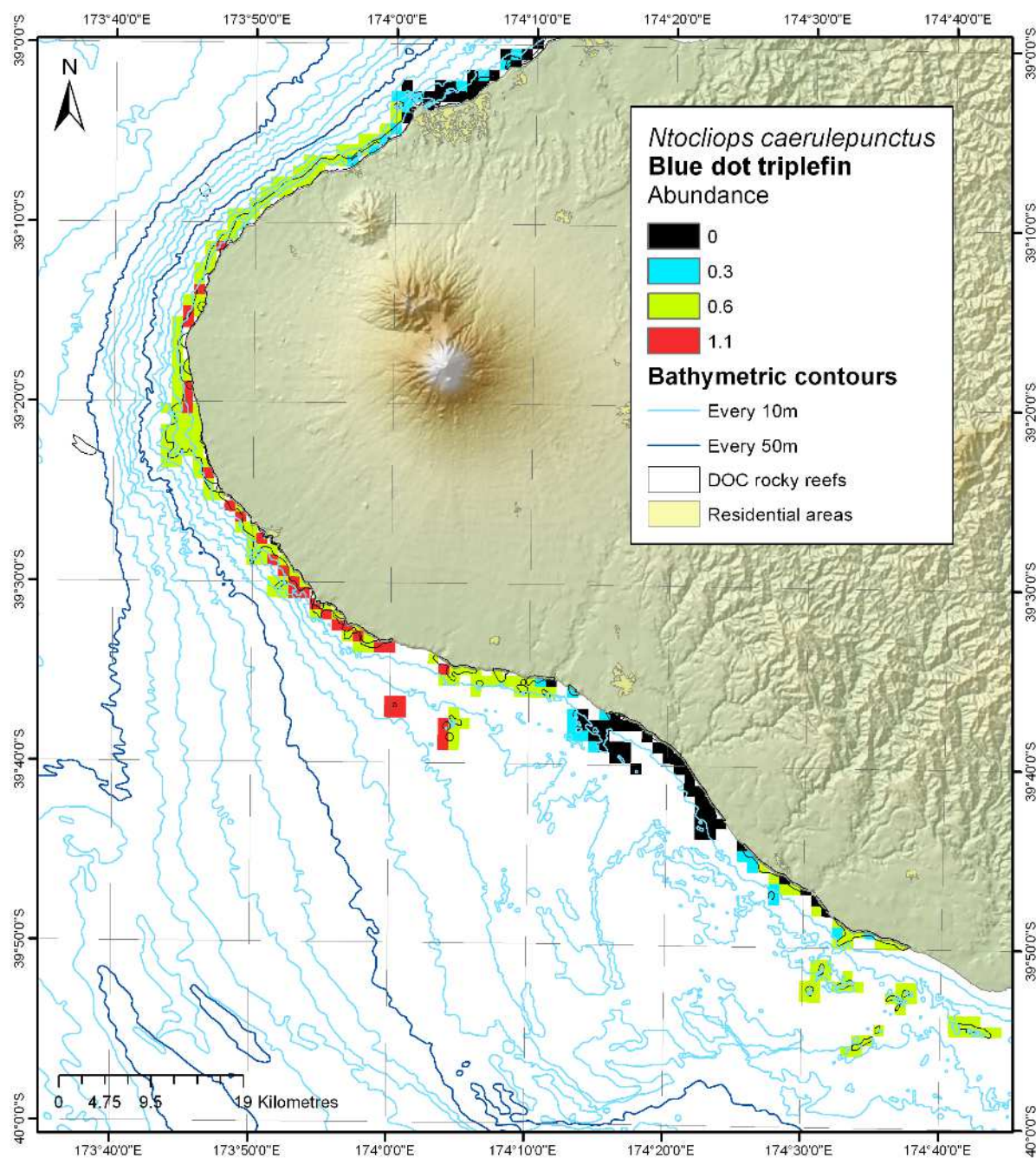
Figure 10-13: Modelled distribution and abundance of blue dot triplefin on Taranaki subtidal reefs.
