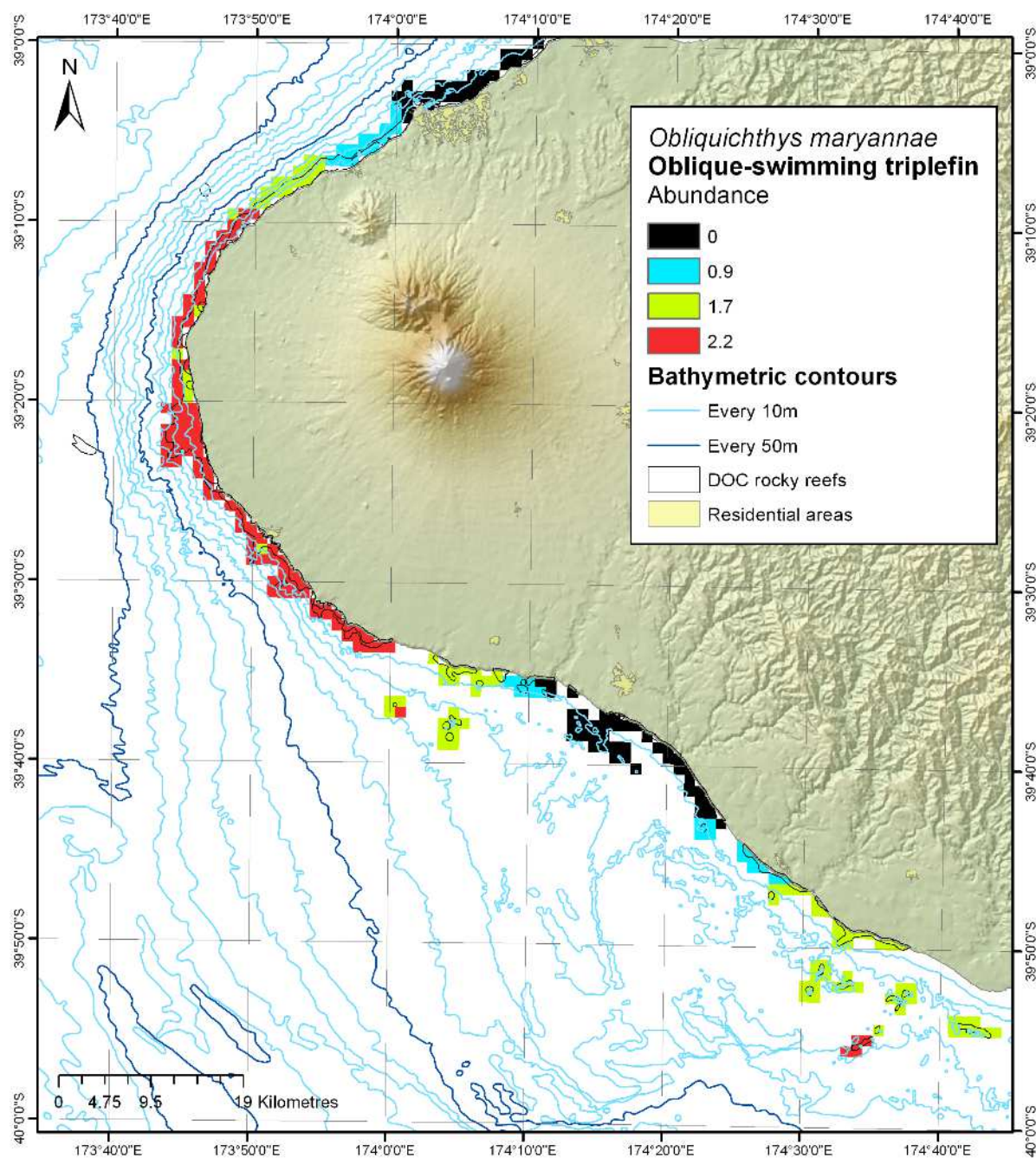
Figure 10-28: Modelled distribution and abundance of oblique-swimming triplefin on Taranaki subtidal reefs.
