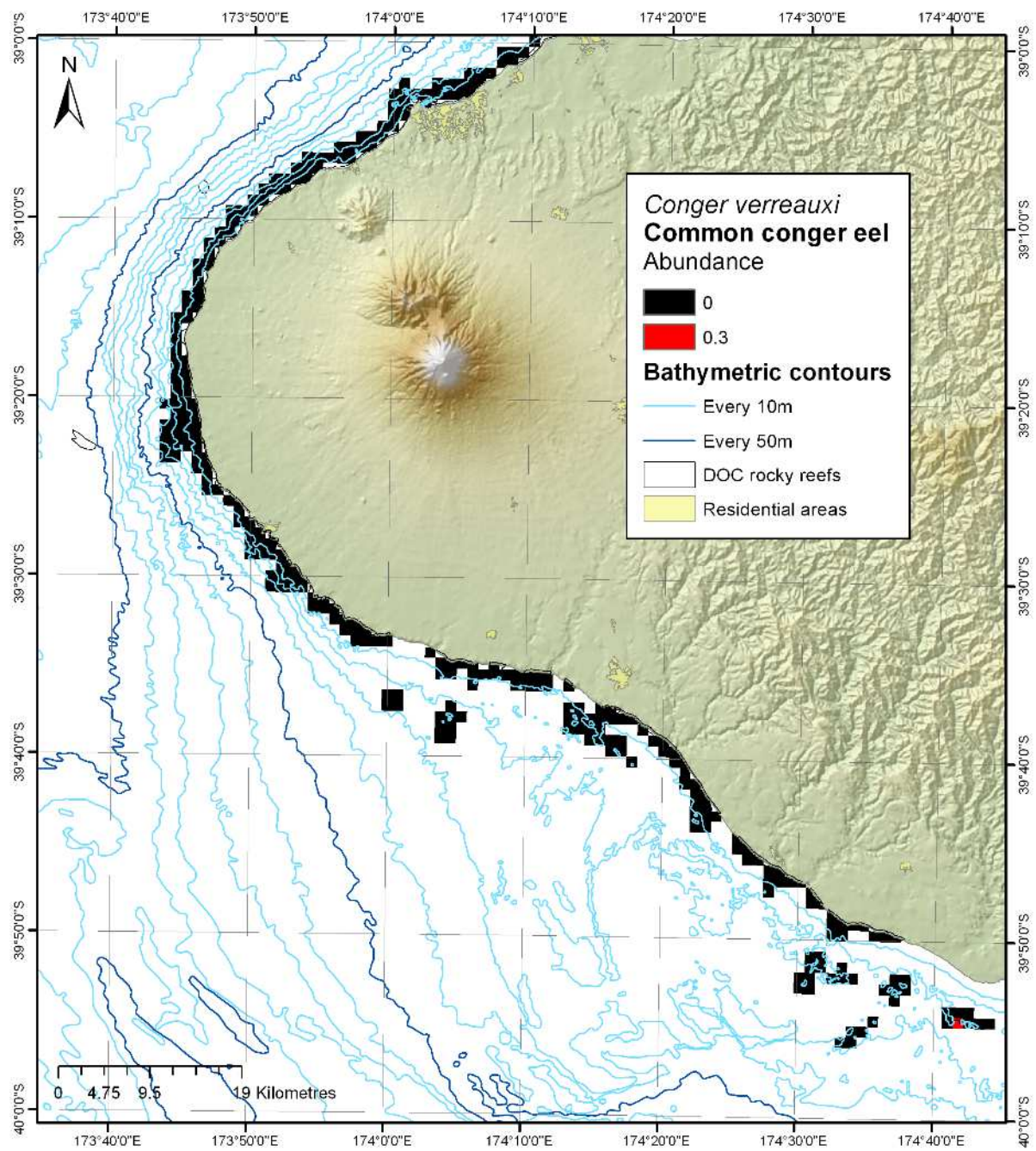
Figure 10-2: Modelled distribution and abundance of conger eel on Taranaki subtidal reefs.
