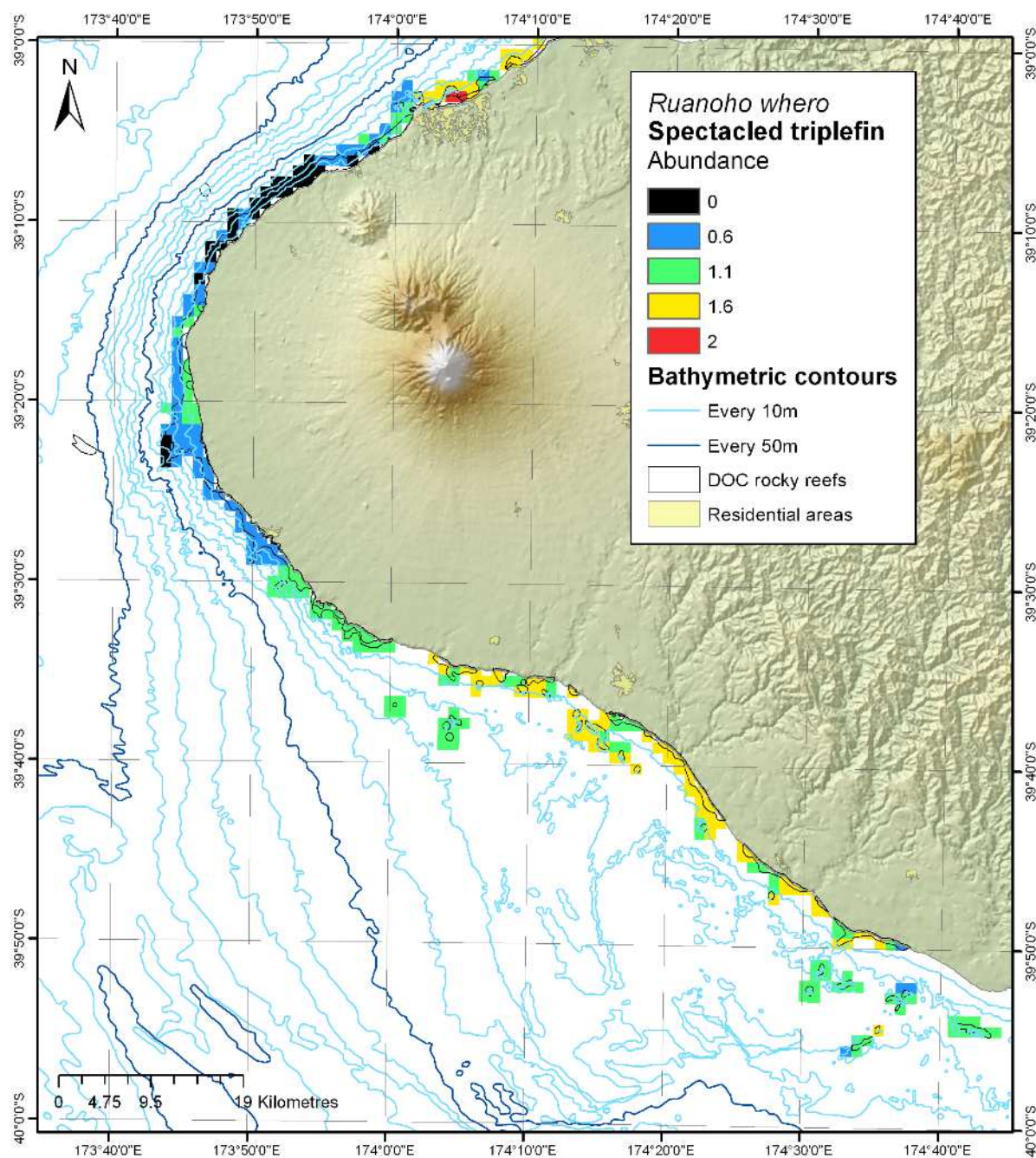
Figure 10-23: Modelled distribution and abundance of spectacled triplefin on Taranaki subtidal reefs.
