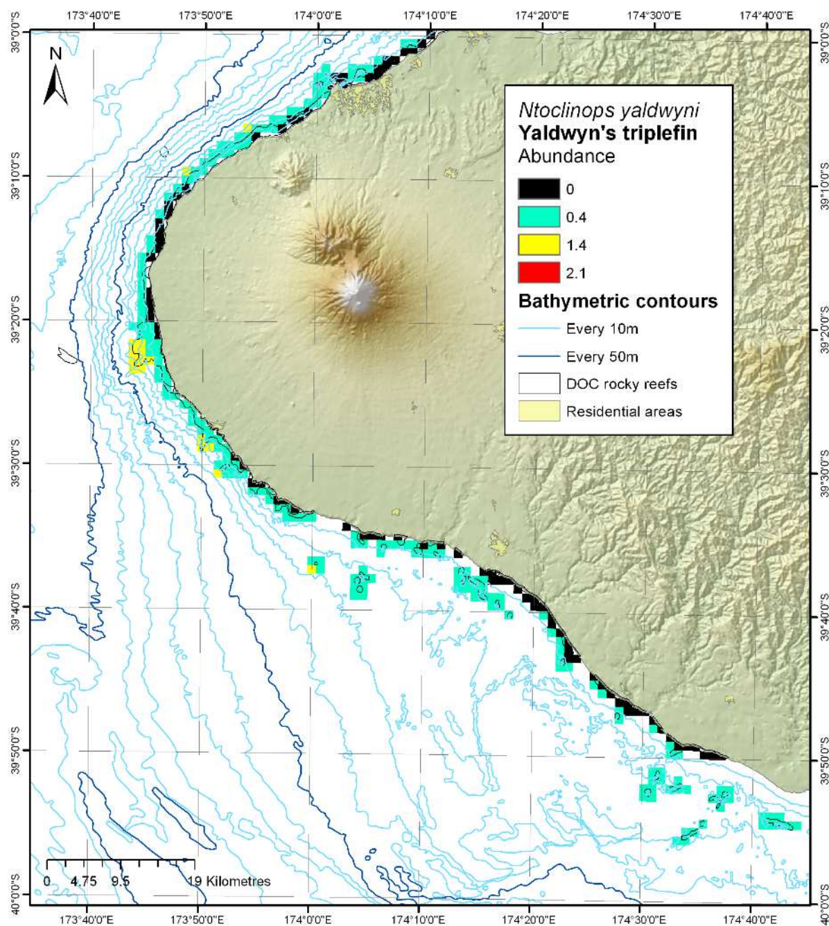
Figure 10-25: Modelled distribution and abundance of Yaldwyn's triplefin on Taranaki subtidal reefs.
