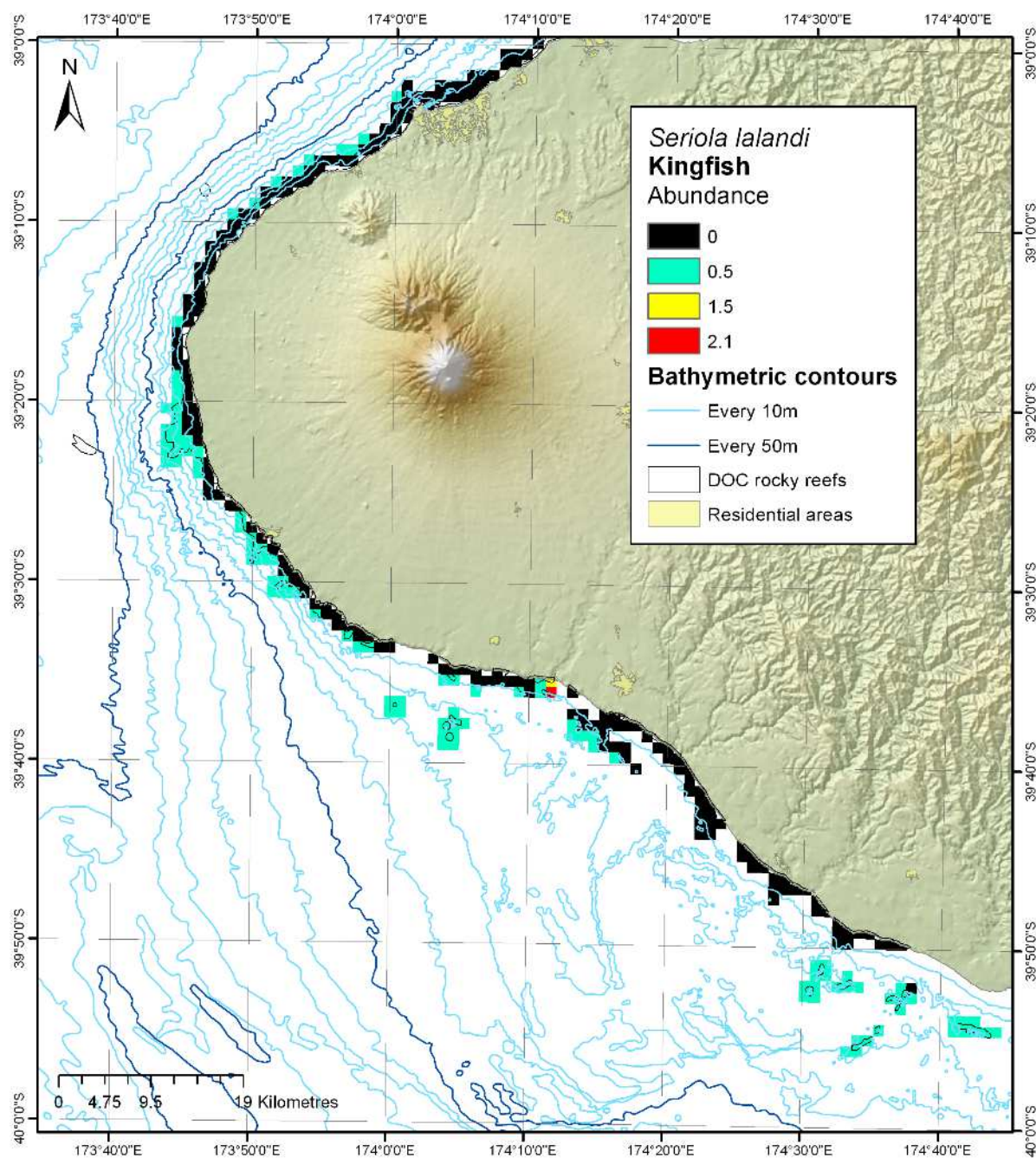
Figure 10-24: Modelled distribution and abundance of kingfish on Taranaki subtidal reefs.
