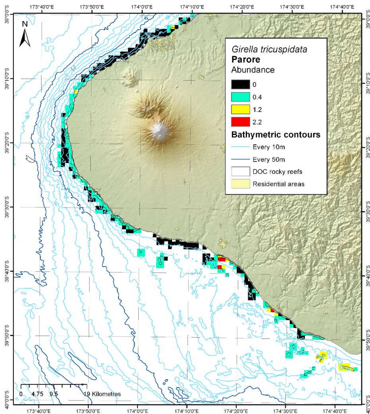
Figure 10-29: Modelled distribution and abundance of parore on Taranaki subtidal reefs.
