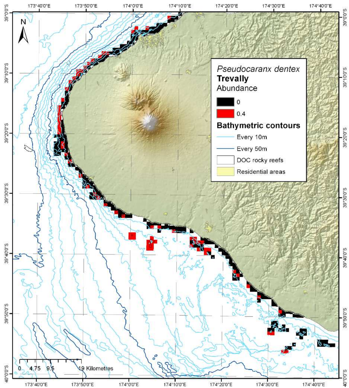
Figure 10-3: Modelled distribution and abundance of trevally on Taranaki subtidal reefs.
