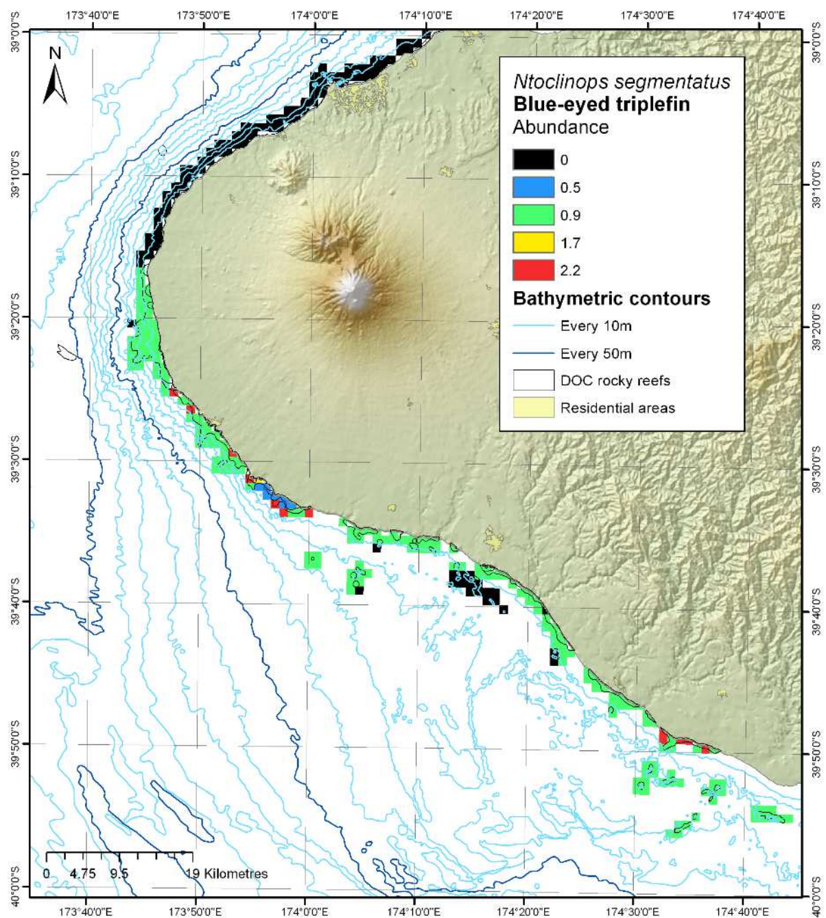
Figure 10-30: Modelled distribution and abundance of blue-eyed triplefin on Taranaki subtidal reefs.
