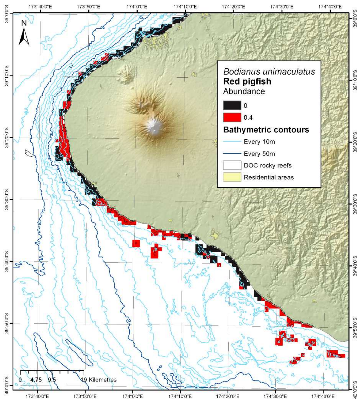
Figure 10-5: Modelled distribution and abundance of red pigfish on Taranaki subtidal reefs.
