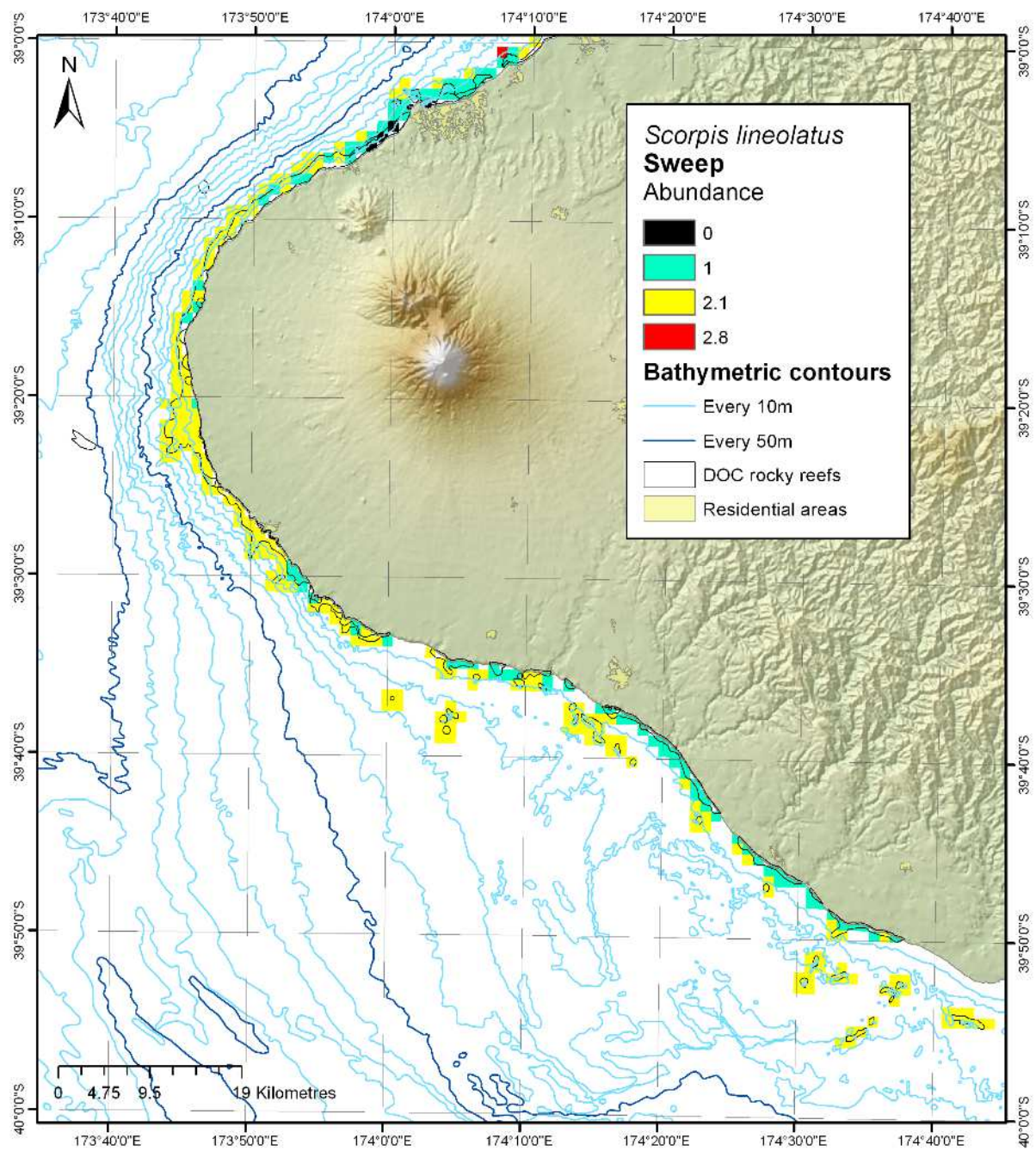
Figure 10-34: Modelled distribution and abundance of sweep on Taranaki subtidal reefs.
