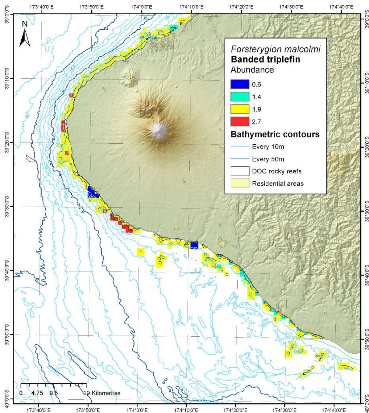
Figure 10-33: Modelled distribution and abundance of banded triplefin on Taranaki subtidal reefs.
