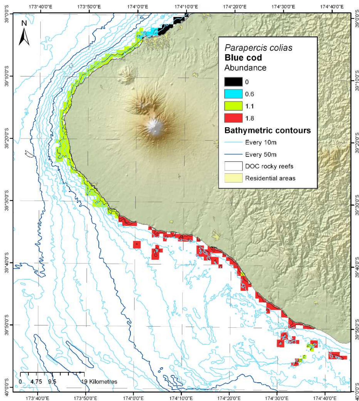
Figure 10-17: Modelled distribution and abundance of blue cod on Taranaki subtidal reefs.
