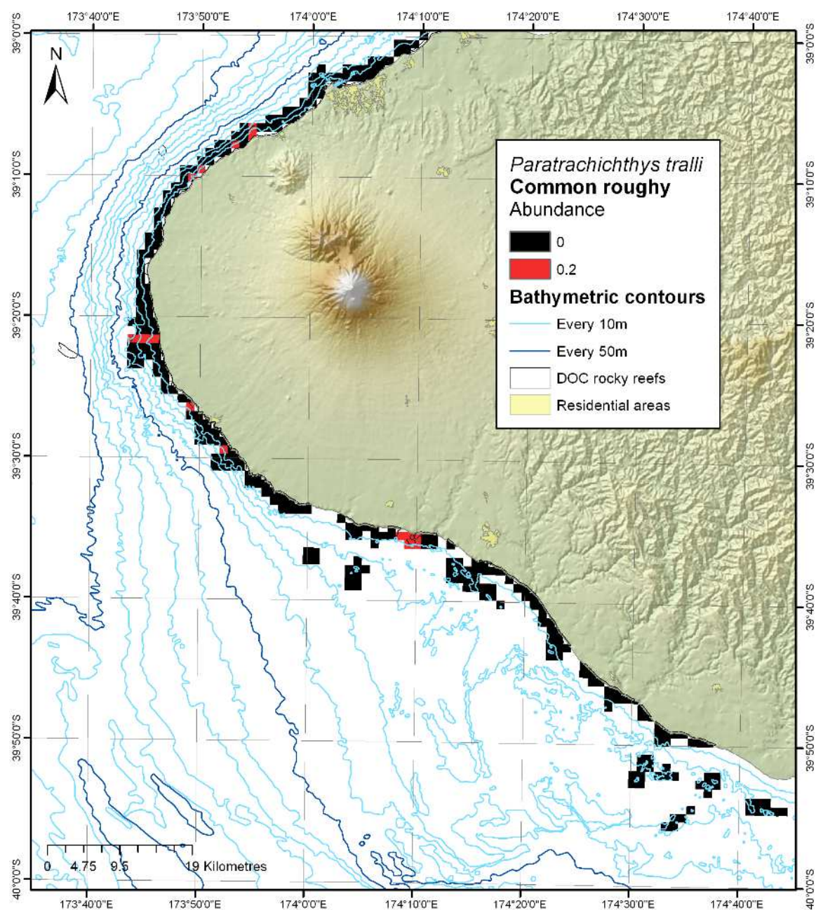
Figure 10-1: Modelled distribution and abundance of common roughy on Taranaki subtidal reefs.
