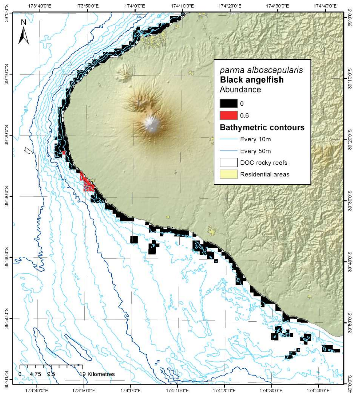
Figure 10-7: Modelled distribution and abundance of black angelfish on Taranaki subtidal reefs.
