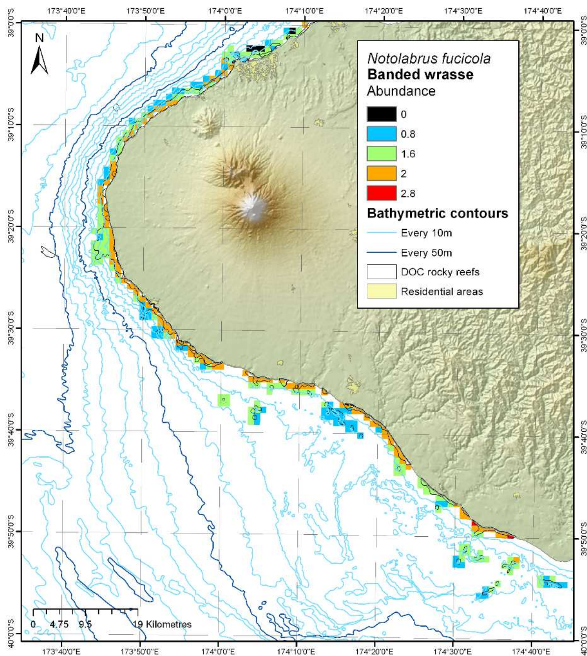
Figure 10-35: Modelled distribution and abundance of banded wrasse on Taranaki subtidal reefs.
