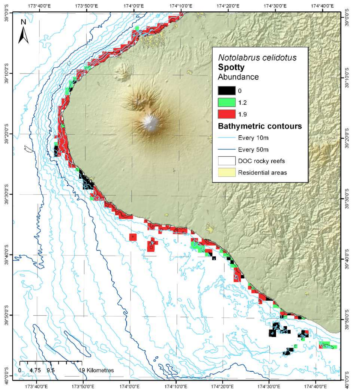
Figure 10-19: Modelled distribution and abundance of spotty on Taranaki subtidal reefs.
