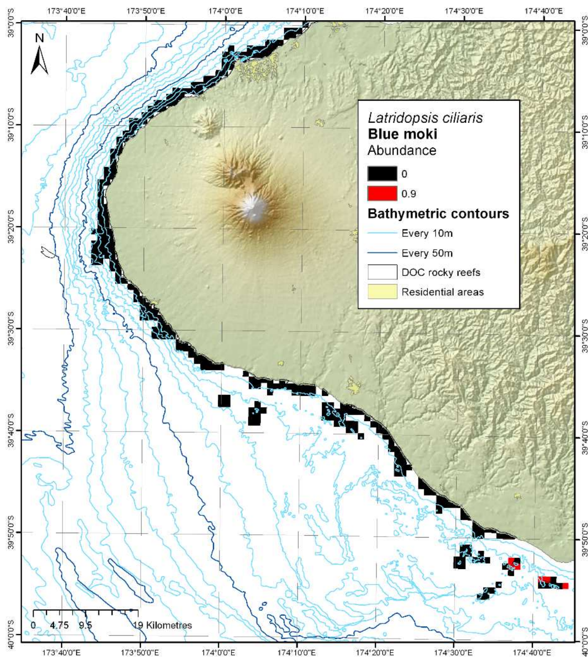
Figure 10-11: Modelled distribution and abundance of blue moki on Taranaki subtidal reefs.
