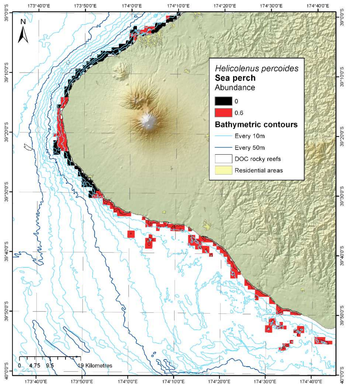
Figure 10-8: Modelled distribution and abundance of sea perch on Taranaki subtidal reefs.
