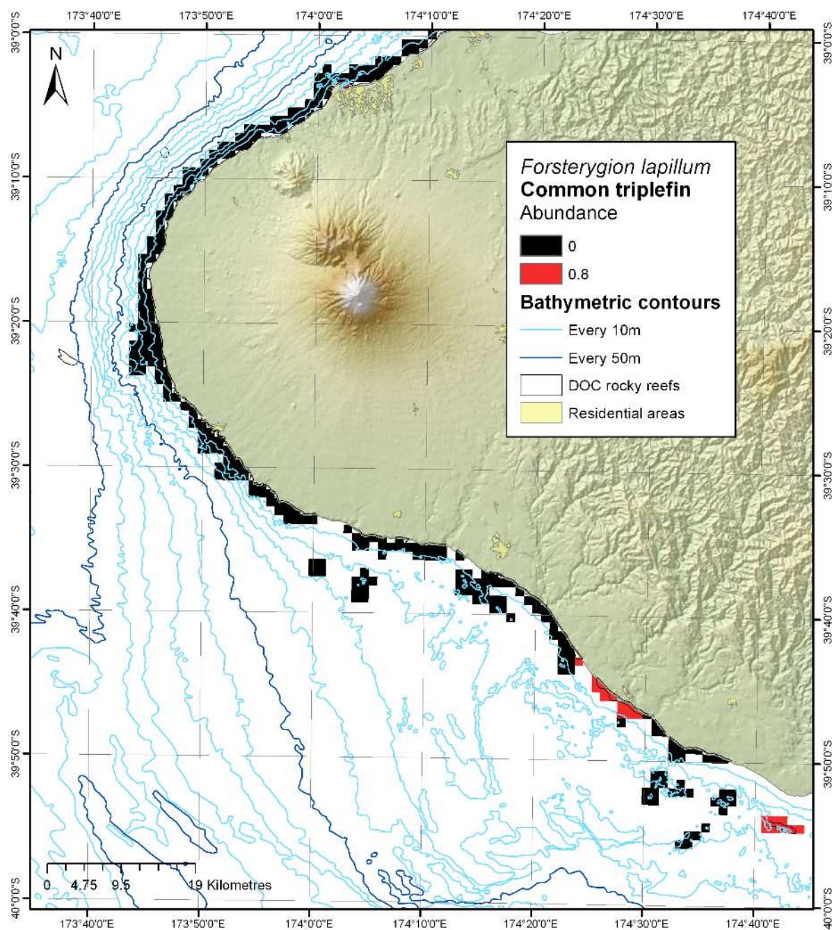
Figure 10-10: Modelled distribution and abundance of common triplefin on Taranaki subtidal reefs.
