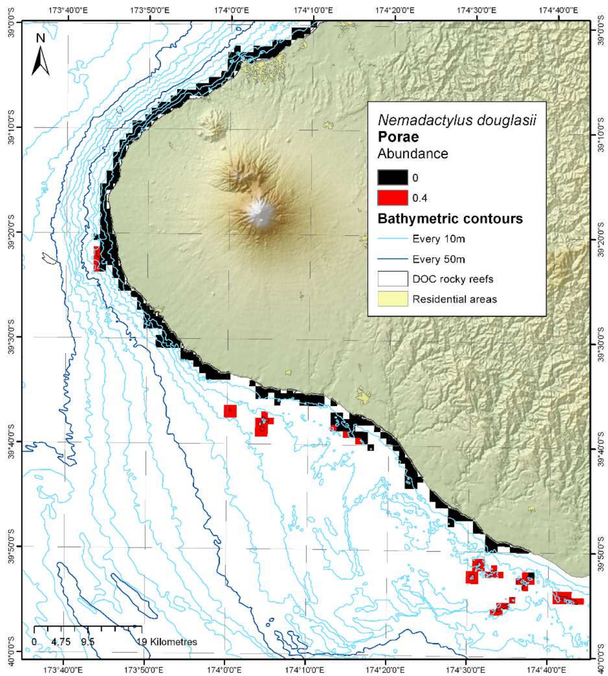
Figure 10-4: Modelled distribution and abundance of porae on Taranaki subtidal reefs.
