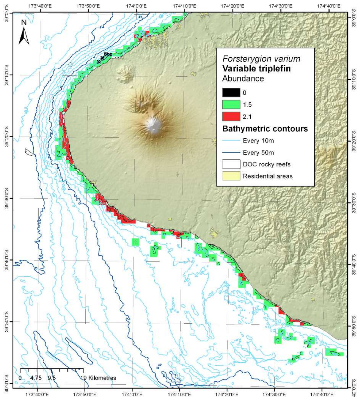
Figure 10-26: Modelled distribution and abundance of variable triplefin on Taranaki subtidal reefs.
