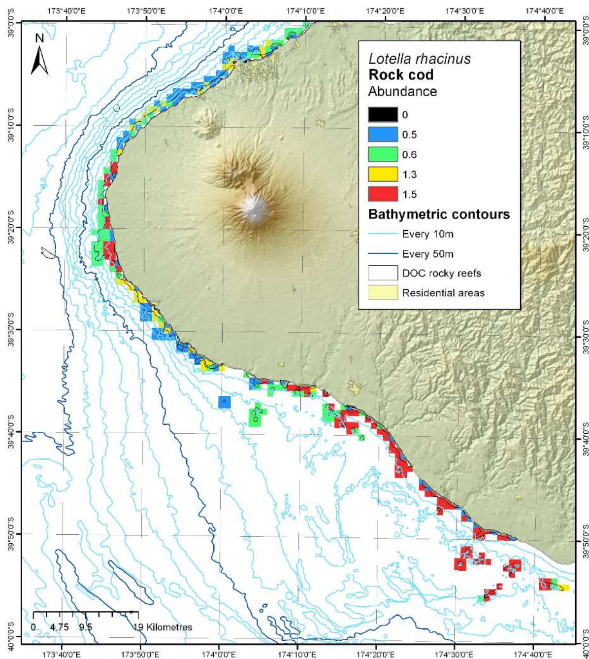
Figure 10-15: Modelled distribution and abundance of rock cod on Taranaki subtidal reefs.
