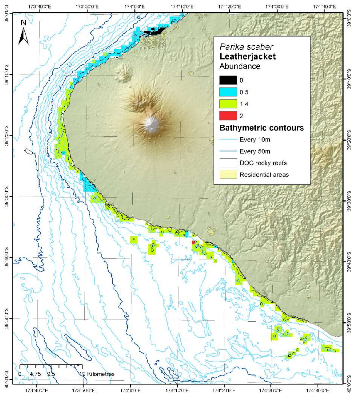
Figure 10-22: Modelled distribution and abundance of leatherjacket on Taranaki subtidal reefs.
