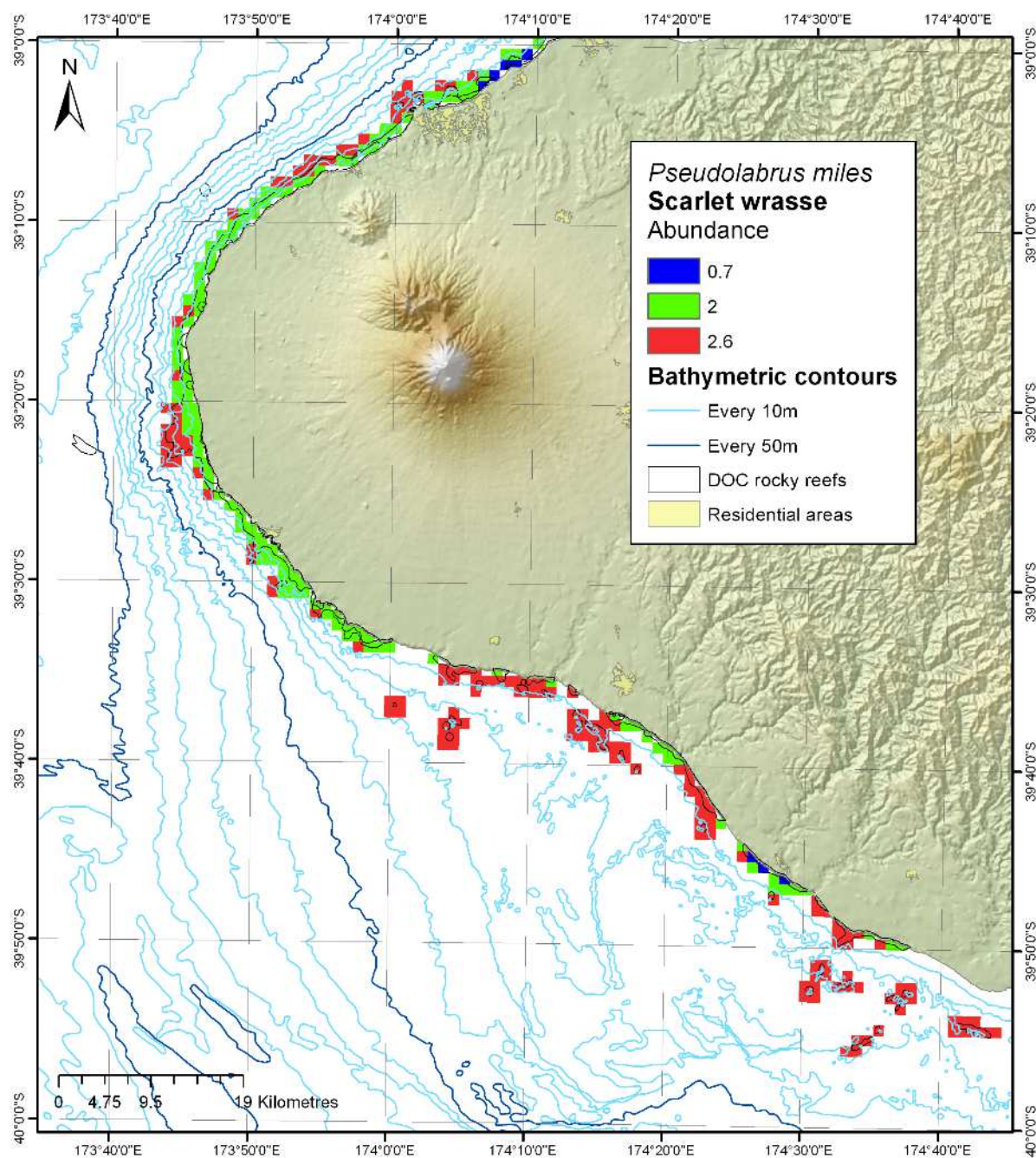
Figure 10-32: Modelled distribution and abundance of scarlet wrasse on Taranaki subtidal reefs.
