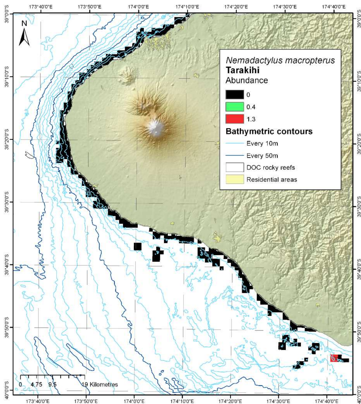
Figure 10-14: Modelled distribution and abundance of tarakihi on Taranaki subtidal reefs.
