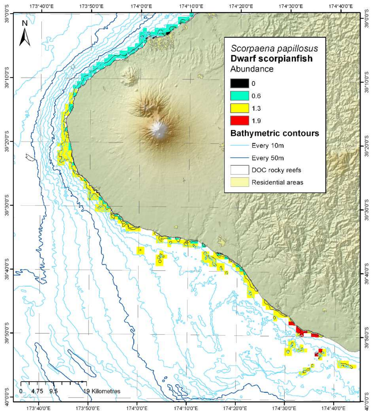
Figure 10-20: Modelled distribution and abundance of dwarf scorpionfish on Taranaki subtidal reefs.
