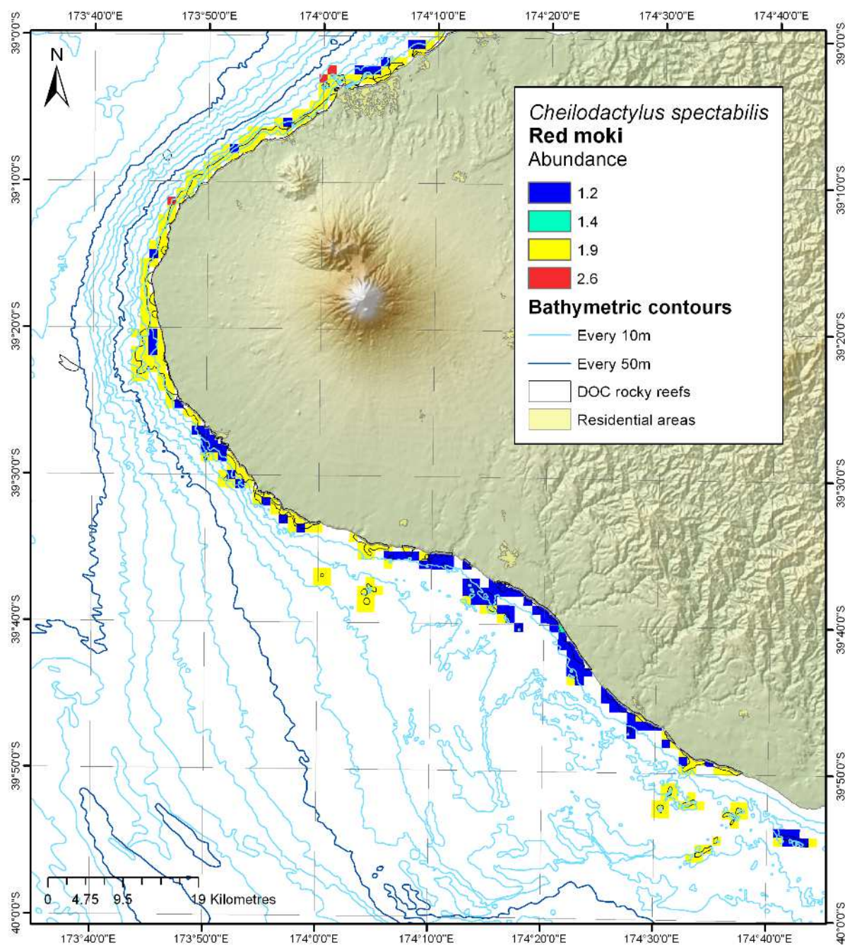
Figure 10-31: Modelled distribution and abundance of red moki on Taranaki subtidal reefs.
