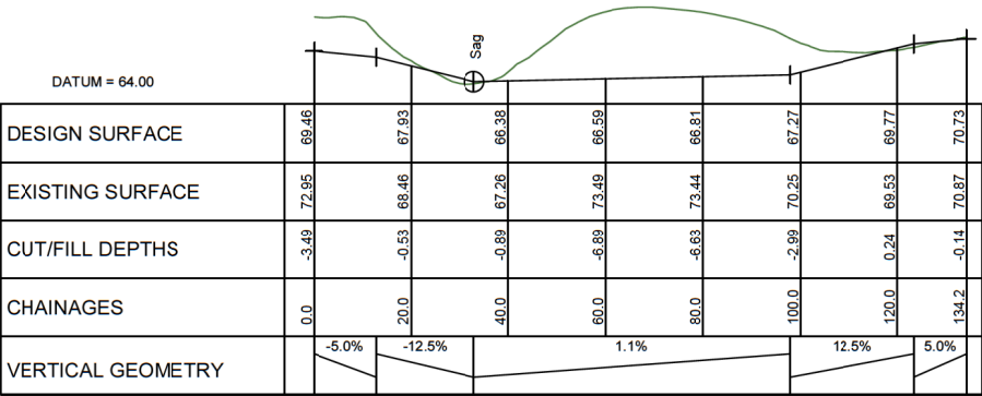
LONGITUDINAL SECTION JOAL 36 SCALE HORIZ=1:1200 @ A1 VERT=1:600 @ A1
