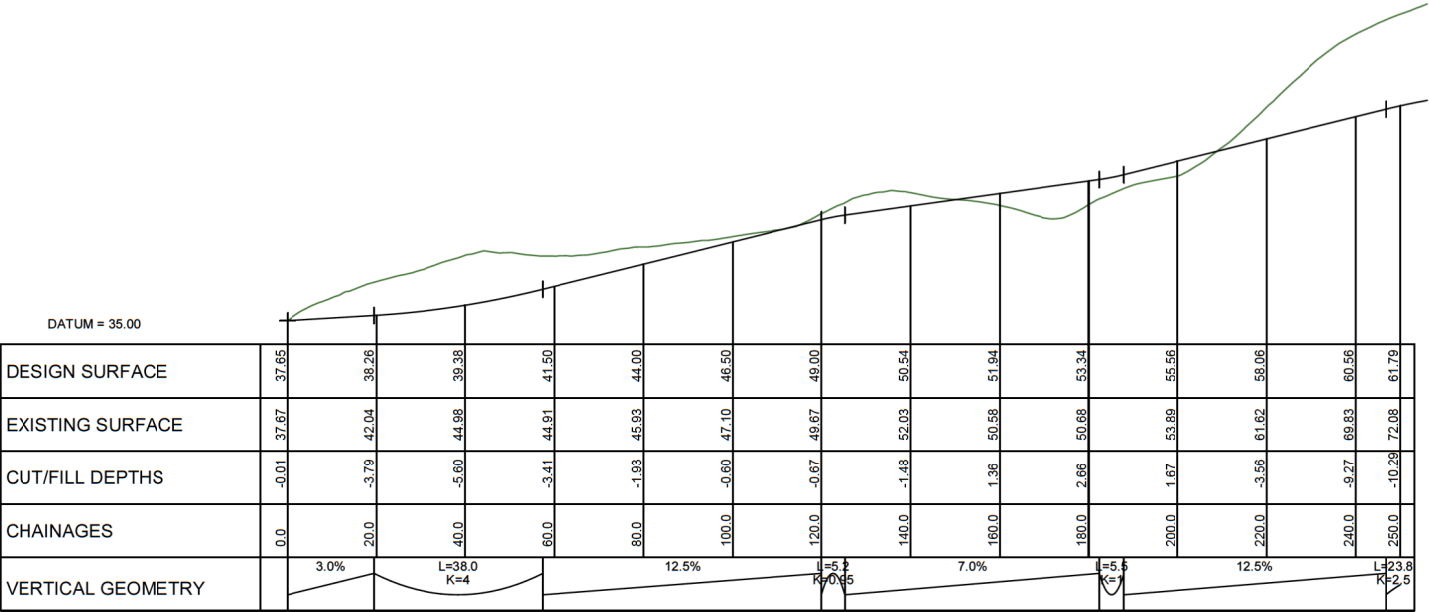
LONGITUDINAL SECTION ROAD 18 SCALE HORIZ=1:1200 @ A1 VERT=1:600 @ A1
