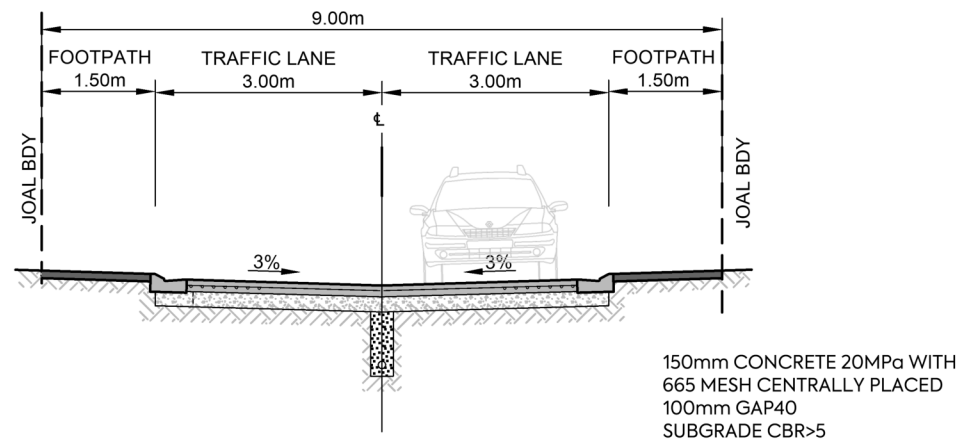
JOAL 5B, 40, 40A M2 300 9.0m JOAL, 6.0m FORMED WIDTH SCALE 1:100 @A3
