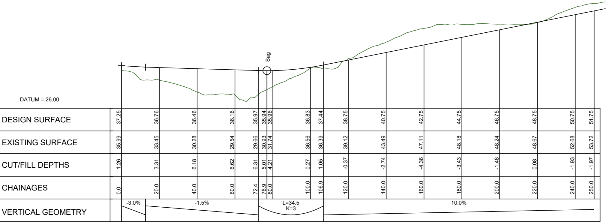
LONGITUDINAL SECTION ROAD 14 SCALE HORIZ=1:1200 @ A1 VERT=1:600 @ A1
