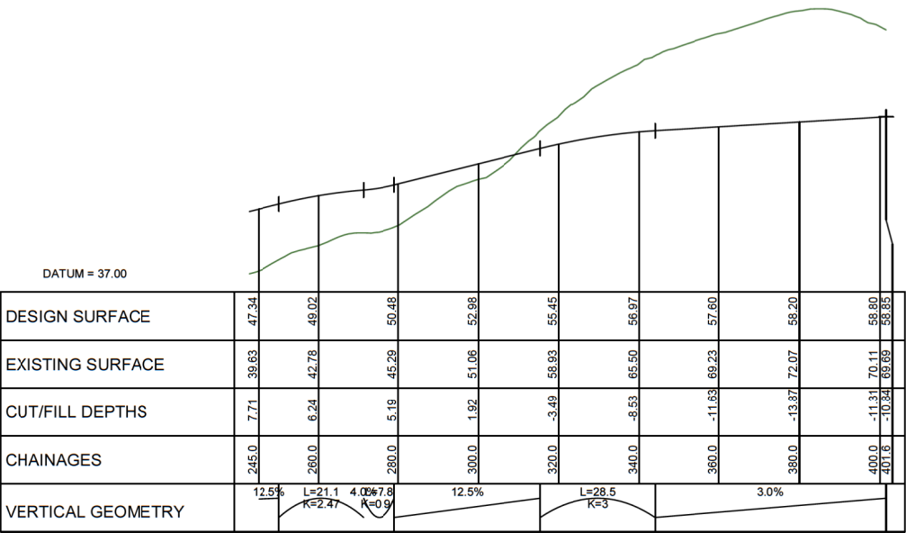
LONGITUDINAL SECTION ROAD 22 SCALE HORIZ=1:1200 @ A1 VERT=1:600 @ A1
