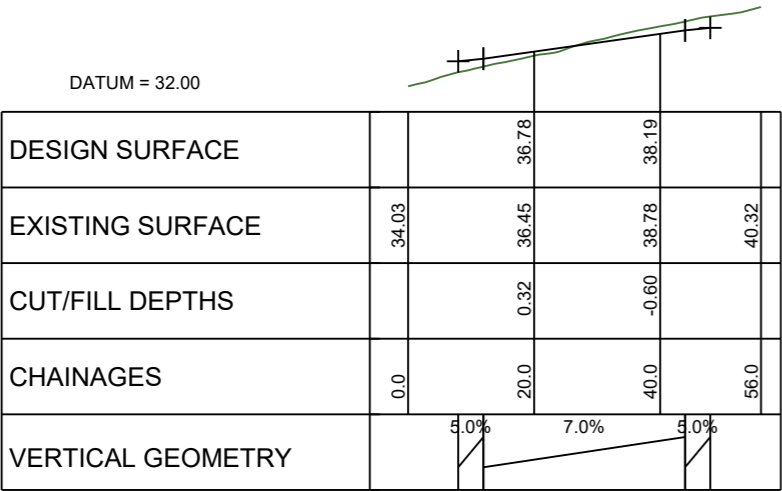
LONGITUDINAL SECTION JOAL 14 SCALE HORIZ=1:1200 @ A1 VERT=1:600 @ A1
