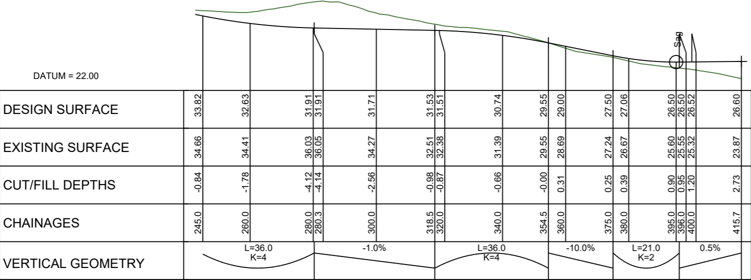
LONGITUDINAL SECTION ROAD 12 SCALE HORIZ=1:1200 @ A1 VERT=1:600 @ A1
