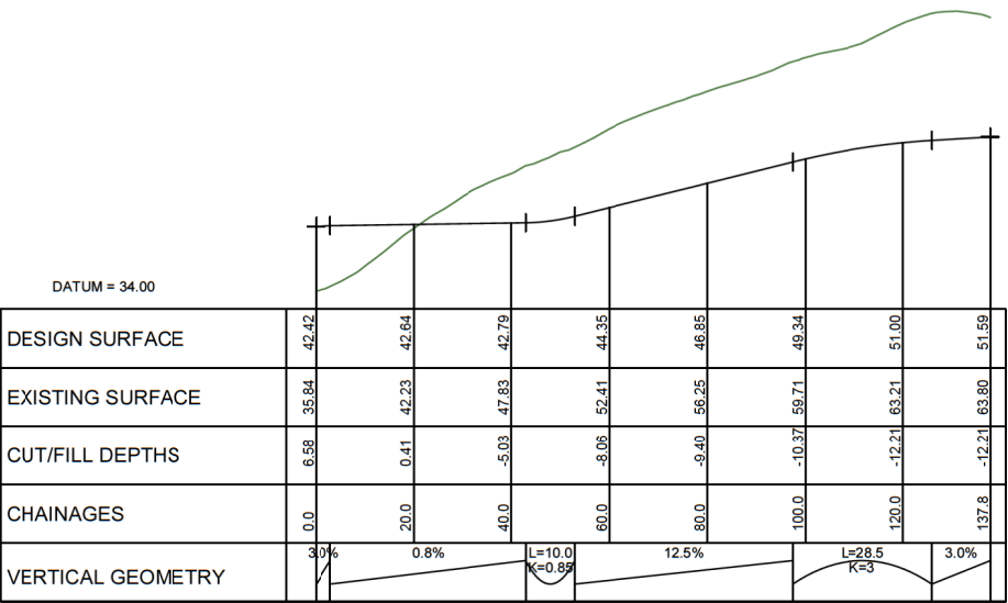
LONGITUDINAL SECTION ROAD 27 SCALE HORIZ=1:1200 @ A1 VERT=1:600 @ A1
