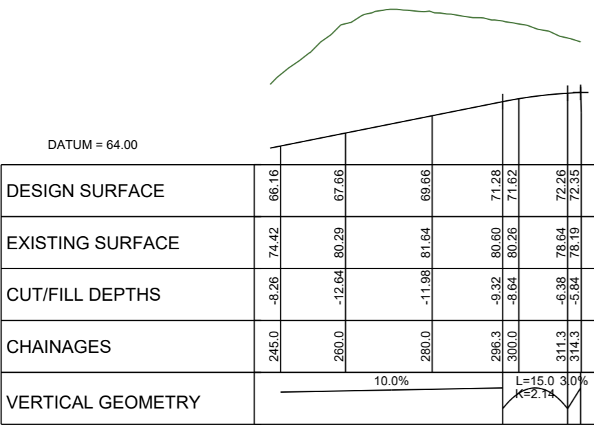
LONGITUDINAL SECTION ROAD 13 SCALE HORIZ=1:1200 @ A1 VERT=1:600 @ A1
