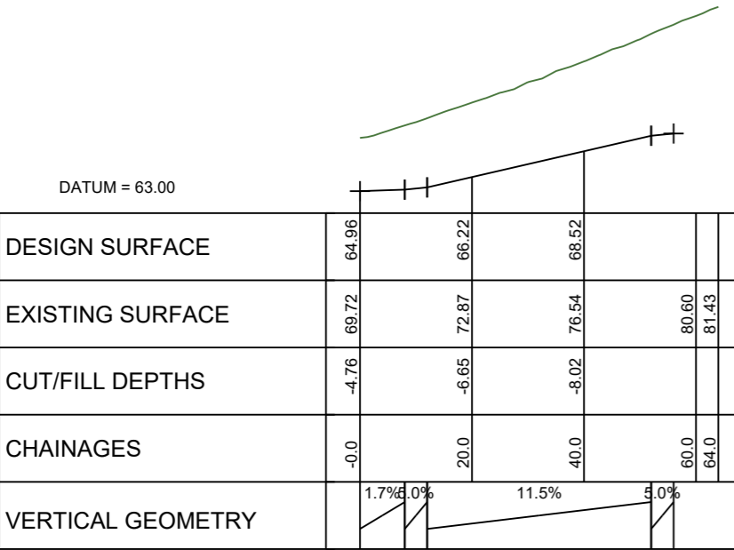
LONGITUDINAL SECTION JOAL 18 SCALE HORIZ=1:1200 @ A1 VERT=1:600 @ A1
