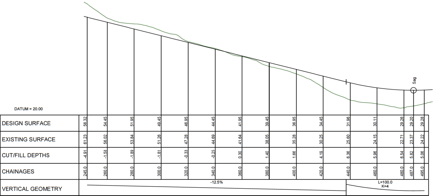
LONGITUDINAL SECTION ROAD 17 SCALE HORIZ=1:1200 @ A1 VERT=1:600 @ A1
