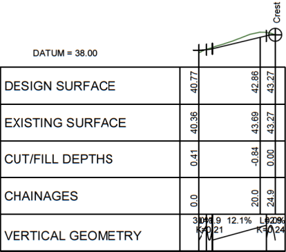
LONGITUDINAL SECTION ROAD 28 SCALE HORIZ=1:1200 @ A1 VERT=1:600 @ A1
