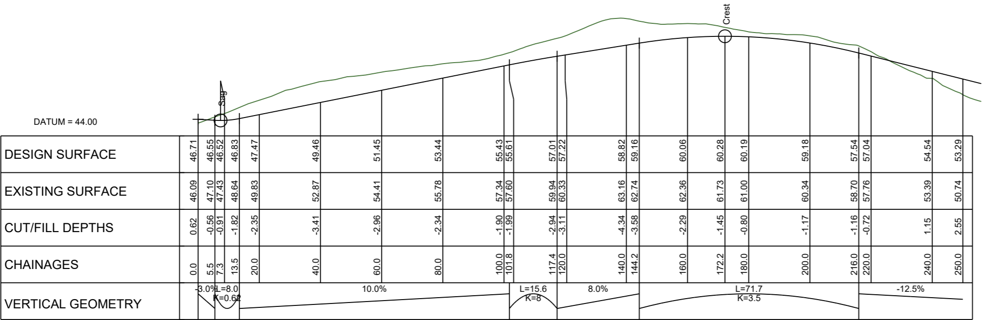
LONGITUDINAL SECTION ROAD 05 SCALE HORIZ=1:1200 @ A1 VERT=1:600 @ A1
