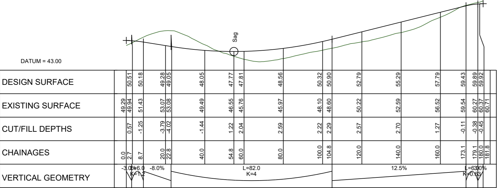
LONGITUDINAL SECTION ROAD 15 SCALE HORIZ=1:1200 @ A1 VERT=1:600 @ A1
