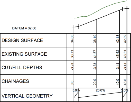
LONGITUDINAL SECTION JOAL 41 SCALE HORIZ=1:1200 @ A1 VERT=1:600 @ A1
