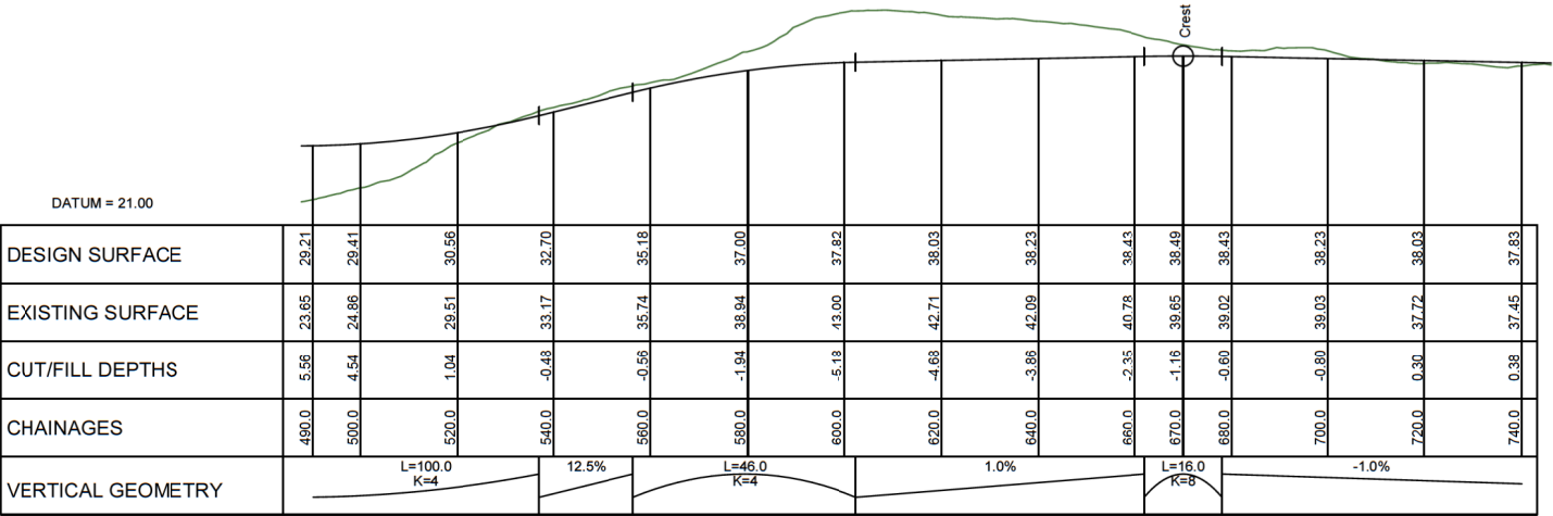
LONGITUDINAL SECTION ROAD 17 SCALE HORIZ=1:1200 @ A1 VERT=1:600 @ A1
