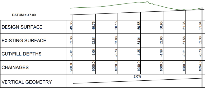
LONGITUDINAL SECTION ROAD 17 SCALE HORIZ=1:1200 @ A1 VERT=1:600 @ A1
