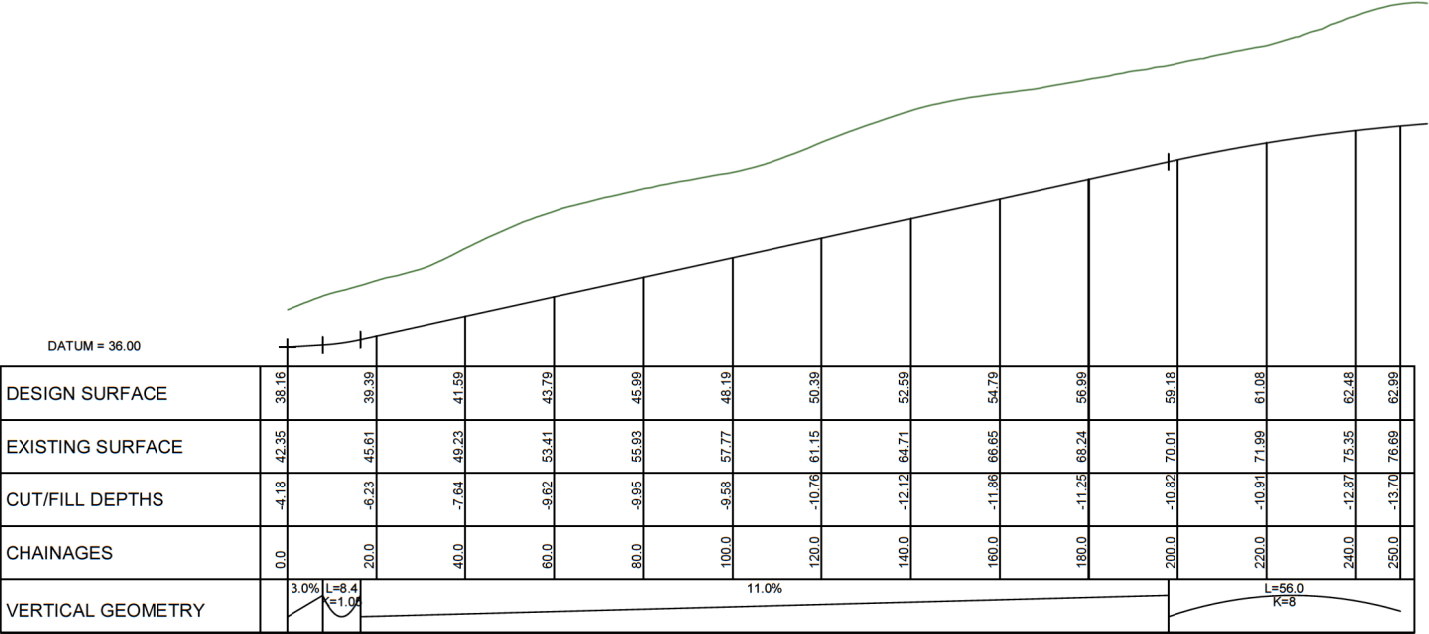
LONGITUDINAL SECTION ROAD 21 SCALE HORIZ=1:1200 @ A1 VERT=1:600 @ A1
