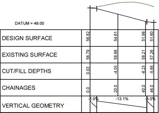
LONGITUDINAL SECTION JOAL 32 SCALE HORIZ=1:1200 @ A1 VERT=1:600 @ A1
