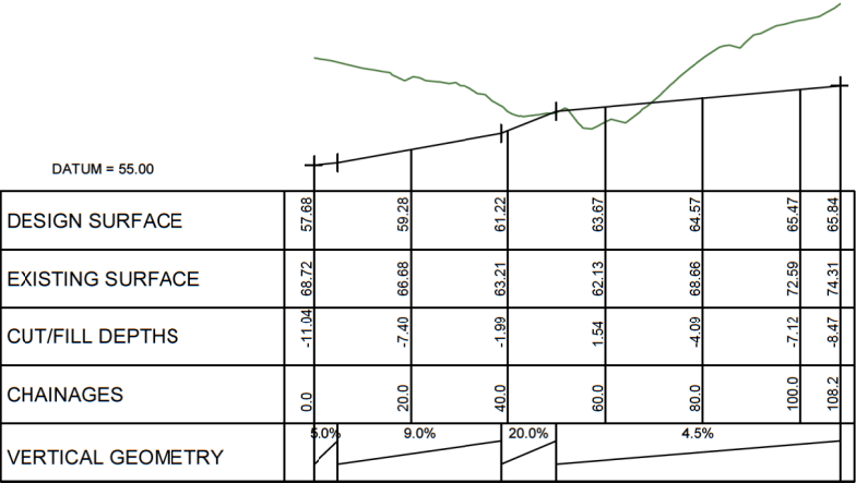
LONGITUDINAL SECTION JOAL 35 SCALE HORIZ=1:1200 @ A1 VERT=1:600 @ A1
