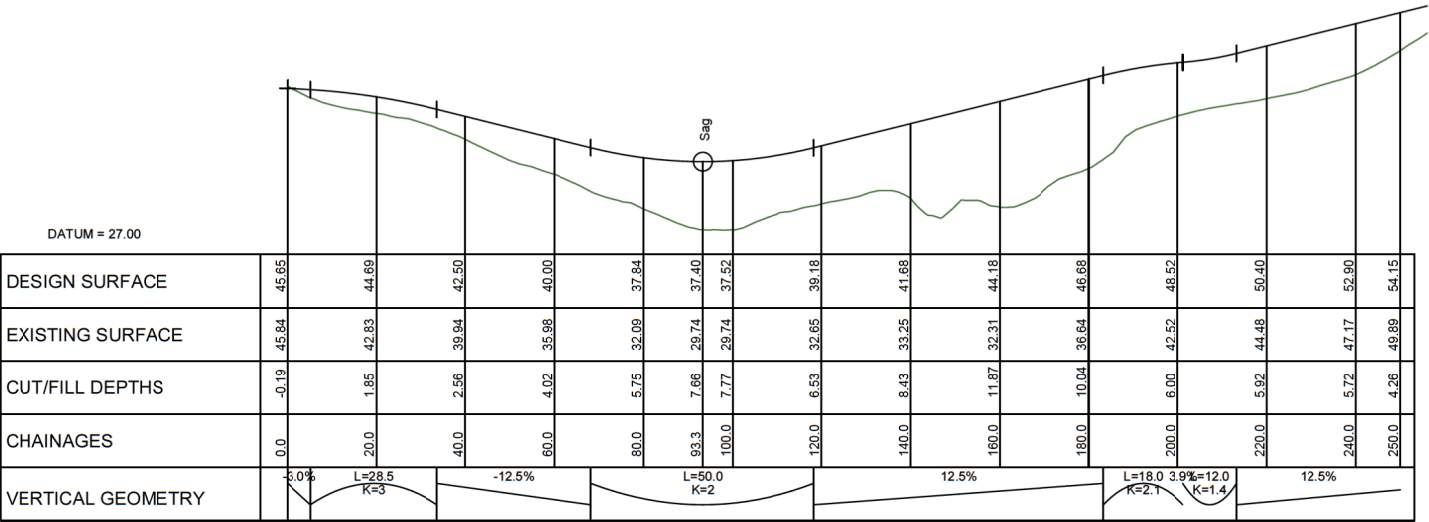
LONGITUDINAL SECTION ROAD 24 SCALE HORIZ=1:1200 @ A1 VERT=1:600 @ A1
