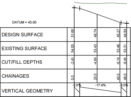
LONGITUDINAL SECTION JOAL 31 SCALE HORIZ=1:1200 @ A1 VERT=1:600 @ A1
