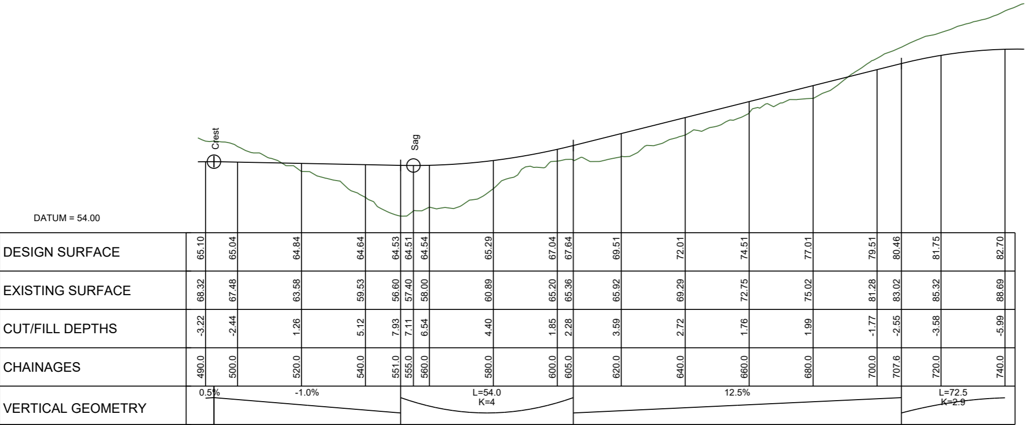
LONGITUDINAL SECTION ROAD 14 SCALE HORIZ=1:1200 @ A1 VERT=1:600 @ A1
