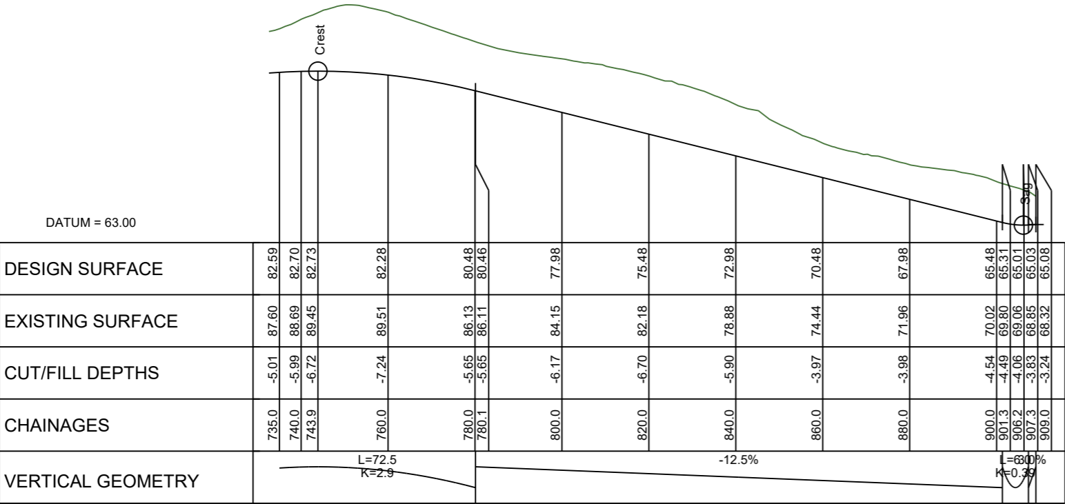
LONGITUDINAL SECTION ROAD 14 SCALE HORIZ=1:1200 @ A1 VERT=1:600 @ A1
