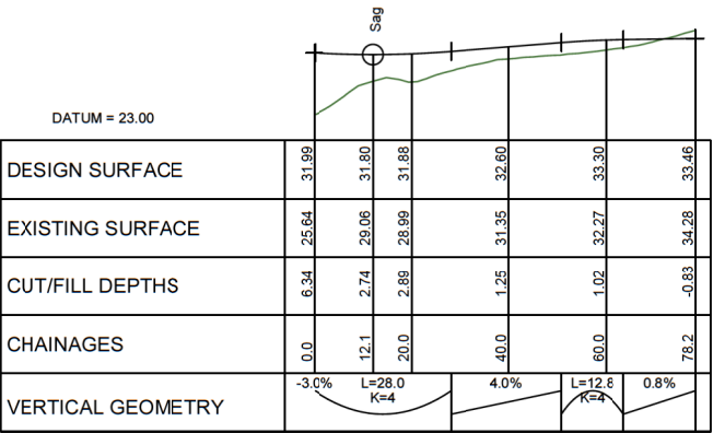
LONGITUDINAL SECTION ROAD 23 SCALE HORIZ=1:1200 @ A1 VERT=1:600 @ A1
