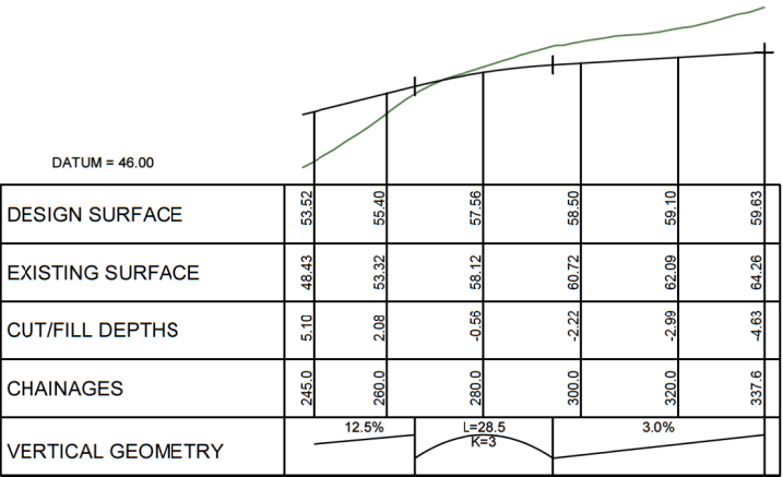
LONGITUDINAL SECTION ROAD 24 SCALE HORIZ=1:1200 @ A1 VERT=1:600 @ A1
