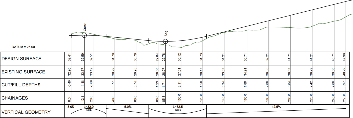
LONGITUDINAL SECTION ROAD 22 SCALE HORIZ=1:1200 @ A1 VERT=1:600 @ A1
