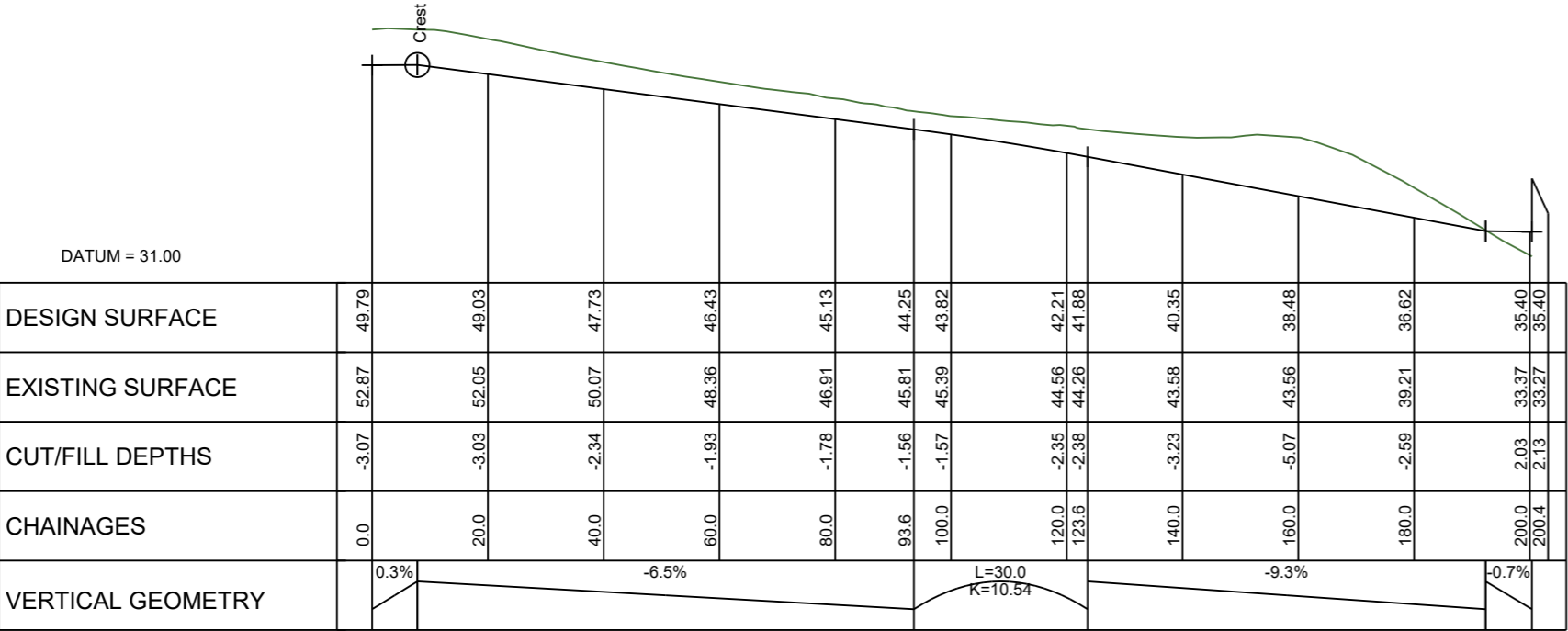
LONGITUDINAL SECTION JOAL 13 SCALE HORIZ=1:1200 @ A1 VERT=1:600 @ A1
