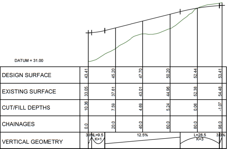
LONGITUDINAL SECTION ROAD 25 SCALE HORIZ=1:1200 @ A1 VERT=1:600 @ A1
