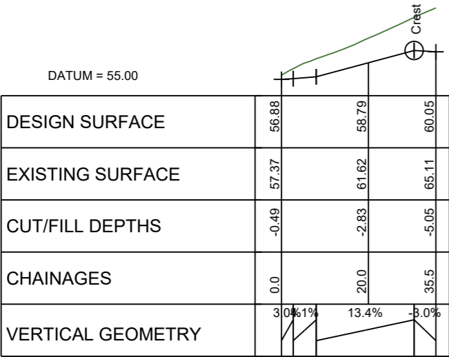
LONGITUDINAL SECTION JOAL 22B SCALE HORIZ=1:1200 @ A1 VERT=1:600 @ A1
