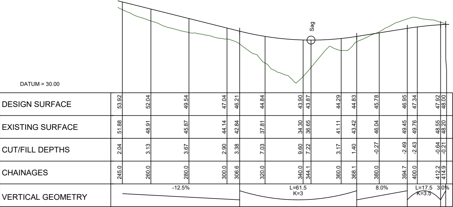
LONGITUDINAL SECTION ROAD 05 SCALE HORIZ=1:1200 @ A1 VERT=1:600 @ A1
