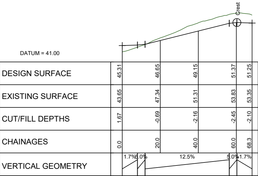
LONGITUDINAL SECTION JOAL 19 SCALE HORIZ=1:1200 @ A1 VERT=1:600 @ A1
