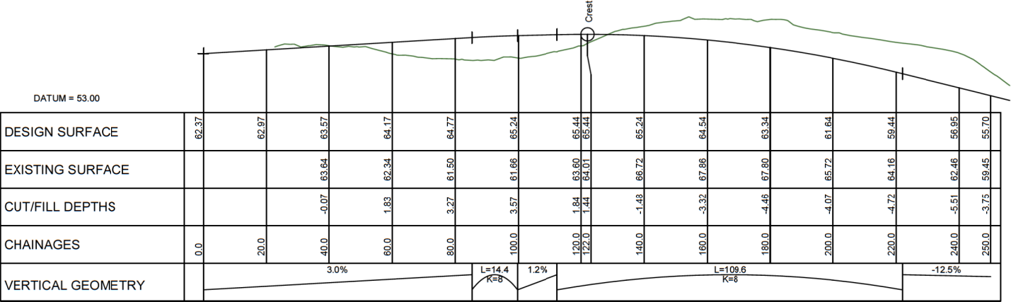
LONGITUDINAL SECTION ROAD 17 SCALE HORIZ=1:1200 @ A1 VERT=1:600 @ A1
