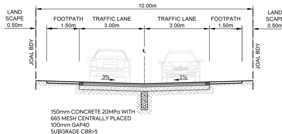
JOAL 3, 9, 21, 22 N2 300 10m JOAL SCALE 1:100 @A3
