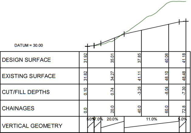
LONGITUDINAL SECTION JOAL 33 SCALE HORIZ=1:1200 @ A1 VERT=1:600 @ A1
