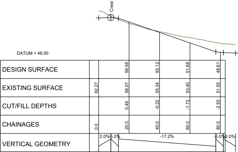
LONGITUDINAL SECTION JOAL 17 SCALE HORIZ=1:1200 @ A1 VERT=1:600 @ A1
