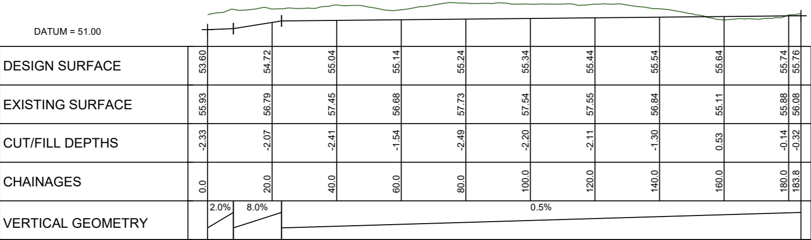
LONGITUDINAL SECTION JOAL 21 SCALE HORIZ=1:1200 @ A1 VERT=1:600 @ A1
