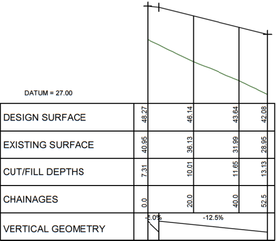
LONGITUDINAL SECTION JOAL 38 SCALE HORIZ=1:1200 @ A1 VERT=1:600 @ A1
