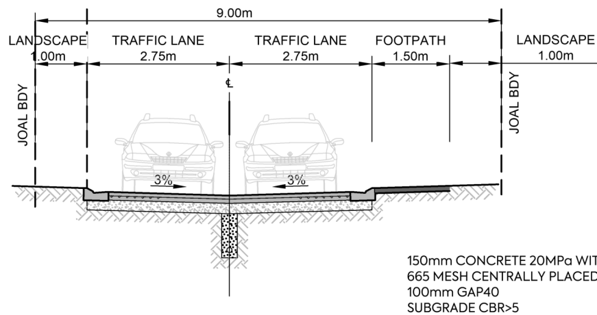
JOAL 35 M1 300 9.0m JOAL, 5.5m FORMED WIDTH SCALE 1:100 @A3
