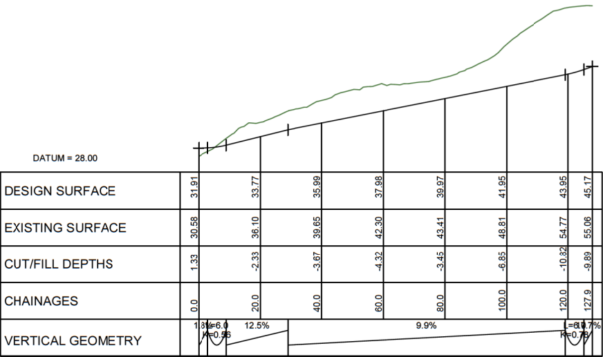
LONGITUDINAL SECTION ROAD 26 SCALE HORIZ=1:1200 @ A1 VERT=1:600 @ A1
