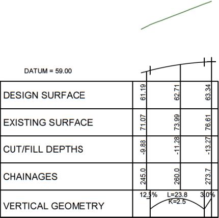
LONGITUDINAL SECTION ROAD 18 SCALE HORIZ=1:1200 @ A1 VERT=1:600 @ A1
