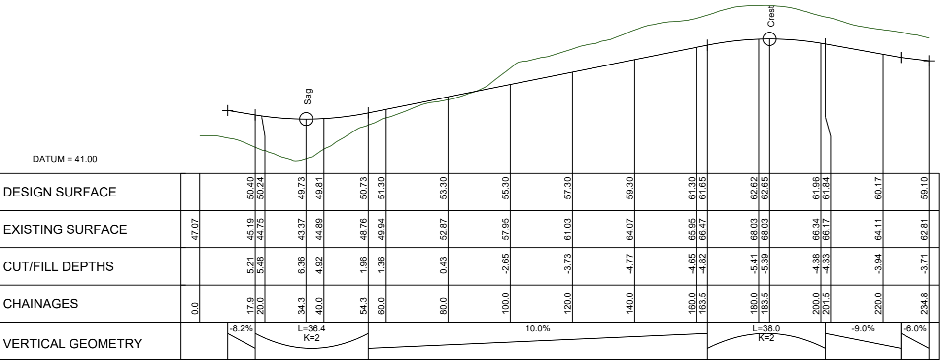
LONGITUDINAL SECTION JOAL 22 SCALE HORIZ=1:1200 @ A1 VERT=1:600 @ A1
