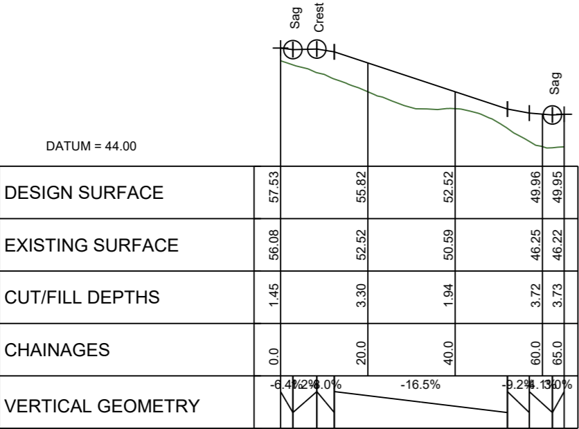
LONGITUDINAL SECTION JOAL 28 SCALE HORIZ=1:1200 @ A1 VERT=1:600 @ A1
