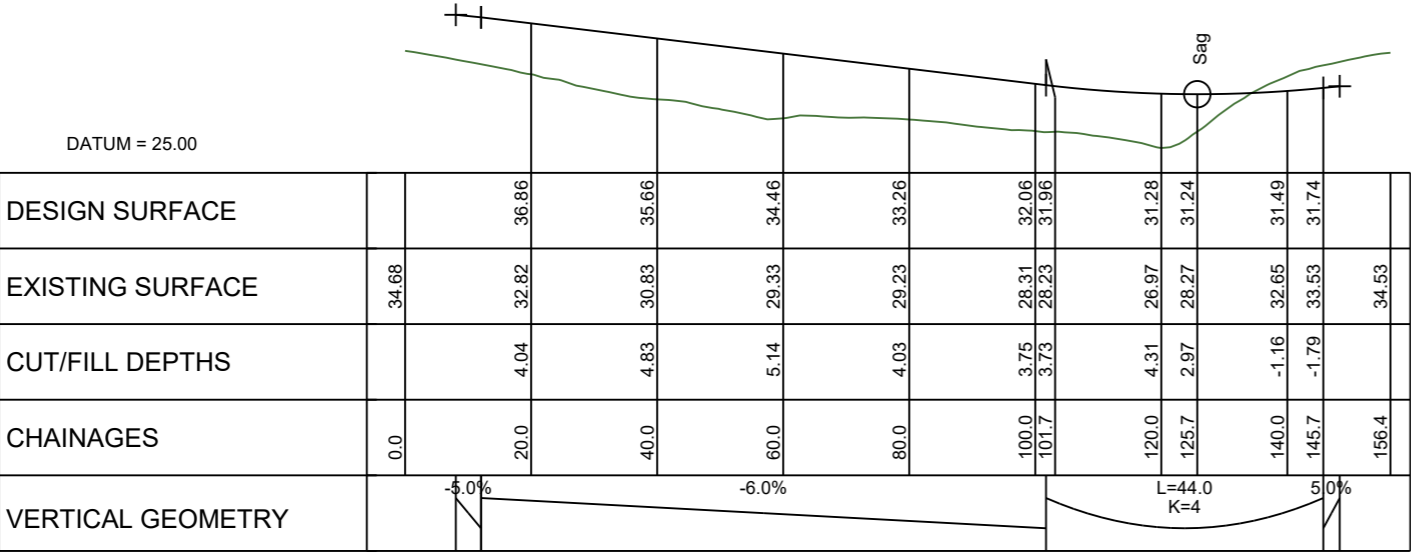
LONGITUDINAL SECTION JOAL 16 SCALE HORIZ=1:1200 @ A1 VERT=1:600 @ A1
