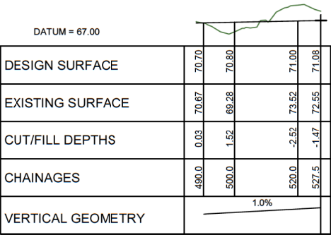
LONGITUDINAL SECTION ROAD 21 SCALE HORIZ=1:1200 @ A1 VERT=1:600 @ A1
