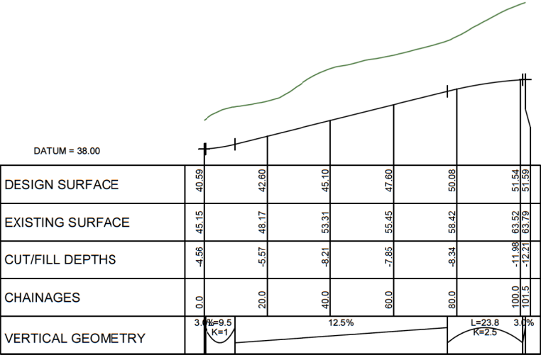
LONGITUDINAL SECTION ROAD 20 SCALE HORIZ=1:1200 @ A1 VERT=1:600 @ A1
