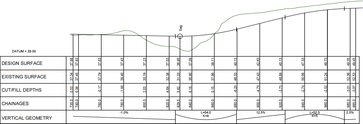
LONGITUDINAL SECTION ROAD 17 SCALE HORIZ=1:1200 @ A1 VERT=1:600 @ A1
