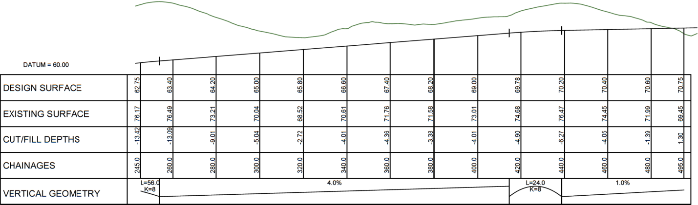
LONGITUDINAL SECTION ROAD 21 SCALE HORIZ=1:1200 @ A1 VERT=1:600 @ A1
