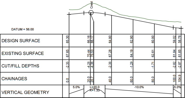
LONGITUDINAL SECTION JOAL 39 SCALE HORIZ=1:1200 @ A1 VERT=1:600 @ A1
