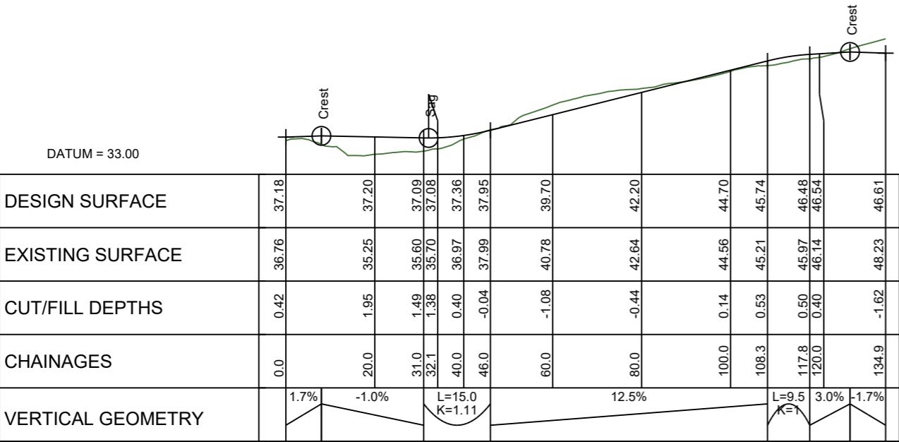
LONGITUDINAL SECTION JOAL 26 SCALE HORIZ=1:1200 @ A1 VERT=1:600 @ A1
