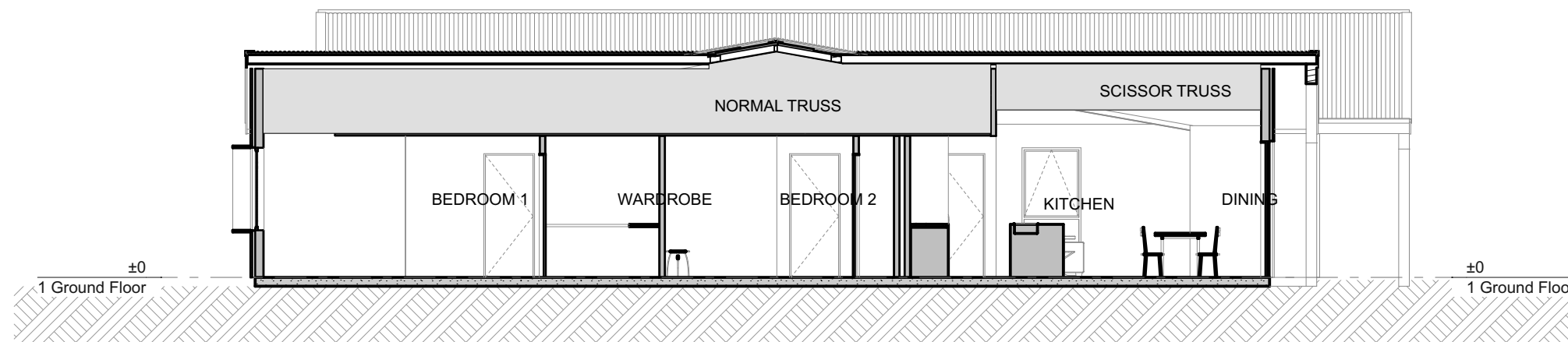
Section 3 1:100
