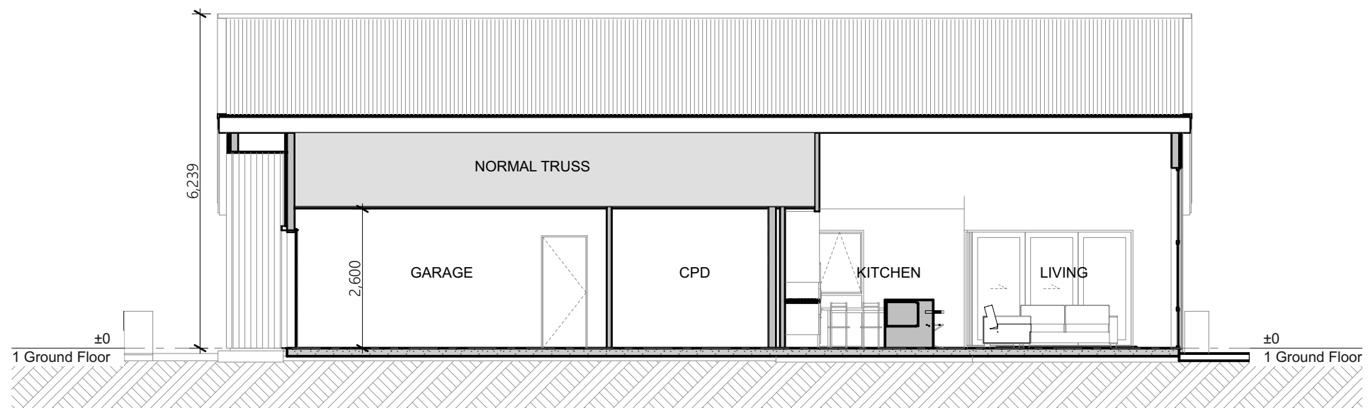
Section 3 1:100
