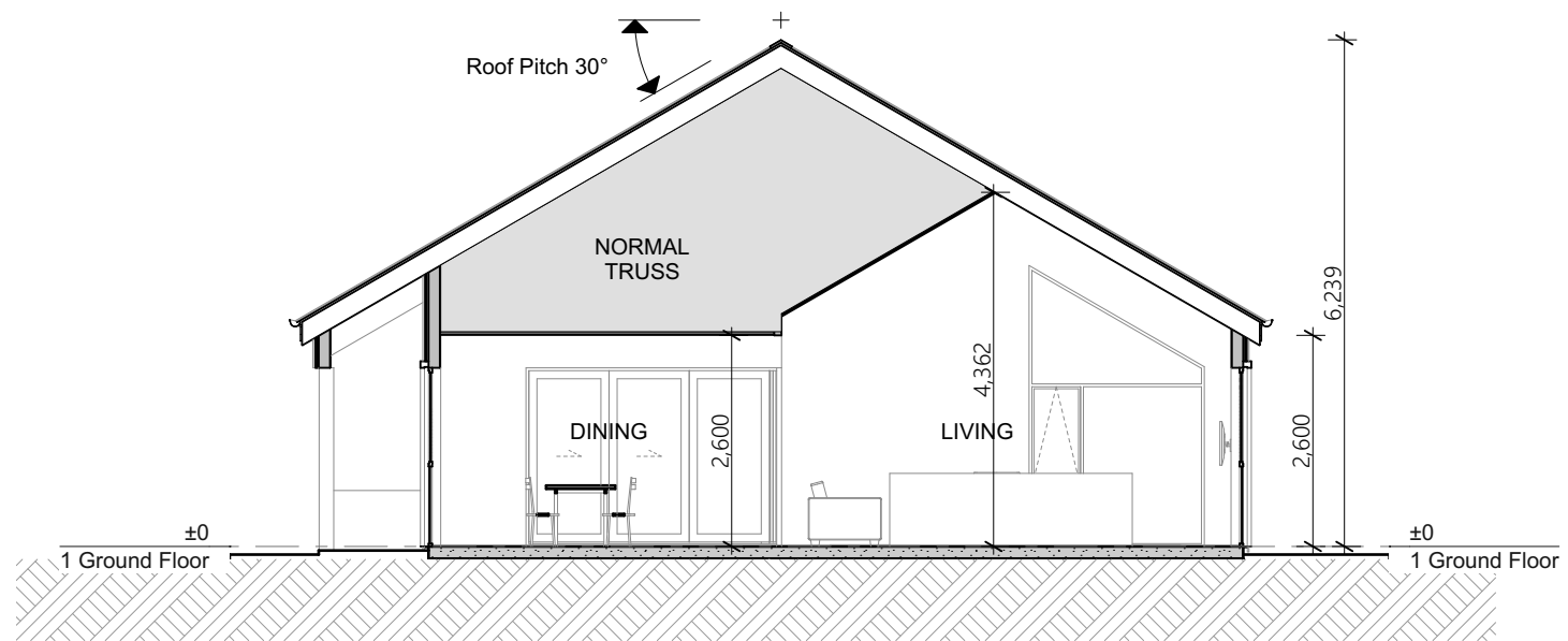
Section 1 1:100
