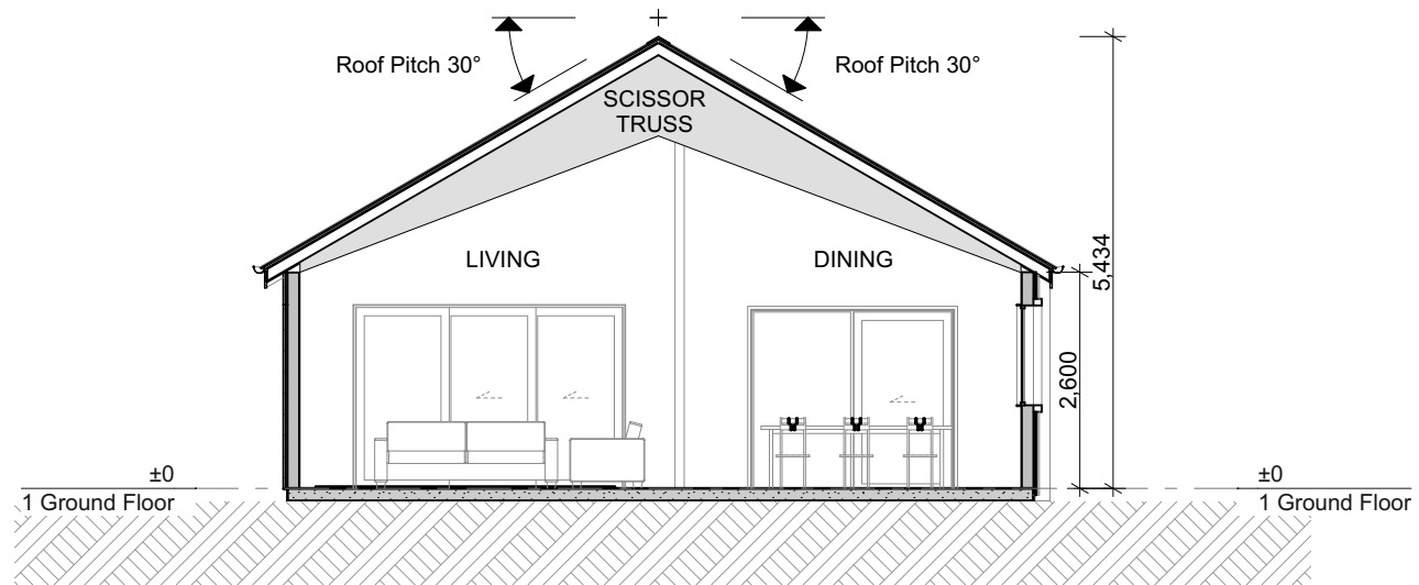
Section 1 1:100
