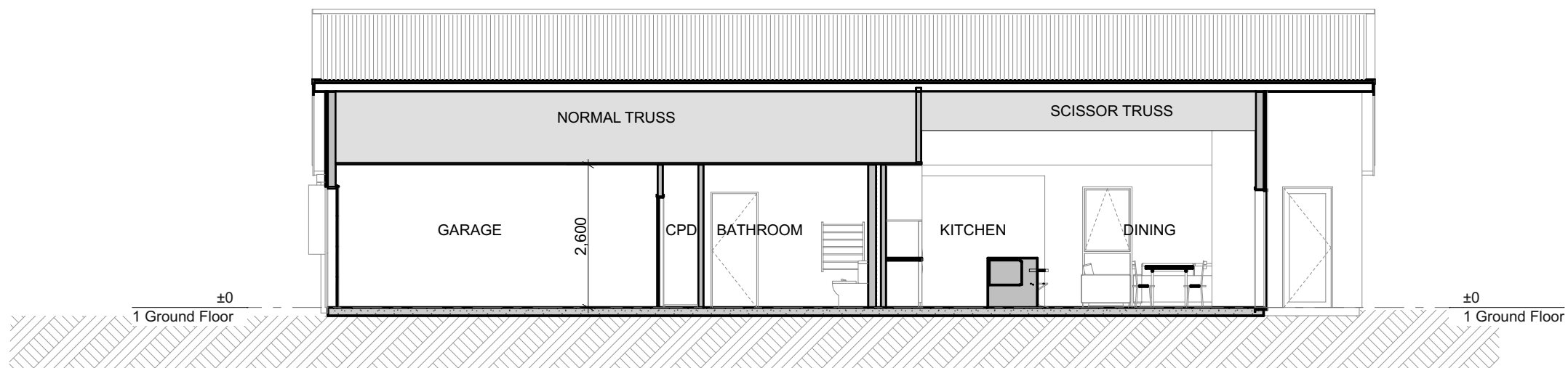
Section 3 1:100
