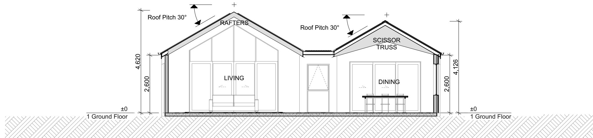
Section 1 1:100
