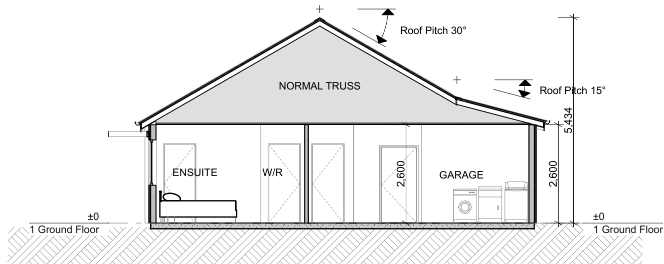
Section 2 1:100
