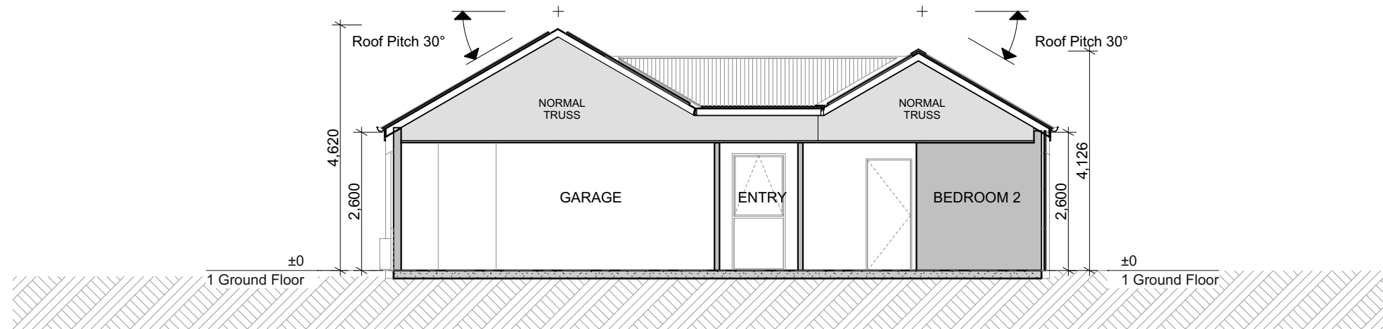
Section 2 1:100
