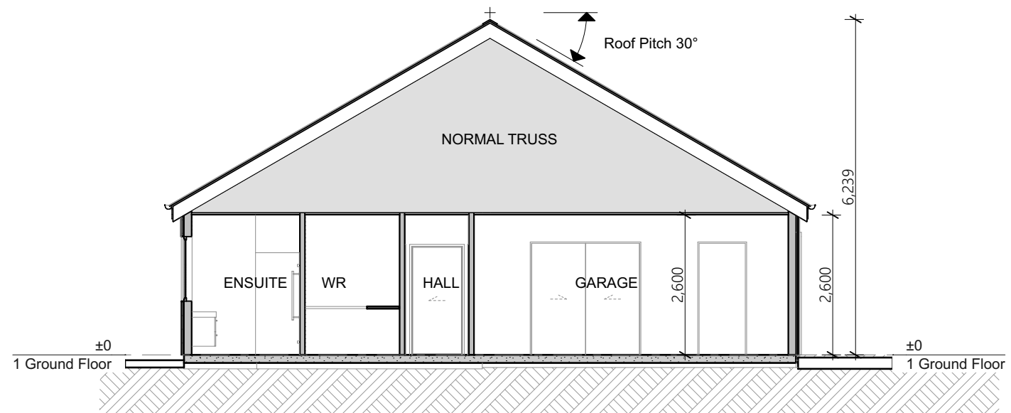
Section 2 1:100
