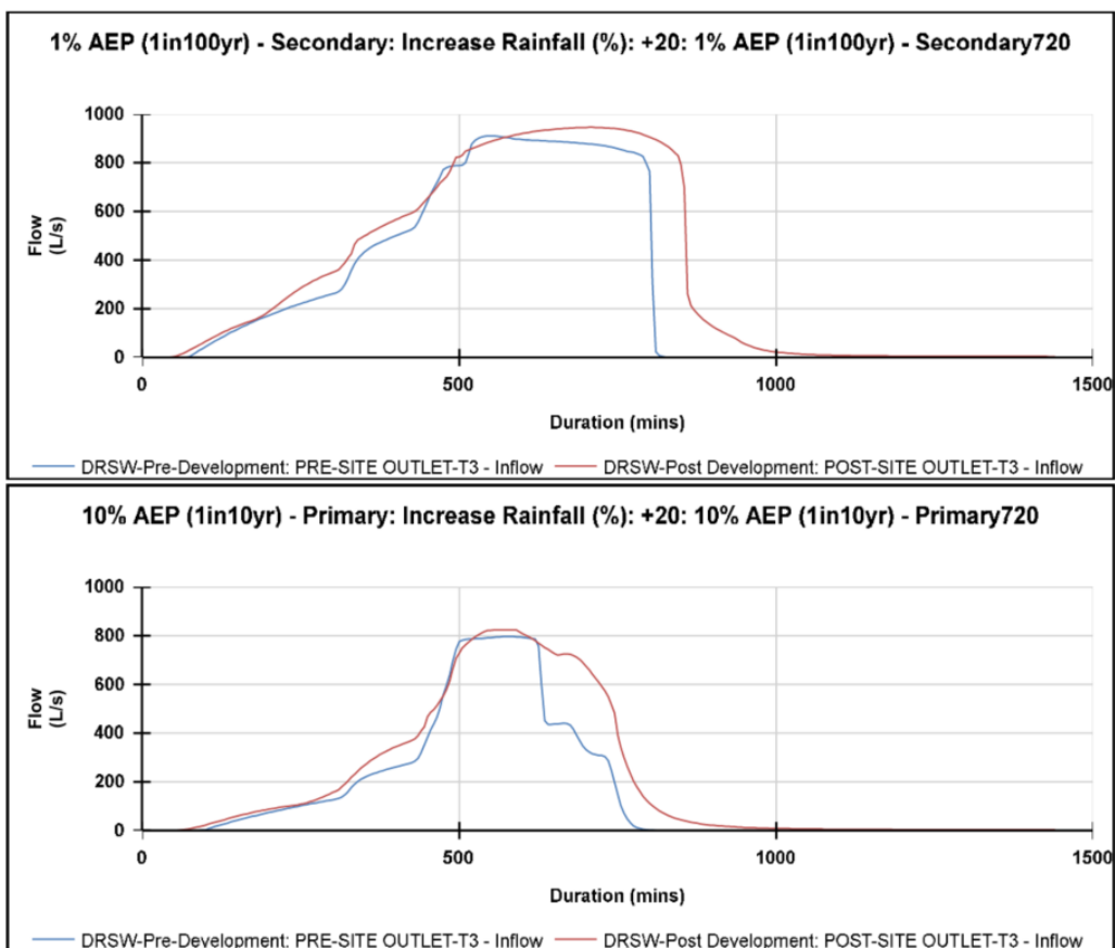
Figure 15. Pre and Post Development Comparison (T3) for the 10- and 100-Year Storm Events
