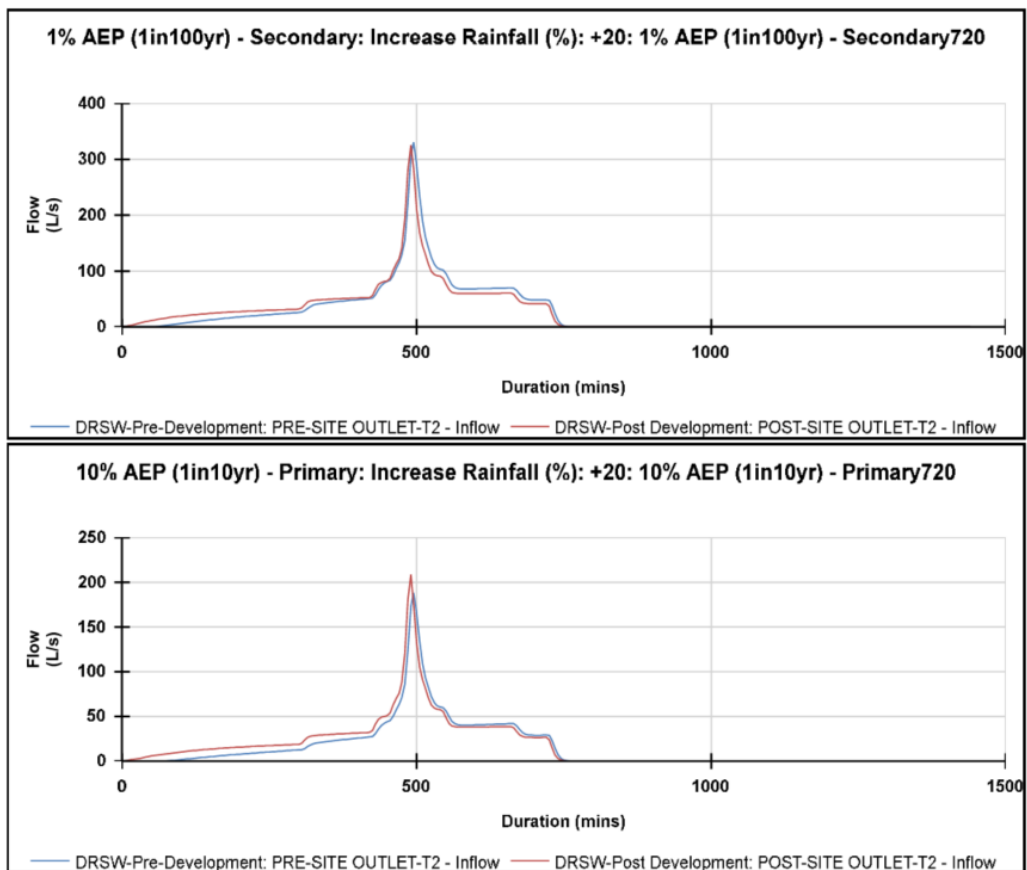
Figure 14. Pre and Post Development Comparison (T2) for the 10- and 100-Year Storm Events
