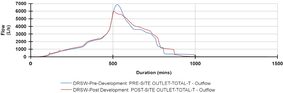
1% AEP (1in100yr) - Secondary: Increase Rainfall (%): +20: 1% AEP (1in100yr) - Secondary720
