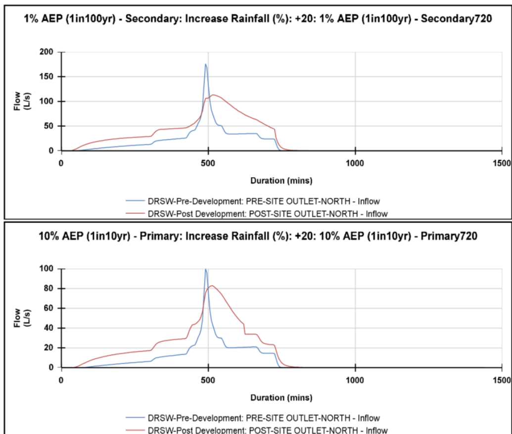
Figure 17. Pre and Post Development Comparison (Muri) for the 10- and 100-Year Storm Events
