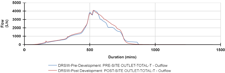
10% AEP (1in10yr) - Primary: Increase Rainfall (%): +20: 10% AEP (1in10yr) - Primary720
