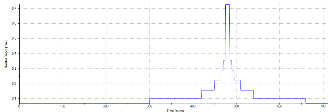
Figure 10. 10% AEP Rainfall Distribution
