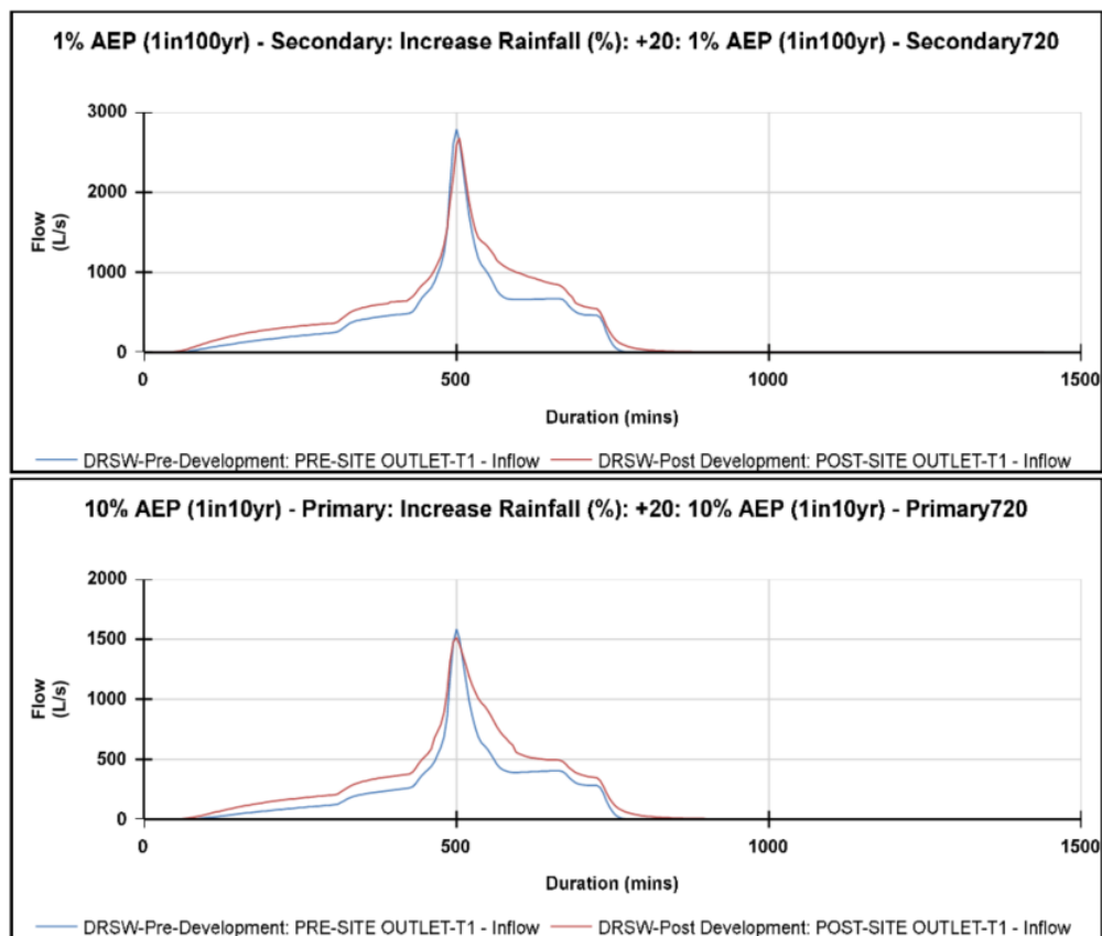
Figure 13. Pre and Post Development Comparison (T1) for the 10- and 100-Year Storm Events
