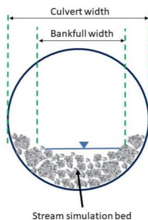
Figure 9. Stream Simulation Sketch (Extract from NZ Fish Passage Guidelines 2018)
