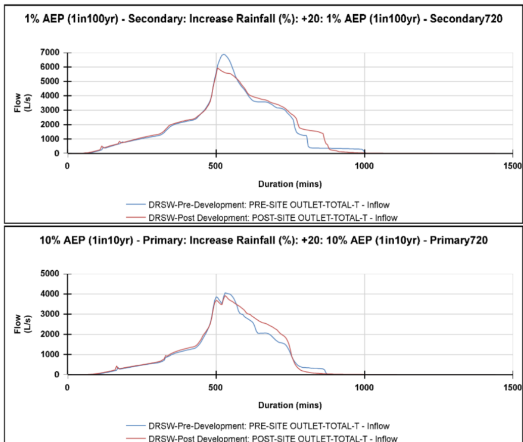
Figure 16. Pre and Post Development Comparison (T-T) for the 10- and 100-Year Storm Events
