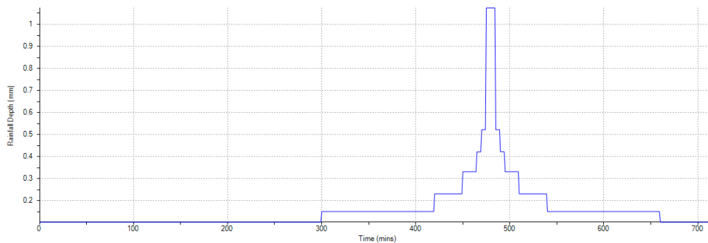
Figure 11. 1% AEP Rainfall Distribution
