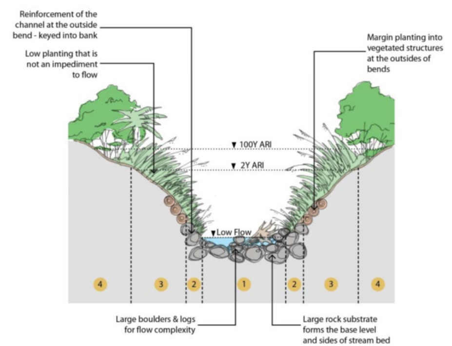
Stream Diversion Type 2 – Steep stream cross section
