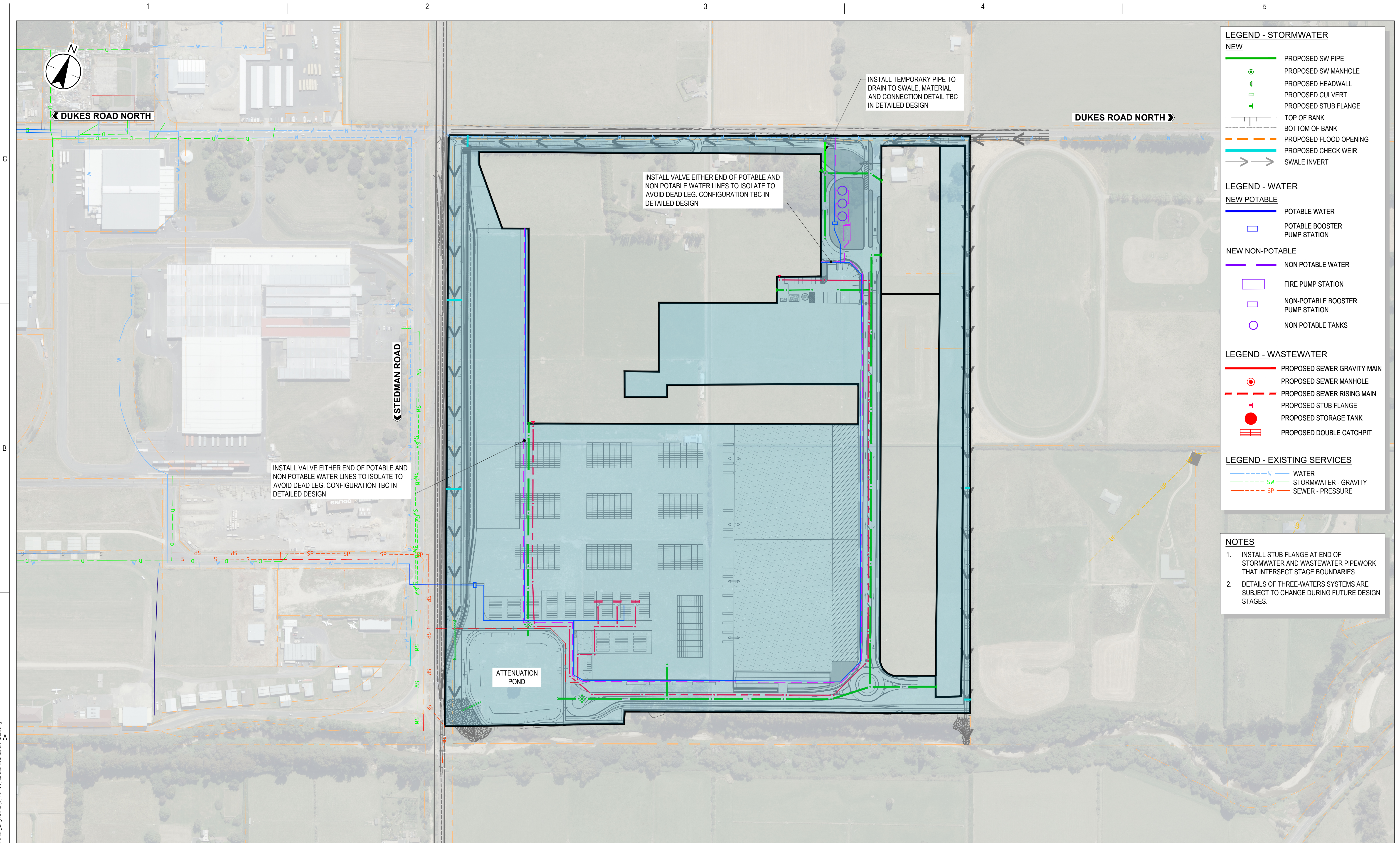
1:2000 20 0 20 40 60 80 100 A1 1:4000 A3 3 WATERS PLAN SCALE - 1:2000
