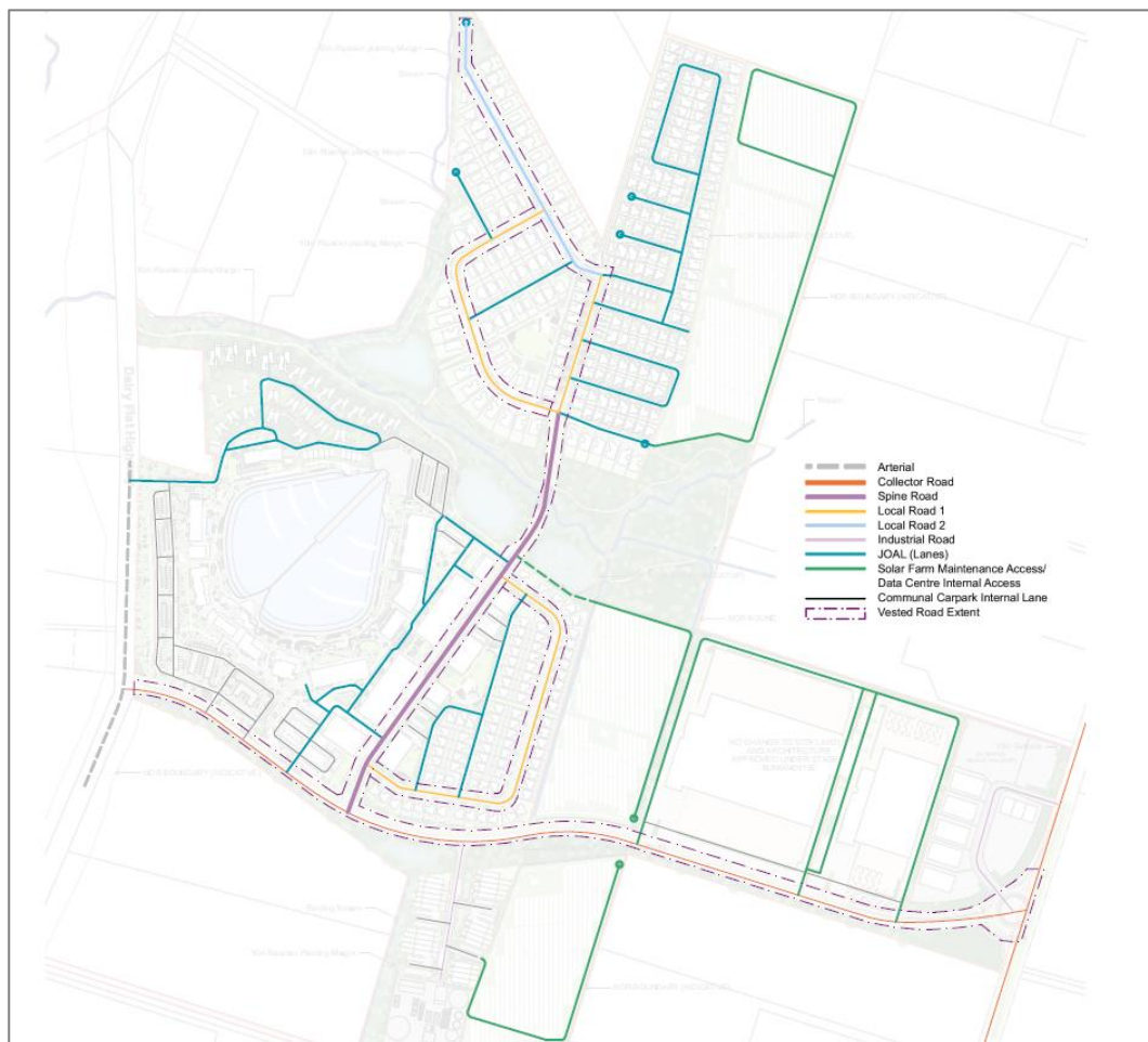
Figure 30: Internal Roading Network and Typologies (Source: Studio Pacific)
