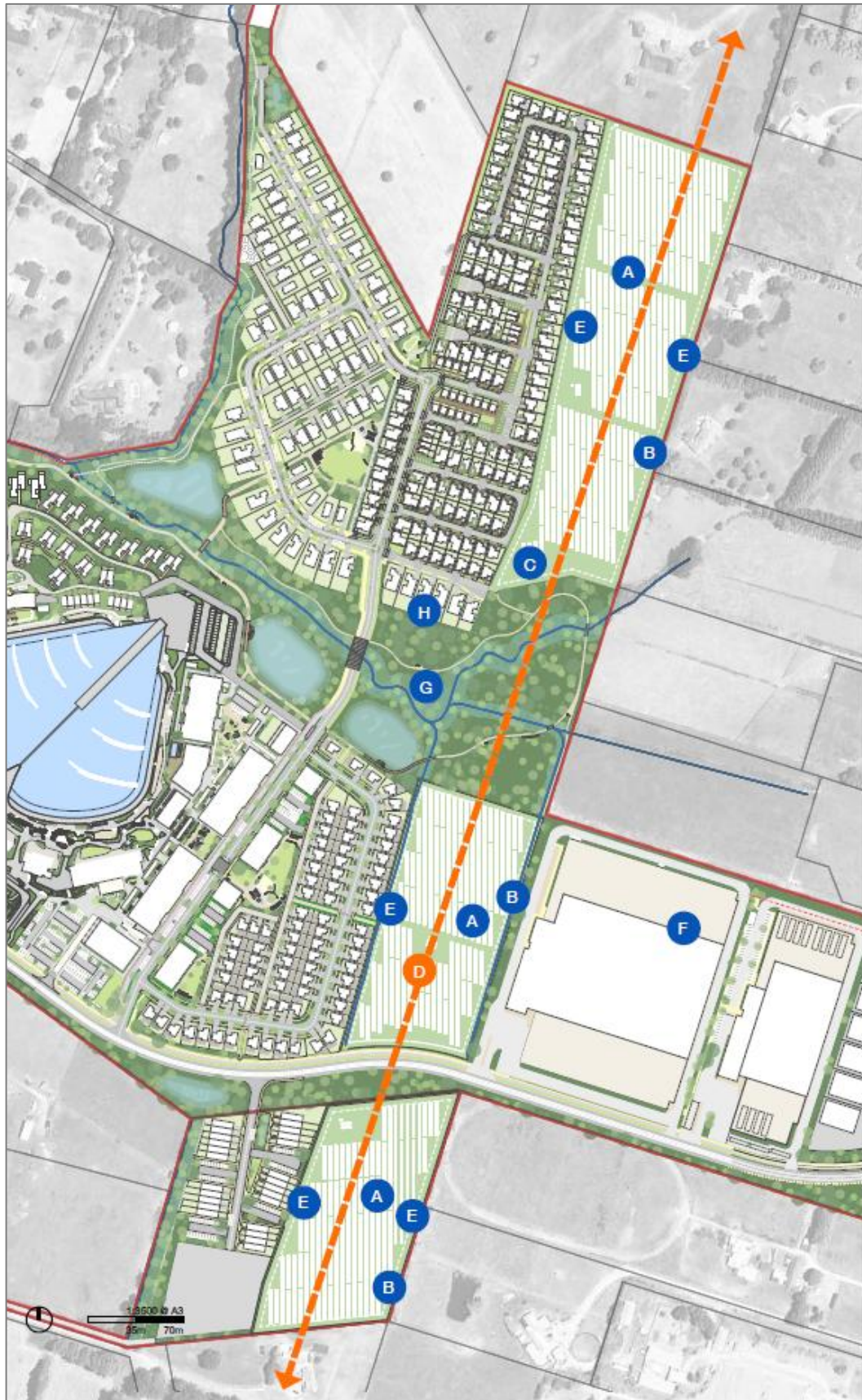
Figure 29: Solar Farm Precinct and RTN corridor. Source: Studio Pacific Architecture.
