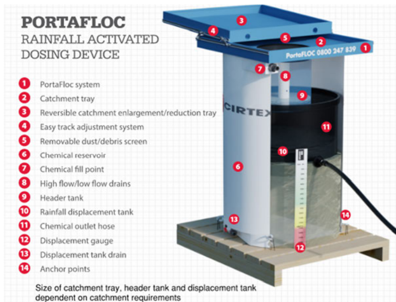
Fig 2 Example Rainfall Activated Flocculation Dosing Detail.
