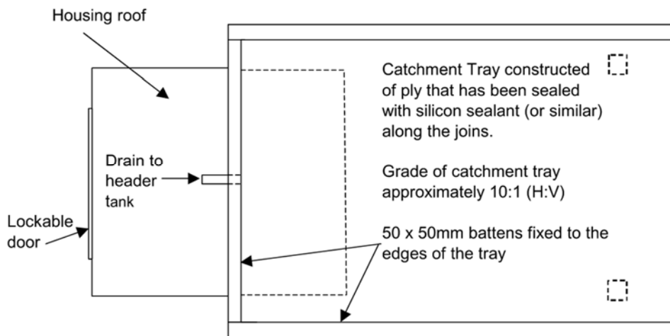
Fig 1: Rainfall Activated Flocculation System Catchment Tray – Plan View
