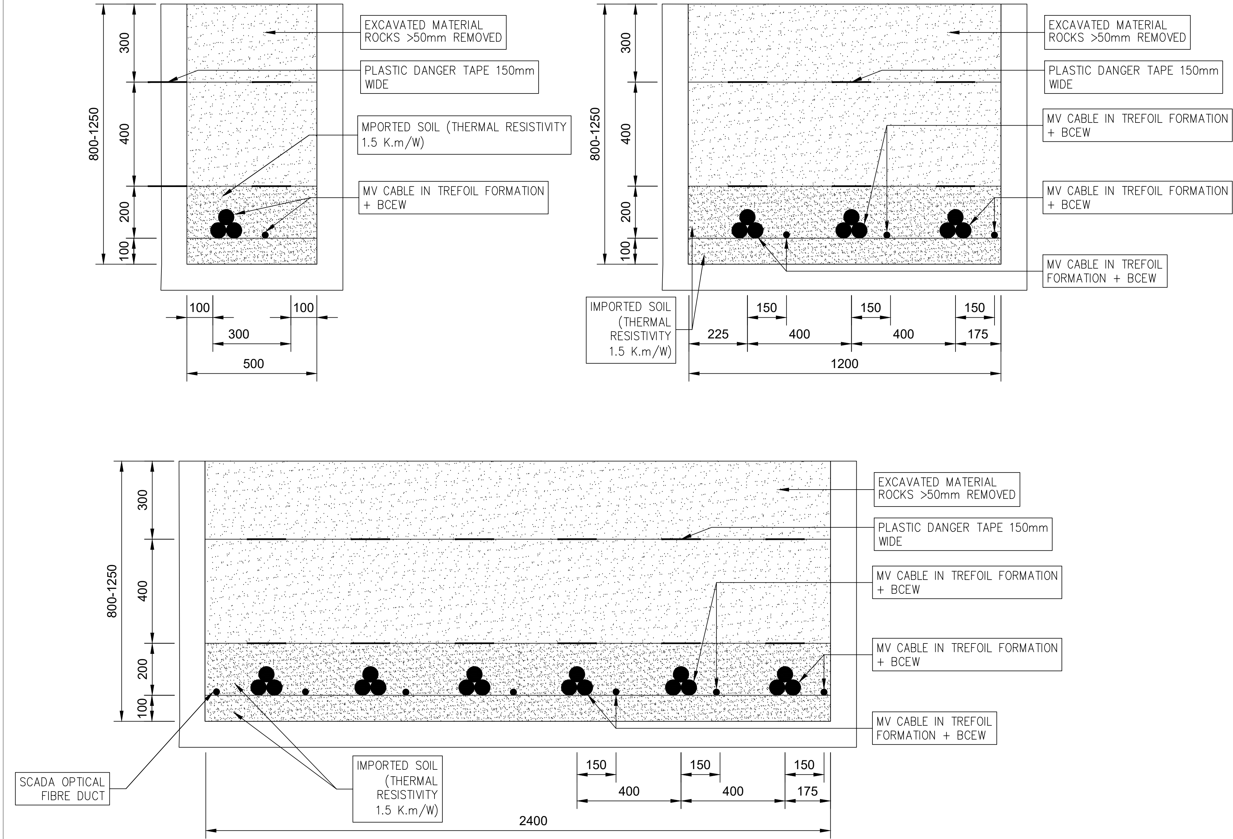
TYPICAL MV TRENCH
