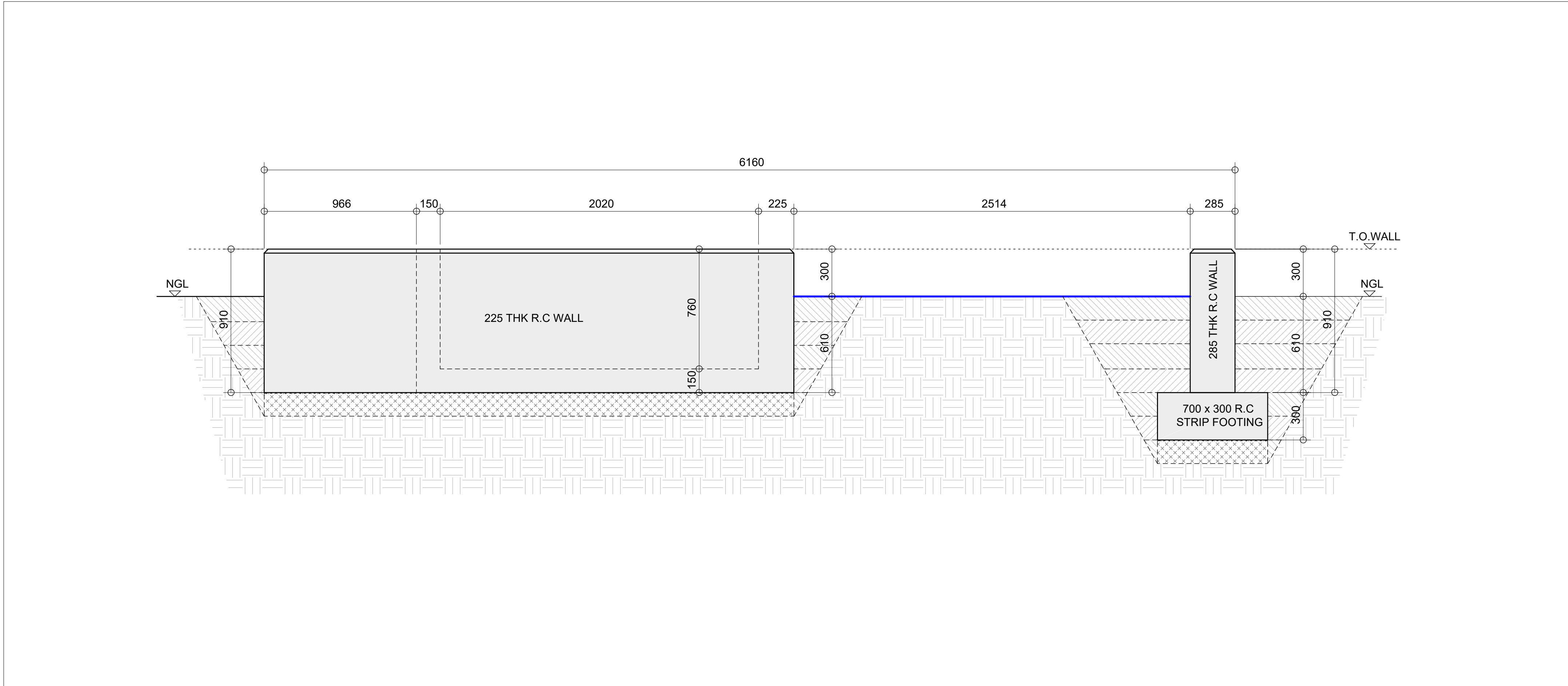
FOUNDATION ELEVATION VIEW
