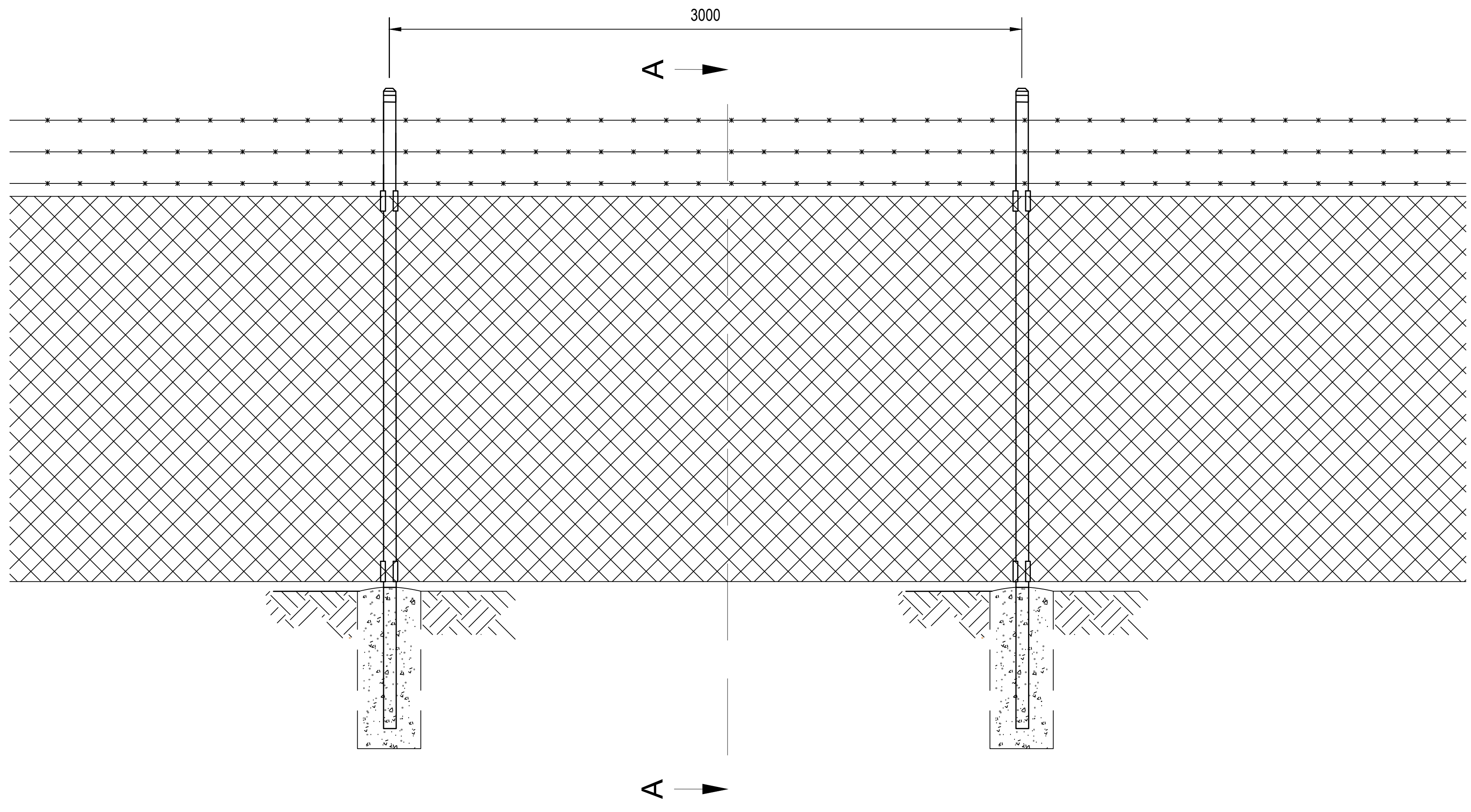
PERIMETER FENCE FRONT VIEW
