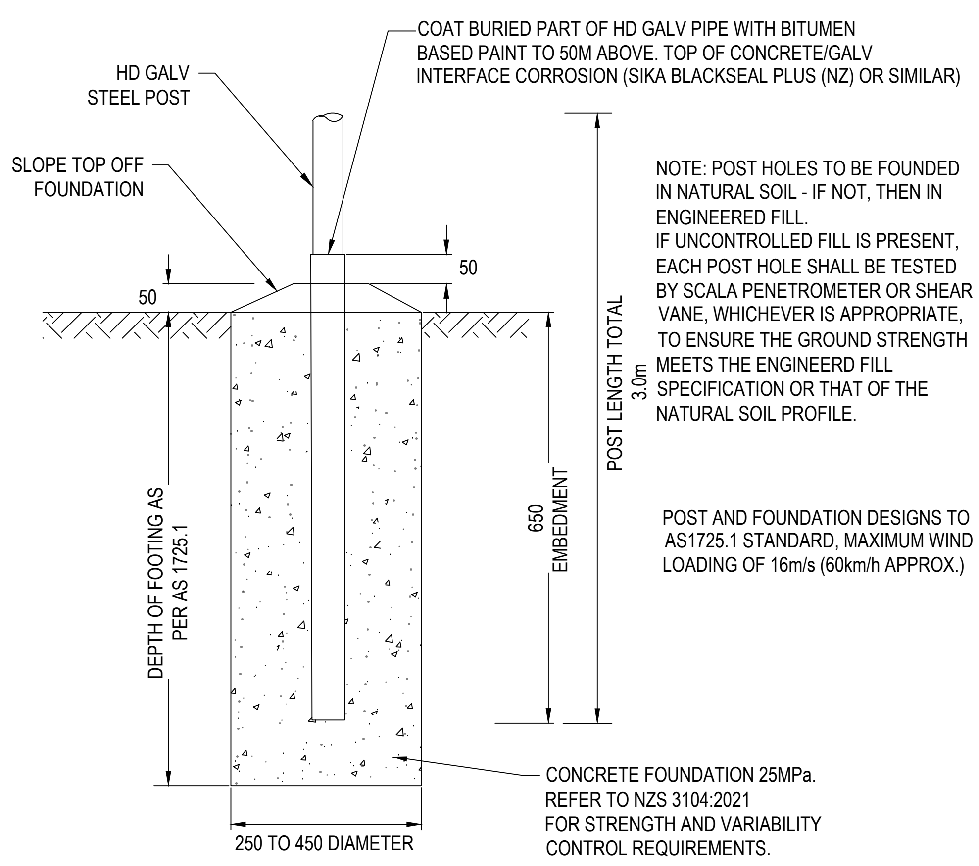
PERIMETER FENCE TYPICAL FOUNDATION DETAIL
