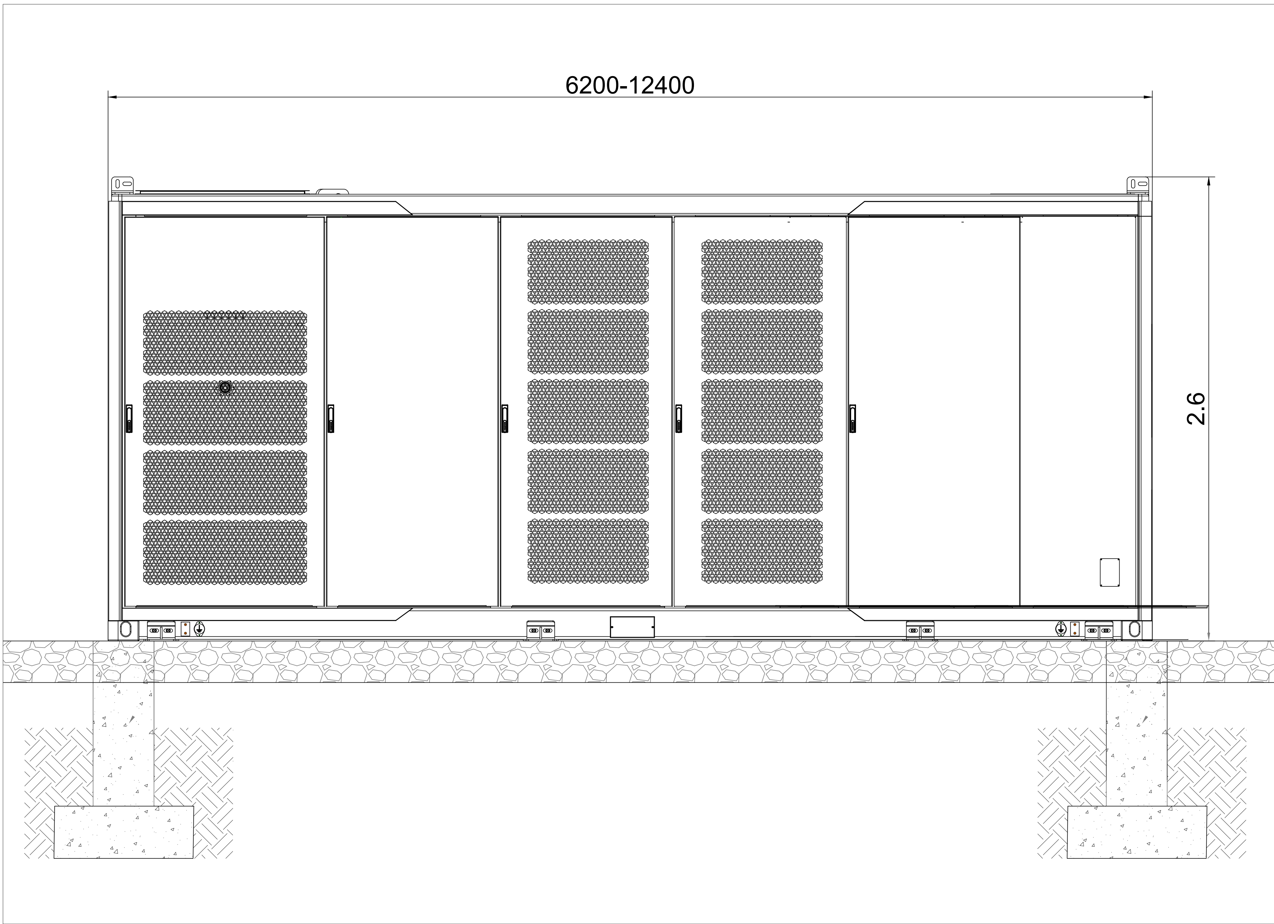
FRONT VIEW
