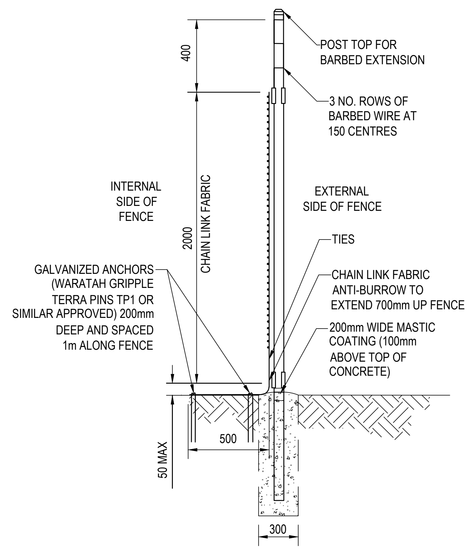
PERIMETER FENCE ANTI-BURROW SECTION A-A
