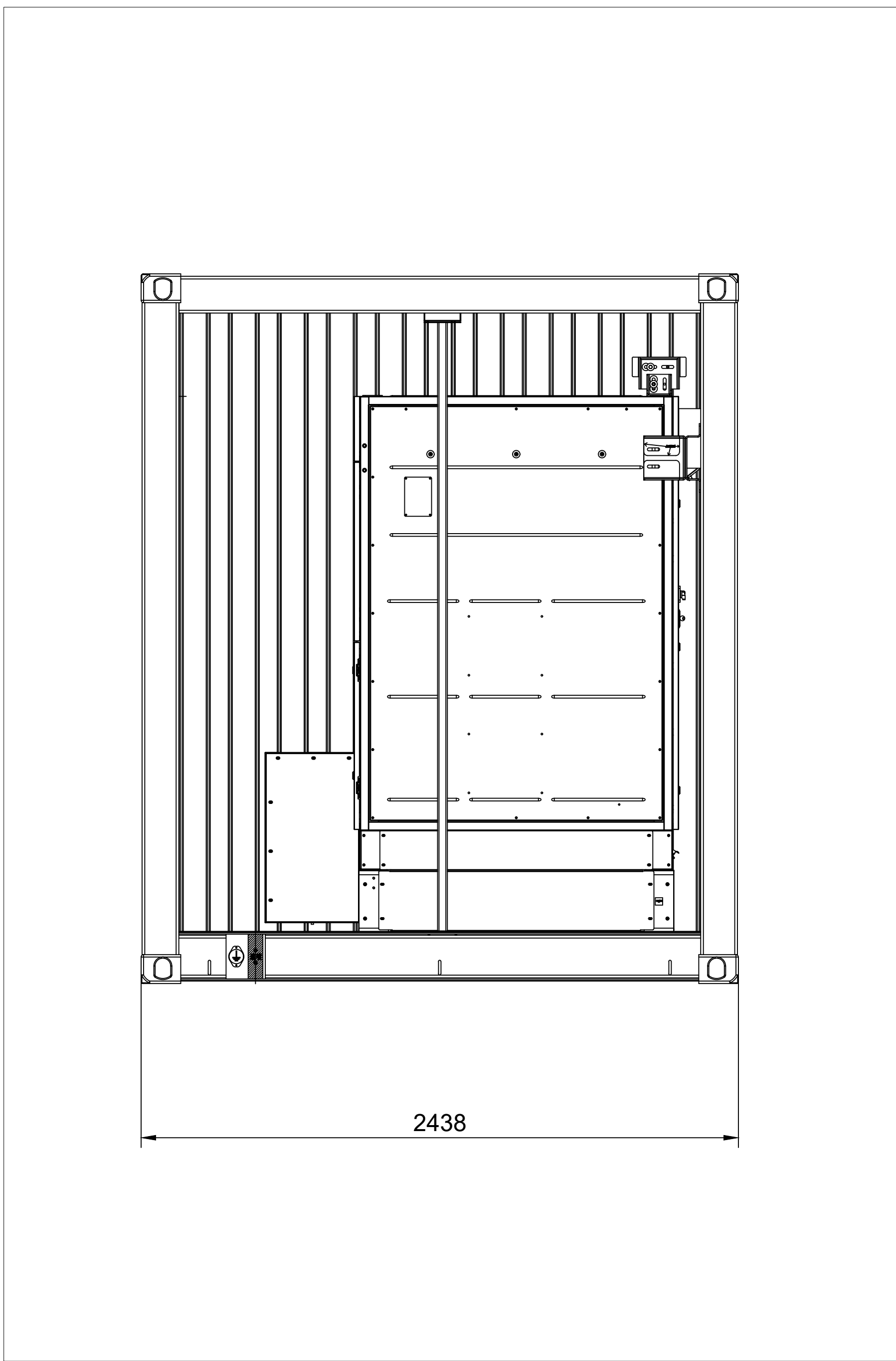
RIGHT VIEW
