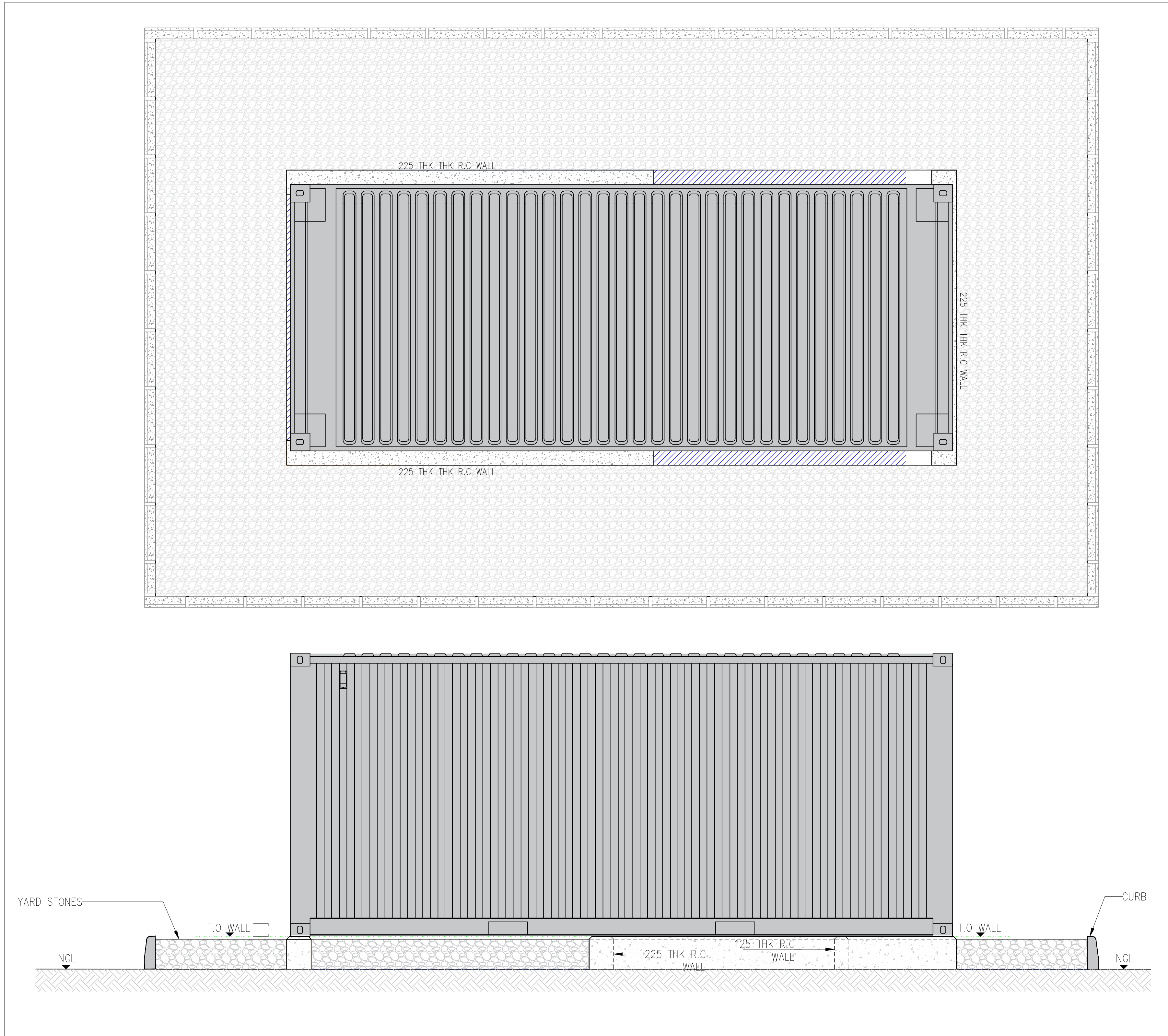
ITS SURROUNDINGS PLAN
