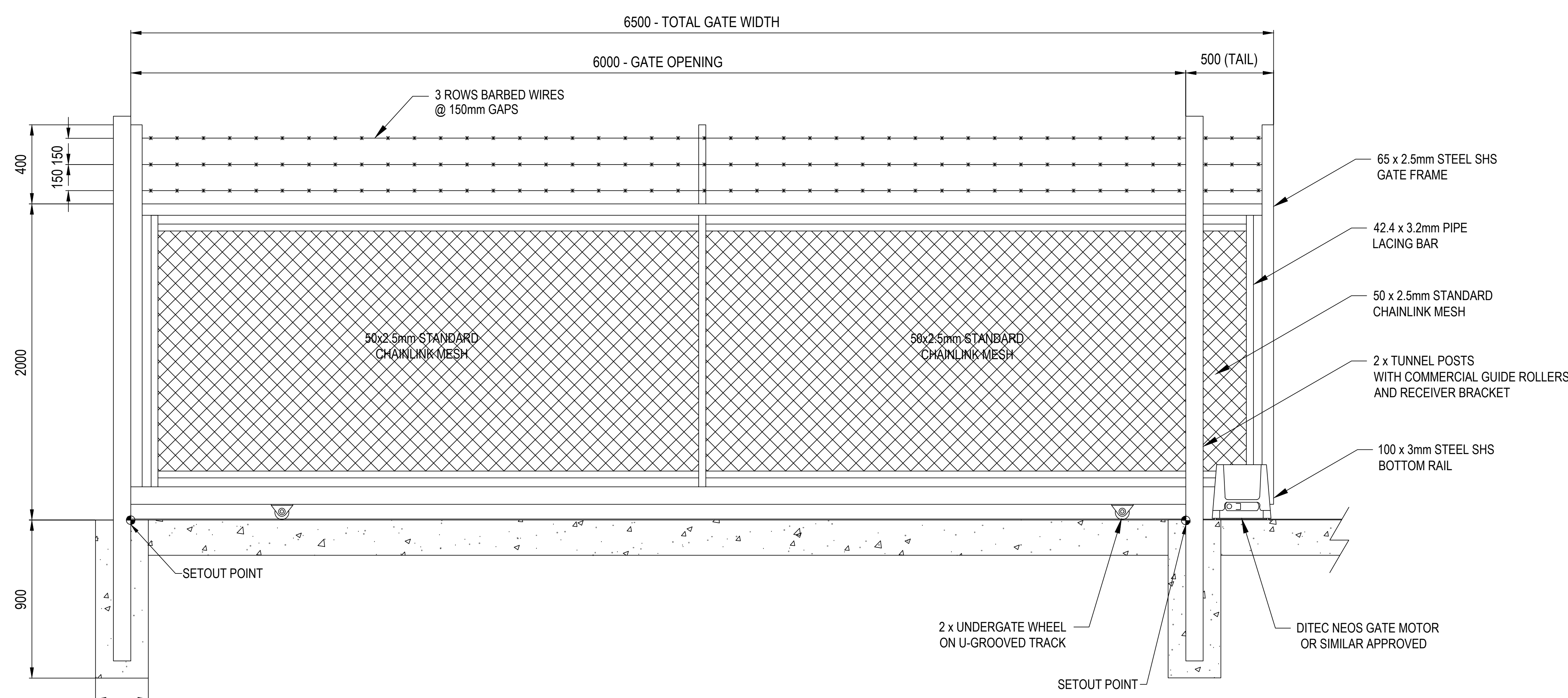
TYPICAL GATE DETAIL
