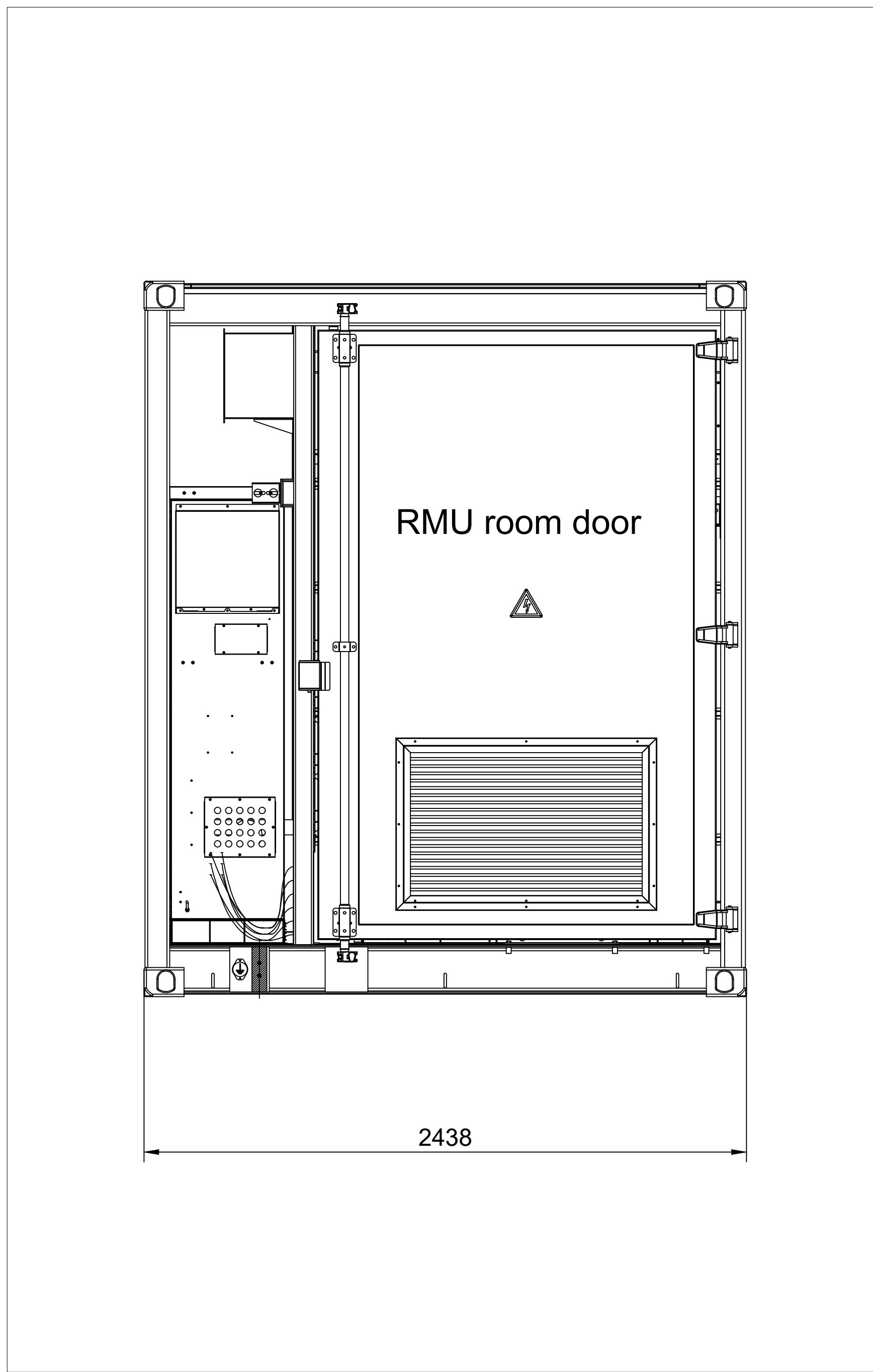
LEFT VIEW
