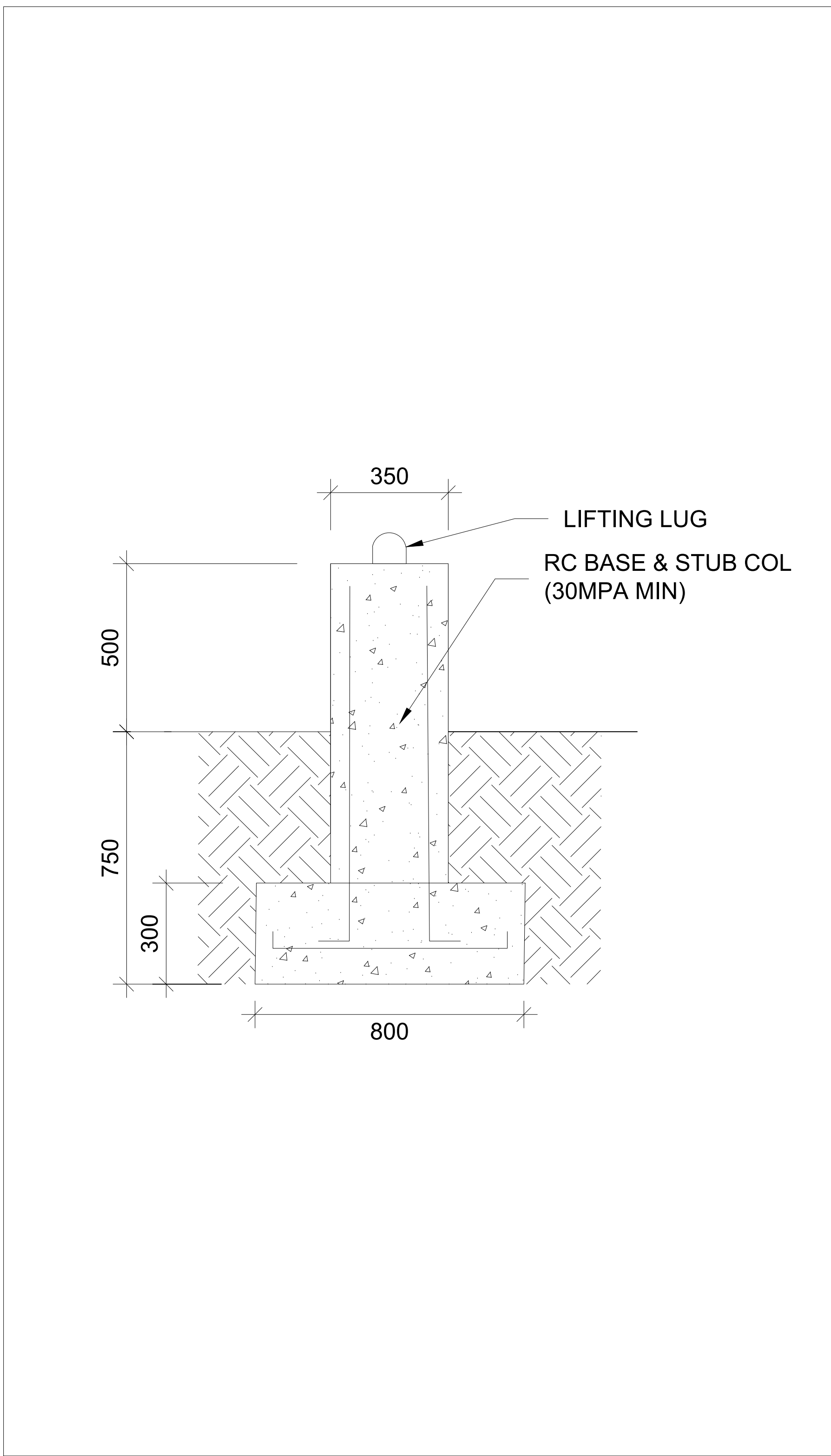
TYPICAL FOOTING SECTION
