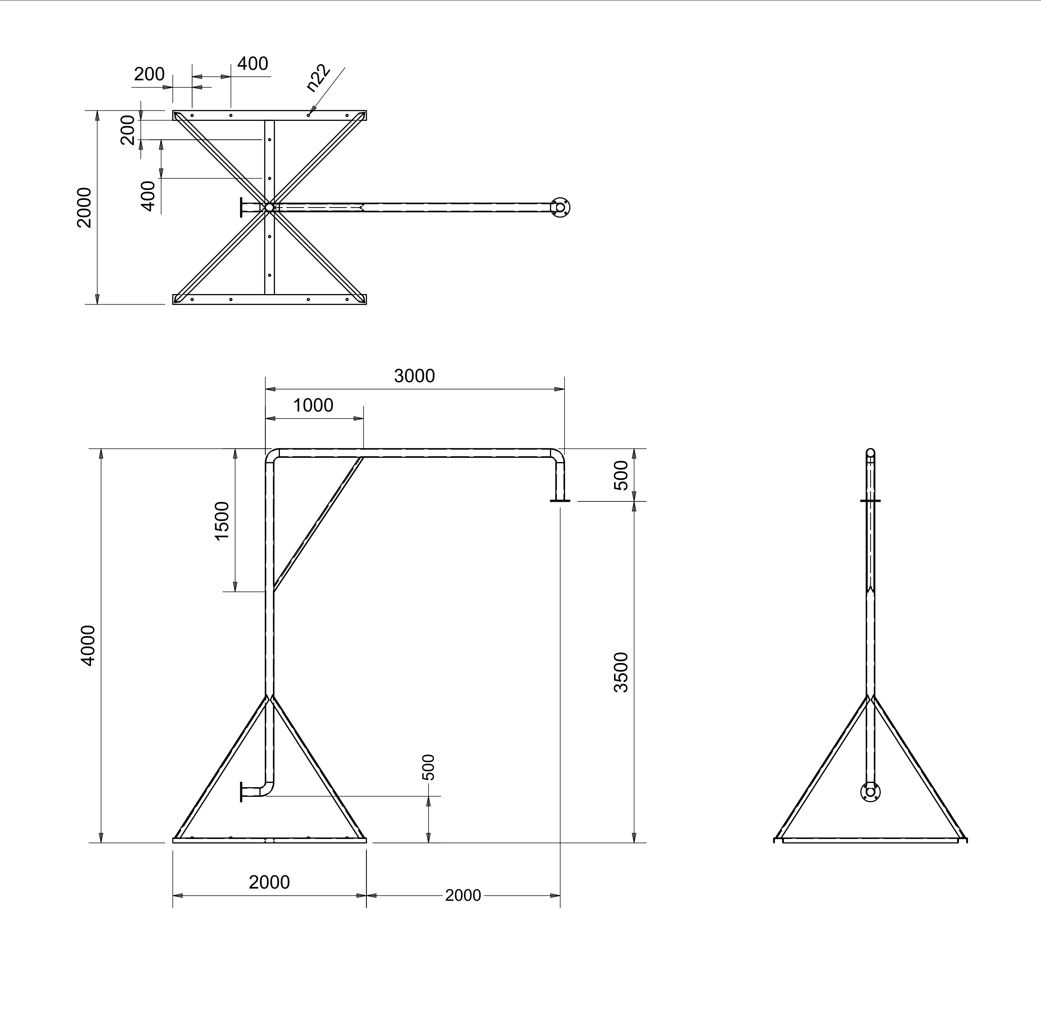
TYPICAL GOOSE NECK DETAILS
