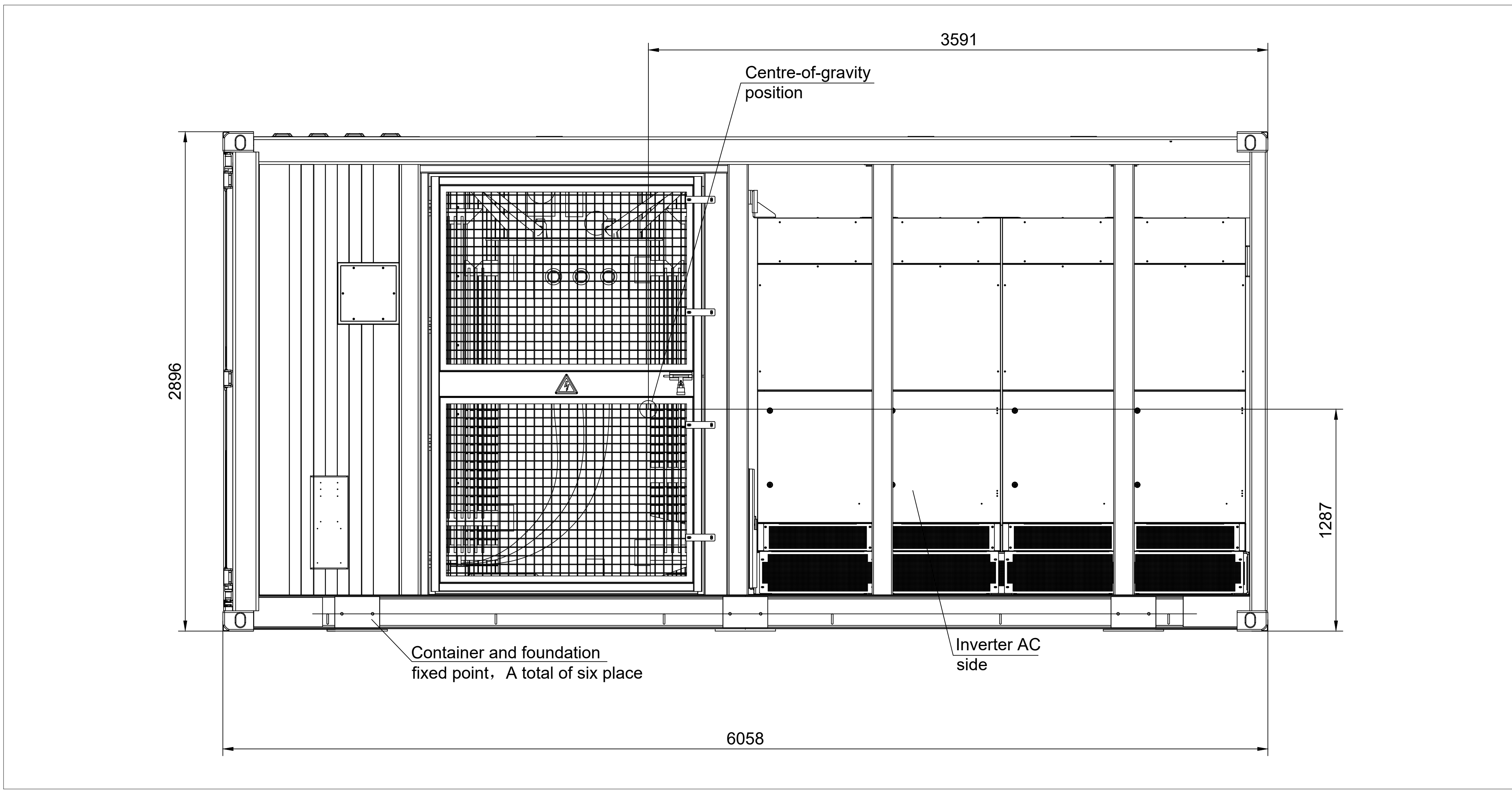
FRONT VIEW
