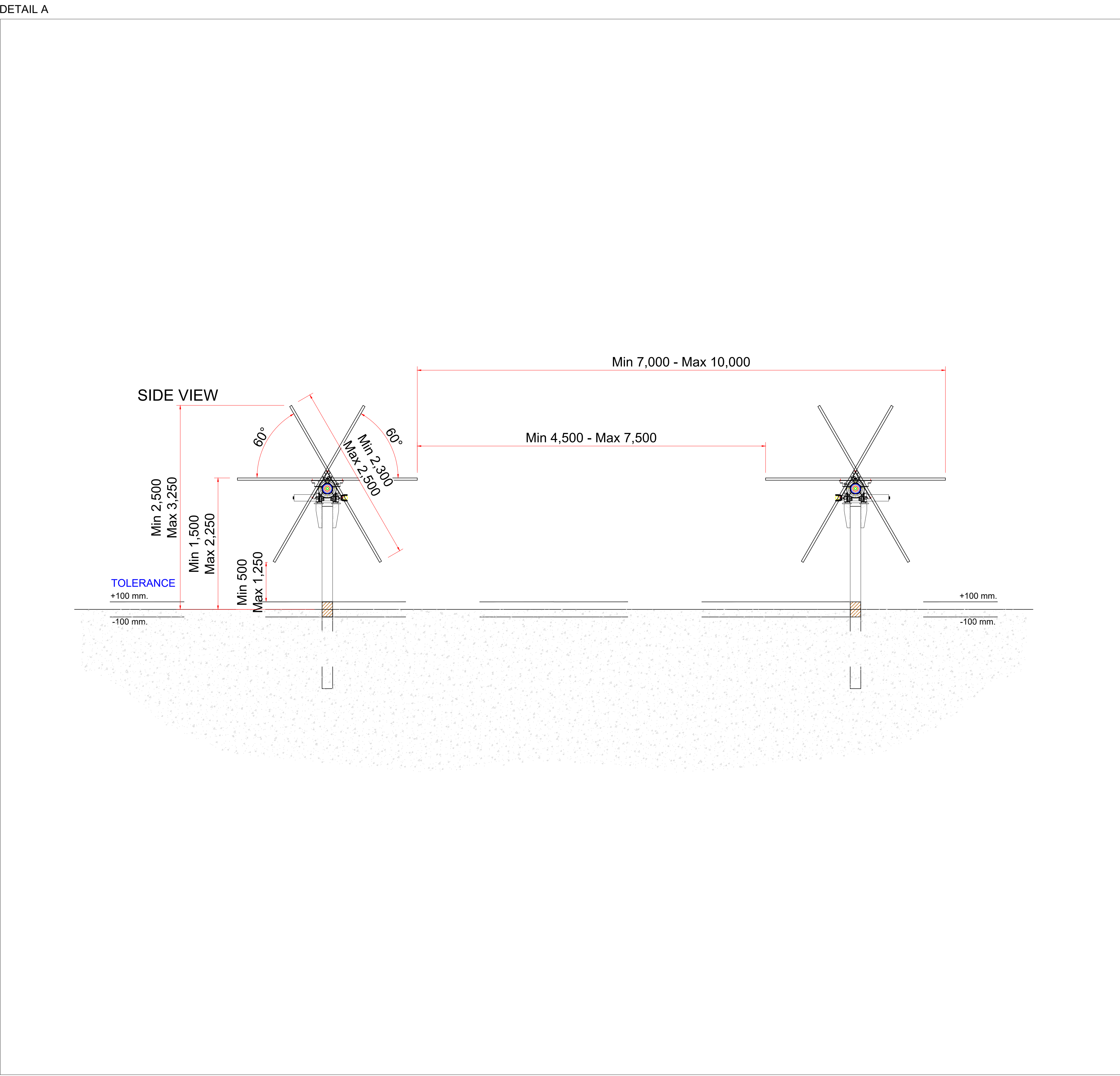
TYPICAL FRONT VIEW
