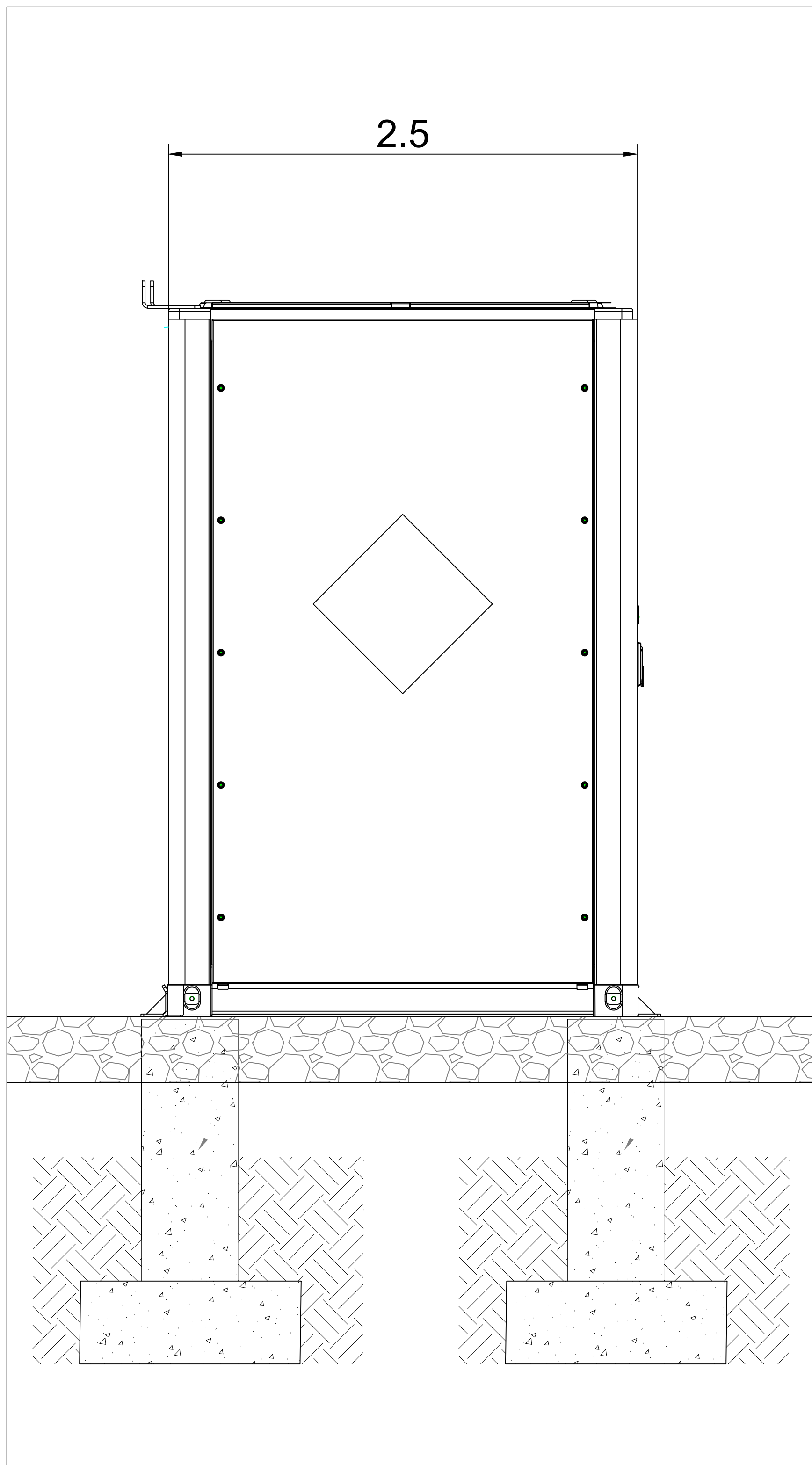
SIDE VIEW
