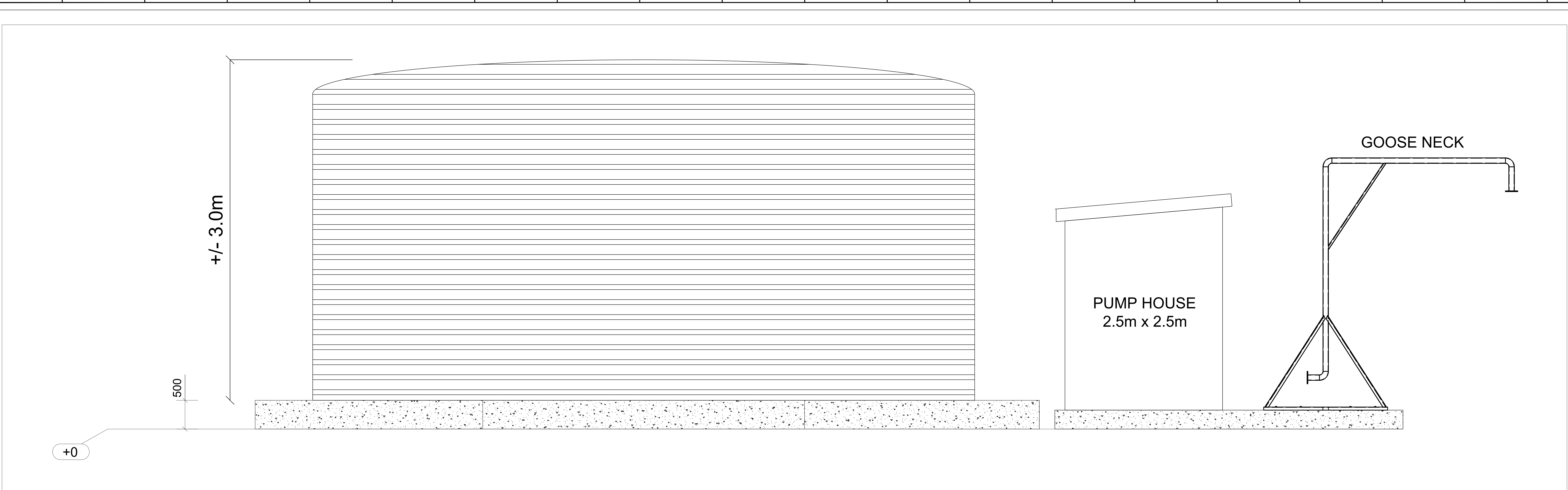
TYPICAL ELEVATION VIEW
