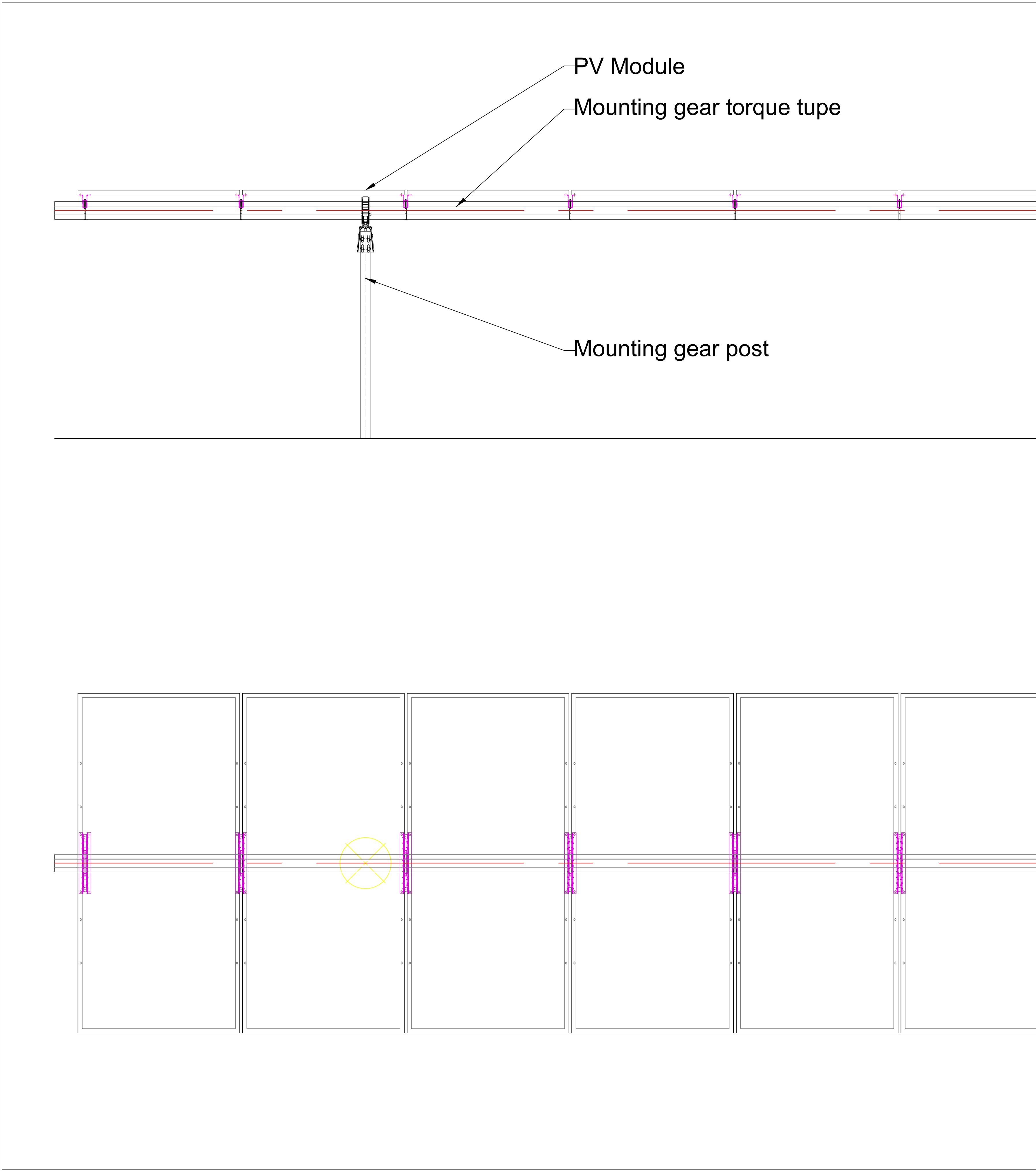
DETAIL A
