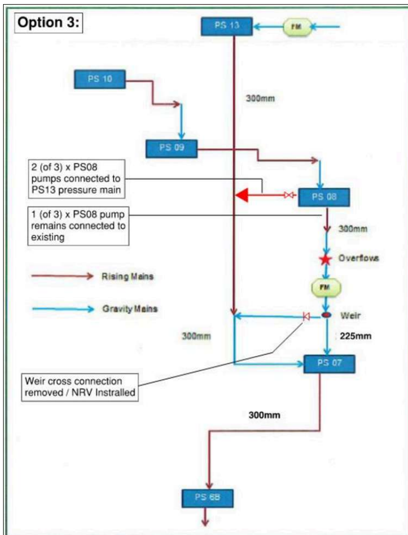
Figure 8: Option 3: Split PS08 Pump Discharge (2x pumps PM13, 1 x pump existing PM08)
