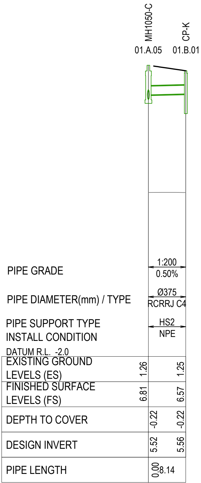
PIPELINE - 01.B 1:500H 1:100V
