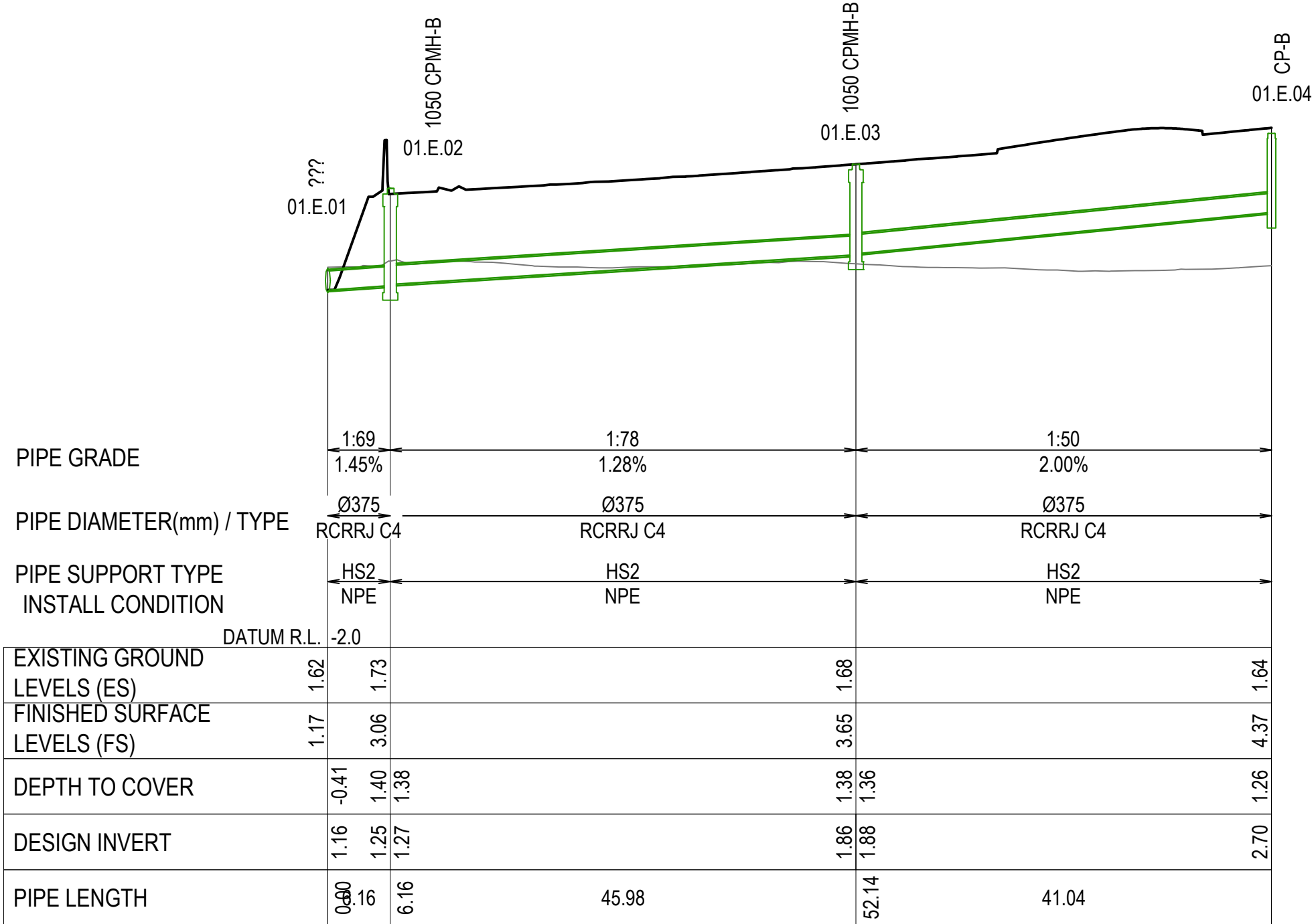
PIPELINE - 01.E 1:500H 1:100V
