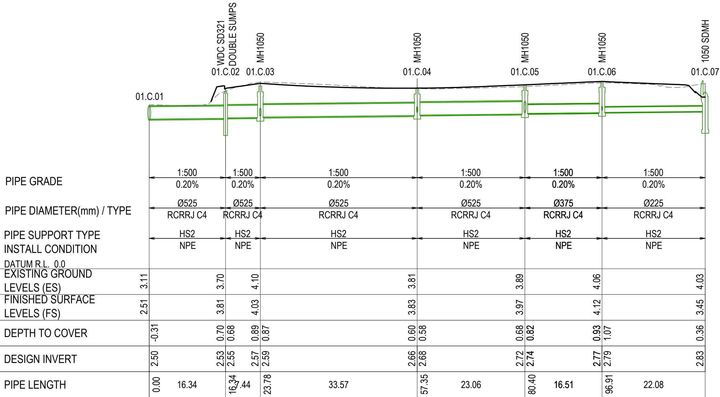
PIPELINE - 01.C 1:500H 1:100V
