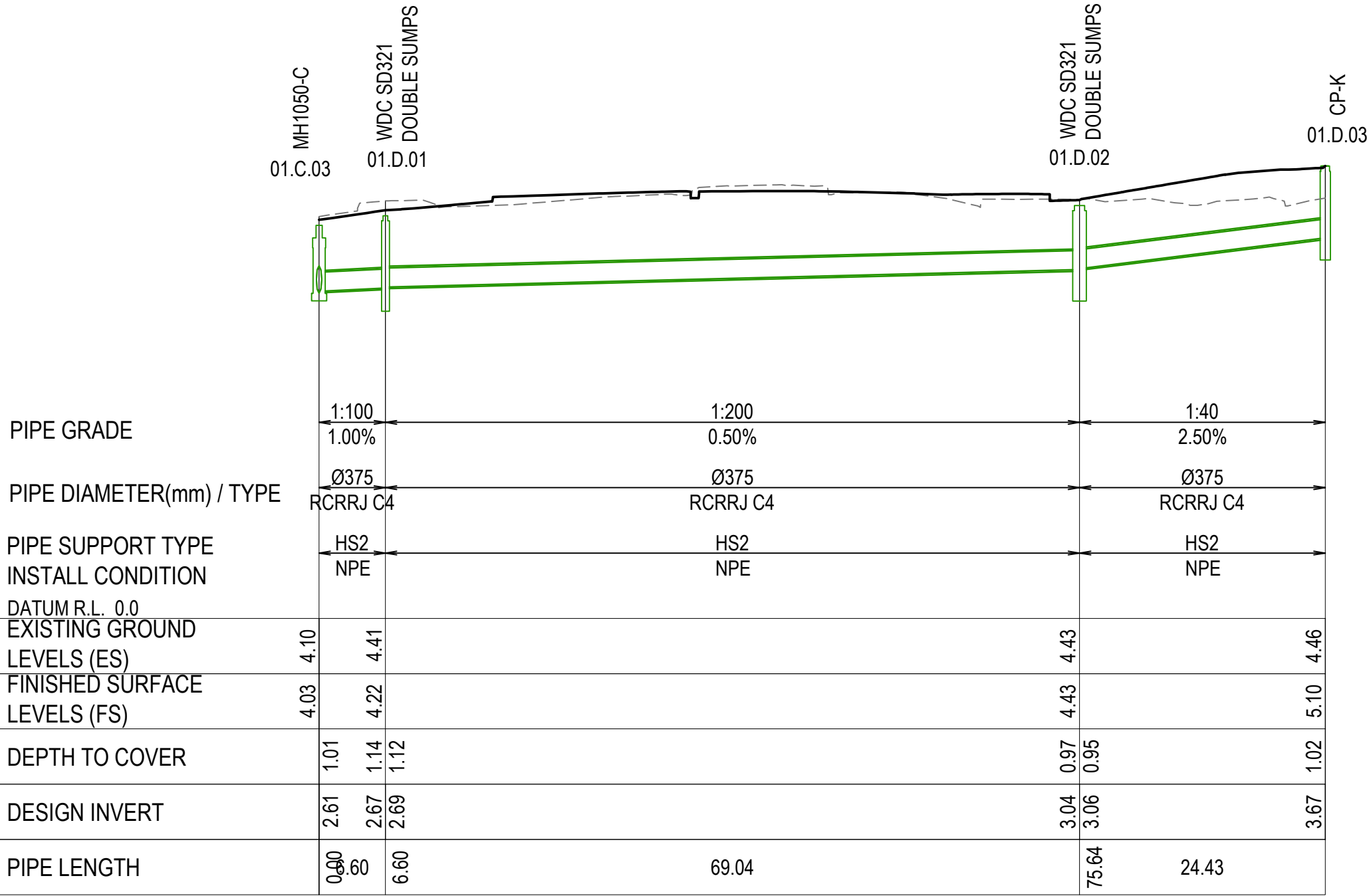
PIPELINE - 01.D 1:500H 1:100V
