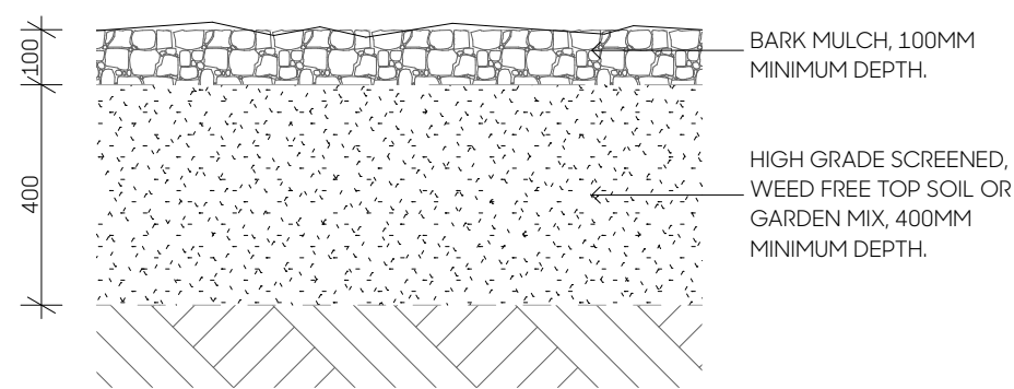
PD-05: GARDEN BEDS 1:15 @ A1, 1:30 @ A3
