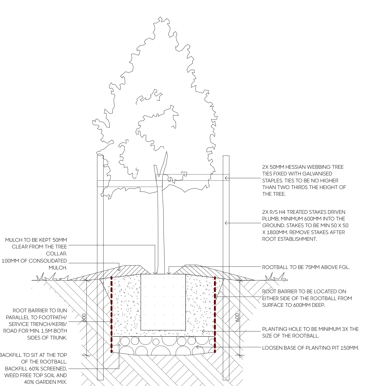
PD-03: TREE WITH ROOT BARRIER 1:15 @ A1, 1:30 @ A3
