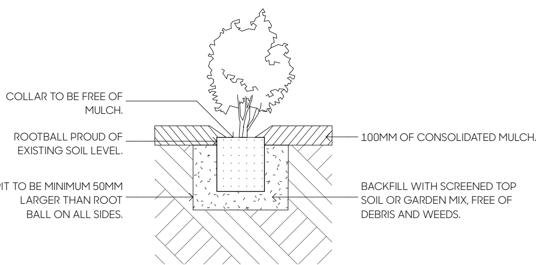
PD-02: SHRUB IN GARDEN 1:15 @ A1, 1:30 @ A3
