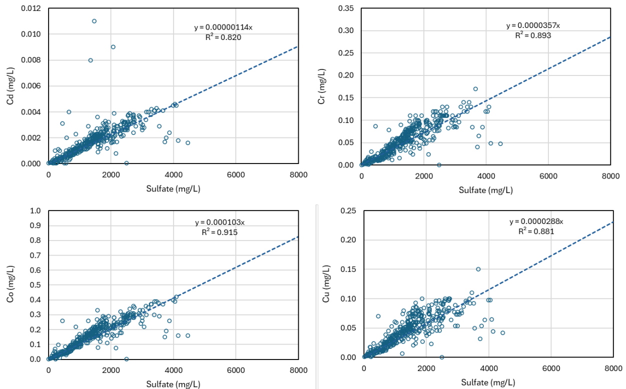
Figure 34: S23 Sulfate versus PCOC: Cd, Cr, Co, Cu. S23 data.
