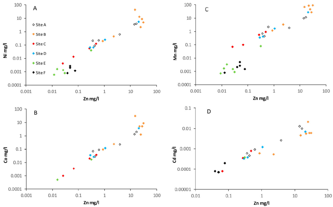
Figure 11: Zn versus trace element concentrations (Brunner Coal Measures).
