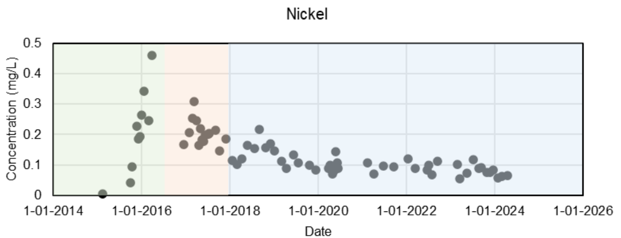
Figure 25: BV ELF Mn and Ni concentrations (February 2015 – April 2024).
