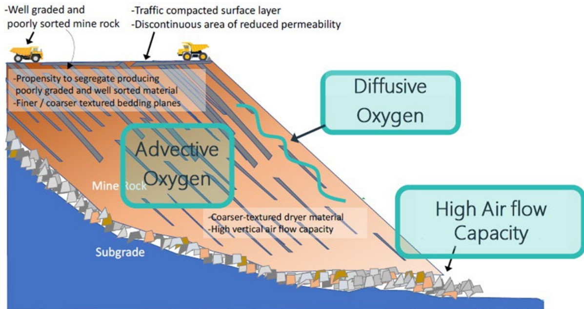
Figure 2. Advective air flow driven by grainsize segregation.
