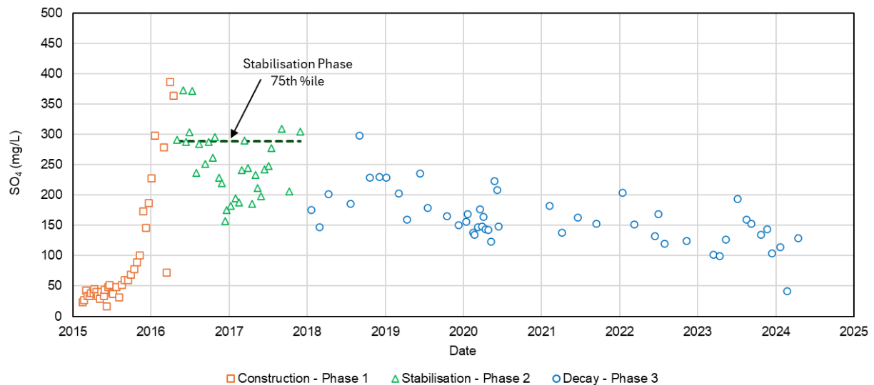
Figure 41. Derivation of SOX load from BV ELF sulfate data.
