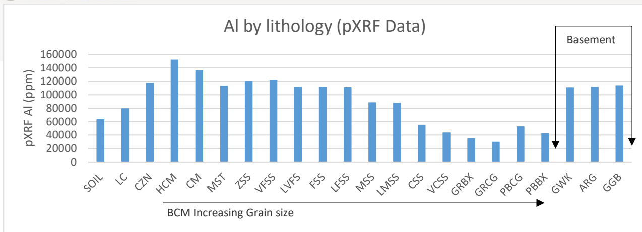
Figure 8. Aluminium concentration by logged sample lithology.
