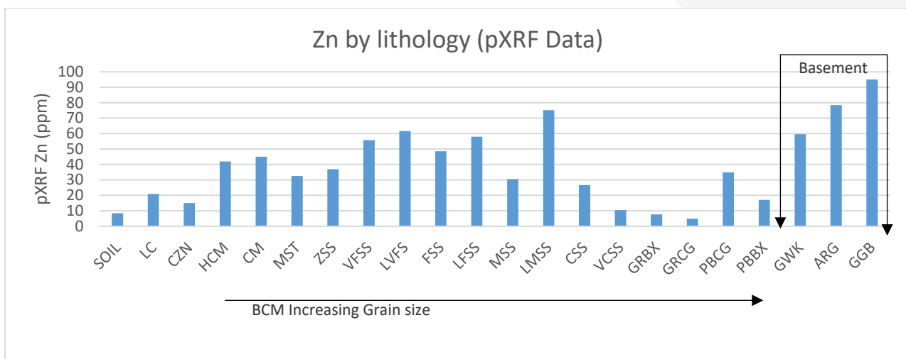
Figure 9. Zinc concentration by logged sample lithology.
