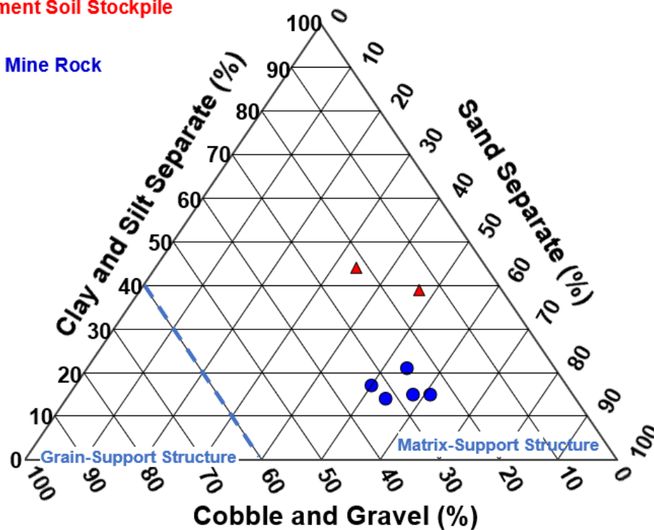
Figure 7: Textural triangle illustrating the texture of the mine rock and stockpile soil.
