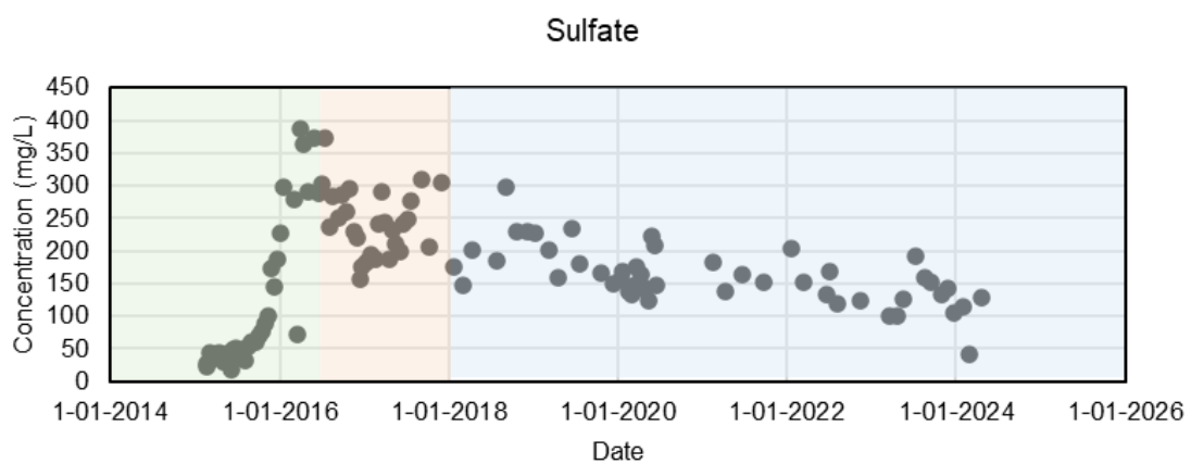
Figure 26. BV ELF Zn and SO 4 concentrations (February 2015 – April 2024).
