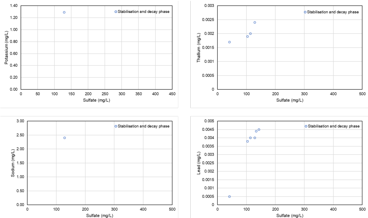
Figure 31: Sulfate versus PCOC: K, TI, Na, and Pb.
