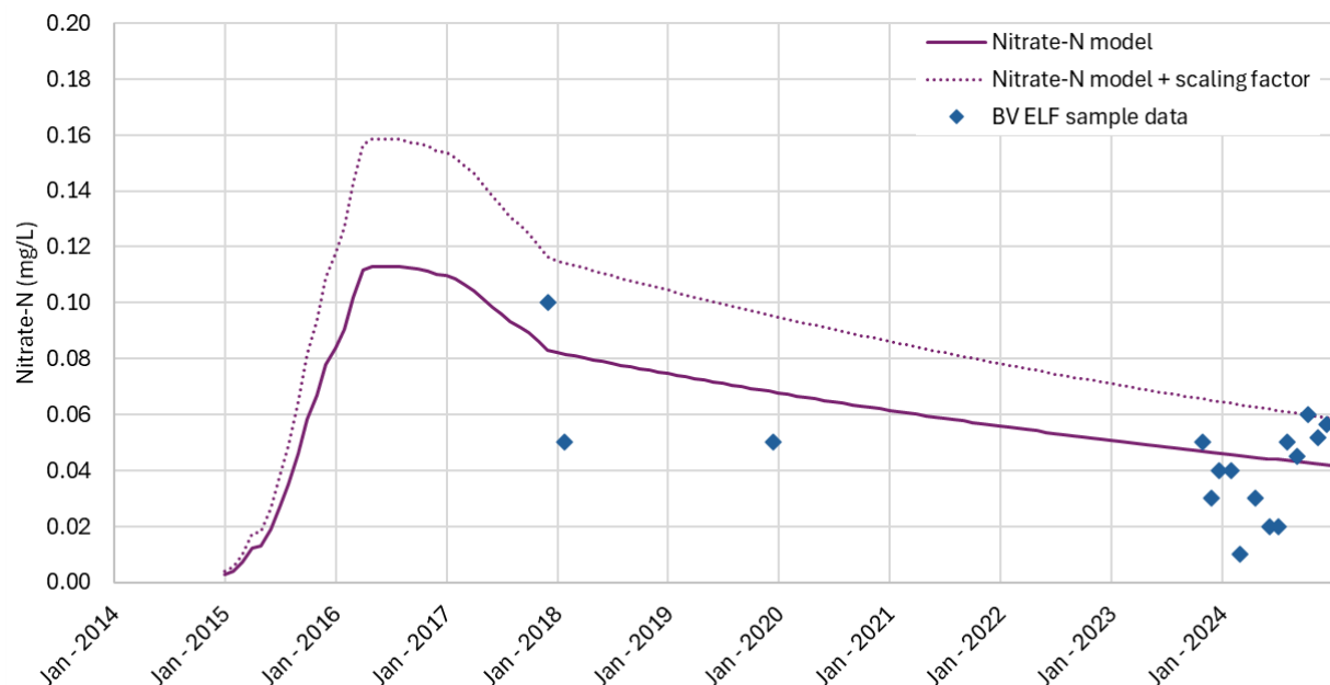
Figure 50. BV ELF nitrate-N model.
