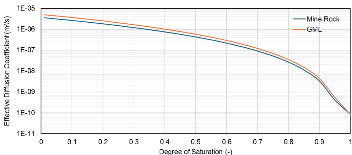
Figure 13: Oxygen diffusion functions for the growth medium and mine rock.
