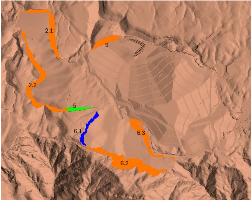
Figure 10: ESE closure highwall (Year 13).
