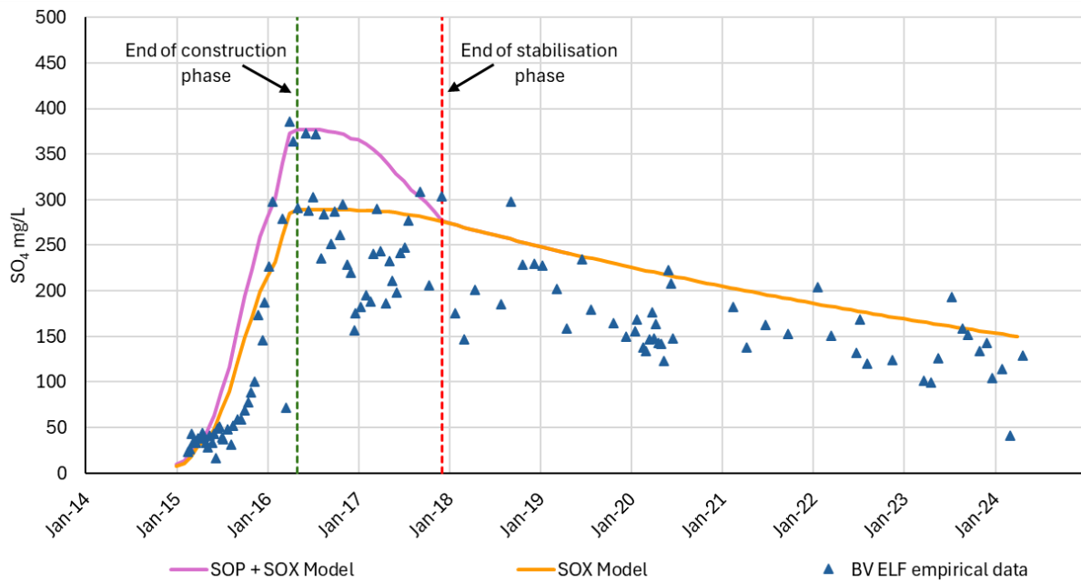
Figure 43. Calculated BV ELF load models and BV ELF sulfate data.
