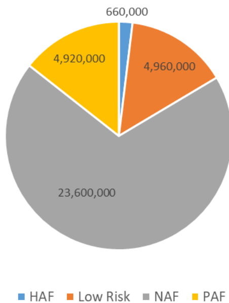
Figure 16. Relative tonnages of waste rock classified by the PFC. Labels show total rock tonnages.
