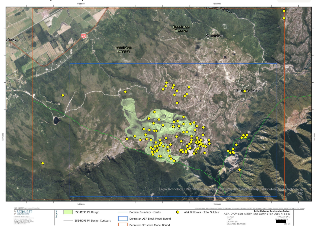
Figure 3 Sample spatial distribution for total sulphur results
