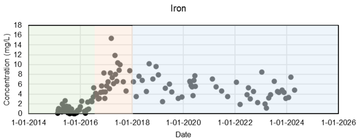
Figure 24: BV ELF Al and Fe concentrations (February 2015 – April 2024).
