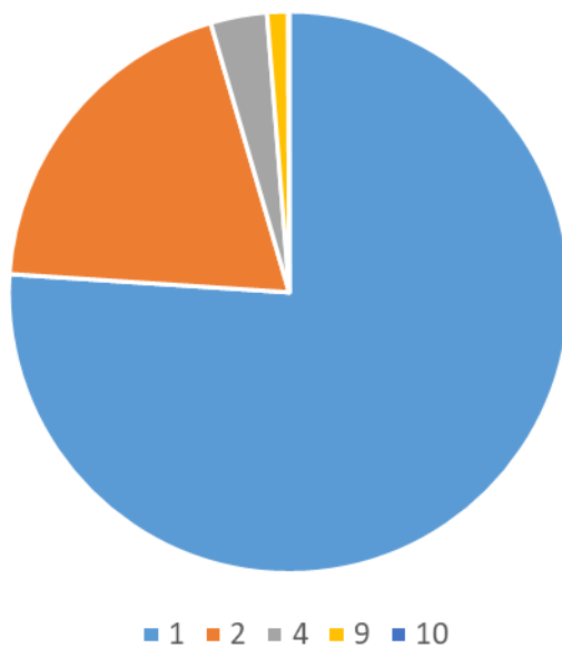
Figure 17. Confidence in the estimation of ABA parameters and subsequent ABA classification. The lower the confidence value, the higher the confidence with the classification.
