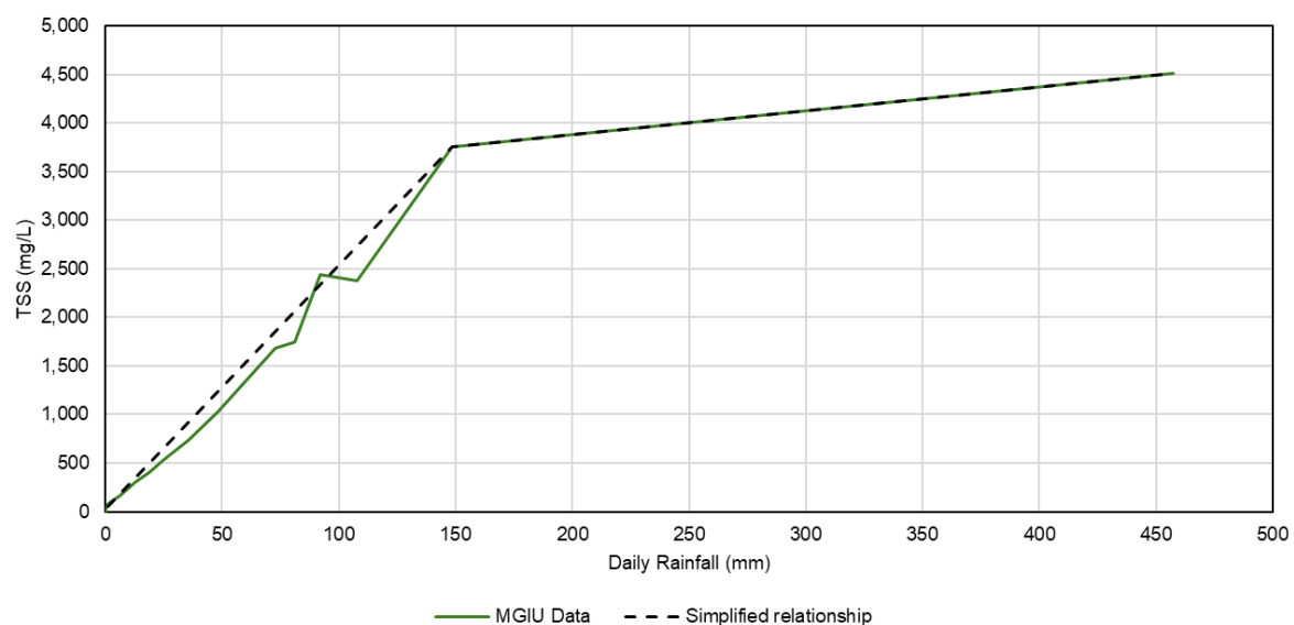
Figure 25: Mine impacted TSS relationship for use in WLBMs.
