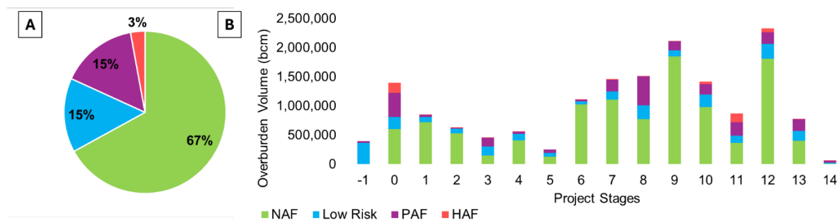
Figure 2: MFS overburden summary based on AMD classification
