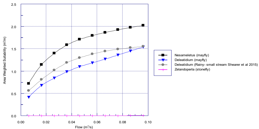
Figure 3: Predicted habitat for Deleatidium , Nesameletus , and Zealandoperla at Site DC3 with changing flow.
