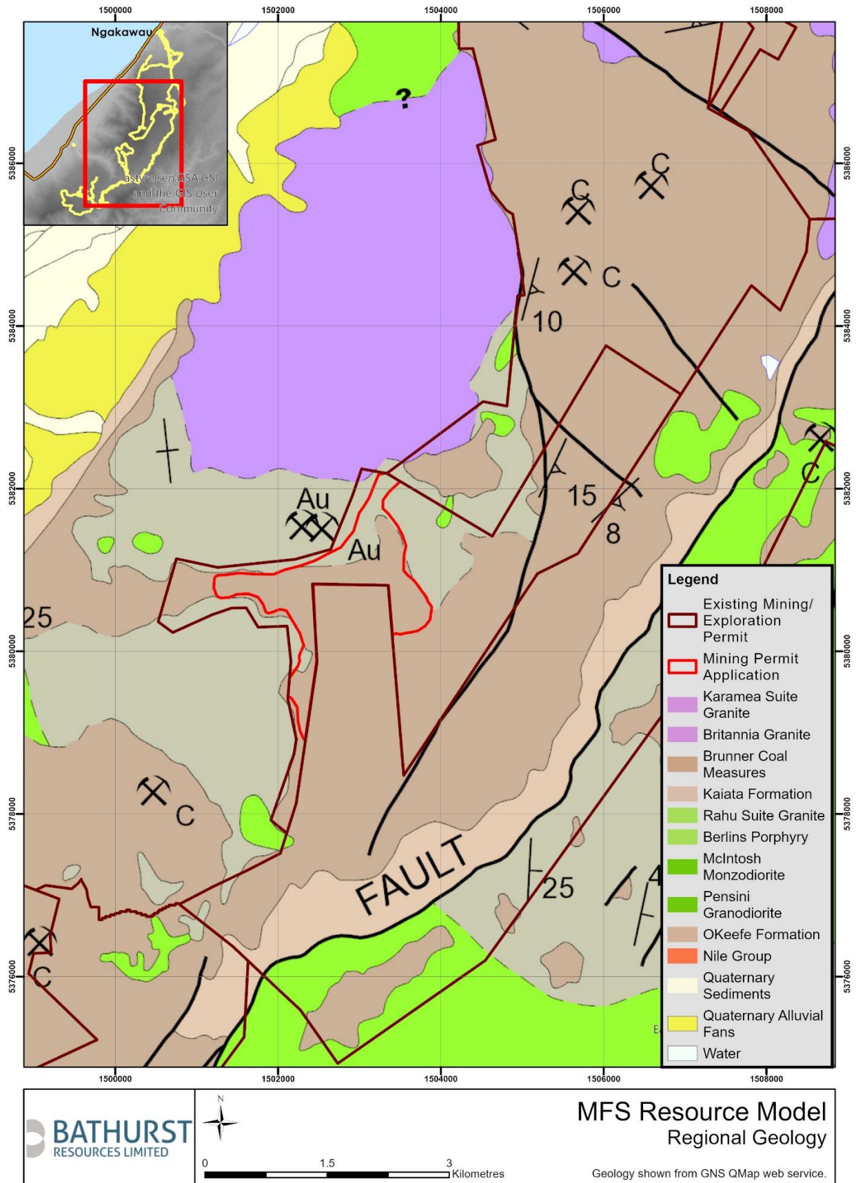
Figure 6: QMap Regional Geology
