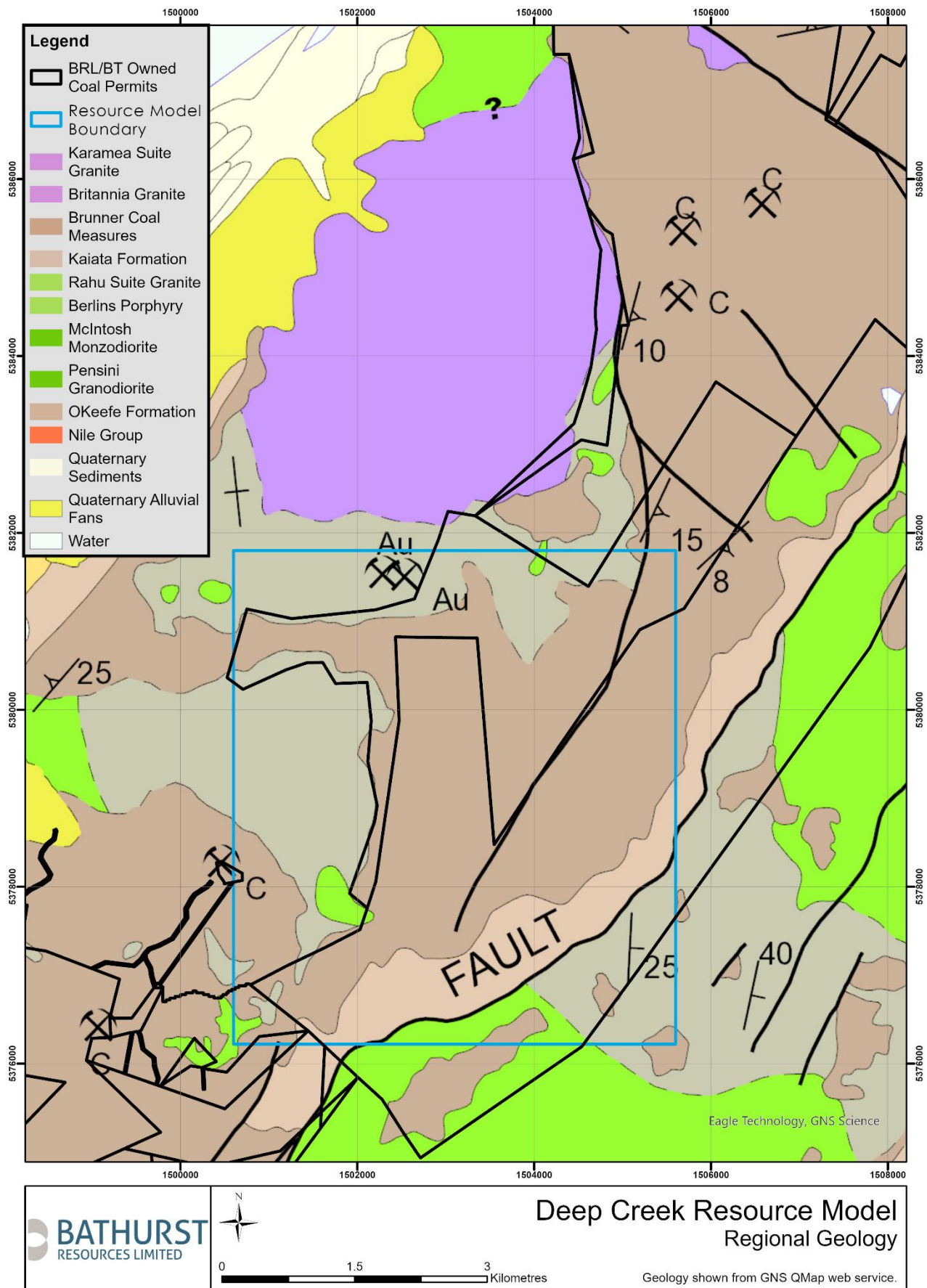
Figure 4: Regional Geology
