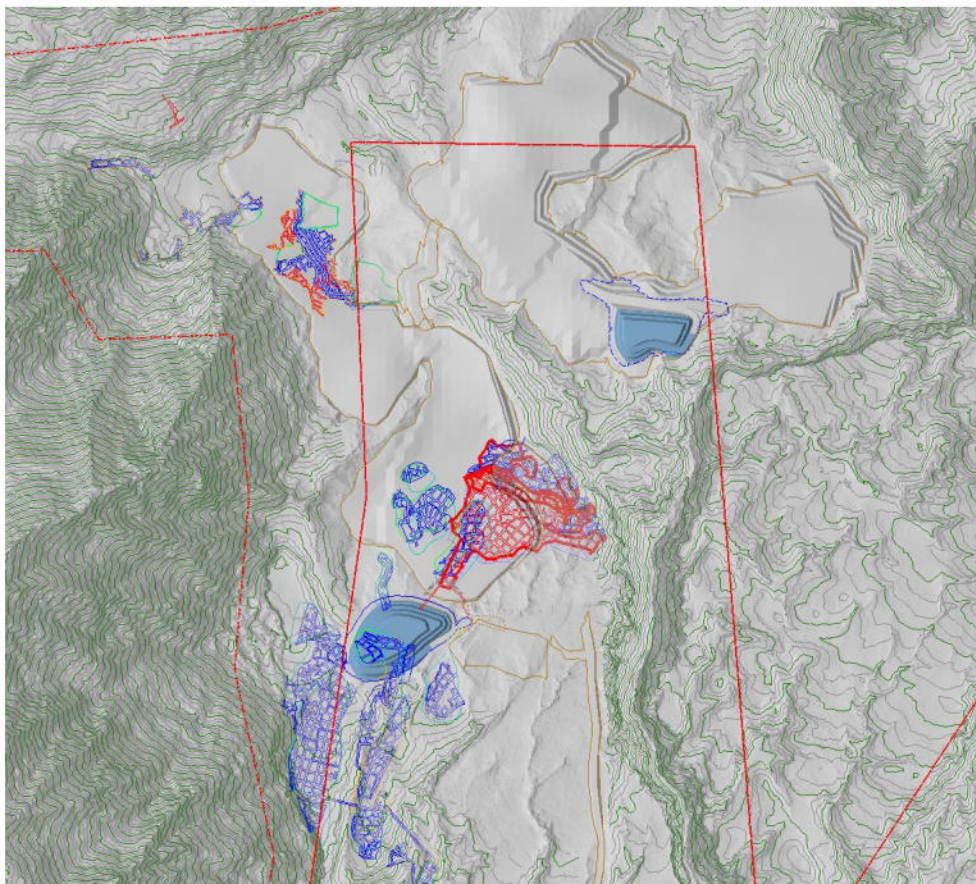
Figure 27: Mount Frederick South Pit plan with previous underground workings
