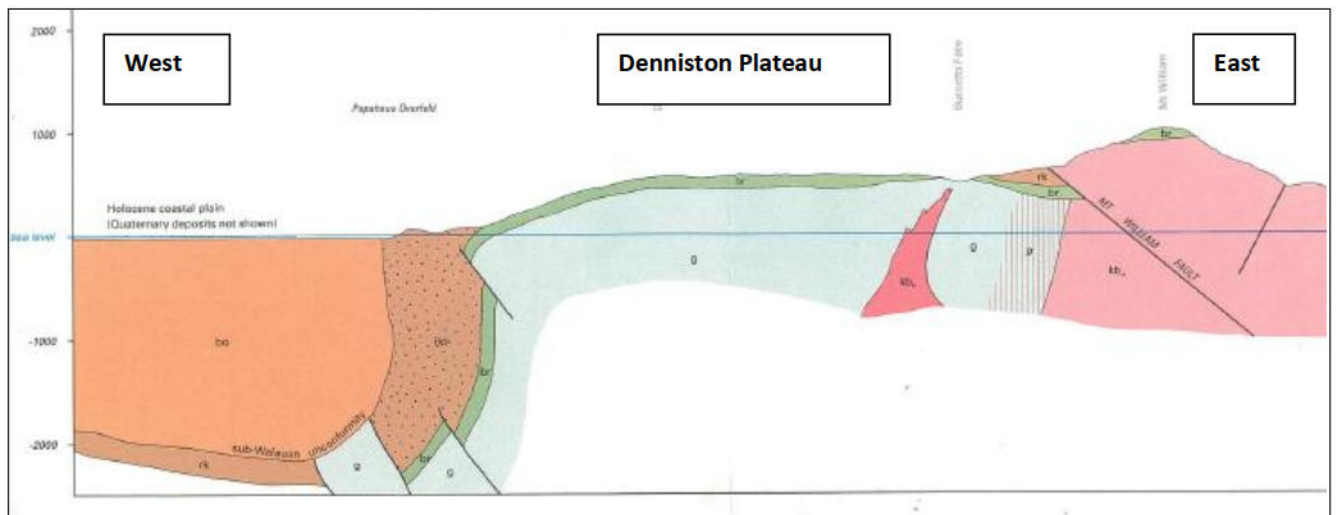
Figure 7: Geological cross section (Nathan, 1996)
