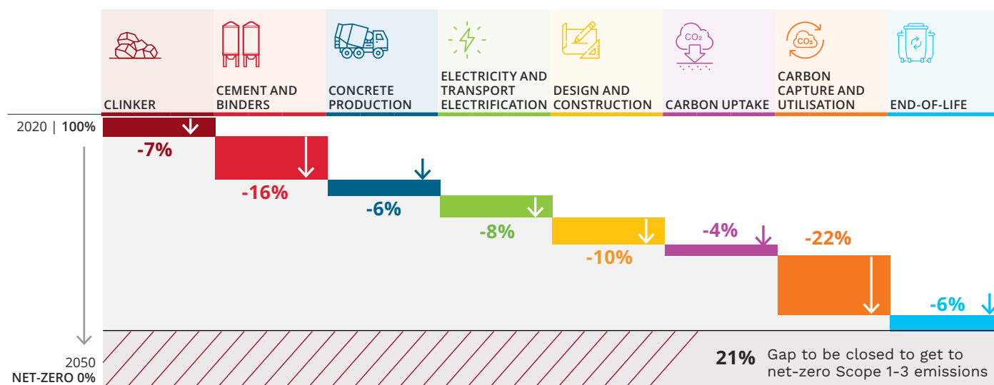
Figure 8. Decarbonisation roadmap of cement and concrete in Aotearoa New Zealand (EPD analysis)
