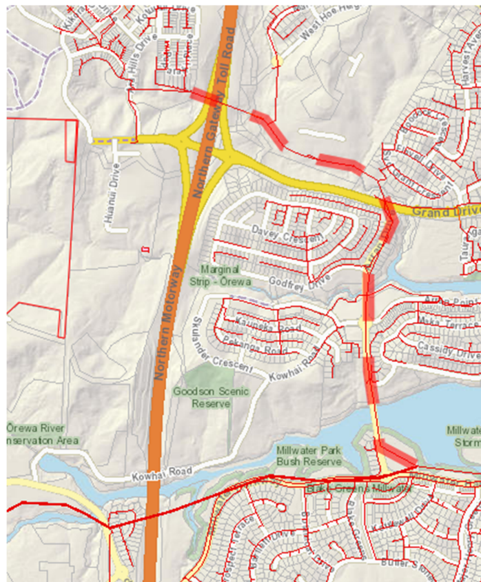
Figure 3 - Route along which pipe capacity has been analysed
