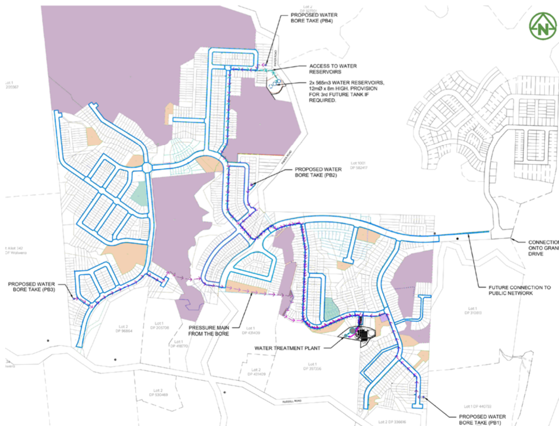
Figure 7 Proposed layout for Stage 1 & 2
