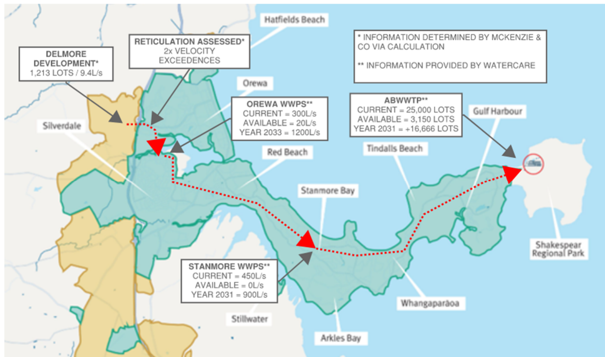
Figure 6 Visualisation of wastewater capacity assessment
