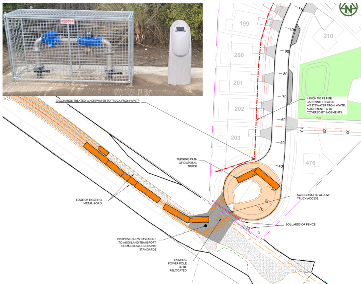
Figure 4 LPS and WWTP
