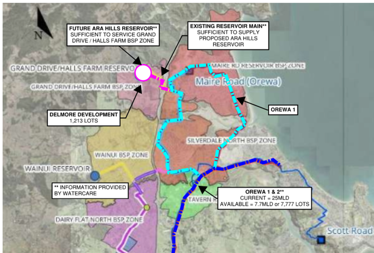
Figure 9 Visualisation of water capacity assessment
