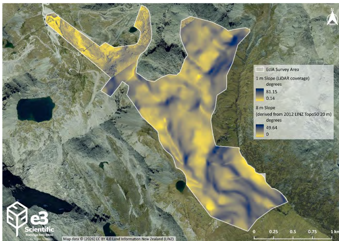
Figure 4: Slope analysis.
