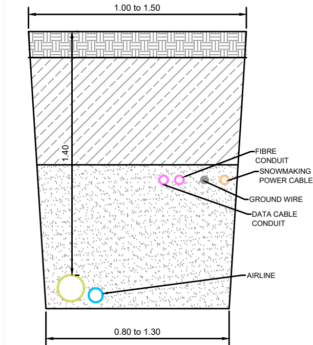
SNOWMAKING TRENCH DETAIL (TRENCH TYPE 4)
