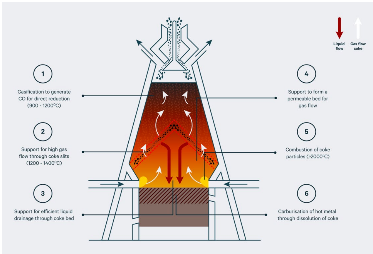
Figure 8: The Role of Coke in a Blast Furnace
