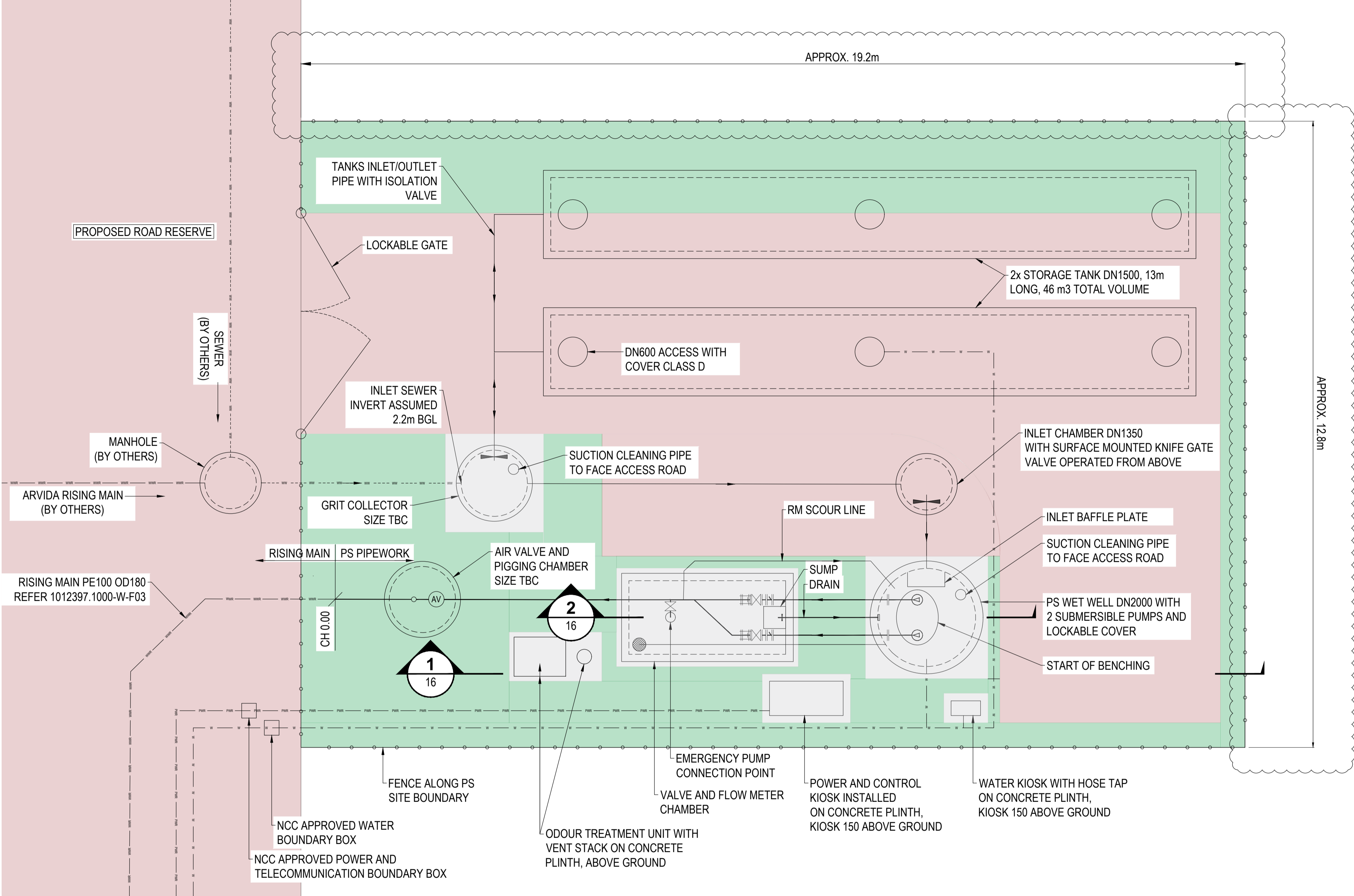
PUMP STATION AND STORAGE TANKS - PLAN 1:50 (A1)
