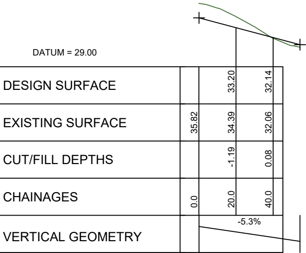
LONGITUDINAL SECTION JOAL EXTRA 1 SCALE HORIZ=1:2000 @ A1 VERT=1:400 @ A1
