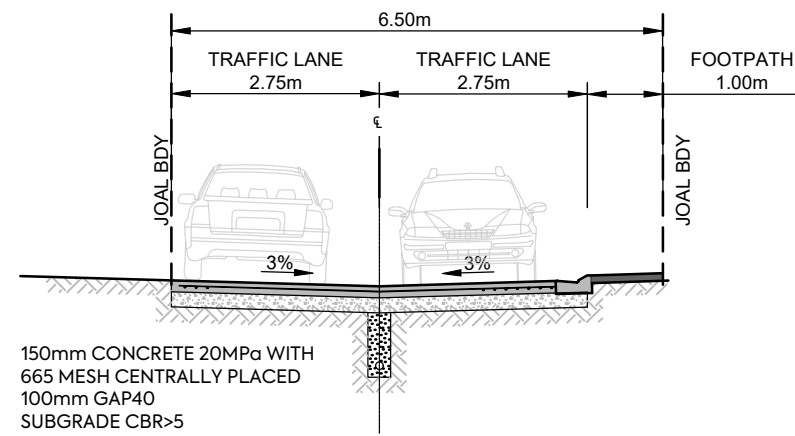
JOAL 30 6.5m JOAL, FOOTPATH ON REAR LOT SIDE SCALE 1:100 @A3
