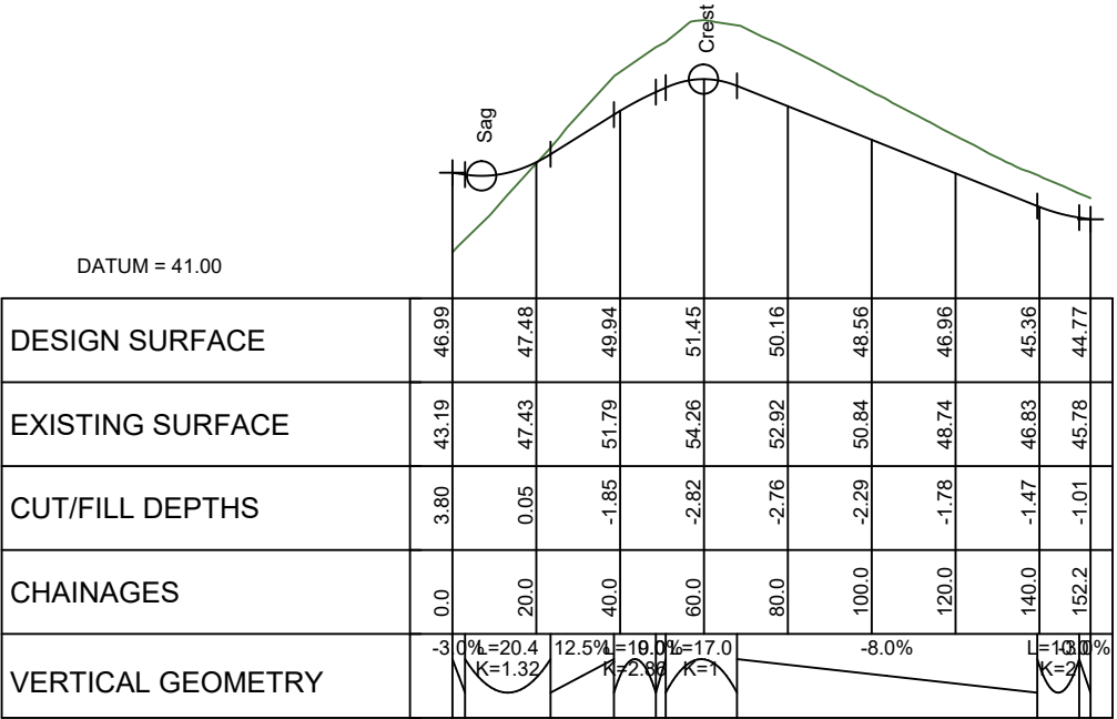
LONGITUDINAL SECTION JOAL 13 SCALE HORIZ=1:2000 @ A1 VERT=1:400 @ A1
