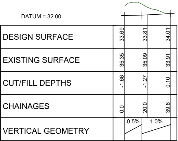
LONGITUDINAL SECTION JOAL 40a SCALE HORIZ=1:2000 @ A1 VERT=1:400 @ A1
