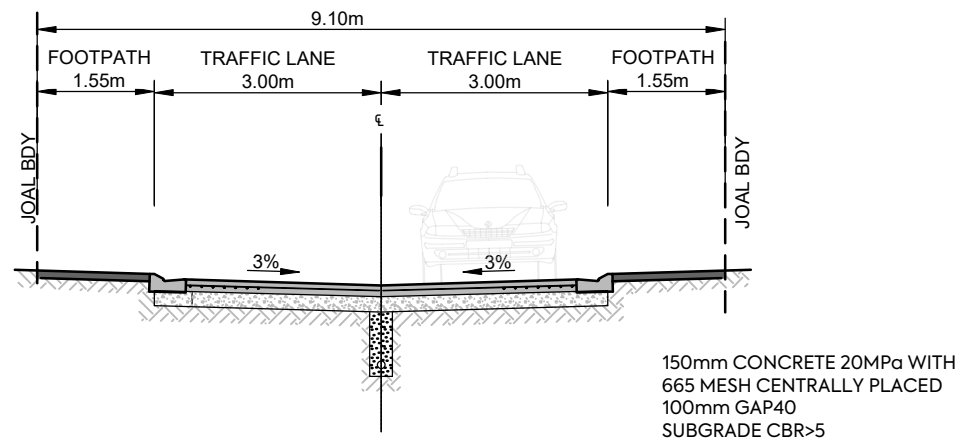
JOAL 40A 9.1m JOAL, 6.0m FORMED WIDTH SCALE 1:100 @A3
