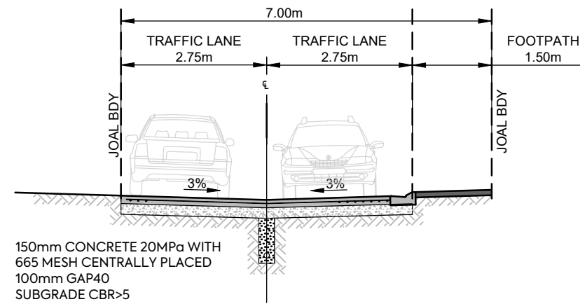
JOAL 11 7.0m JOAL, FOOTPATH ON REAR LOT SIDE SCALE 1:100 @A3
