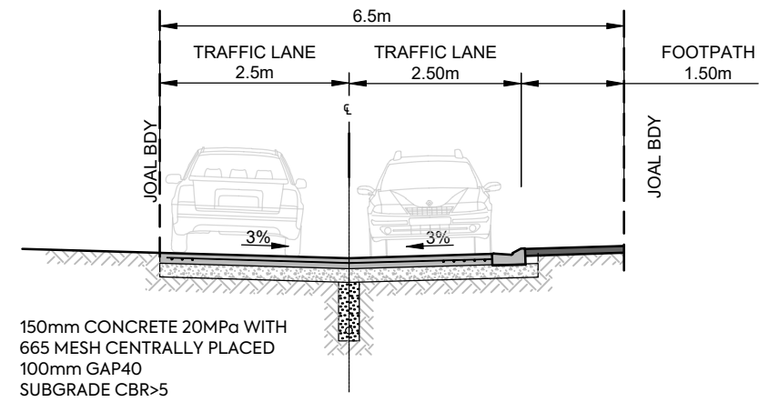
JOAL 2, 6, 8, 10 6.5m JOAL, FOOTPATH ON REAR LOT SIDE SCALE 1:100 @A3
