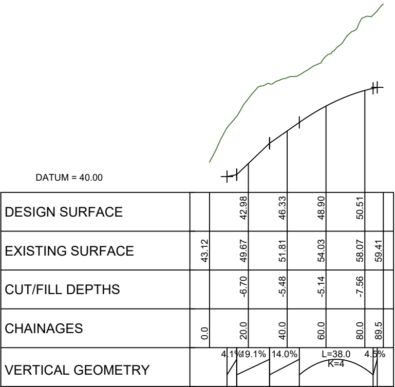
LONGITUDINAL SECTION JOAL02 SCALE HORIZ=1:2000 @ A1 VERT=1:400 @ A1
