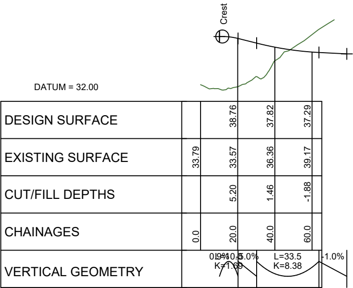
LONGITUDINAL SECTION JOAL 34 SCALE HORIZ=1:2000 @ A1 VERT=1:400 @ A1
