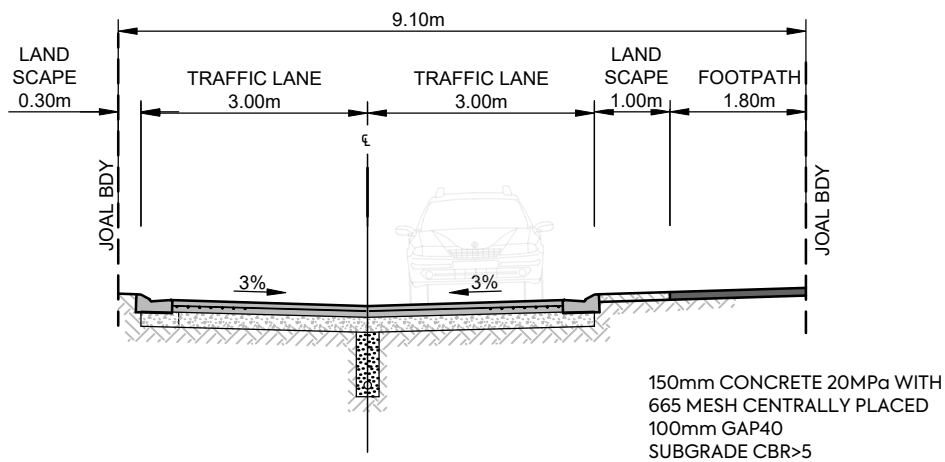
JOAL 40, 5b 9.1m JOAL, 6.0m FORMED WIDTH SCALE 1:100 @A3
