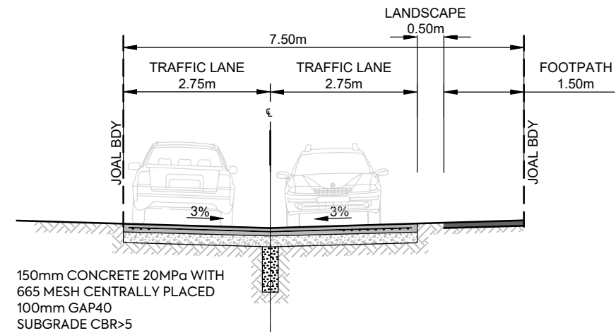
JOAL 4B 7.5m JOAL, FOOTPATH ON REAR LOT SIDE SCALE 1:100 @A3
