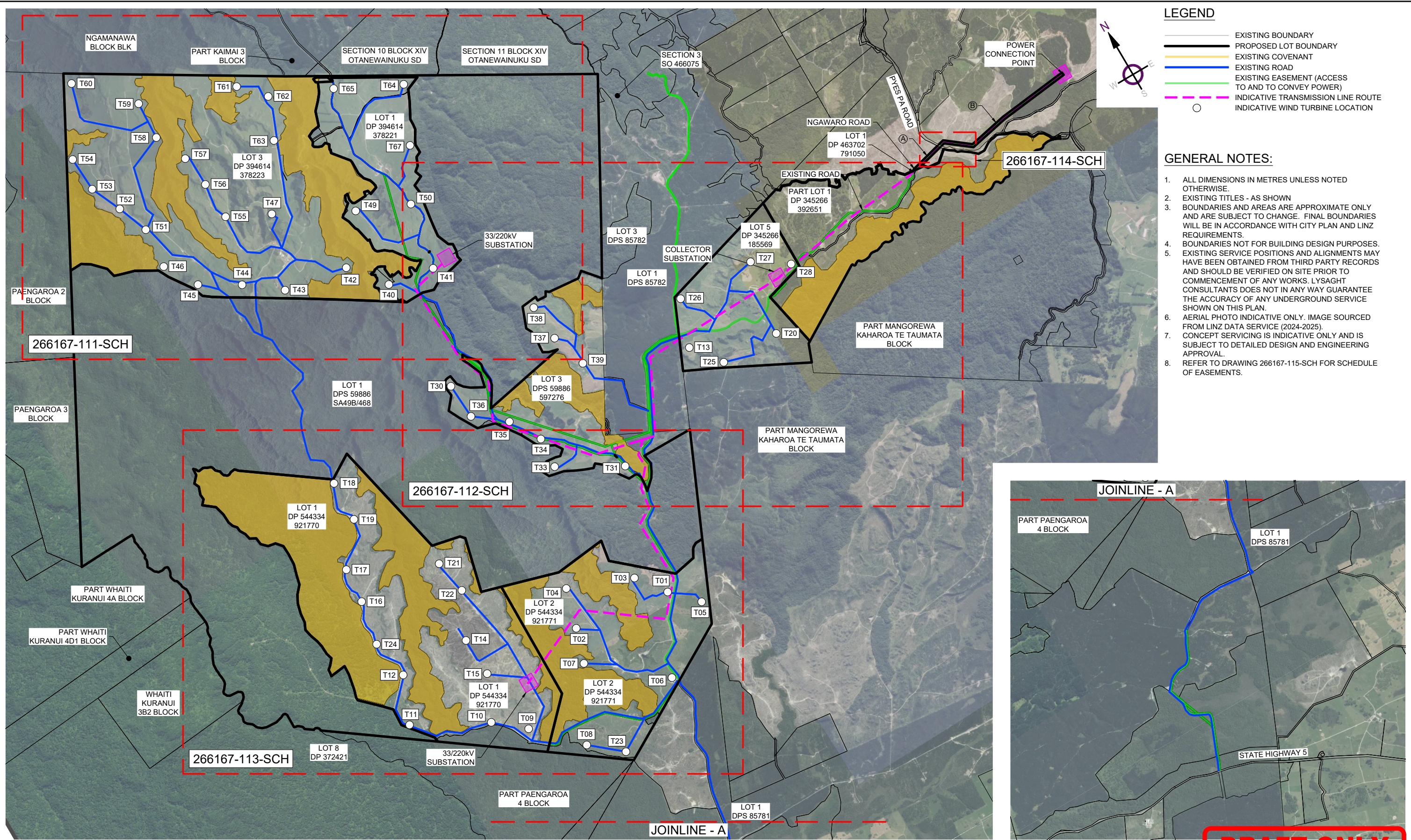
OVERALL LAYOUT PLAN SCALE 1:50000
