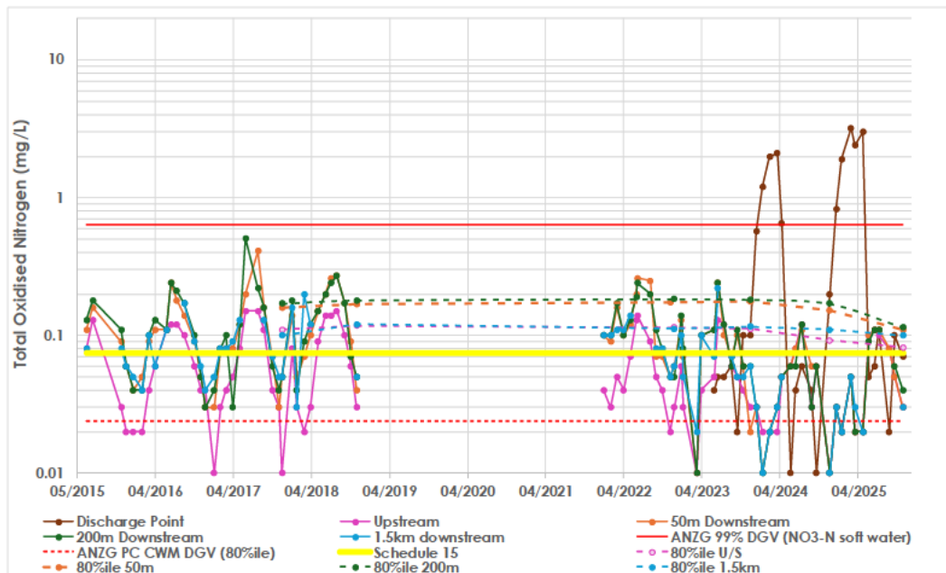
Figure 6-2: Total Oxidised Nitrogen (Nitrate) Compliance Monitoring Results.
