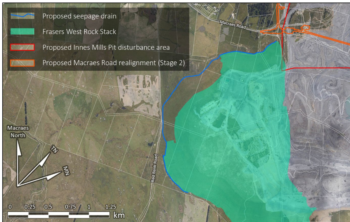
Figure 2. Seepage drain extent around the around Frasers West Waste Rock Stack.
