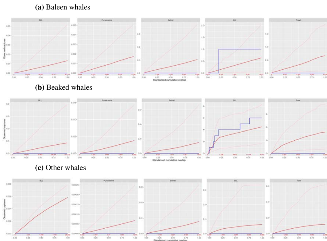
Figure 38: Cumulative number of observed captures vs. species group overlap, for each whale species group and fishing method using seasonal occurrence probability distribution layers for some species. The expected values predicted from the model (thick red line) and 90% credible interval (thin red lines) are also presented for reference.
