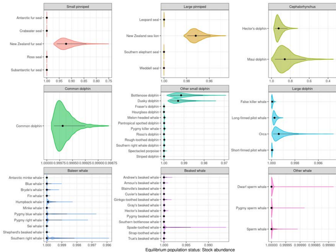
Figure 48: Predicted equilibrium status ( I'_s ) using stock population size, Model M_\bullet , mean annual commercial effort from 2016/17 to 2018/19, and other defined input parameters. Violin plots represent the central 99% of the approximated posterior distribution, and black dots and error bars are the posterior median and central 90% credible interval. Separate panels are presented for each species group.
