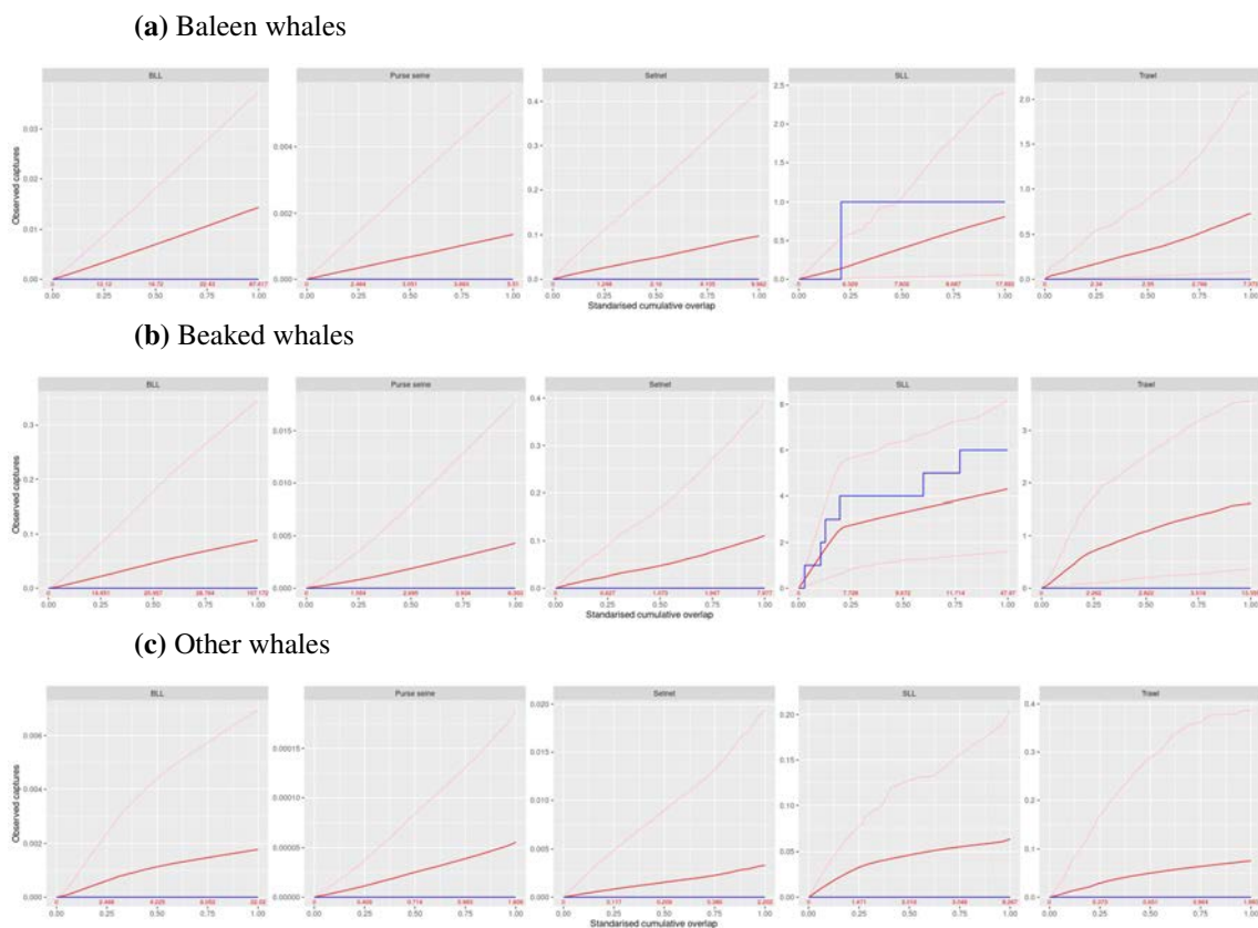
Figure 28: Cumulative number of observed captures vs. species group overlap, for each whale species group and fishing method. The expected values predicted from the model (thick red line) and 90% credible interval (thin red lines) are also presented for reference.
