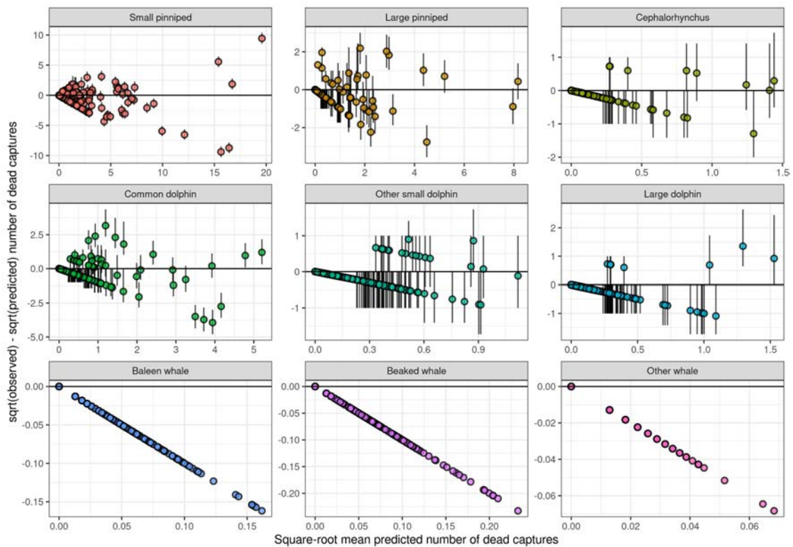
Figure 25: Difference between actual and predicted number of observed dead captures from M_{\bullet} (i.e., residuals), for each unique summarised data input (i.e., species group \times fishing group \times fishing month). The square root of the number of captures has been calculated prior to taking the difference.
