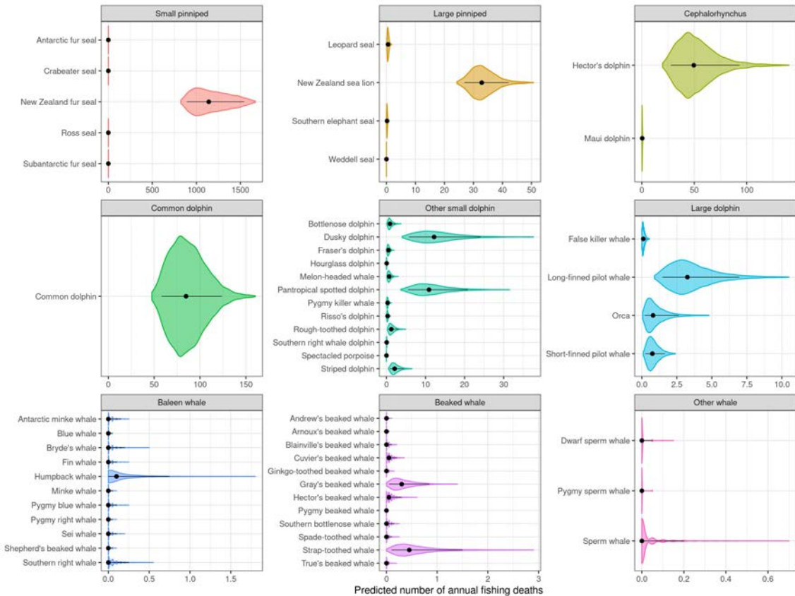
Figure 45: Predicted number of expect annual deaths of each species ( D_s ) using Model M_\bullet , mean annual commercial effort from 2016/17 to 2018/19, and other defined input parameters. Violin plots represent the central 99% of the approximated posterior distribution, and black dots and error bars are the posterior median and central 90% credible interval. Separate panels are presented for each species group.
