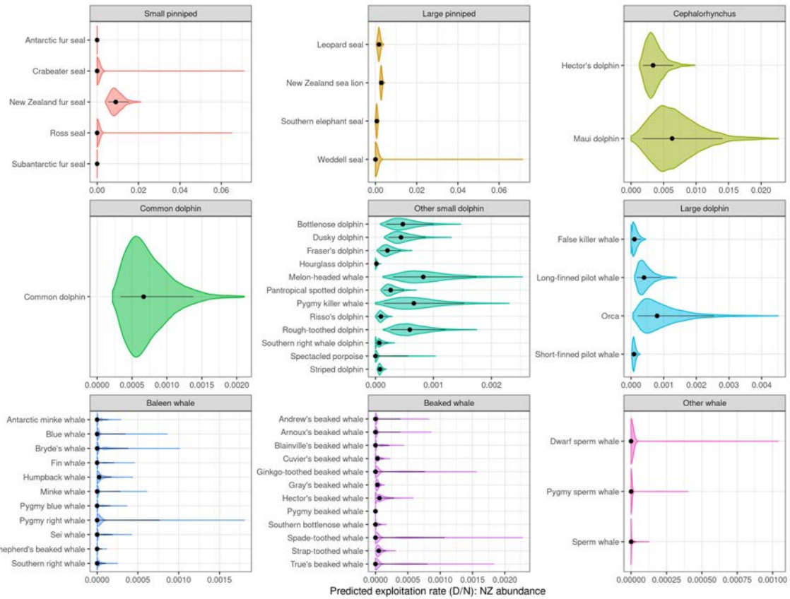
Figure 47: Predicted exploitation rate for each species ( U_s = D_s/N_s ) using NZ population size, Model M_e , mean annual commercial effort from 2016/17 to 2018/19, and other defined input parameters. Violin plots represent the central 99% of the approximated posterior distribution, and black dots and error bars are the posterior median and central 90% credible interval. Separate panels are presented for each species group.
