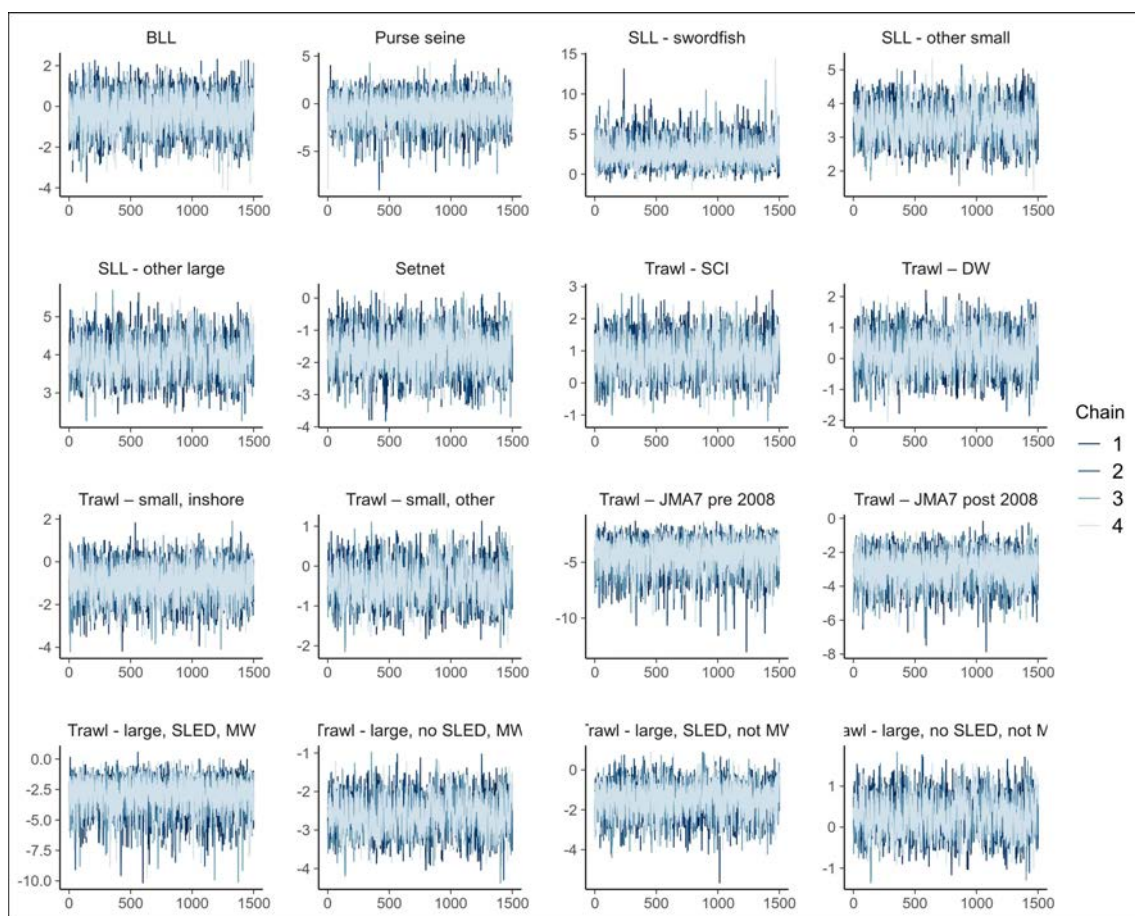
Figure C.5: Traceplot of fishing group live capture terms
