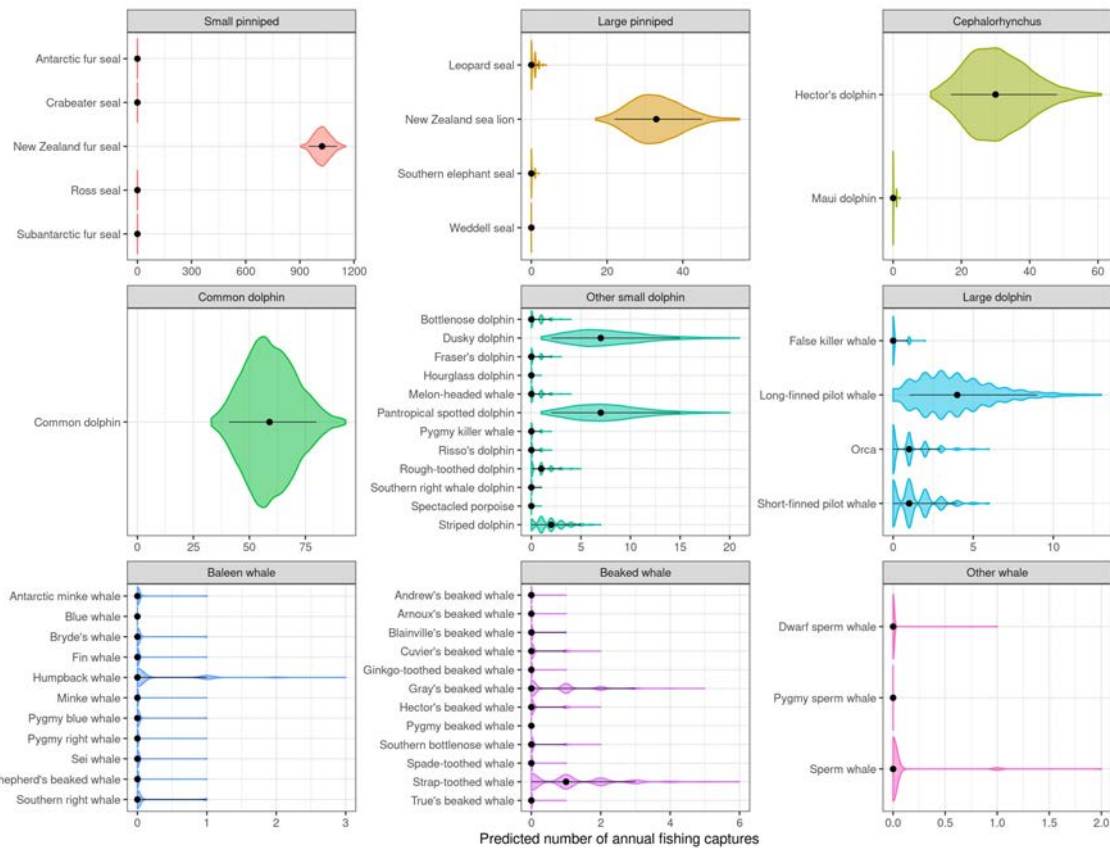
Figure 44: Predicted number of expected annual observable captures of each species ( C_s ) using Model M_{\bullet} , mean annual commercial effort from 2016/17 to 2018/19, and other defined input parameters. Violin plots represent the central 99% of the approximated posterior distribution, and black dots and error bars are the posterior median and central 90% credible interval. Separate panels are presented for each species group.
