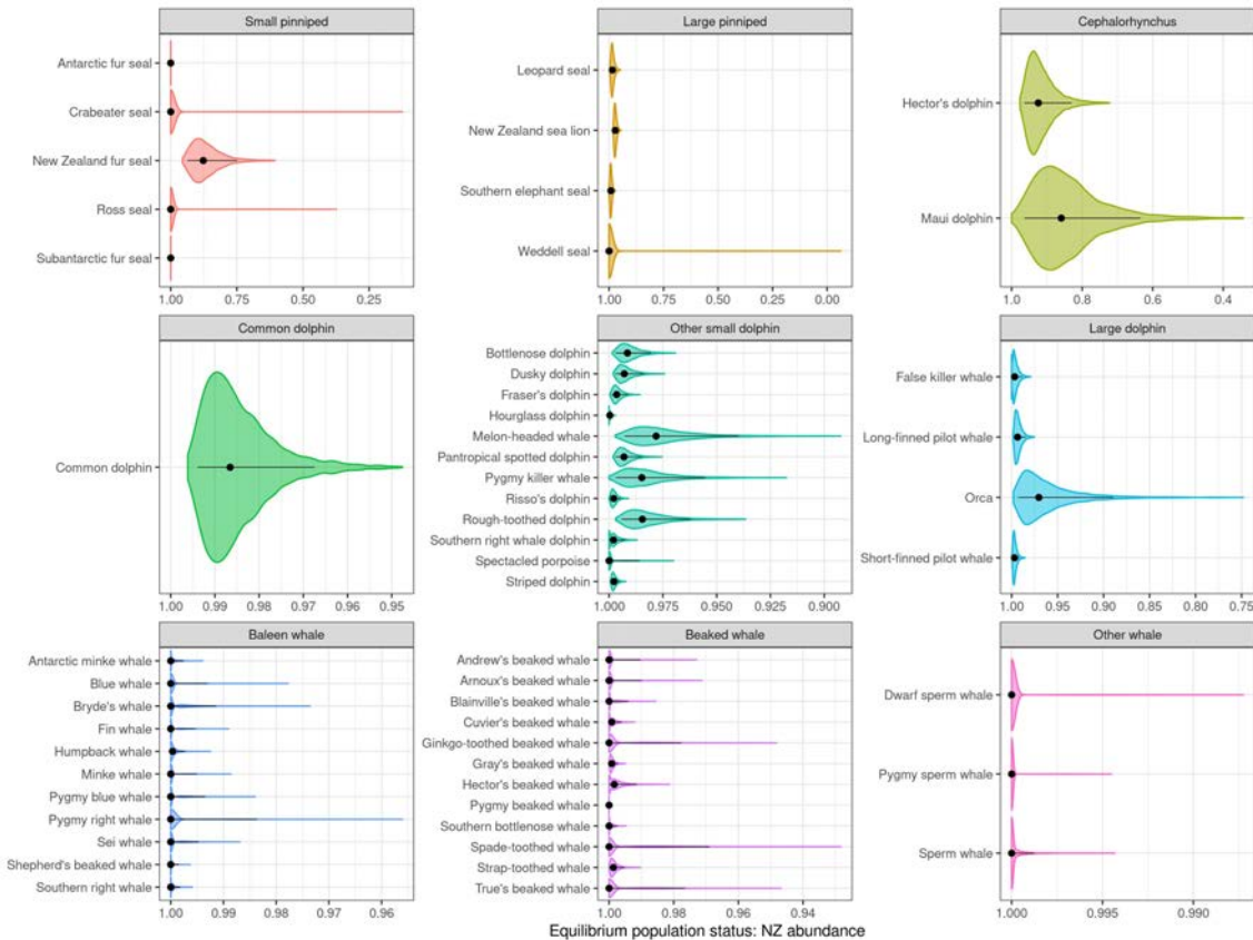
Figure 49: Predicted equilibrium status ( I'_s ) using New Zealand population size, Model M_{\bullet} , mean annual commercial effort from 2016/17 to 2018/19, and other defined input parameters. Violin plots represent the central 99% of the approximated posterior distribution, and black dots and error bars are the posterior median and central 90% credible interval. Separate panels are presented for each species group.
