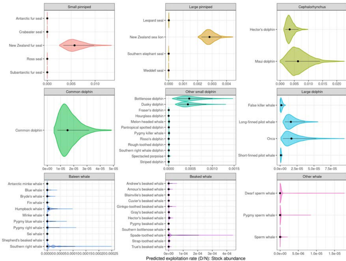
Figure 46: Predicted exploitation rate for each species ( U_s = D_s/N_s ) using stock population size, Model M_{\bullet} , mean annual commercial effort from 2016/17 to 2018/19, and other defined input parameters. Violin plots represent the central 99% of the approximated posterior distribution, and black dots and error bars are the posterior median and central 90% credible interval. Separate panels are presented for each species group.
