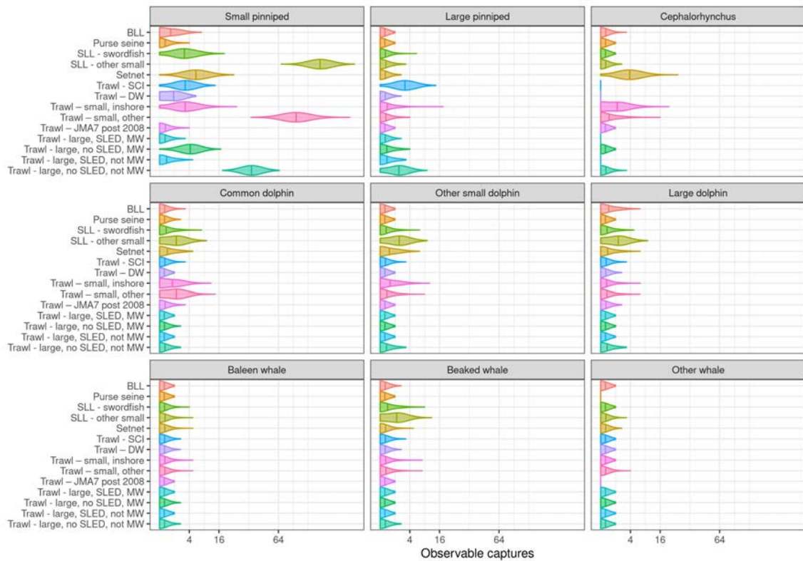
Figure 36: Posterior distribution for the number of observable live captures estimated using mean annual commercial effort from 2016/17 to 2018/19 by fishing group (as defined for M_{\bullet} ).
