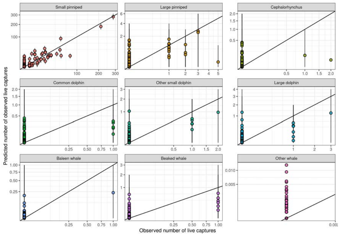
Figure 21: Actual vs. predicted number of observed live captures from M_{\bullet} , for each unique summarised data input record (i.e., species group \times fishing group \times fishing month). Axes are on square-root scale.
