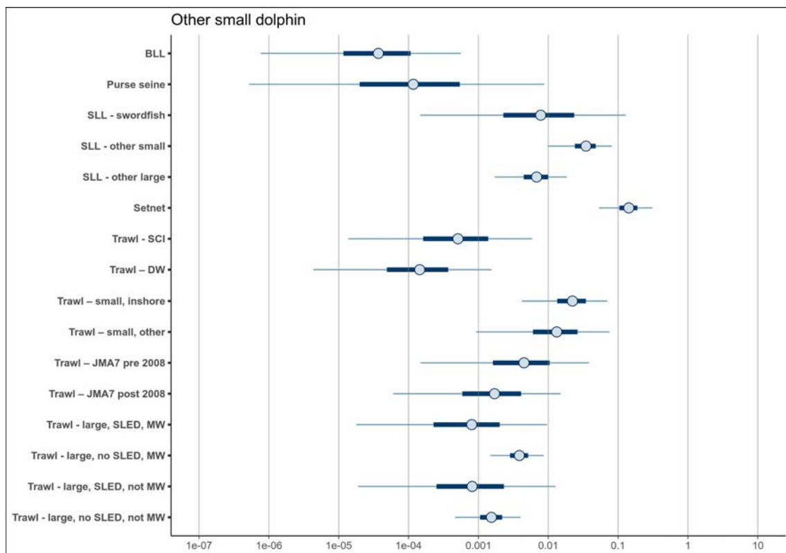
Figure 7: Posterior distribution of catchability ( q_{j,z} ) of other small dolphins in each fishing group as defined in M_{\bullet} . The posterior median, central 50 th and central 95 th quantiles of the distributions are presented.
