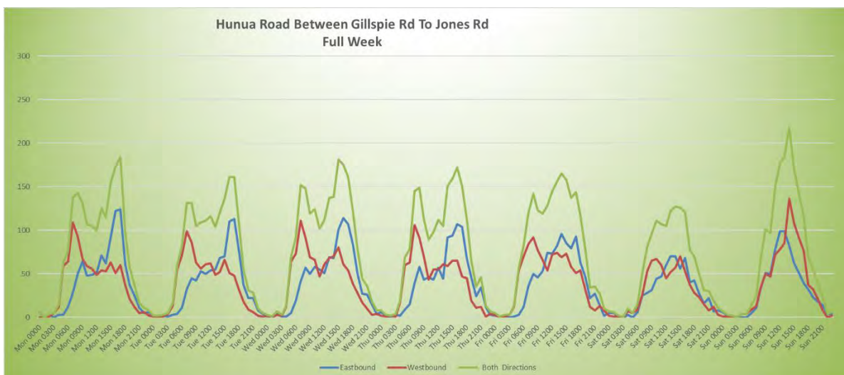
Figure 2-1: Traffic Volumes
