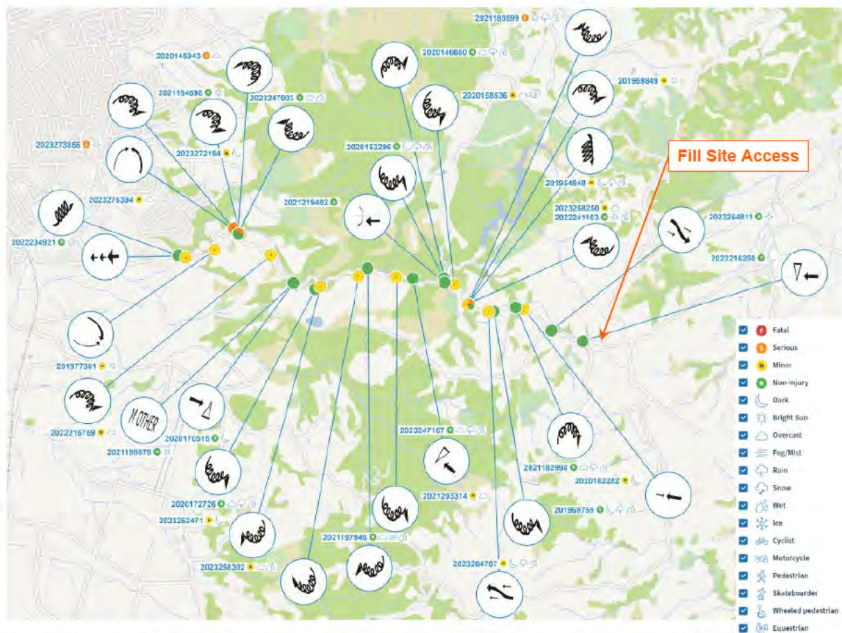
Figure 2-2: Collision Diagram
