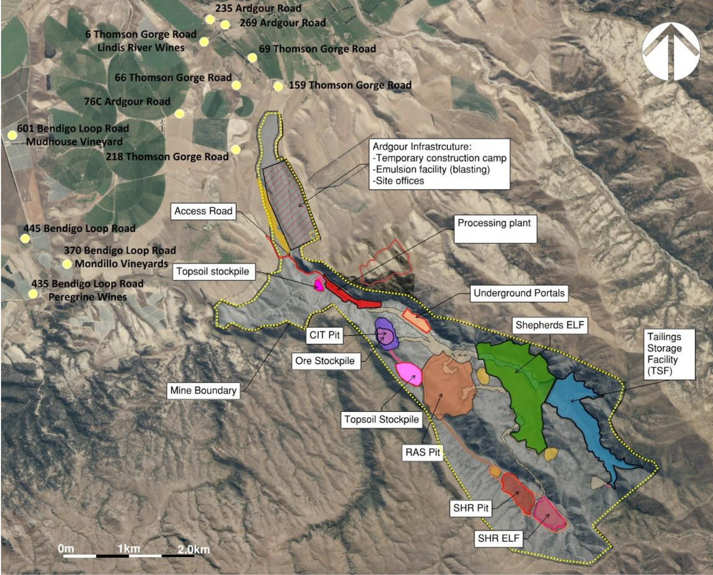
Figure 1: Proposed mine layout and nearest receivers
