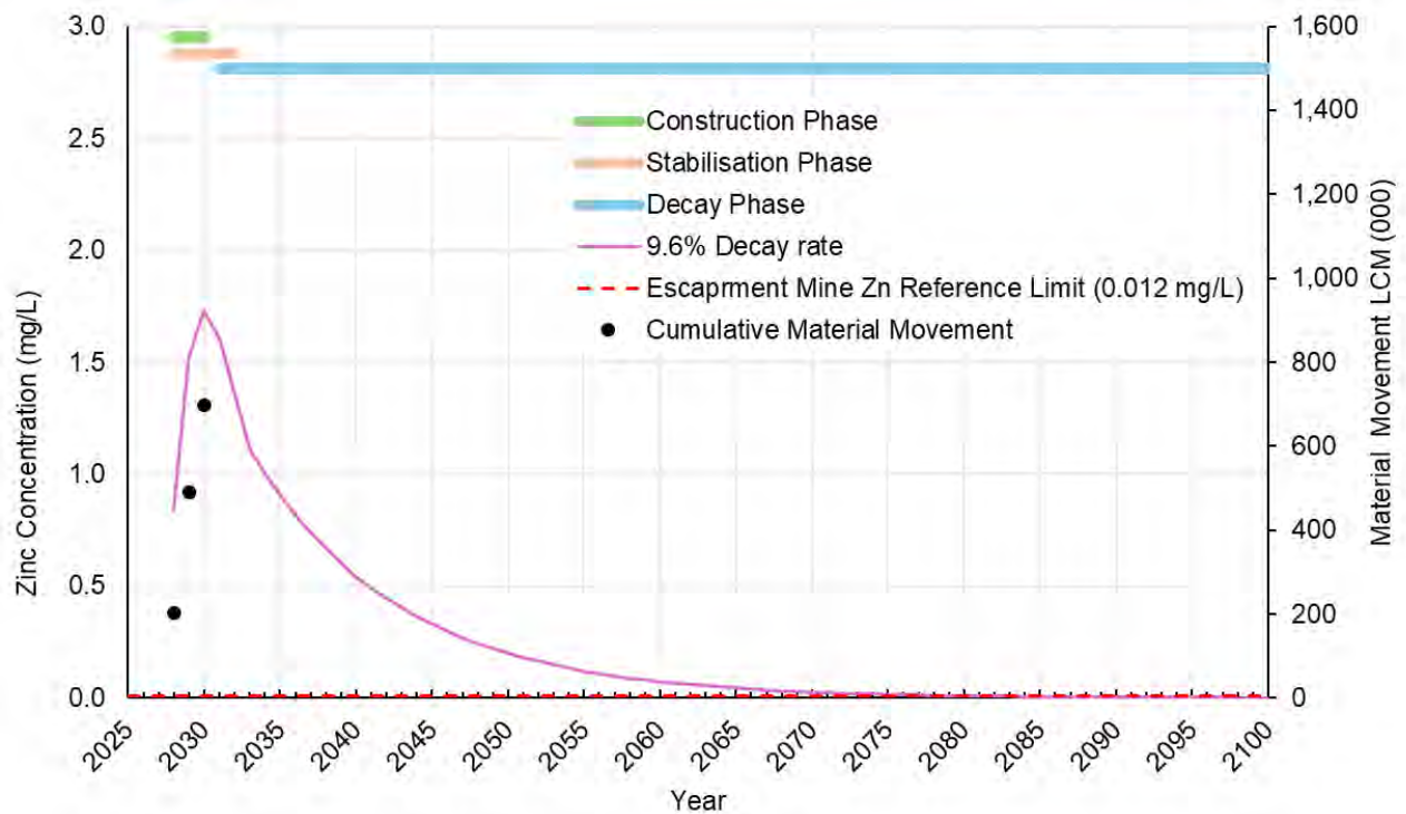
Figure 8: PPG ELF Zn decay.
