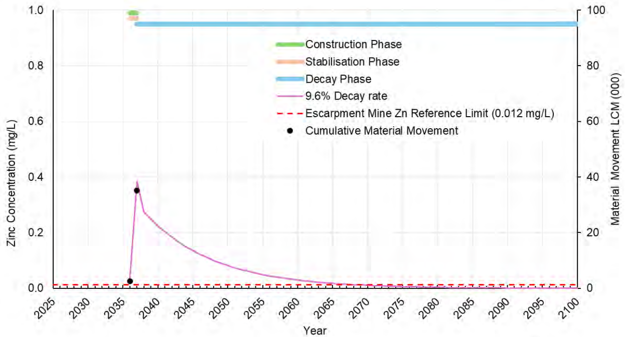
Figure 19: MDC2 ELF Zn decay.
