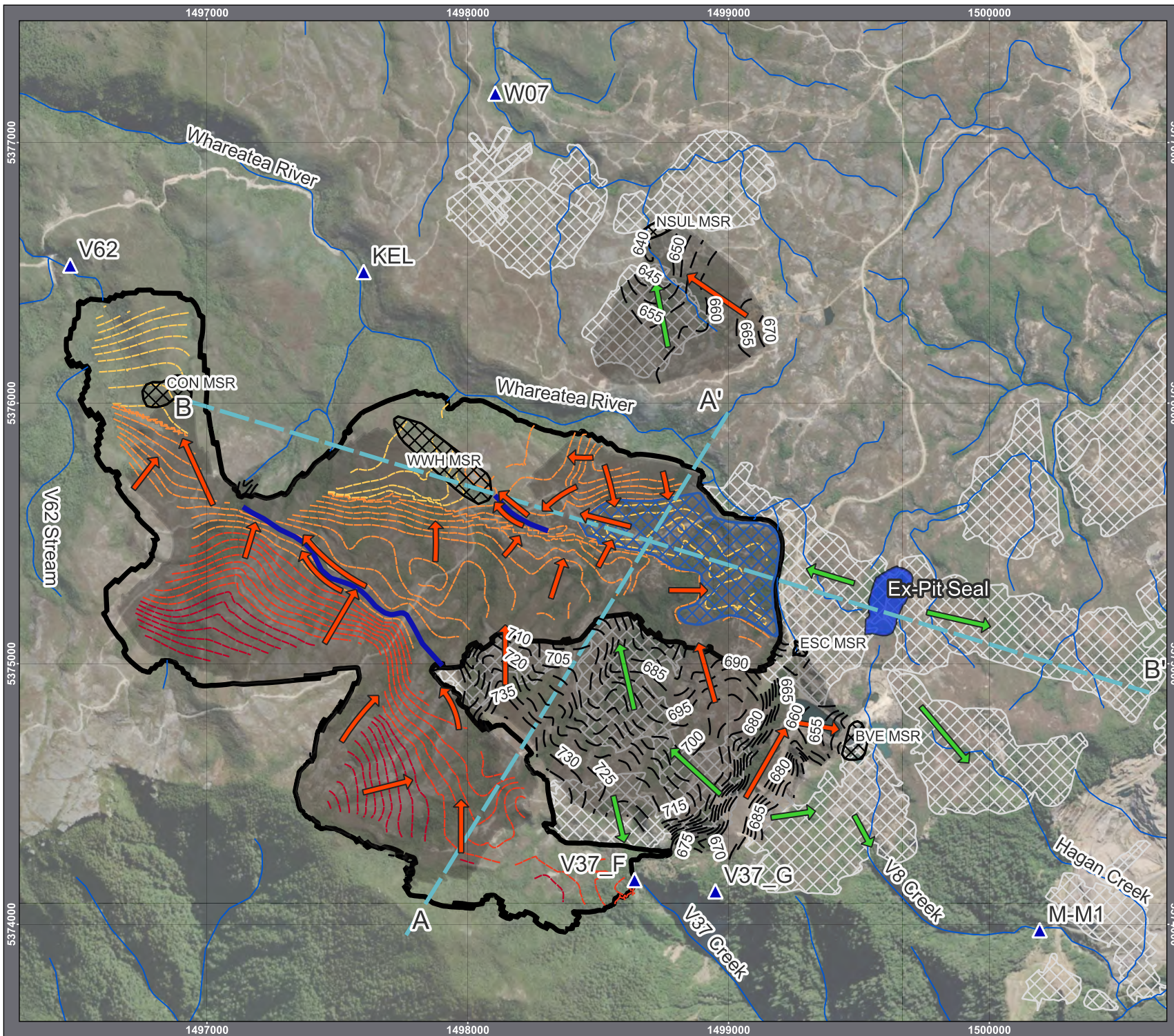
Figure 23: Post-closure Sub-ELF Seepage Flow Path Escarpment Extended Mine Project
