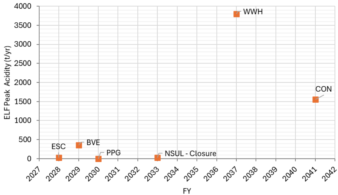
Figure 25: ESE peak ELF acidity loads
