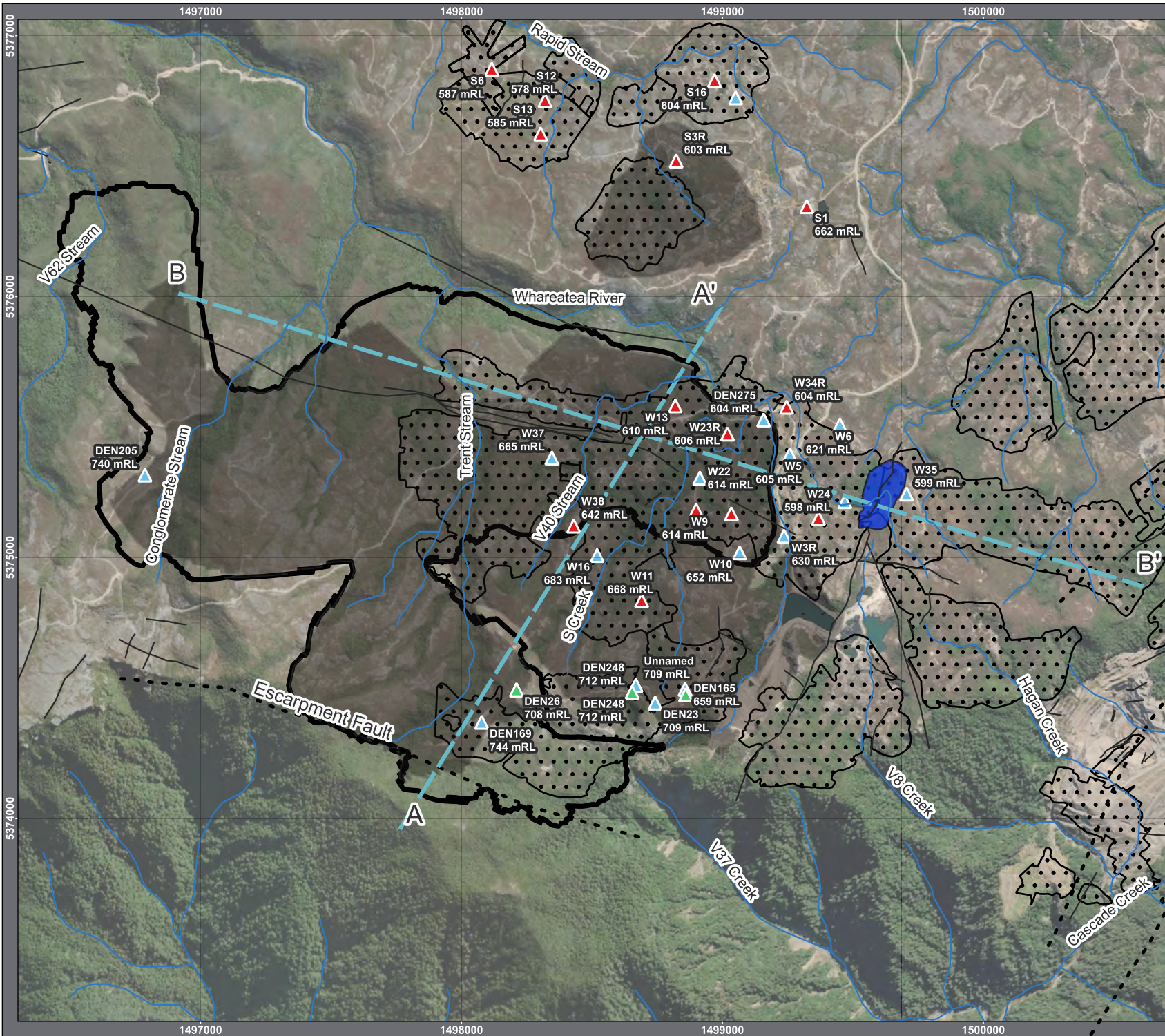
Figure 20: Cross Section Location Escarpment Extended Mine Project
