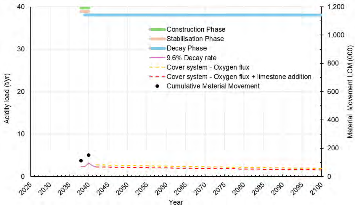
Figure 22: MSR10 ELF acidity decay.
