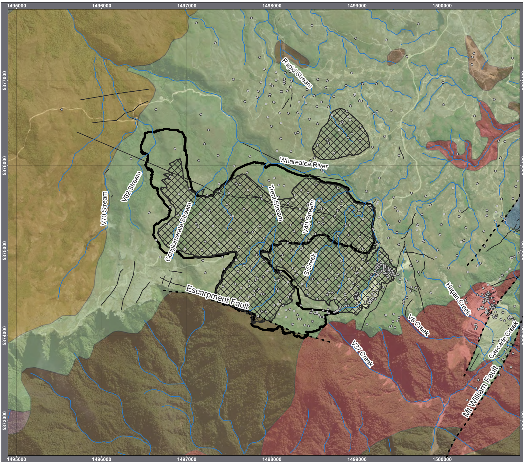
Figure 12: Site Geology and Faults Escarpment Extended Mine Project
