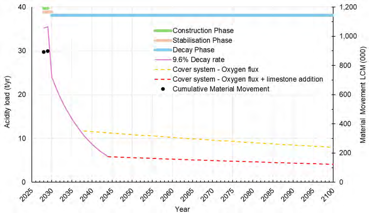
Figure 11: MSR1 ELF acidity decay.
