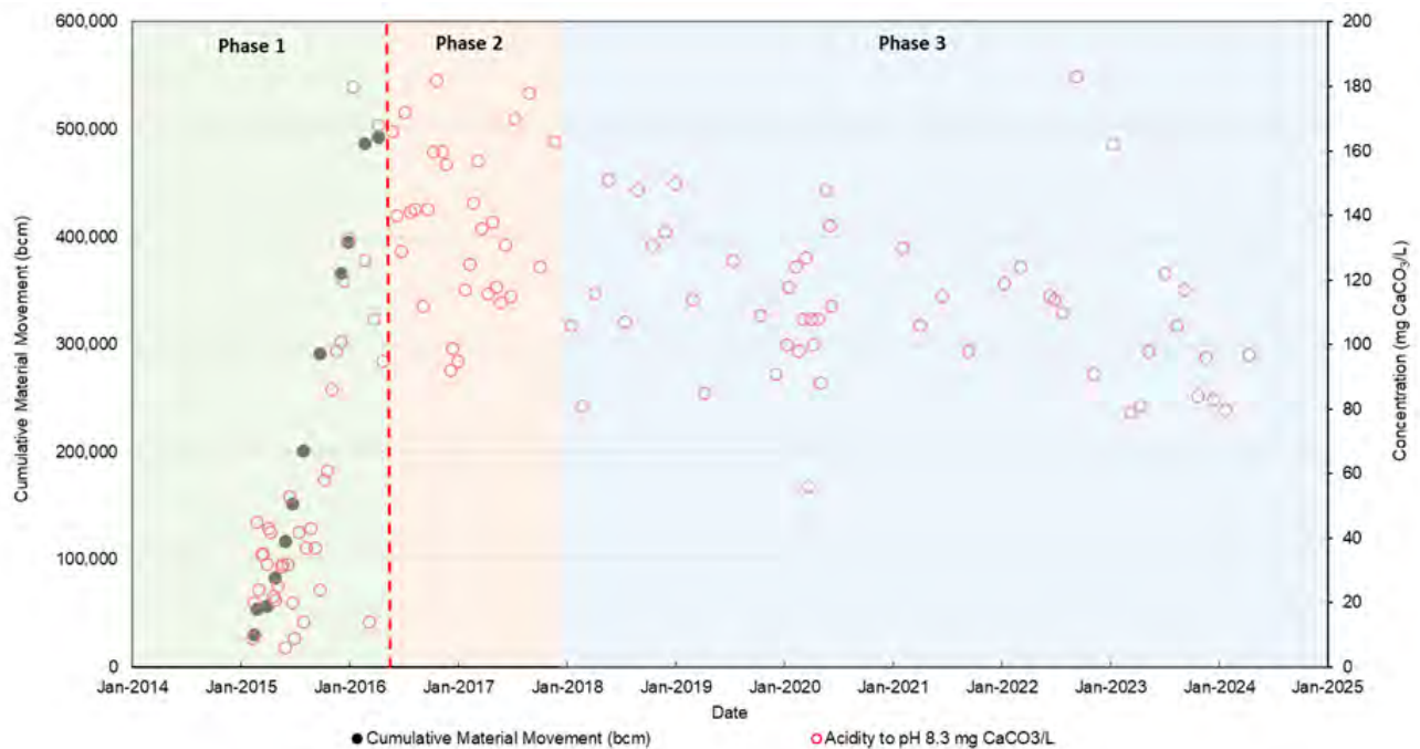
Figure 4: BV-ELF acidity concentration data.
