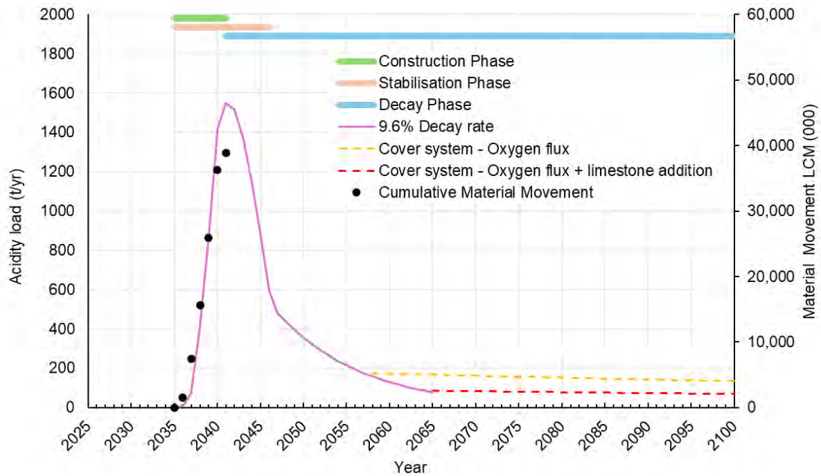
Figure 6: CON ELF acidity decay.
