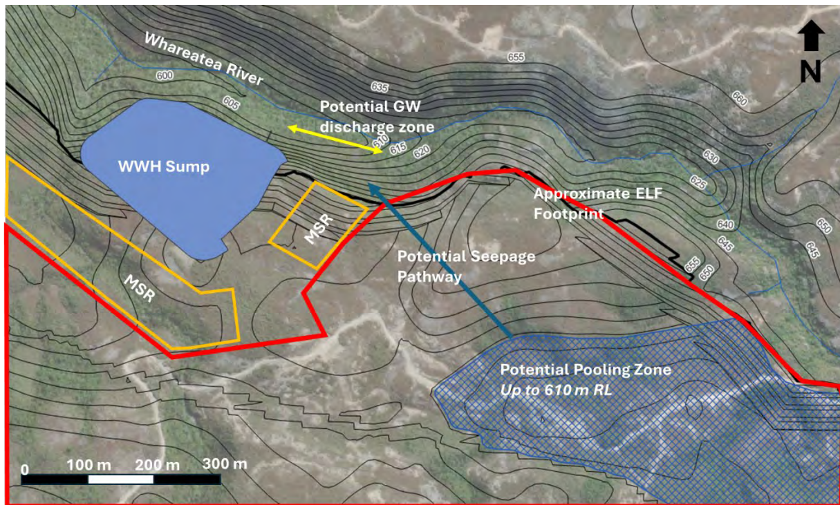
Figure 25: Potential untreated groundwater discharge zone from groundwater pooling.
