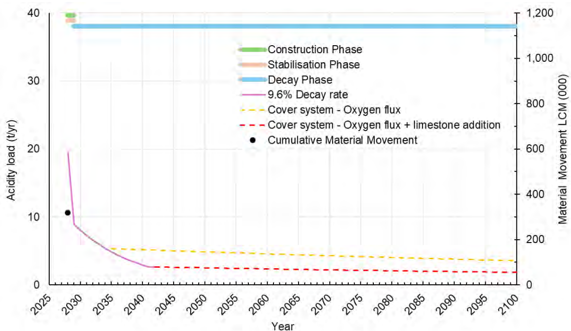
Figure 24: MSR12 ELF key parameter contaminant decay.
