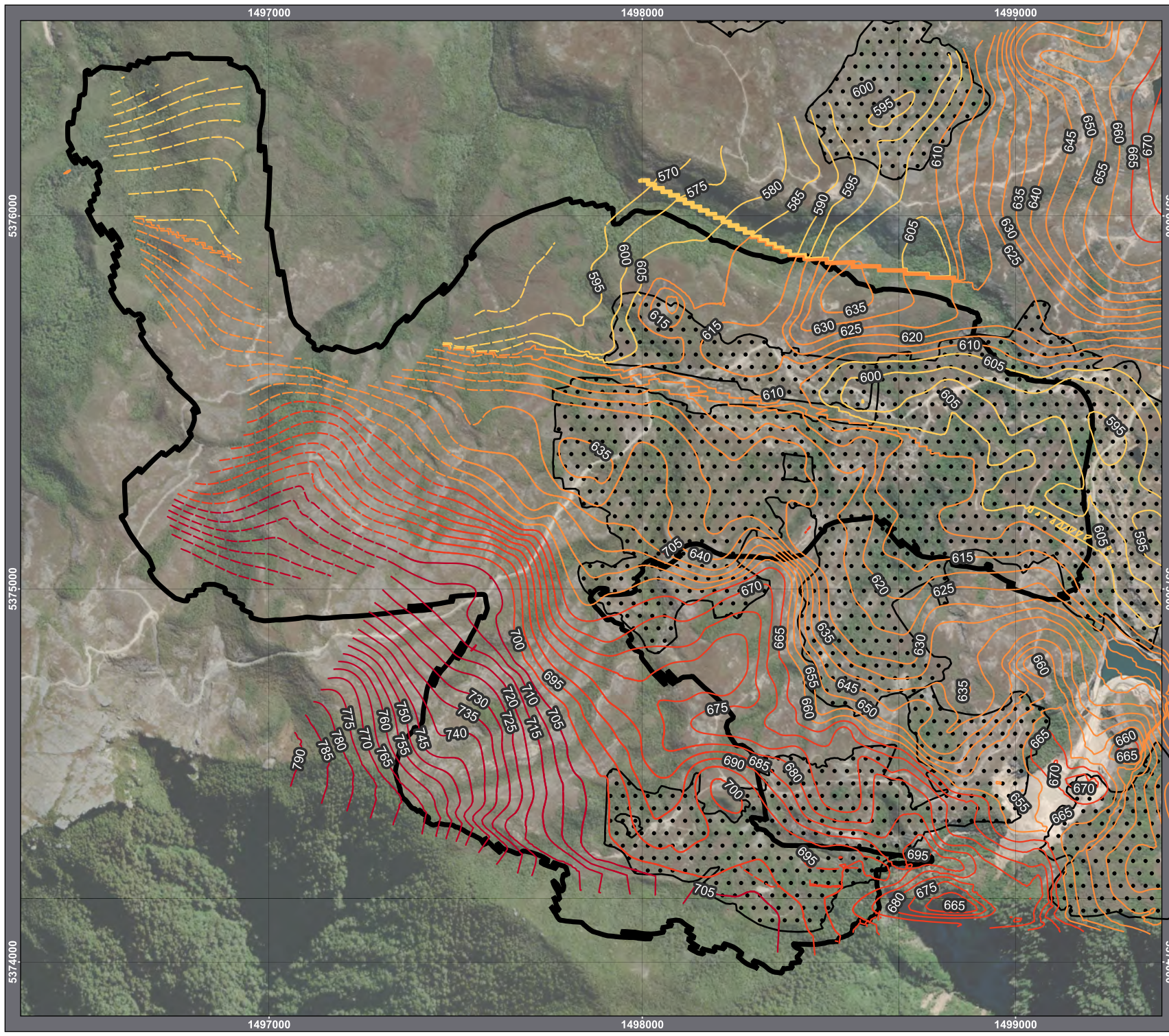
Figure 13: Coal Floor Contours Escarpment Extended Mine Project
