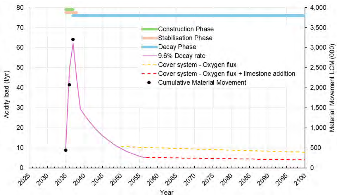
Figure 14: MSR4 ELF acidity decay.
