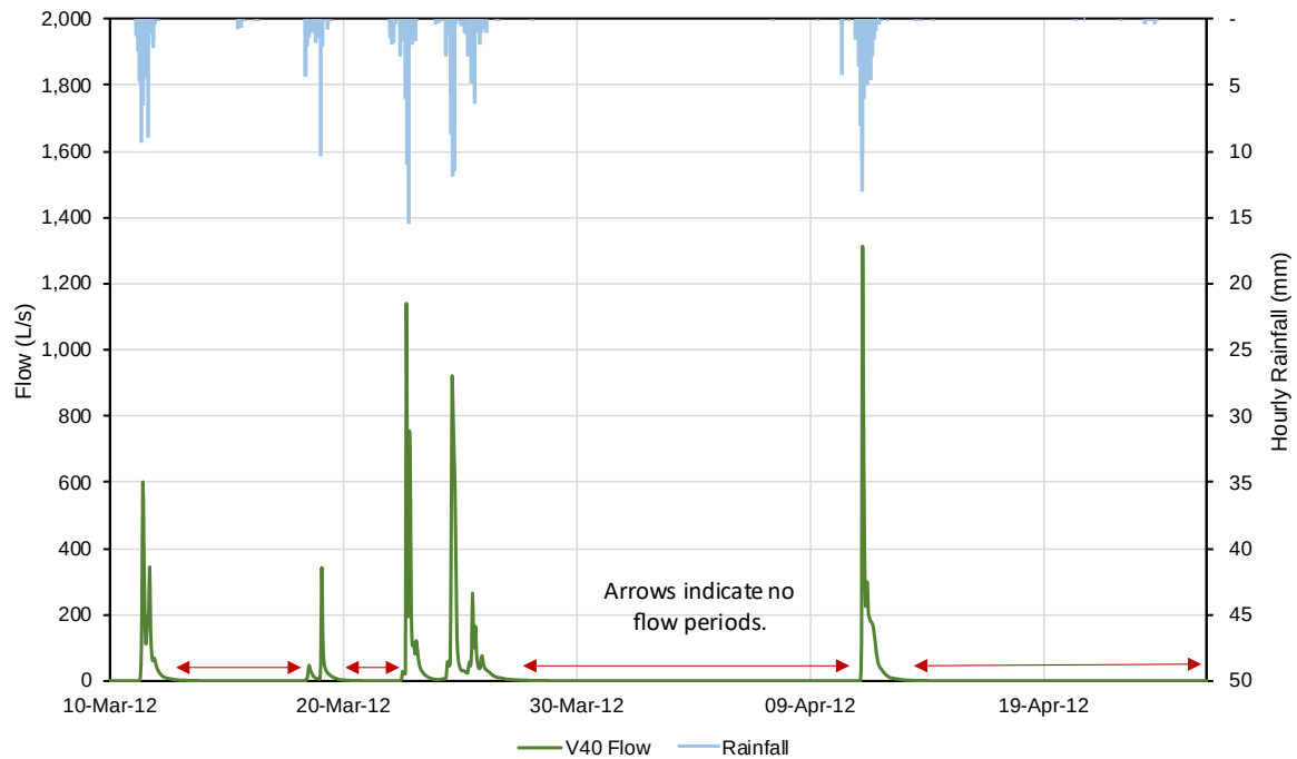
Figure 10: V40 Stream flow record.
