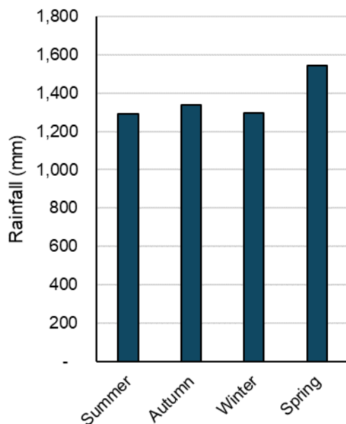
Figure 5: Seasonal average rainfall.
