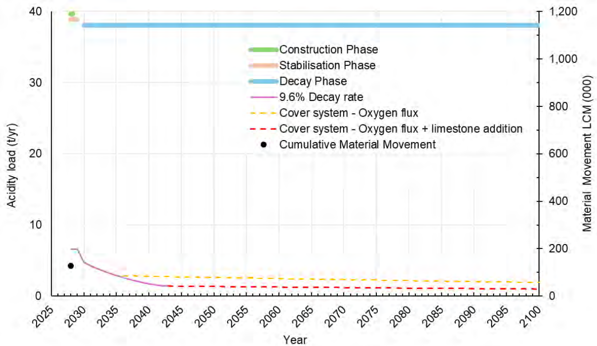
Figure 12: MSR2 ELF acidity decay.
