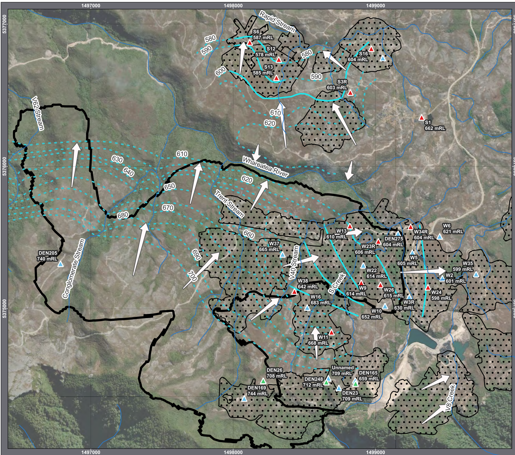
Figure 15: Groundwater Flow Regime Escarpment Extended Mine Project
