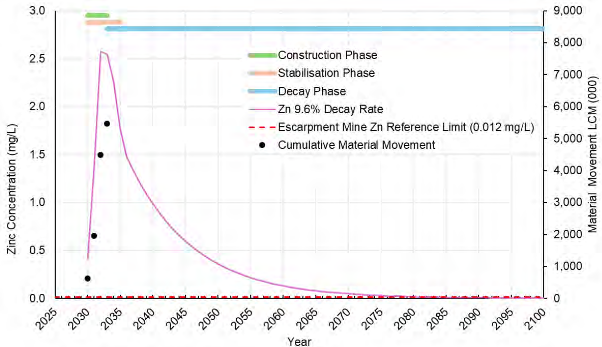
Figure 7: NSUL ELF closure Zn decay.
