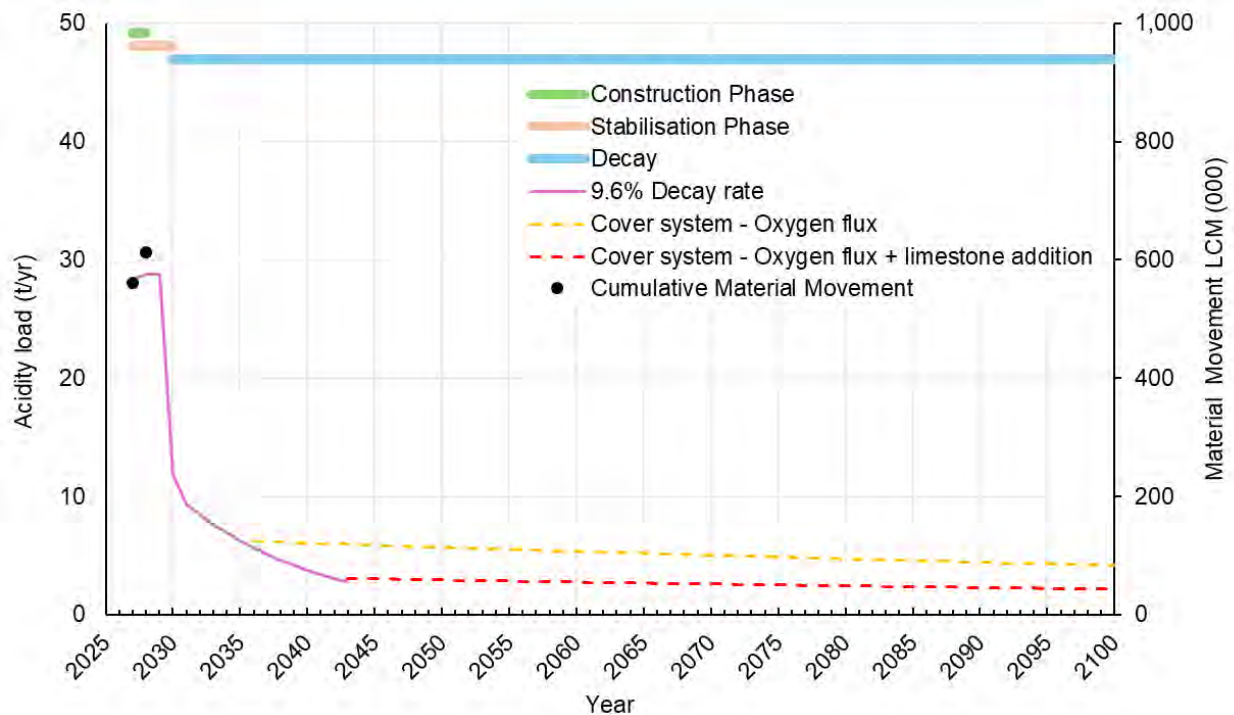
Figure 9: ESC ELF acidity decay.
