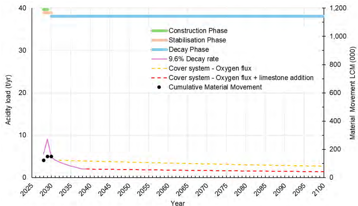
Figure 13: MSR3 ELF acidity decay.
