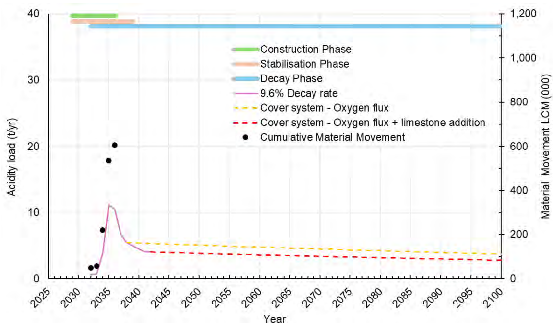
Figure 16: MSR6 ELF acidity decay.
