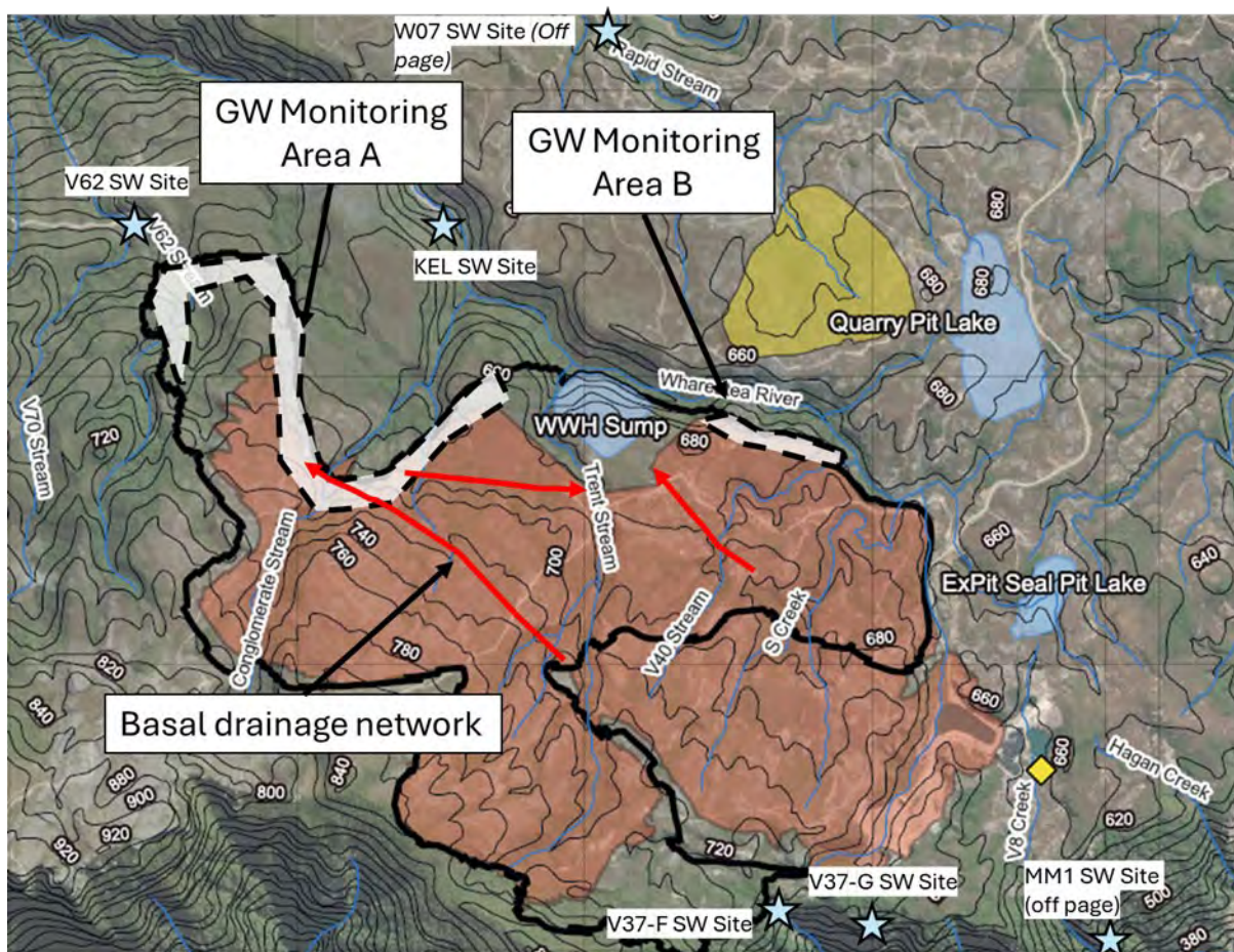
Figure 26: Proposed groundwater monitoring areas.
