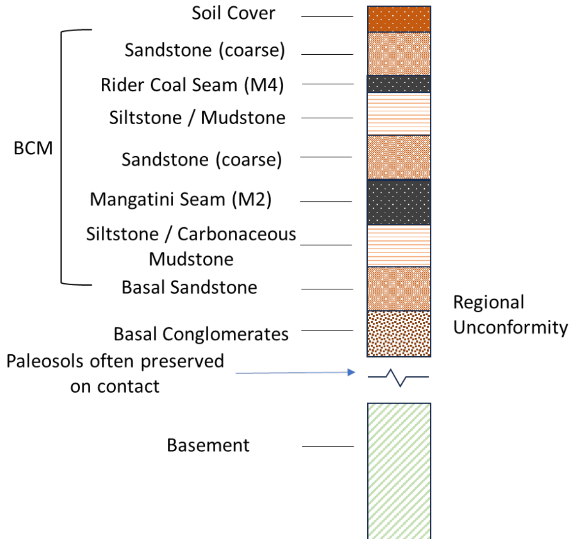
Figure 11: ESE Stratigraphy.
