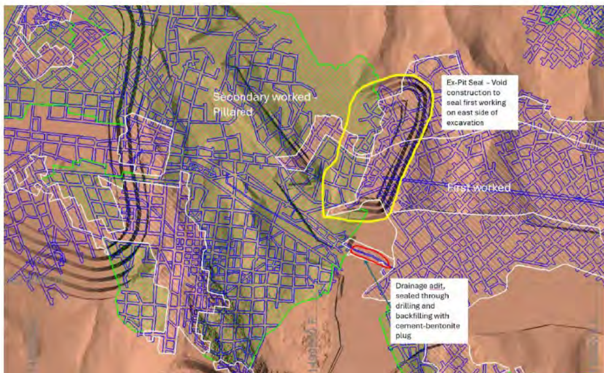
Figure 24: Ex-Pit Seal location.
