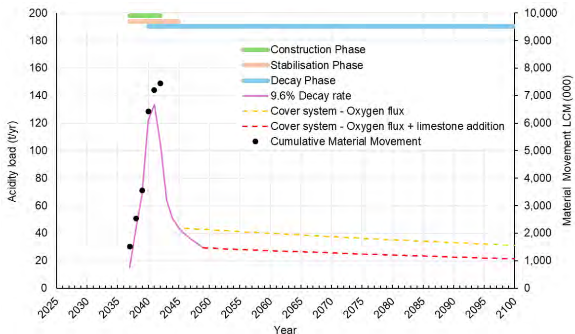
Figure 20: MSR8 ELF acidity decay.
