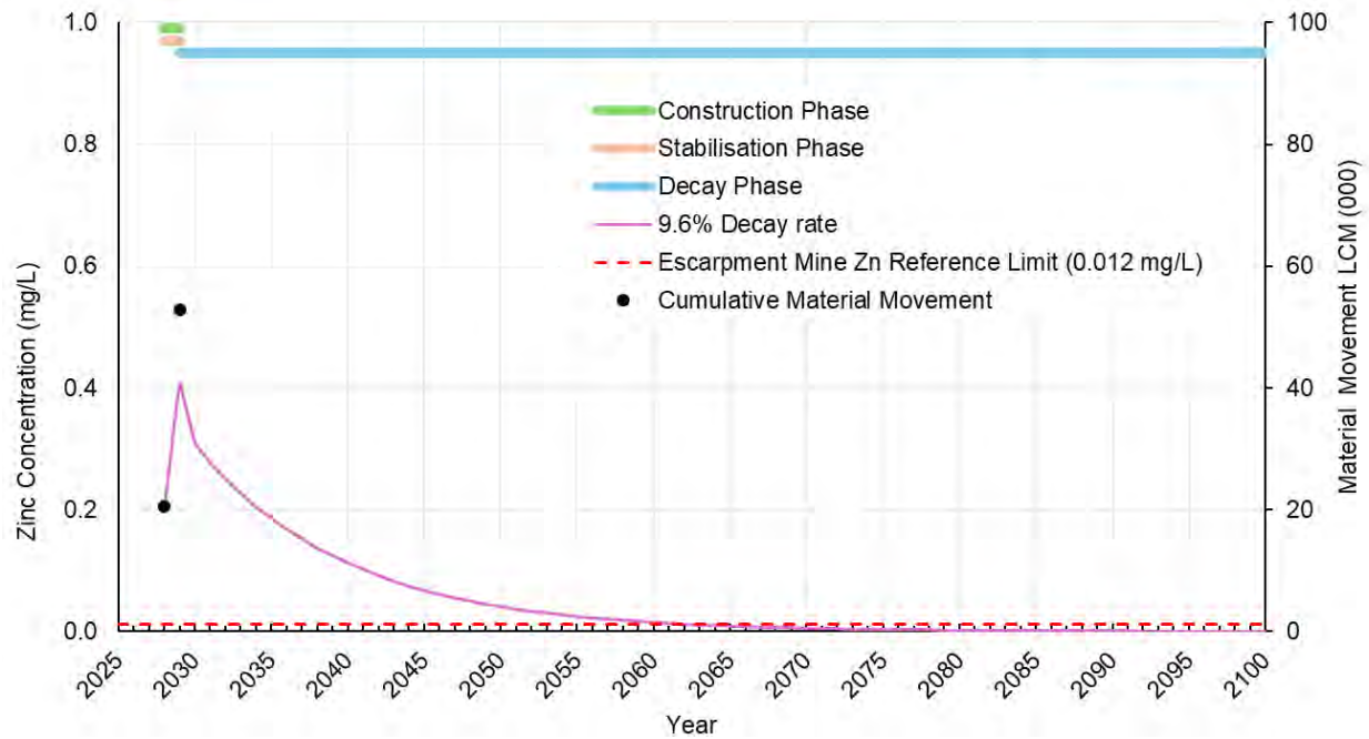
Figure 18: MDC1 ELF Zn decay.
