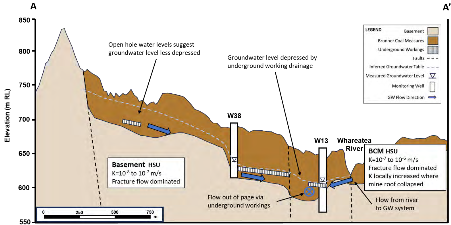
Figure 18: Baseline conceptual model - Section A-A'.
