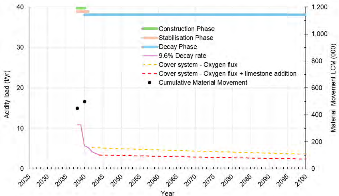
Figure 21: MSR9 ELF acidity decay.
