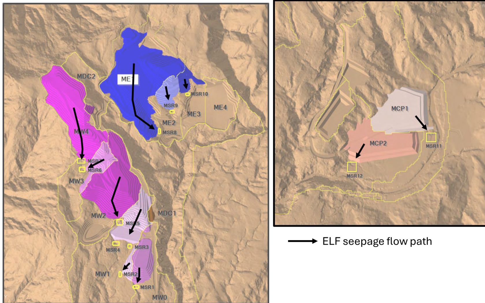
Figure 3: Mt Fred South Project ELF basal sub-catchments and MSR locations (yellow boxes)
