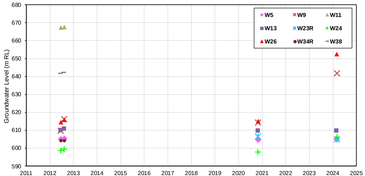
Figure 16: Groundwater levels in monitoring wells.
