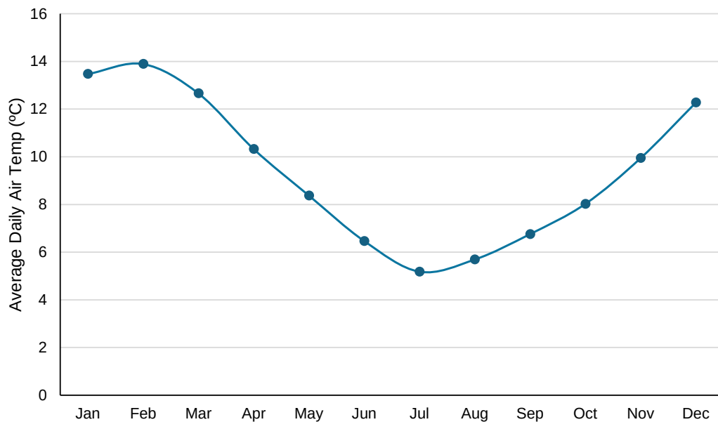
Figure 6: Average daily air temperature.
