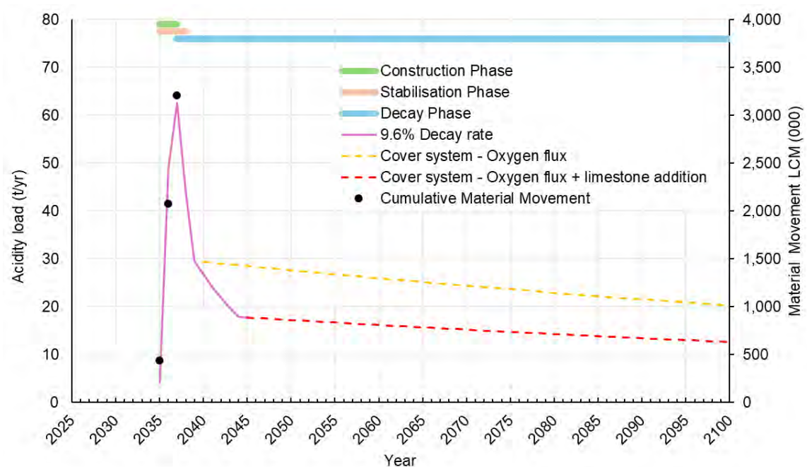
Figure 17: MSR7 ELF acidity decay.
