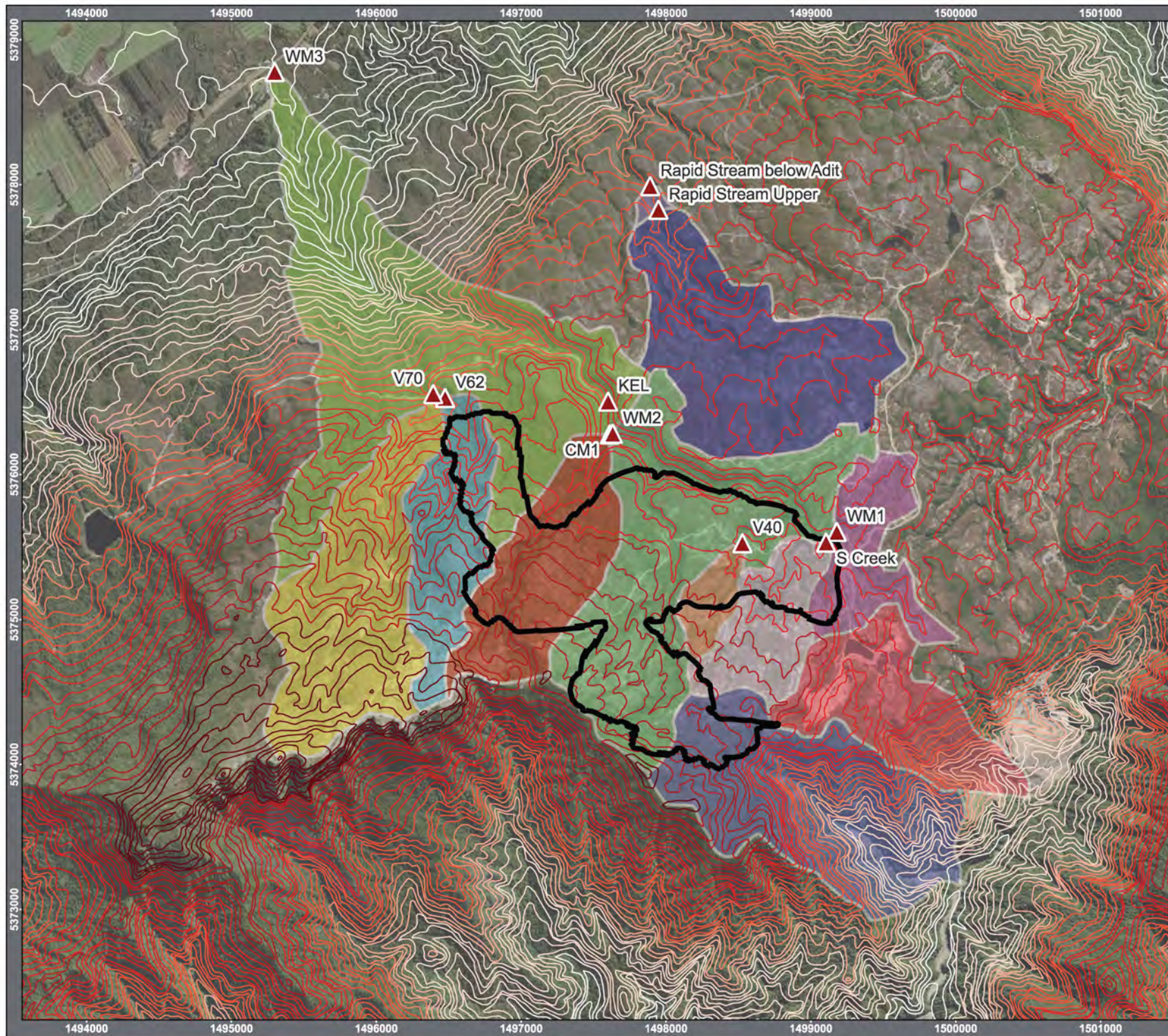
Figure 8: Flow recorder sites Escarpment Extended Mine Project
