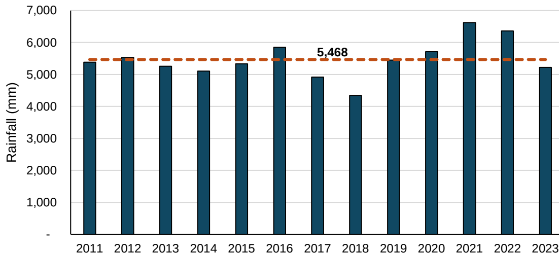
Figure 4: Average annual rainfall.
