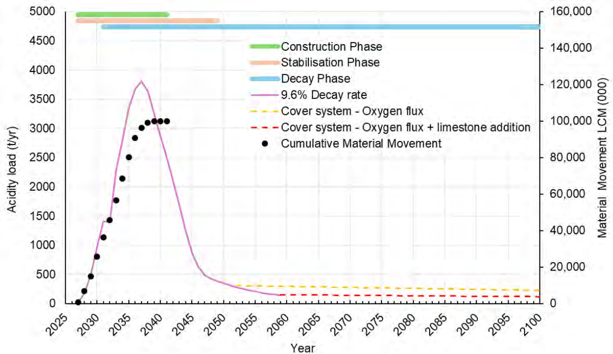
Figure 10: WWH ELF acidity decay.
