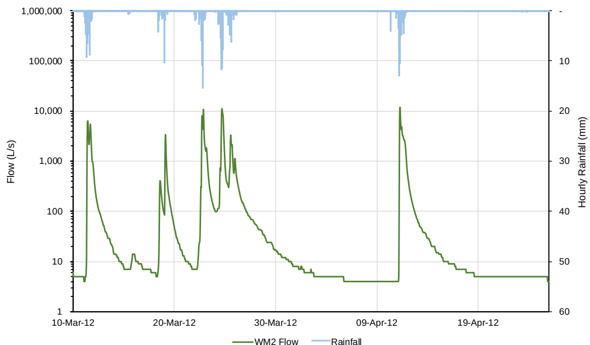
Figure 9: WM2 flow record.
