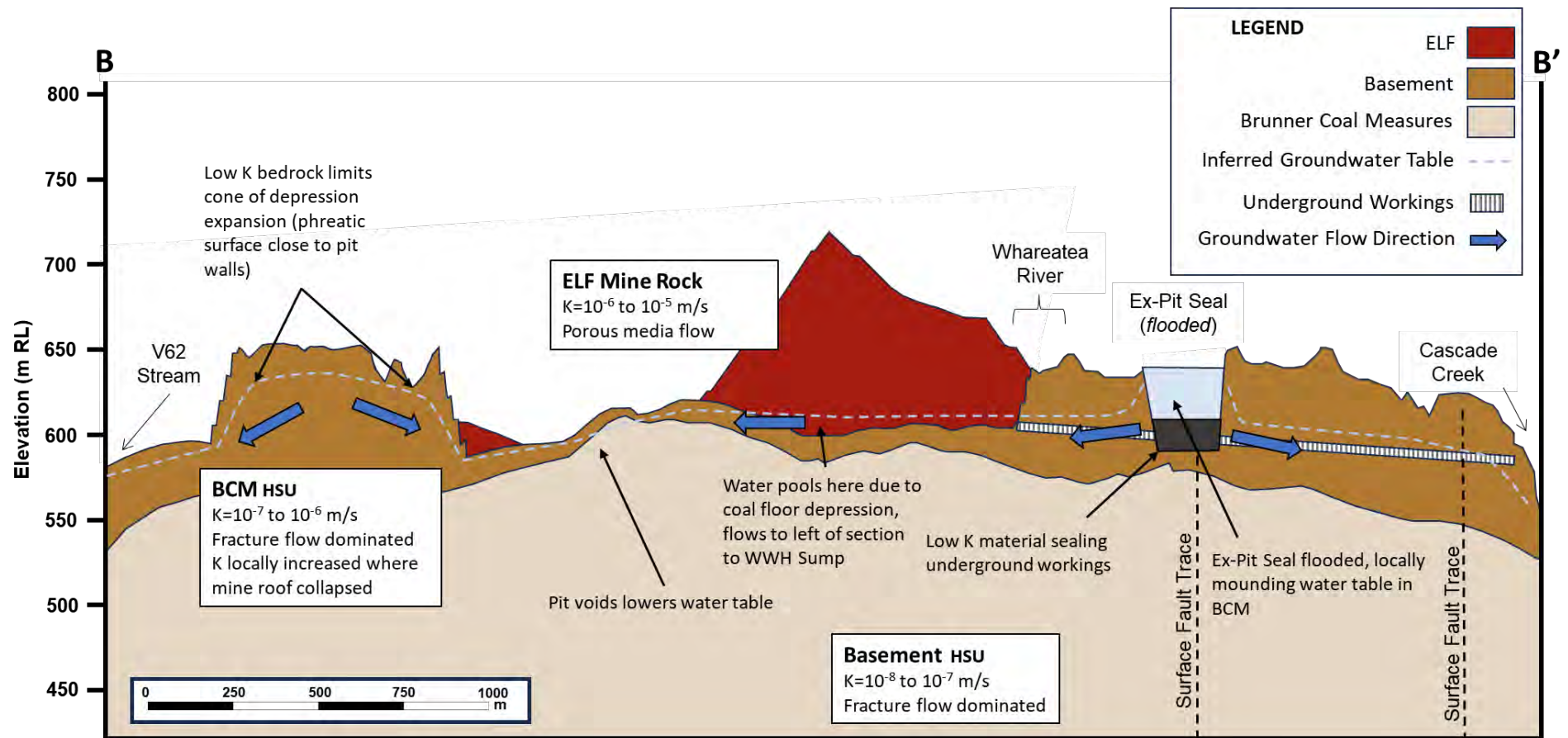
Figure 22: Operations and Post-closure conceptual model - Section B-B'.
