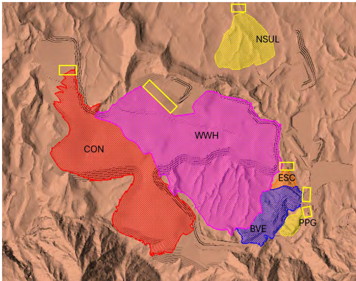
Figure 2: Escarpment Extended Project ELF basal sub-catchments and MSR locations.
