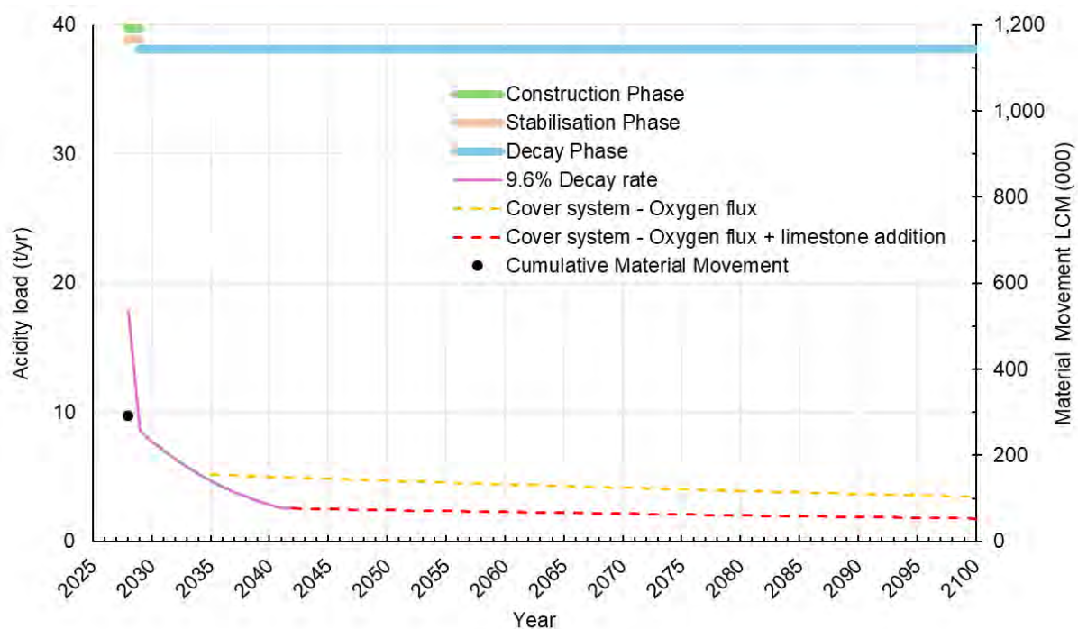
Figure 23: MSR11 ELF acidity decay.
