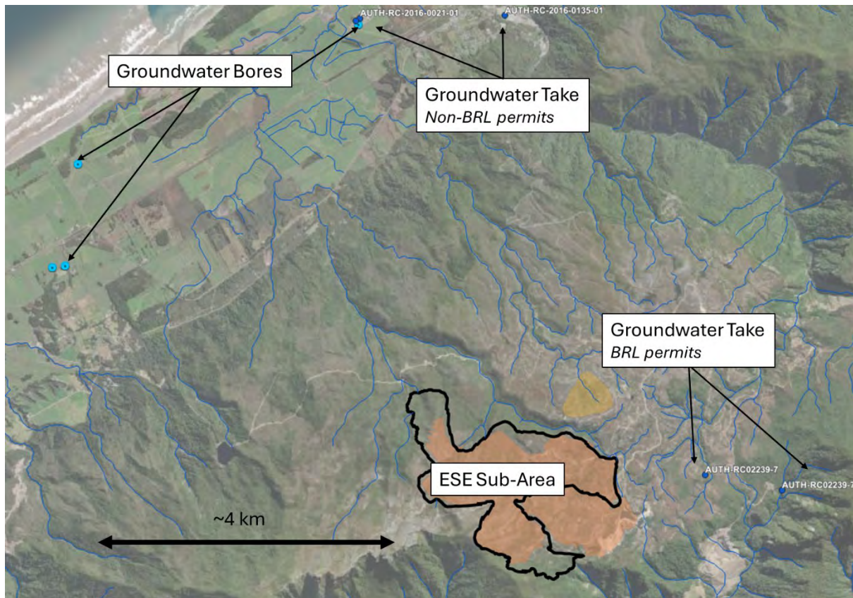
Figure 17: Nearby groundwater bores and permitted takes.
