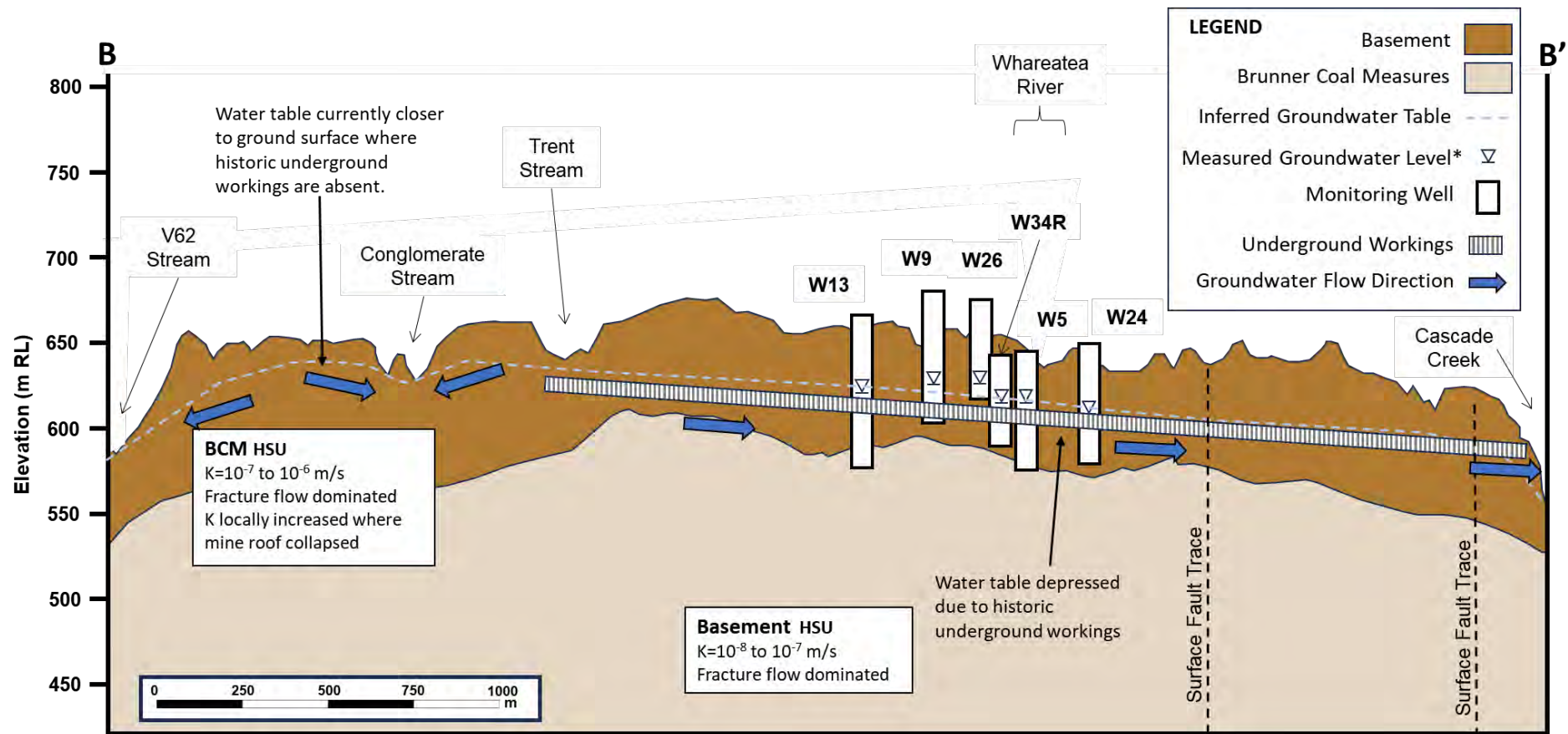
Figure 19: Baseline conceptual model - Section B-B'.
