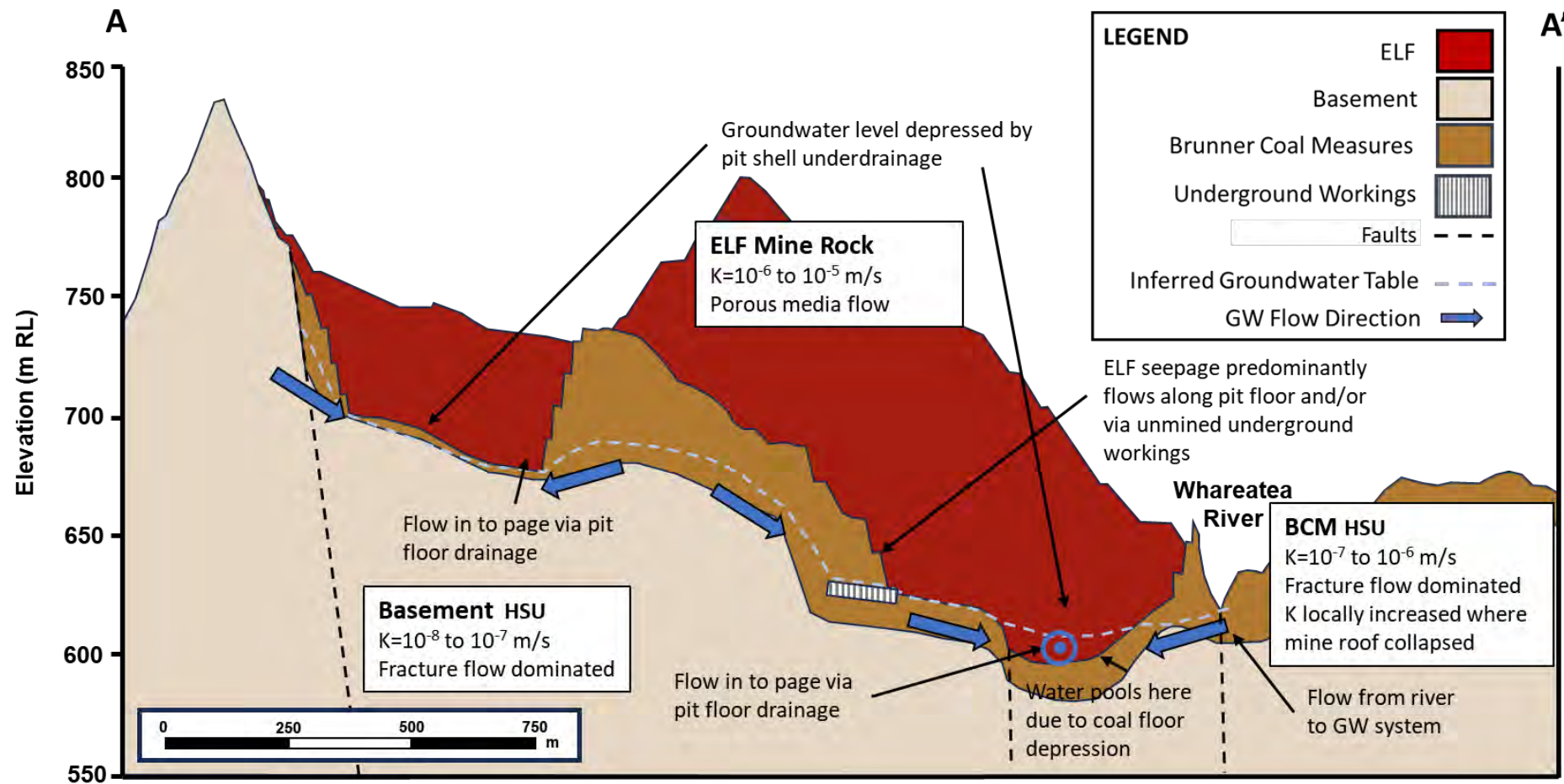
Figure 21: Operations and Post-closure conceptual model - Section A-A'.
