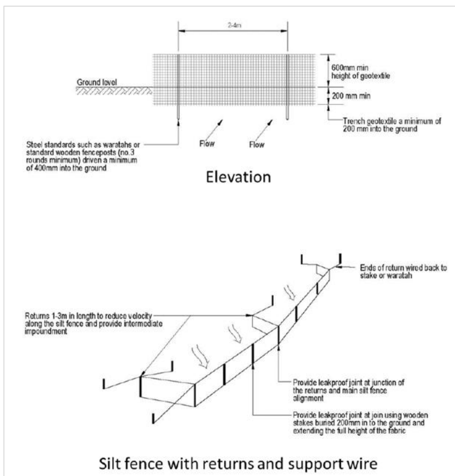
Figure 12: General silt fence schematic
