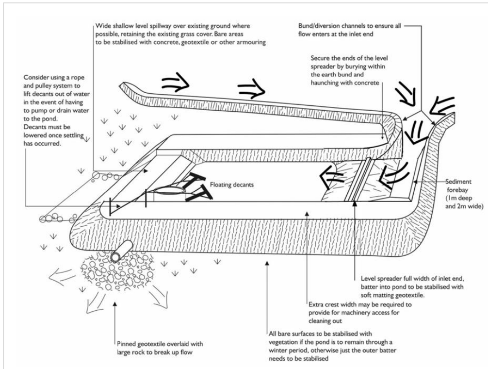
Figure 10: Schematic of a SRP
