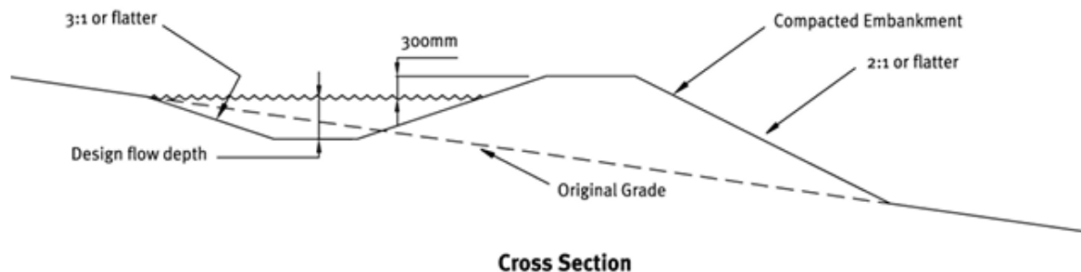
Figure 9: Cross section of a dirty water diversion (GD05)
