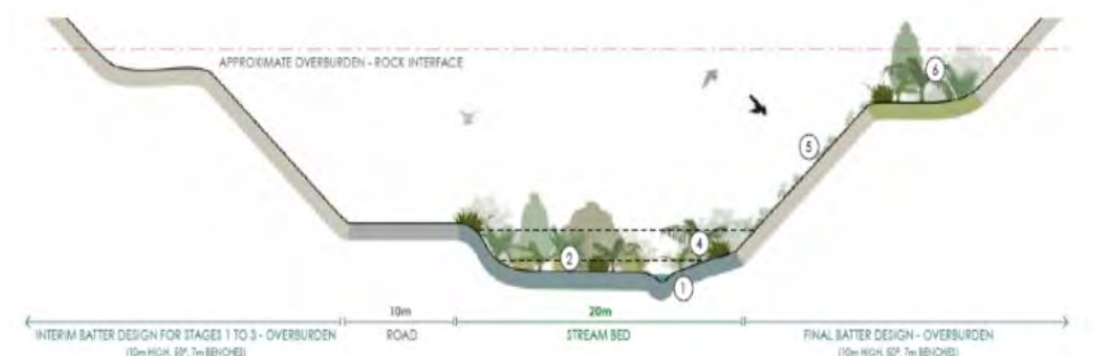
Figure 5: Mangapū Stream Realignment and Riparian Enhancement Concept at Stage 2
