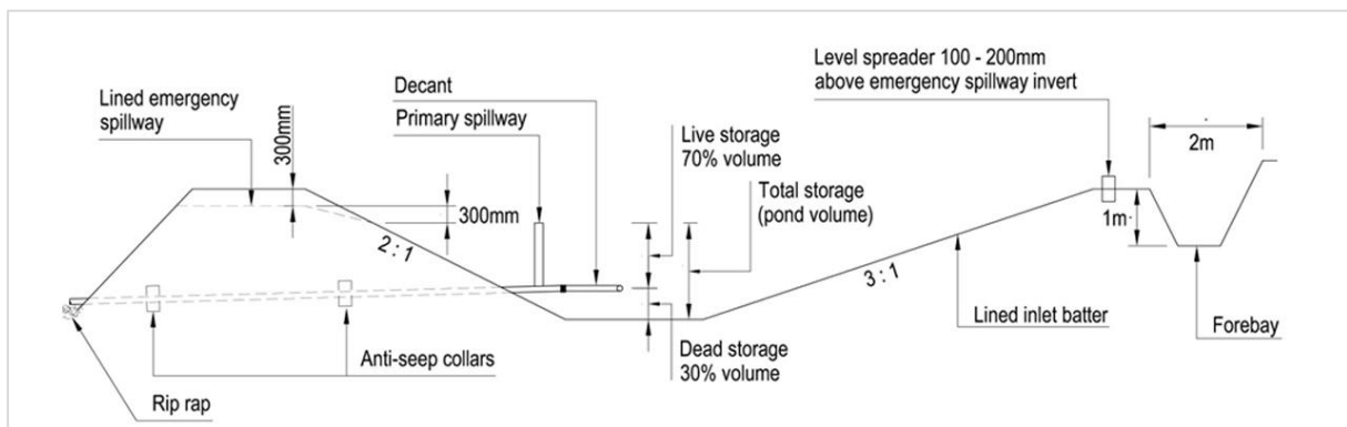
Figure 11: SRP Cross Section
