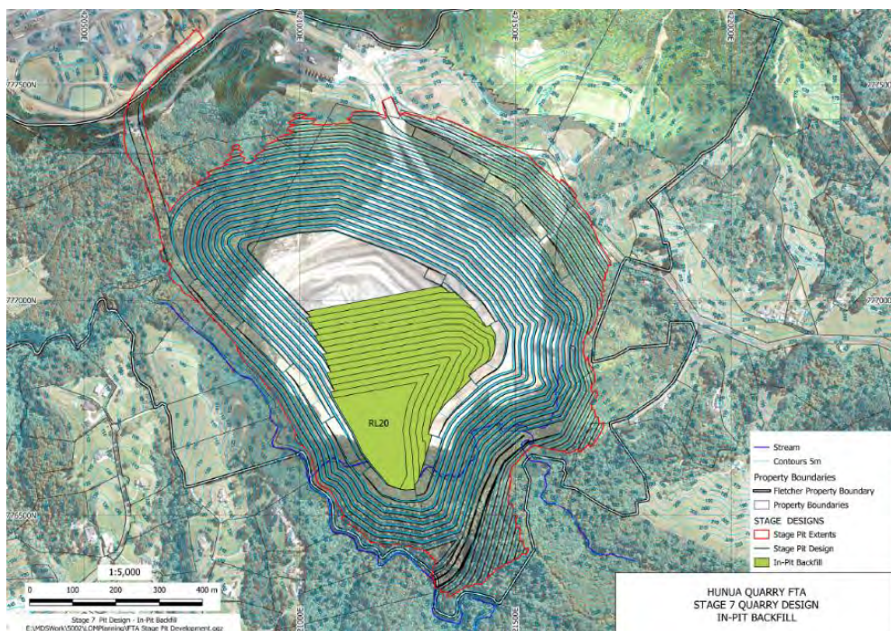
Figure 6: Stage 7 OBPA infill of Symonds Hill Pit
