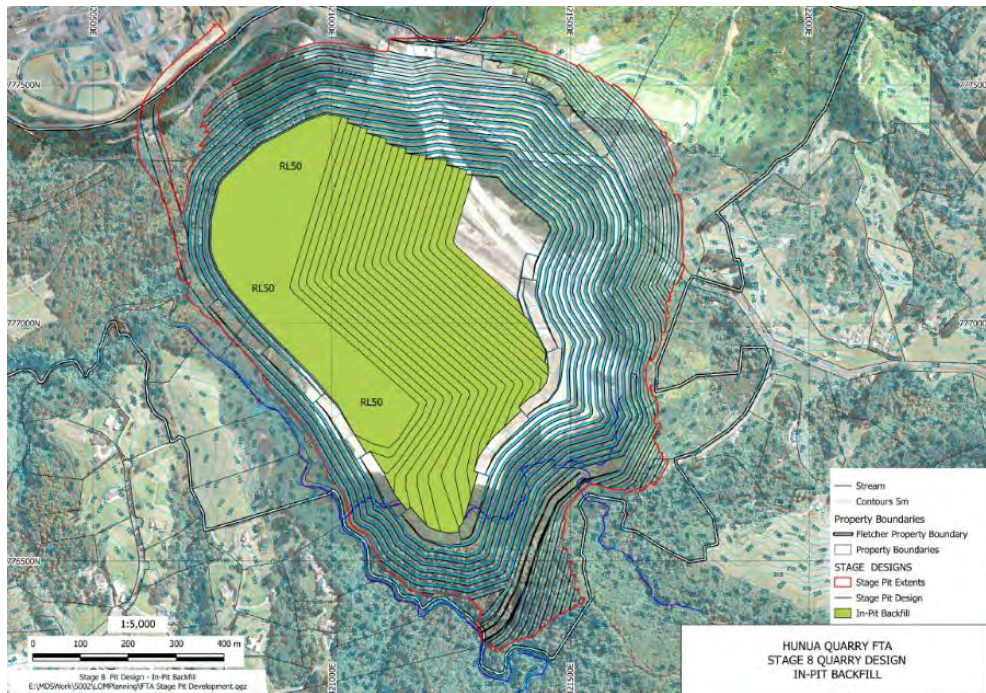
Figure 7: Stage 8 OBPA infill of Symonds Hill Pit
