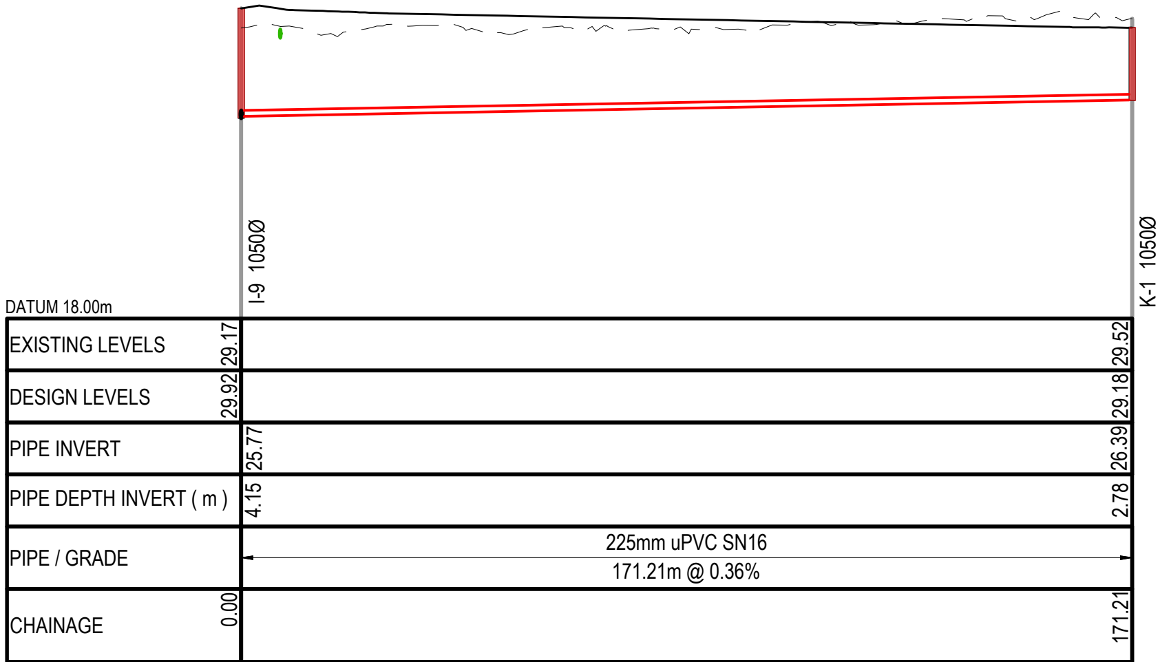
WASTEWATER LINE K SCALE: HORI 1:1000 VERT 1:200
