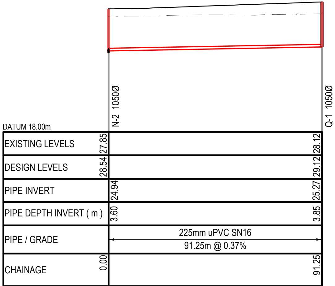
WASTEWATER LINE Q SCALE: HORI 1:1000 VERT 1:200
