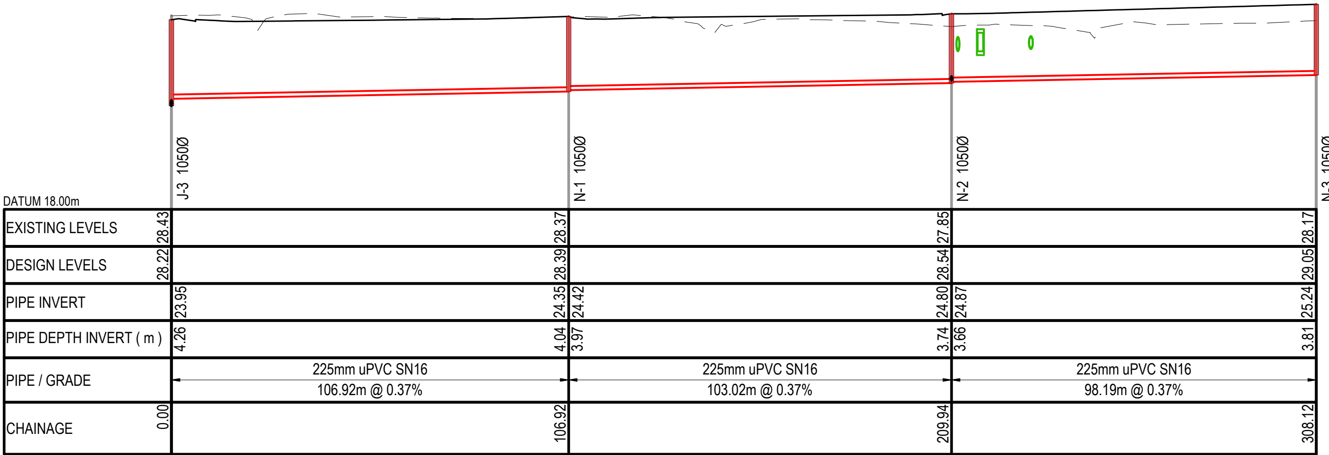
WASTEWATER LINE N SCALE: HORI 1:1000 VERT 1:200
