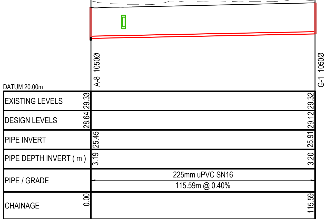
WASTEWATER LINE G SCALE: HORI 1:1000 VERT 1:200
