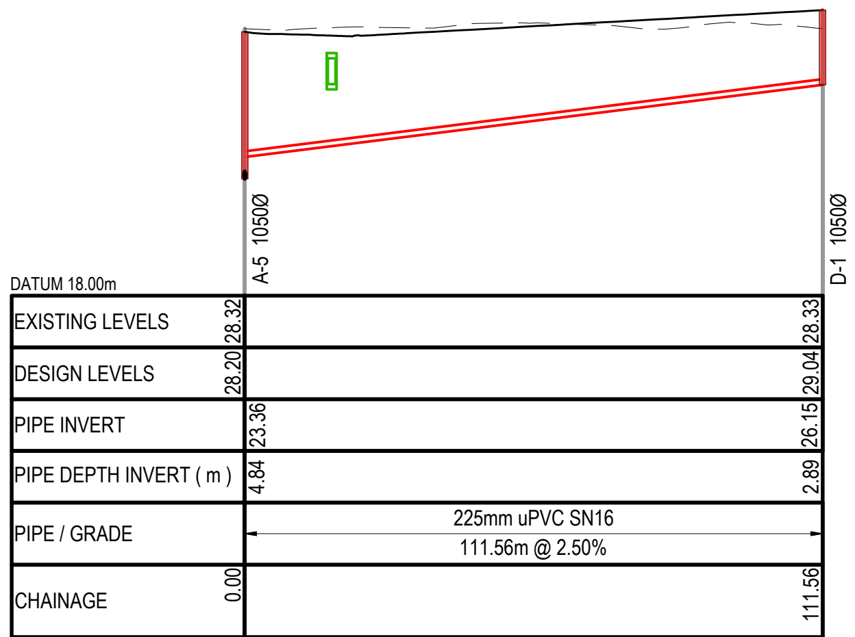
WASTEWATER LINE D SCALE: HORI 1:1000 VERT 1:200
