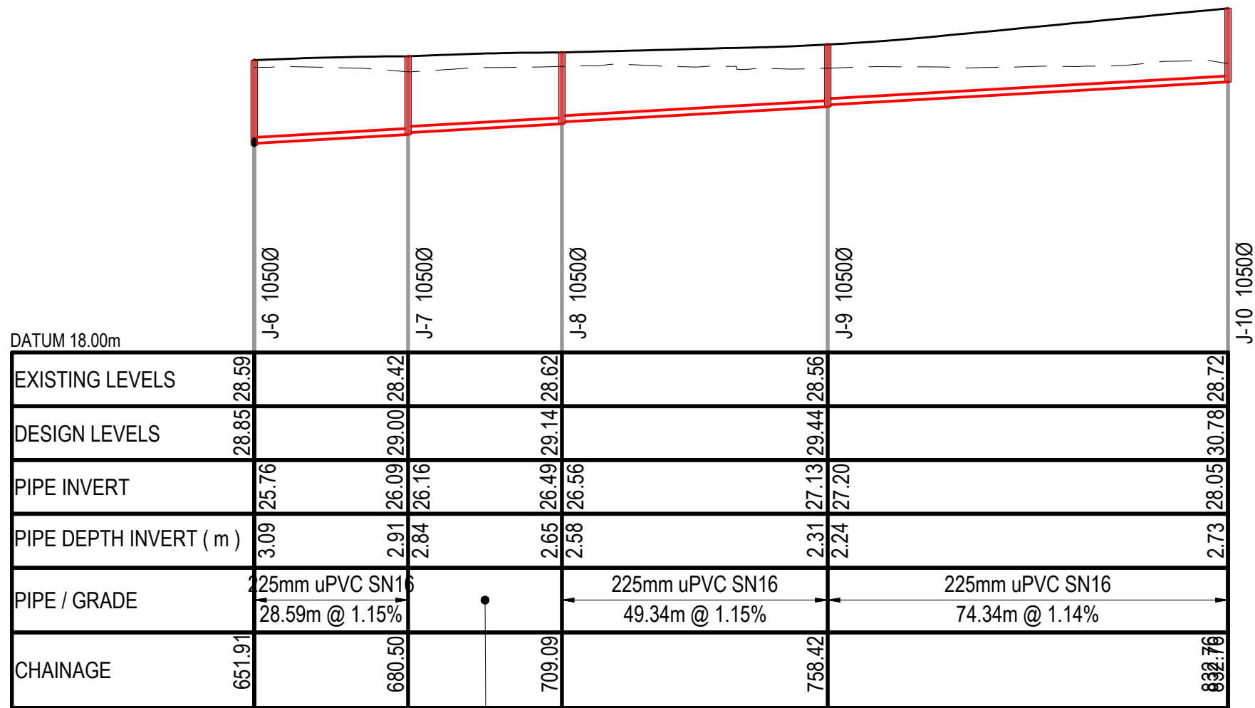
225mm uPVC SN16 28.59m @ 1.14% WASTEWATER LINE J SCALE: HORI 1:1000 VERT 1:200
