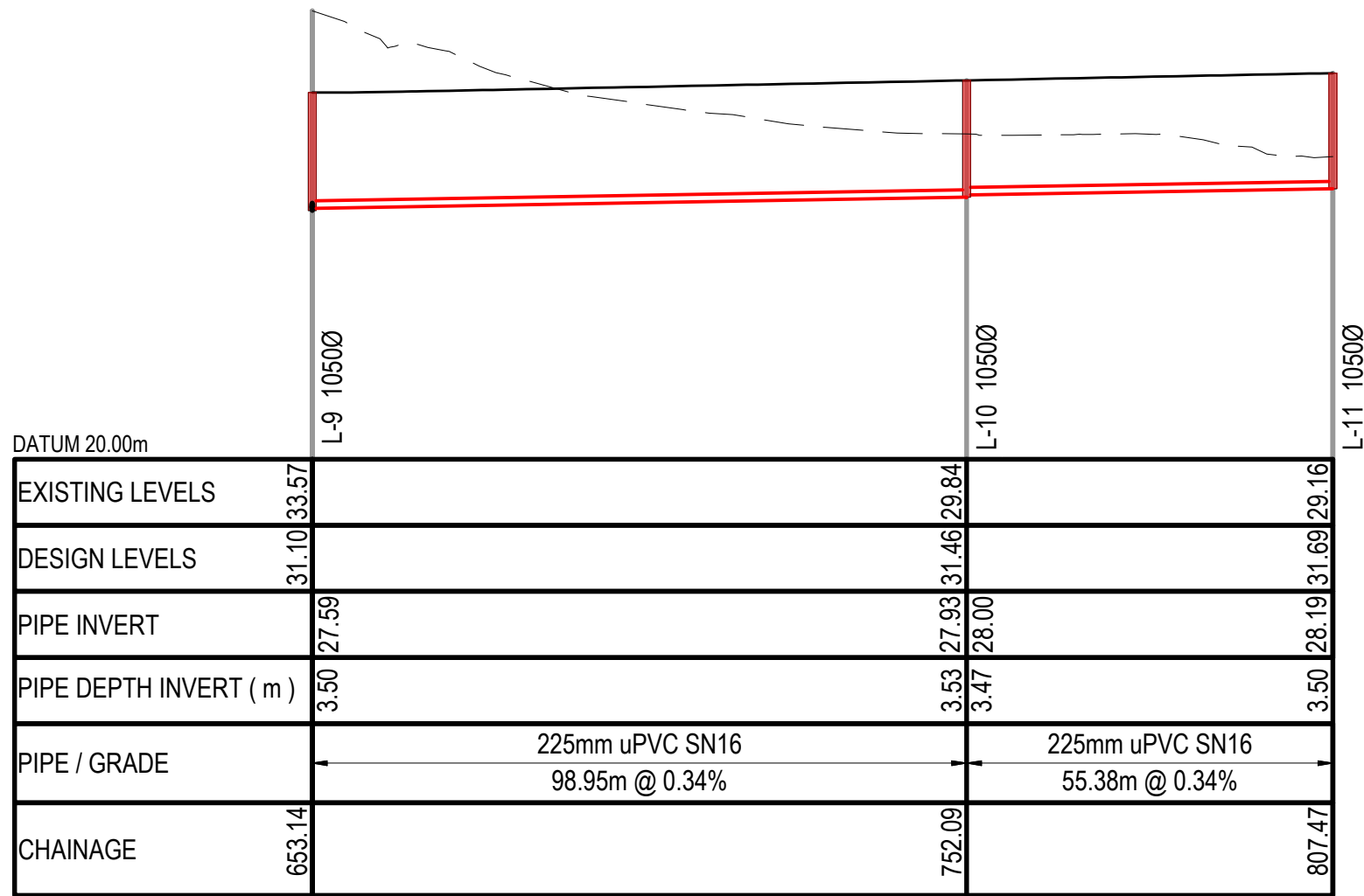
WASTEWATER LINE L SCALE: HORI 1:1000 VERT 1:200
