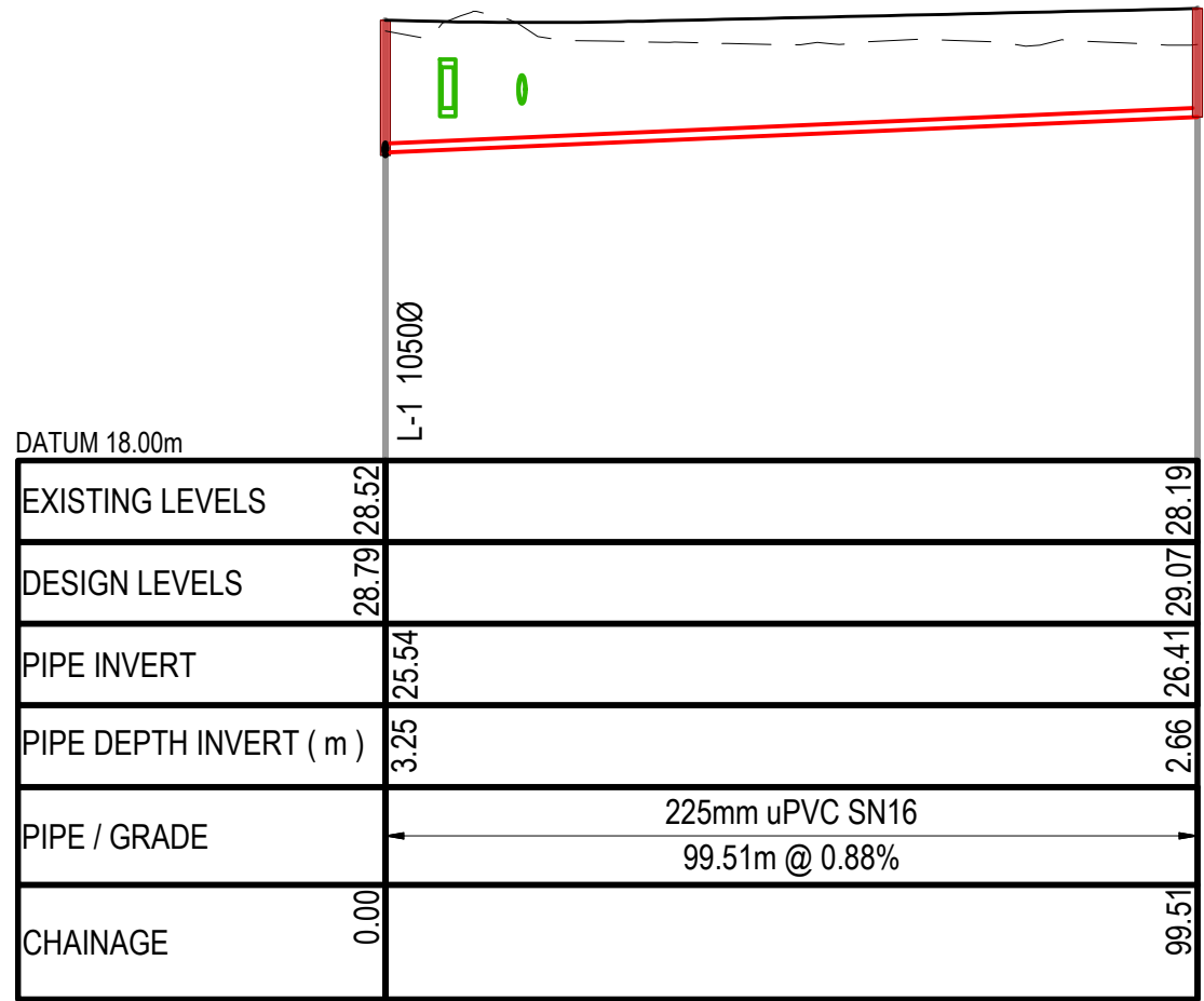
WASTEWATER LINE M SCALE: HORI 1:1000 VERT 1:200
