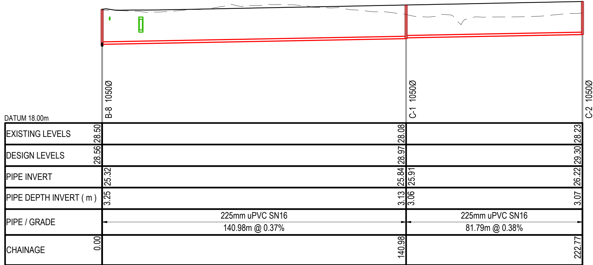
WASTEWATER LINE C SCALE: HORI 1:1000 VERT 1:200
