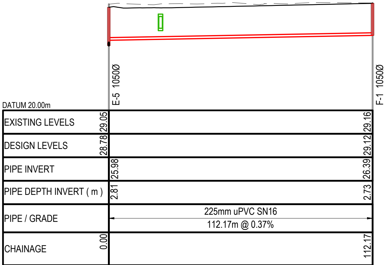
WASTEWATER LINE F SCALE: HORI 1:1000 VERT 1:200
