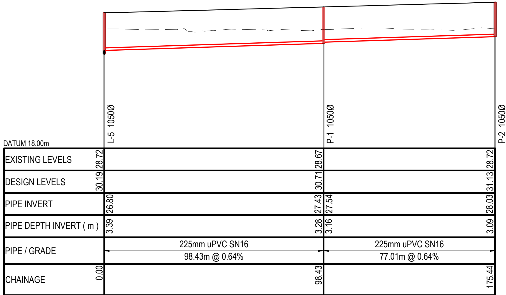
WASTEWATER LINE P SCALE: HORI 1:1000 VERT 1:200
