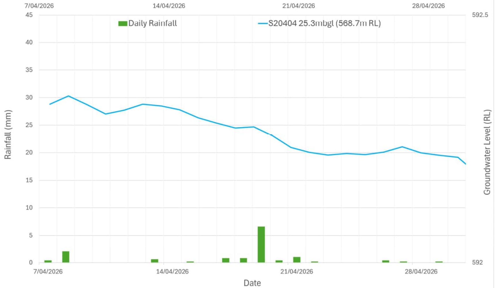
MDD506 - Vibrating Wire Piezometers (7 April 2026 to 30 April 2026)
