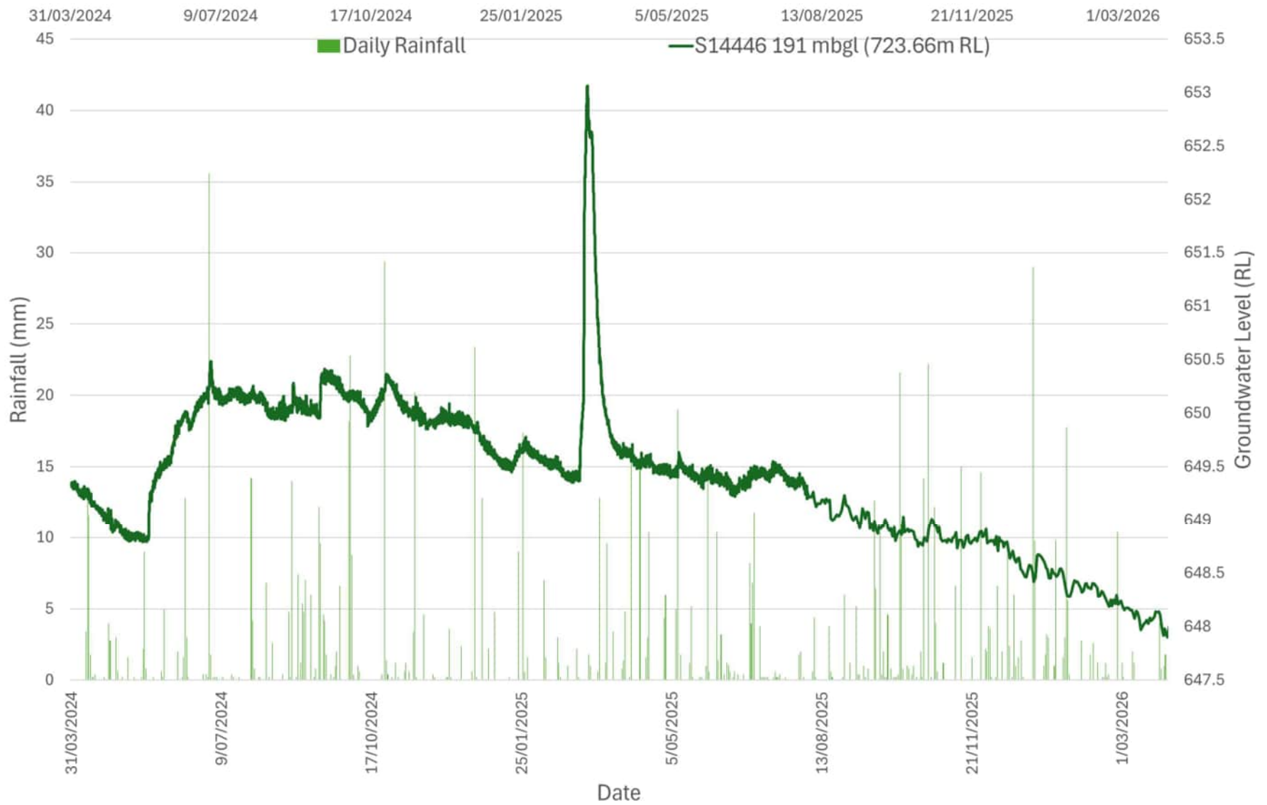
MDD290 - Vibrating Wire Piezometers (31/3/2024 to 31/3/2026)
