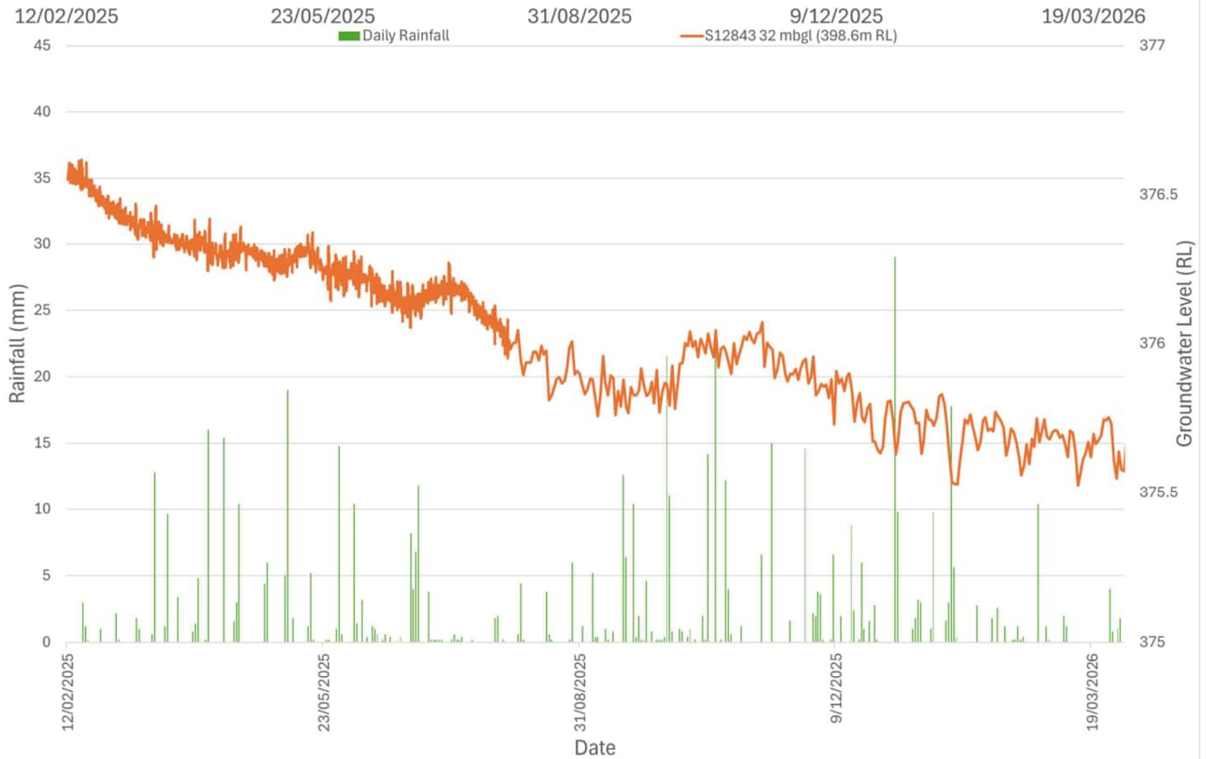
MDD365 - Vibrating Wire Piezometers (12/2/2025 to 31/3/2026)
