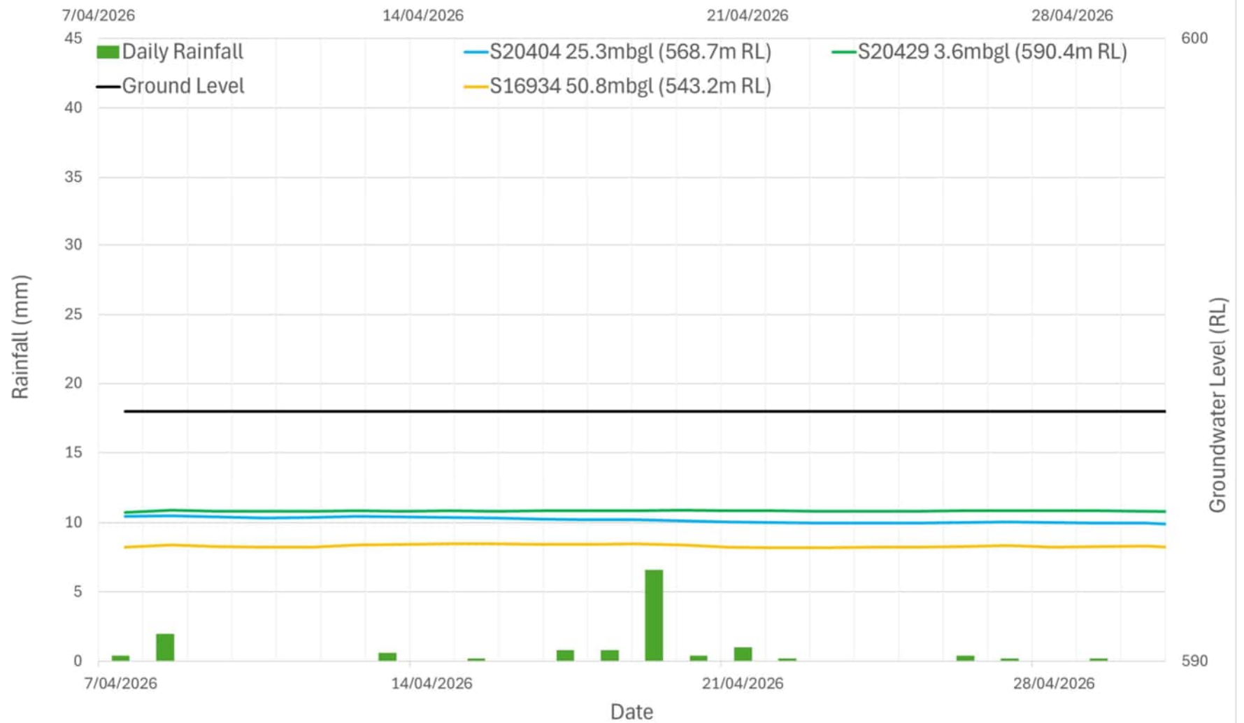
MDD506 - Vibrating Wire Piezometers (7 April 2026 to 30 April 2026)
