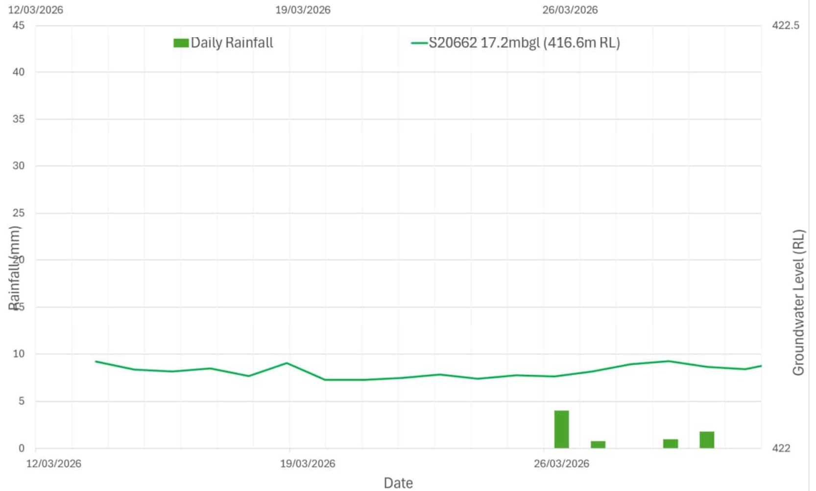
MDD511 - Vibrating Wire Piezometers (12 Mar 2026 to 31 Mar 2026)
