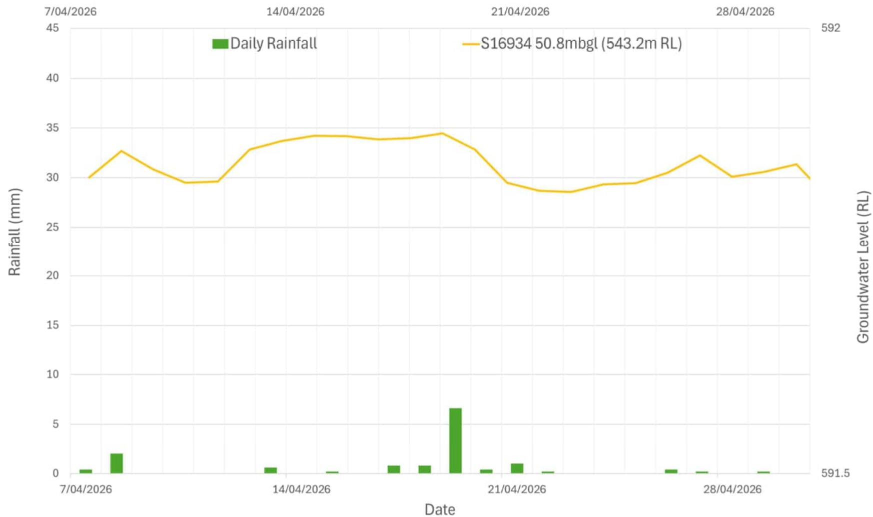
MDD506 - Vibrating Wire Piezometers (7 April 2026 to 30 April 2026)
