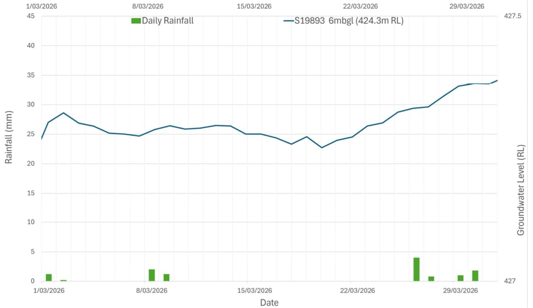
MDD499 - Vibrating Wire Piezometers (1 Mar 2026 to 31 Mar 2026)
