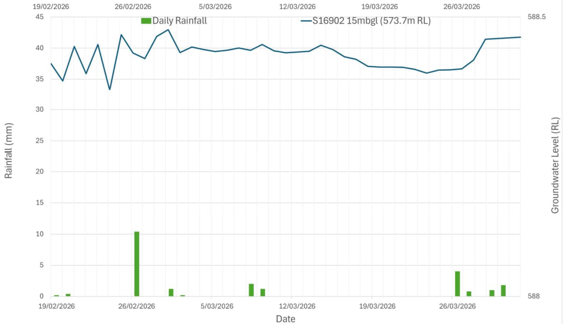
MDD502 - Vibrating Wire Piezometers (19 Feb 2026 to 27 Feb 2026)
