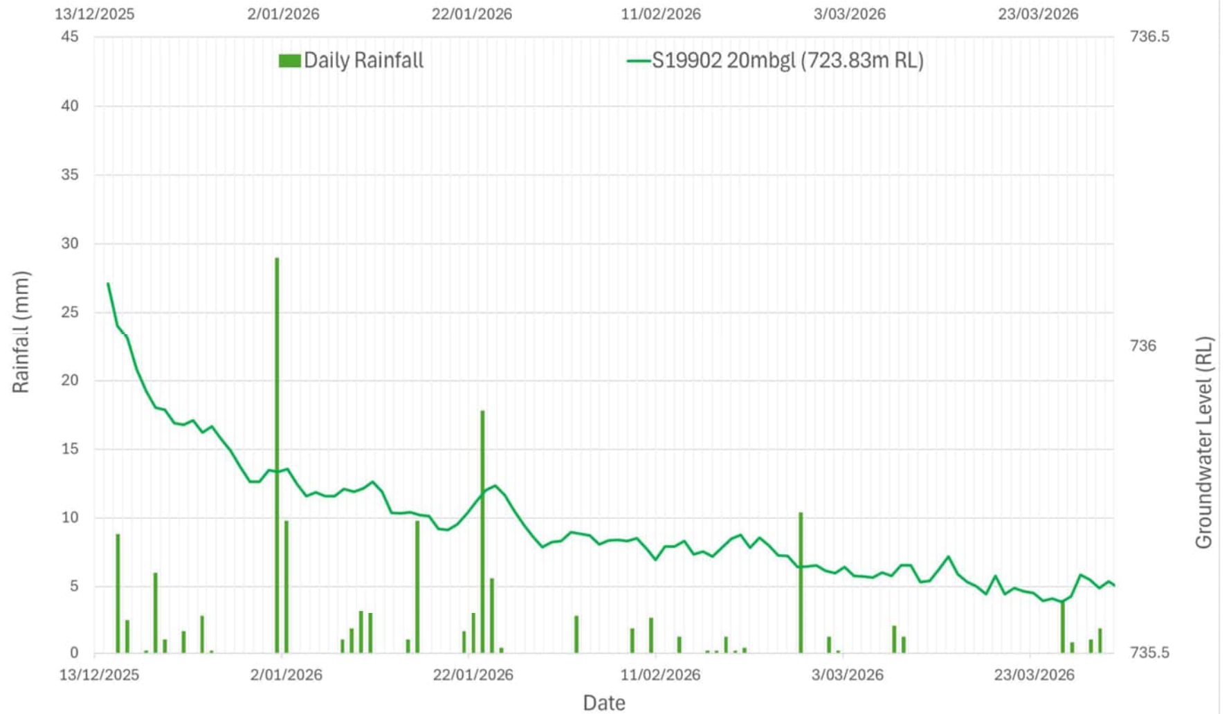
MDD491 - Vibrating Wire Piezometers (13 Dec 2025 to 31 Mar 2026)
