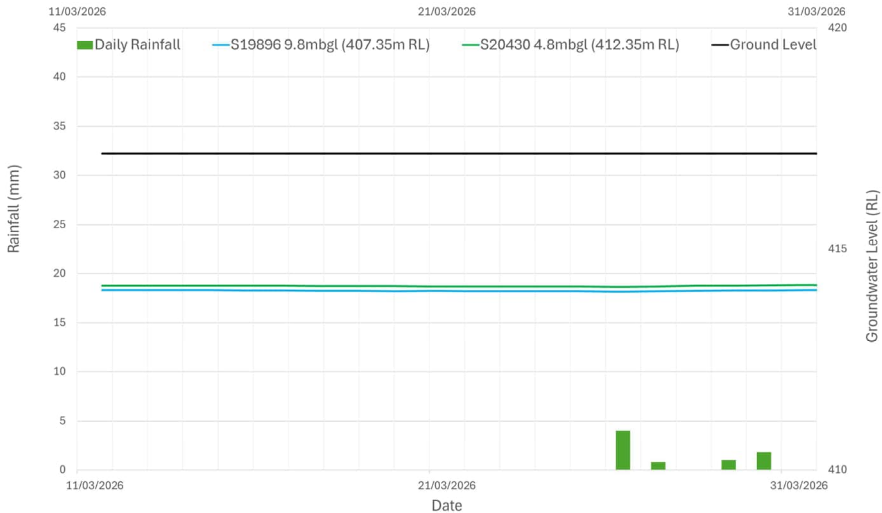
MDD508 - Vibrating Wire Piezometers (11 Mar 2026 to 31 Mar 2026)
