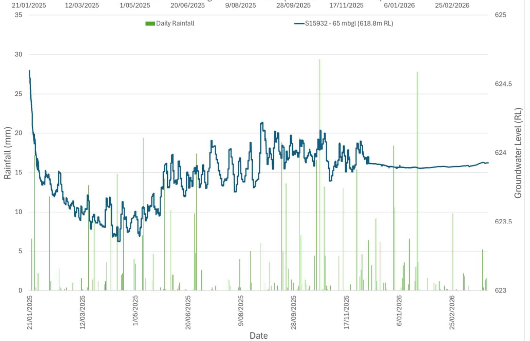
MDD399 - Vibrating Wire Piezometers (21/1/2025 to 31/3/2026)
