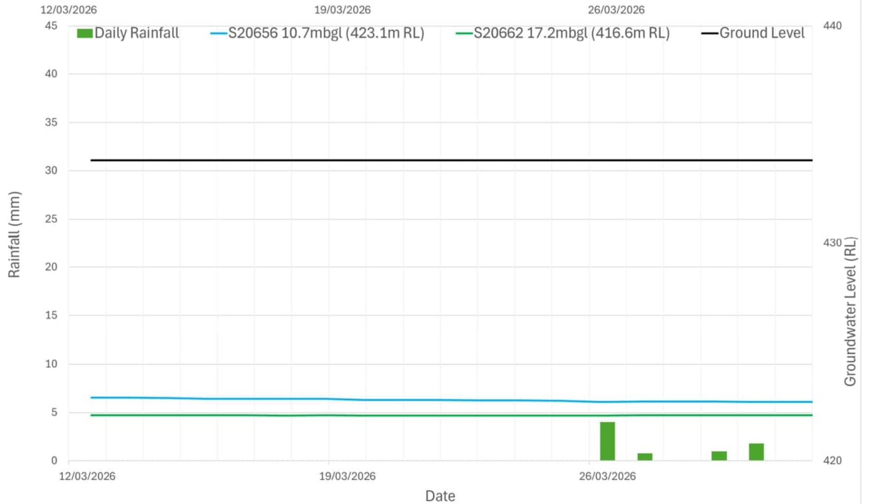
MDD511 - Vibrating Wire Piezometers (12 Mar 2026 to 31 Mar 2026)
