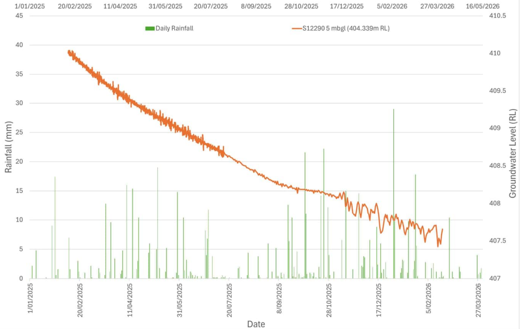
MDD362 - Vibrating Wire Piezometers (1 Jan 2025 to 31 Mar 2026)
