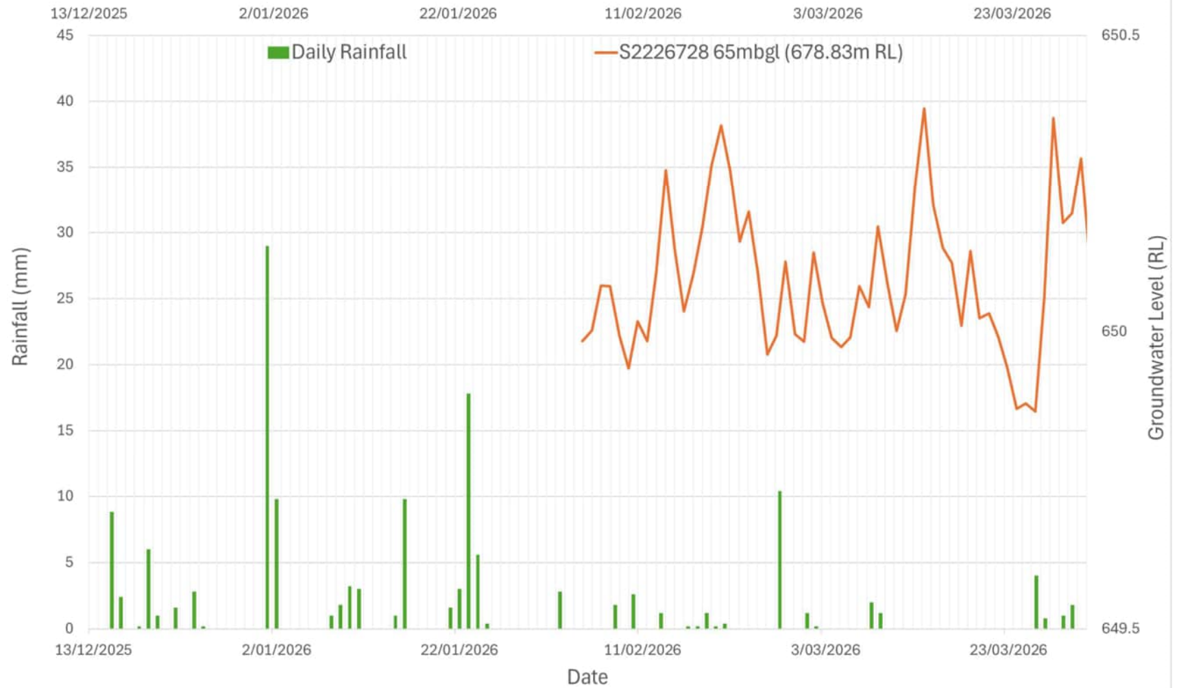
MDD491 - Vibrating Wire Piezometers (13 Dec 2025 to 31 Mar 2026)
