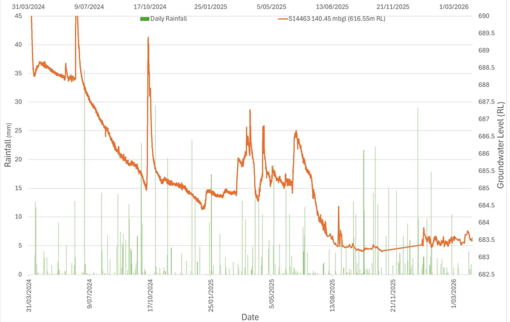
MDD289 - Vibrating Wire Piezometers (31/3/2024 to 31/3/2026)
