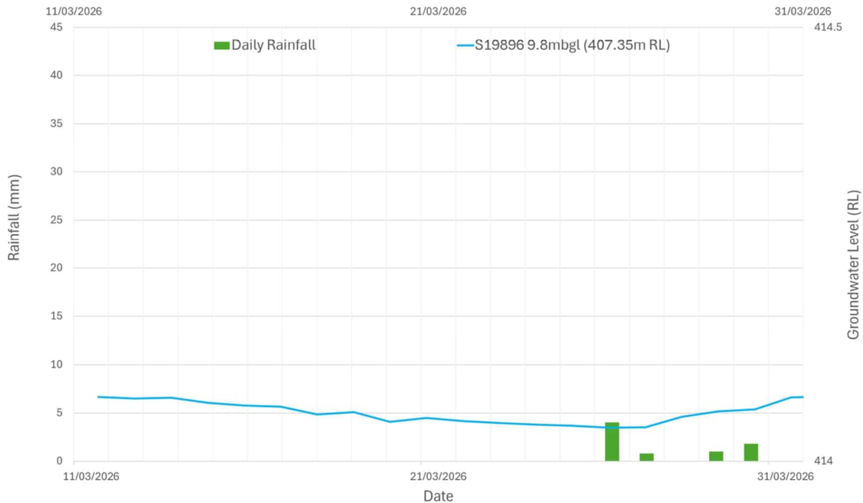
MDD508 - Vibrating Wire Piezometers (11 Mar 2026 to 31 Mar 2026)
