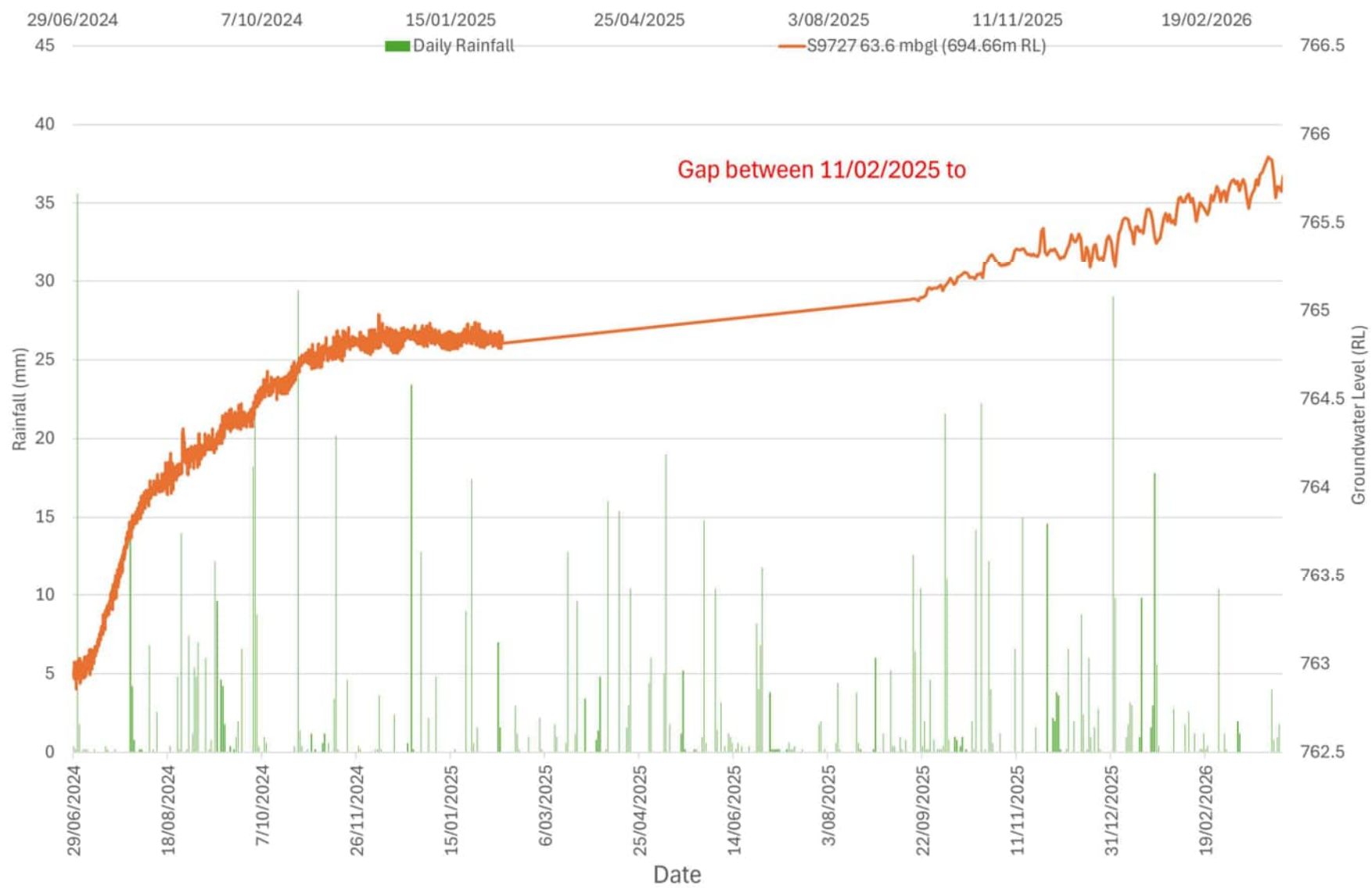
MDD327 - Vibrating Wire Piezometers (29/6/2024 to 31/3/2026)
