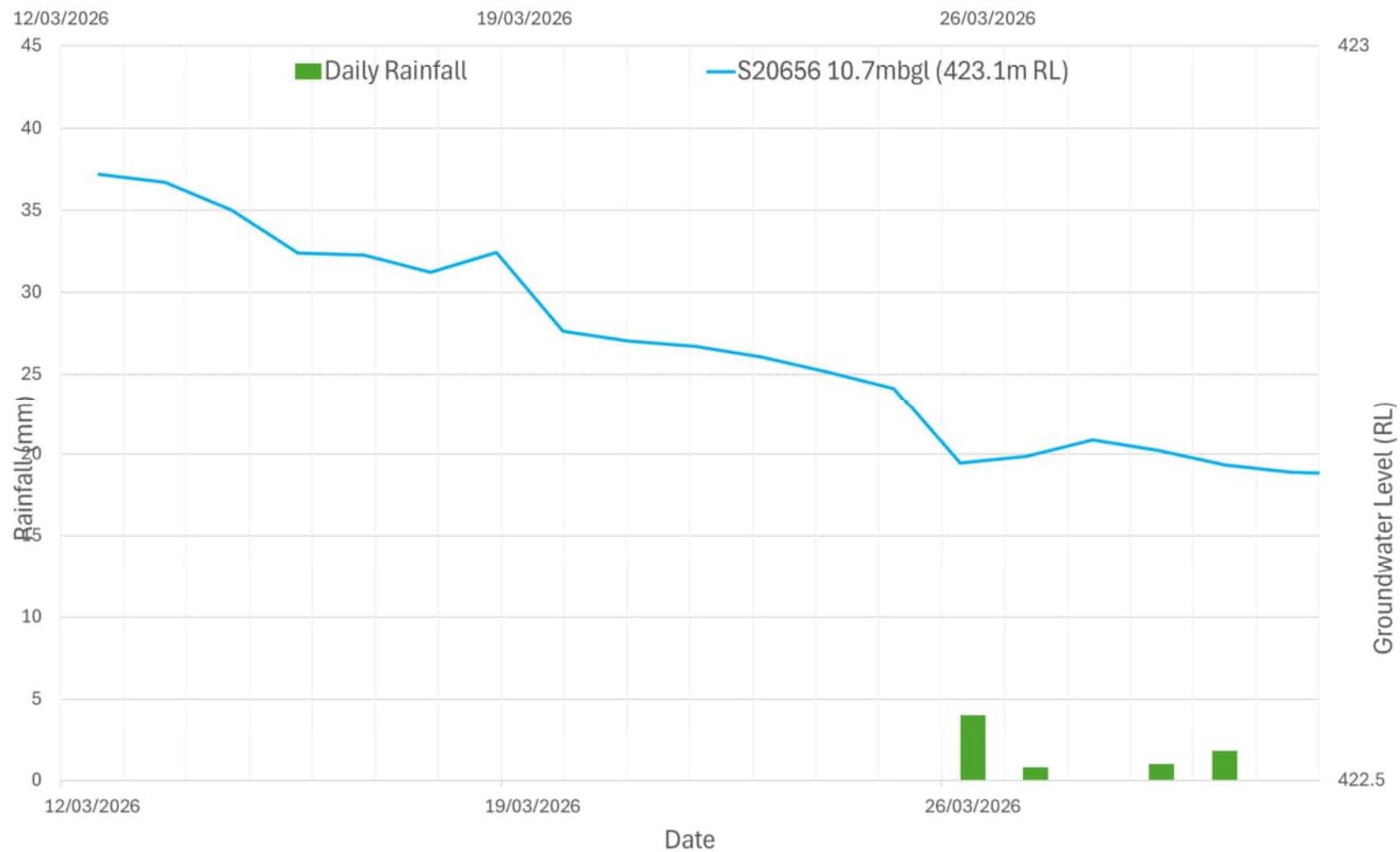
MDD511 - Vibrating Wire Piezometers (12 Mar 2026 to 31 Mar 2026)
