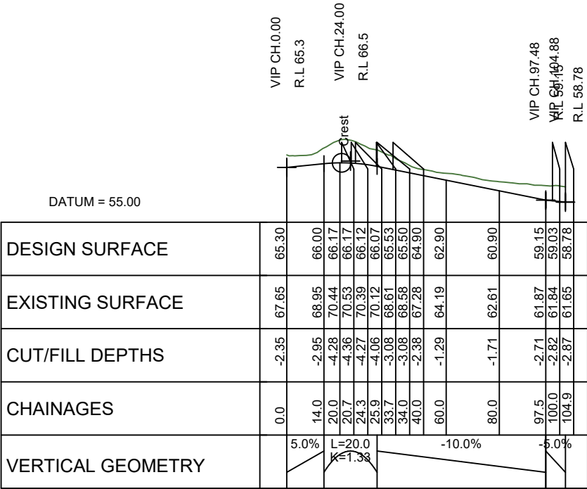
LONGITUDINAL SECTION JOAL 39 SCALE HORIZ=1:2000 @ A1 VERT=1:1000 @ A1
