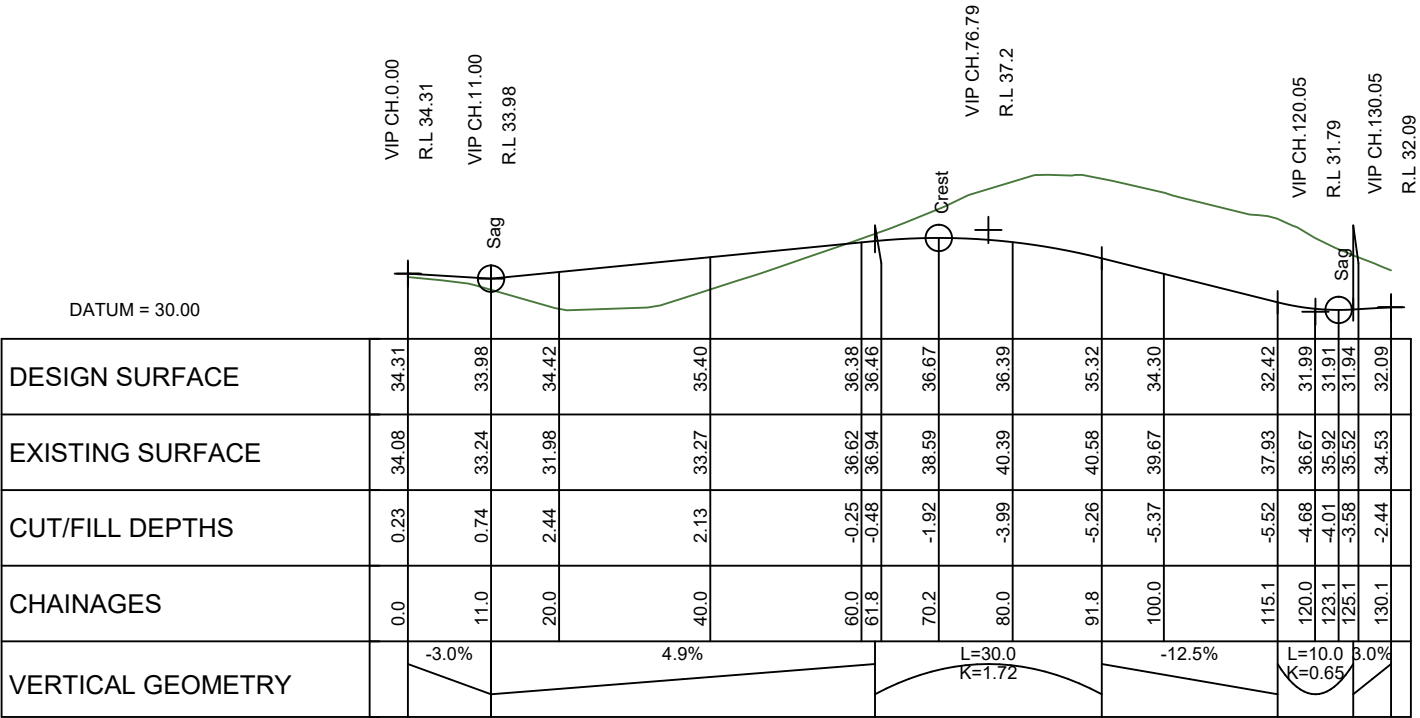
LONGITUDINAL SECTION ROAD 07 SCALE HORIZ=1:1000 @ A1 VERT=1:500 @ A1
