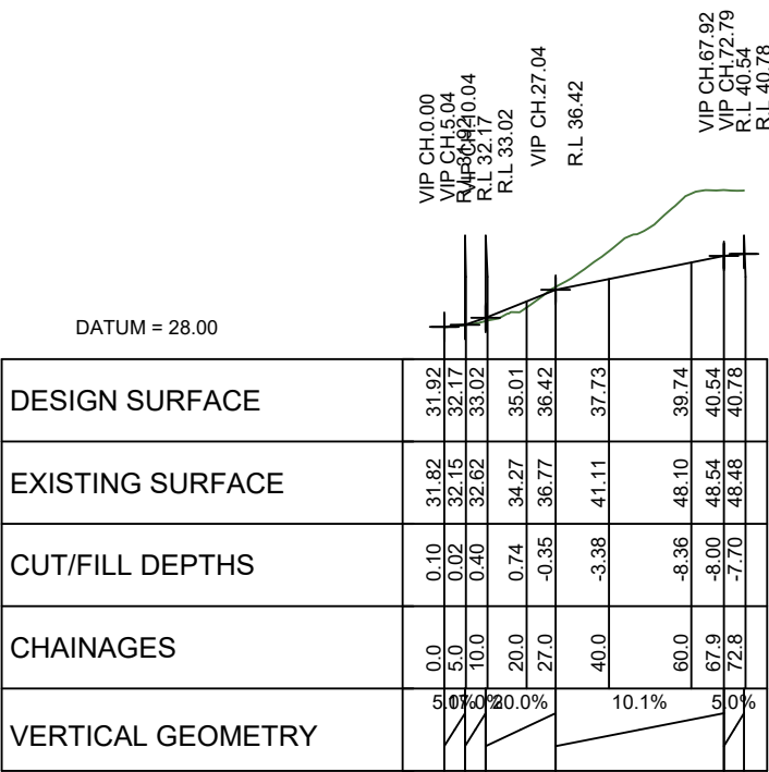
LONGITUDINAL SECTION JOAL 33 SCALE HORIZ=1:2000 @ A1 VERT=1:1000 @ A1
