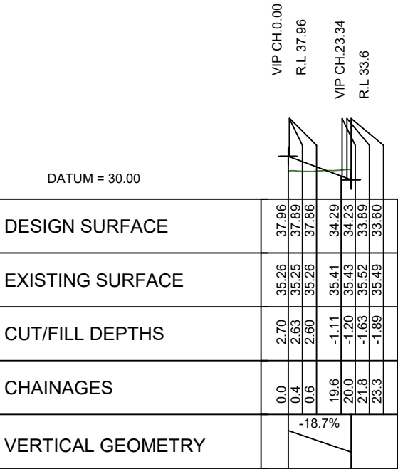
LONGITUDINAL SECTION ROAD 103 SCALE HORIZ=1:2000 @ A1 VERT=1:1000 @ A1
