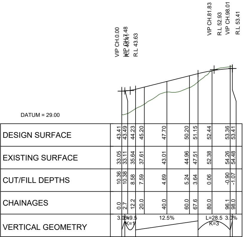
LONGITUDINAL SECTION ROAD 25 SCALE HORIZ=1:2000 @ A1 VERT=1:1000 @ A1
