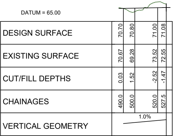
LONGITUDINAL SECTION ROAD 21 SCALE HORIZ=1:2000 @ A1 VERT=1:1000 @ A1
