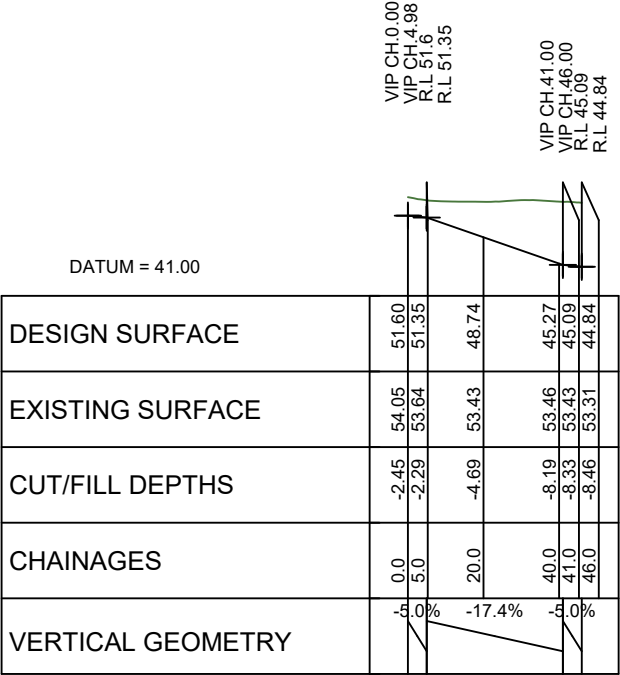
LONGITUDINAL SECTION JOAL 31 SCALE HORIZ=1:2000 @ A1 VERT=1:1000 @ A1
