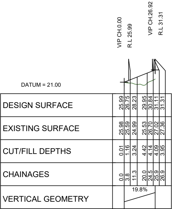
LONGITUDINAL SECTION ROAD 101 SCALE HORIZ=1:2000 @ A1 VERT=1:1000 @ A1
