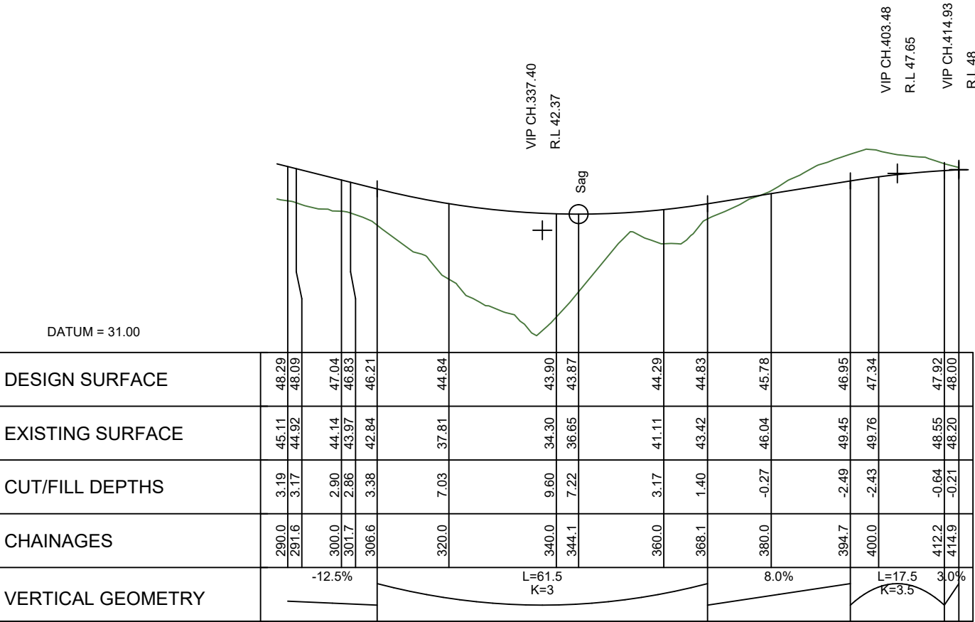
LONGITUDINAL SECTION ROAD 05 SCALE HORIZ=1:1000 @ A1 VERT=1:500 @ A1
