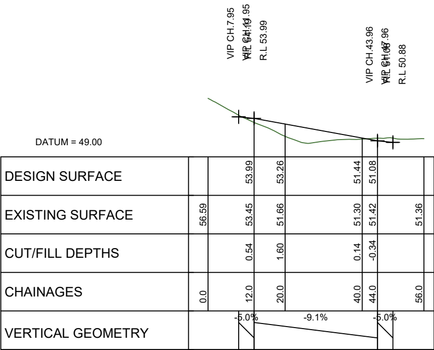
LONGITUDINAL SECTION JOAL 15 SCALE HORIZ=1:1000 @ A1 VERT=1:500 @ A1
