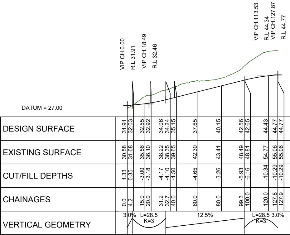
LONGITUDINAL SECTION ROAD 26 SCALE HORIZ=1:2000 @ A1 VERT=1:1000 @ A1
