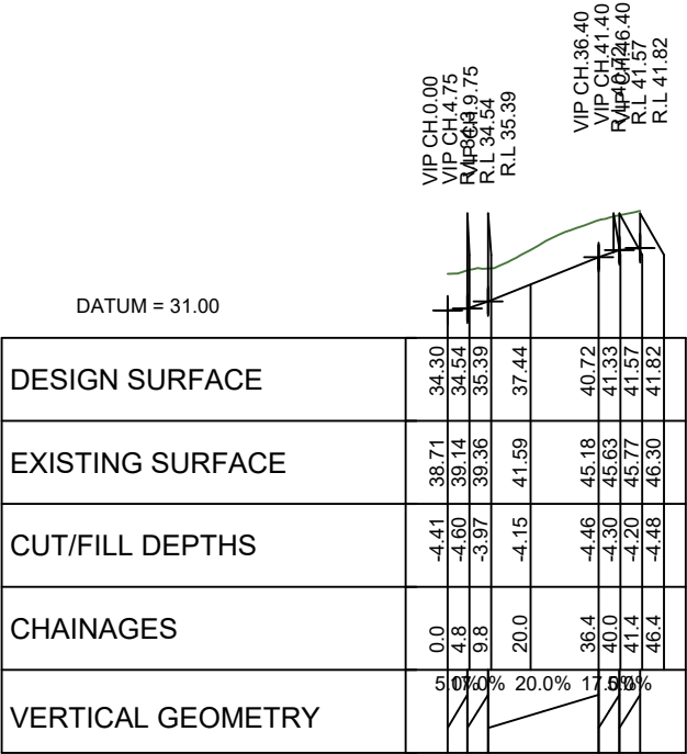
LONGITUDINAL SECTION JOAL 28 SCALE HORIZ=1:2000 @ A1 VERT=1:1000 @ A1
